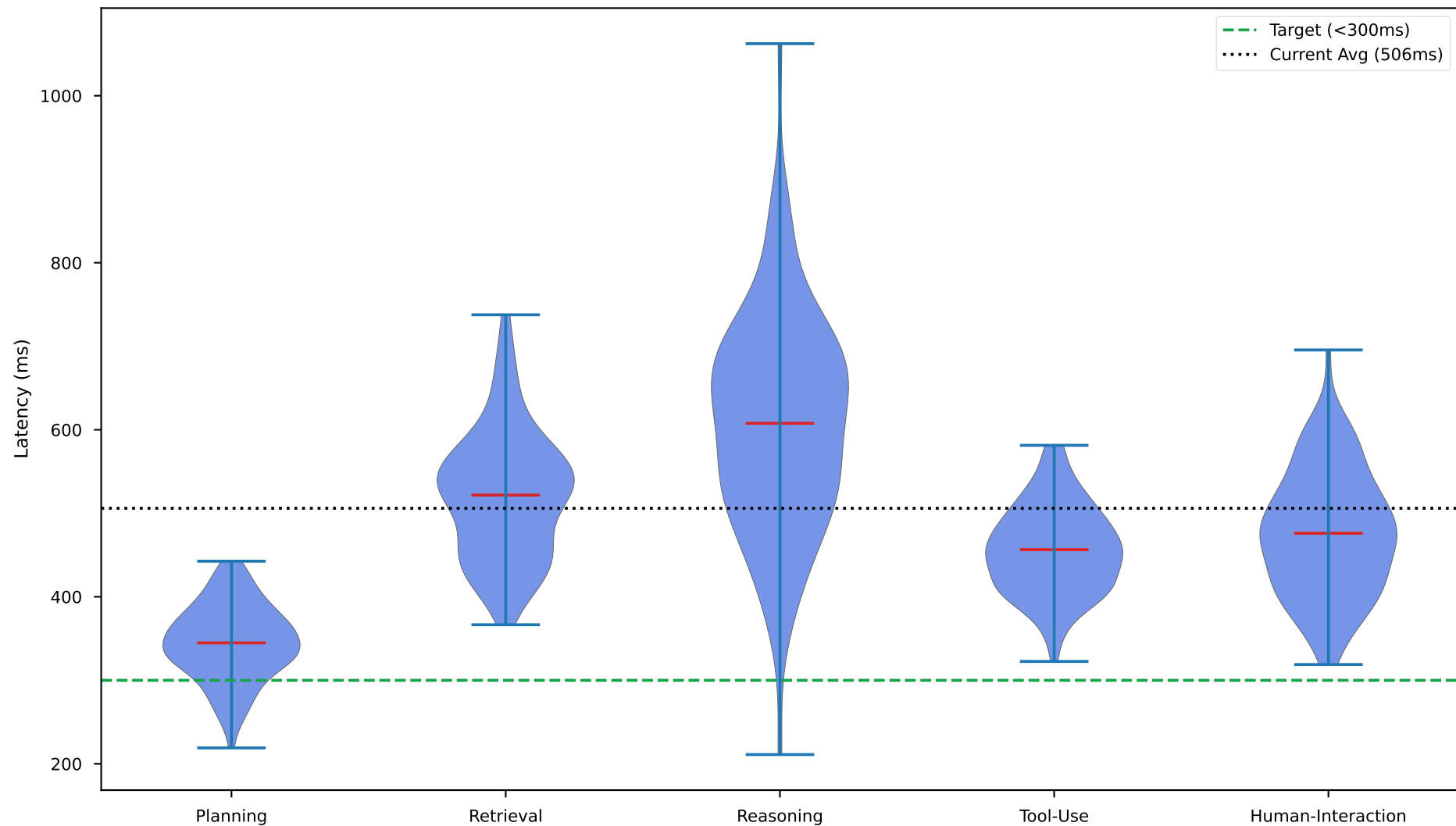
Detection Latency Distribution by Category
