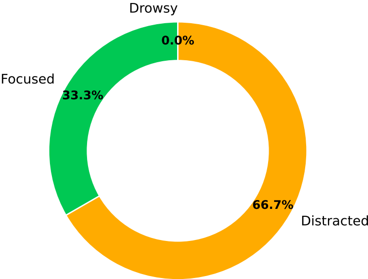
Attention Breakdown
