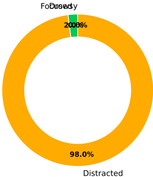
Attention Breakdown
