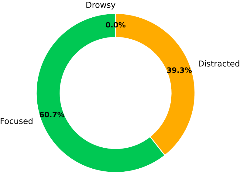
Attention Breakdown
