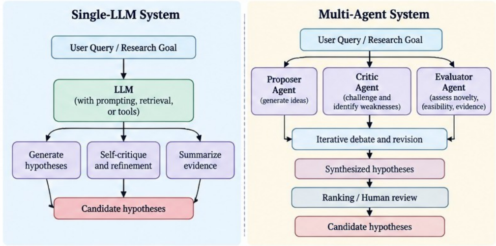
Fig. 1. Conceptual comparison of single-LLM and multi-agent systems for scientific hypothesis generation. Single-LLM systems rely on one model with prompting, retrieval or tool use, while multi-agent systems employ specialized agents that interact through debate, critique and iterative revision to produce and refine candidate hypotheses.
