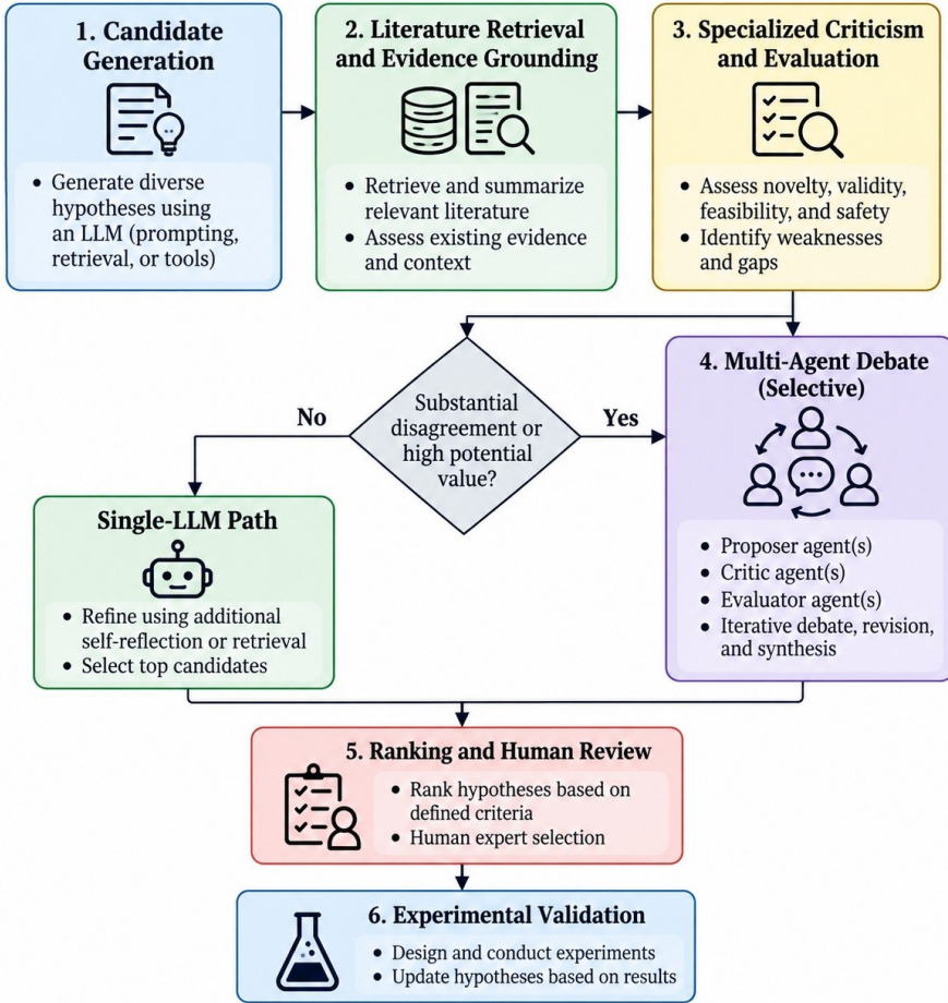
Fig. 2. Proposed hybrid workflow for scientific hypothesis generation. The system begins with candidate generation using a single LLM, followed by literature retrieval and specialized evaluation. Multi-agent debate is activated selectively when there is substantial disagreement among evaluators or high potential value in further exploration. The final candidates are ranked and reviewed by human experts before experimental validation.
