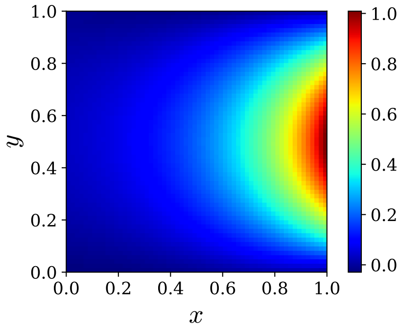
PINN Prediction (No Autodiff)
