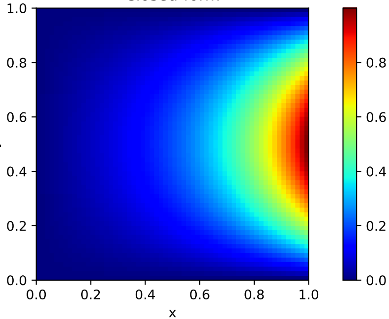
Closed-form
