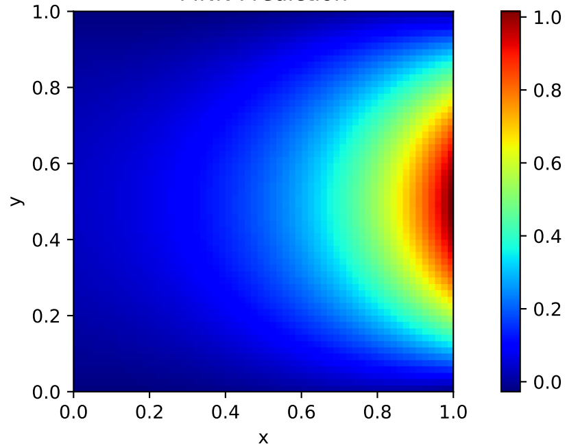
PINN Prediction
