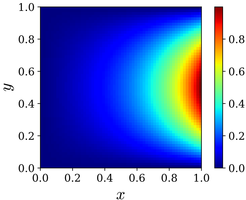
Analytic Solution
