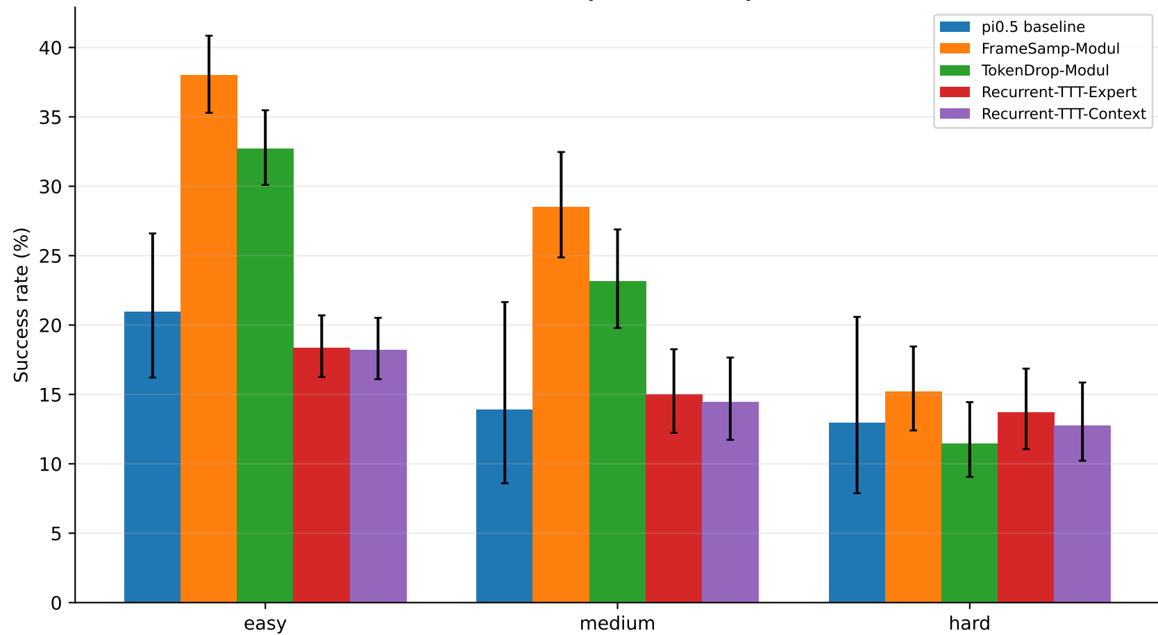
Success by task difficulty
