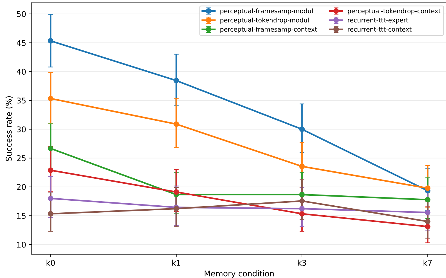
Success decays as relevant memory is pushed farther back
