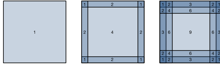
Figure 7.3.1 Pixel utilization for convolutions of size 1 \times 1 , 2 \times 2 , and 3 \times 3 respectively.
