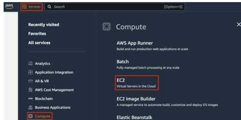
Figure 23.3.1 Open the EC2 console.
