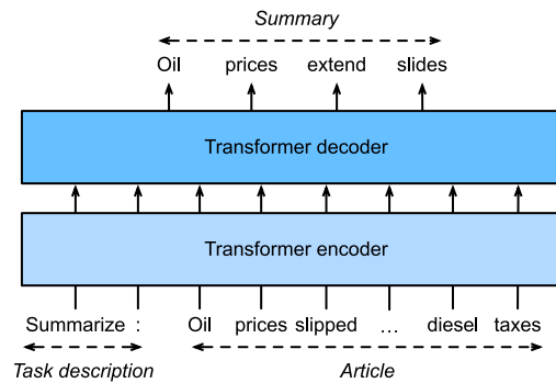
Figure 11.8.4 Fine-tuning T5 for text summarization. Both the task description and article tokens are fed into the Transformer encoder for predicting the summary.
