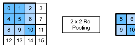
Figure 14.8.3 A 2 \times 2 region of interest pooling layer.
