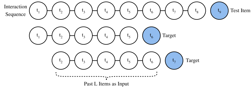
Figure 21.7.2 Illustration of the data generation process
