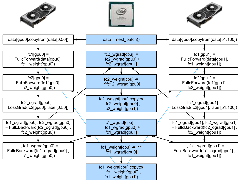
Figure 13.3.1 The computational graph and its dependencies of a two-layer MLP on a CPU and two GPUs.
