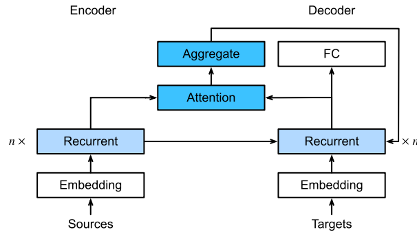
Figure 11.4.2 Layers in an RNN encoder-decoder model with the Bahdanau attention mechanism.
