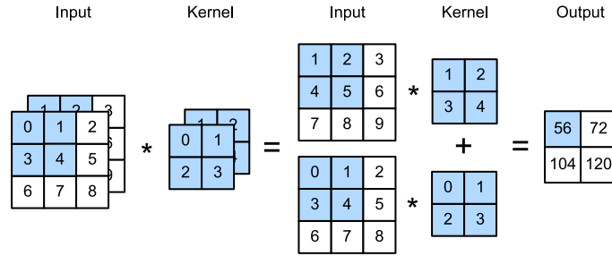
Figure 7.4.1 Cross-correlation computation with 2 input channels.
