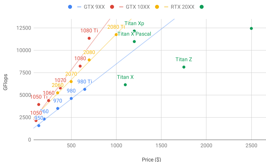
Figure 23.5.1 Floating-point compute power and price comparison.
