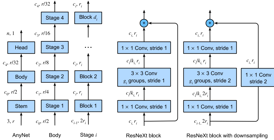
Figure 8.8.1 The AnyNet design space. The numbers (c, r) along each arrow indicate the number of channels c and the resolution r \times r of the images at that point. From left to right: generic network structure composed of stem, body, and head; body composed of four stages; detailed structure of a stage; two alternative structures for blocks, one without downsampling and one that halves the resolution in each dimension. Design choices include depth d_i , the number of output channels c_i , the number of groups g_i , and bottleneck ratio k_i for any stage i .
