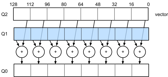
Figure 13.4.5 128 bit NEON vectorization.
