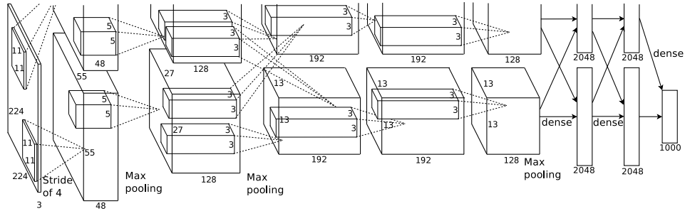
Figure 13.5.1 Model parallelism in the original AlexNet design due to limited GPU memory.
