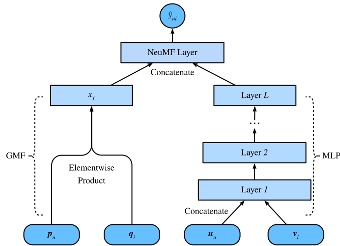
Figure 21.6.1 Illustration of the NeuMF model
