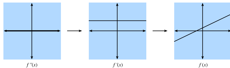
Figure 22.3.3 If we assume the second derivative is zero, then the first derivative is constant, which implies the function itself is a straight line.
