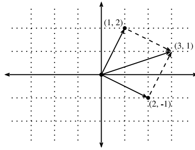
Figure 22.1.3 We can visualize vector addition by first following one vector, and then another.
