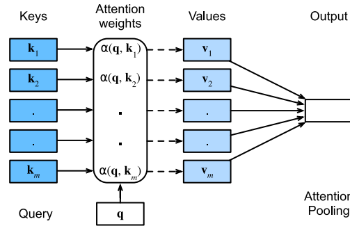
Figure 11.1.1 The attention mechanism computes a linear combination over values \mathbf{v}_i via attention pooling, where weights are derived according to the compatibility between a query \mathbf{q} and keys \mathbf{k}_i .
