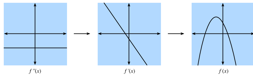
Figure 22.3.2 If we assume the second derivative is a negative constant, then the first derivative is decreasing, which implies the function itself has a maximum.
