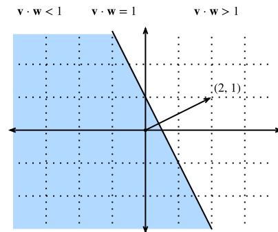
Figure 22.1.6 If we now consider the inequality version of the expression, we see that our hyperplane (in this case: just a line) separates the space into two halves.
