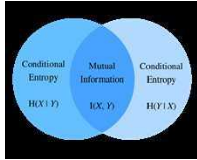
Figure 22.11.1 Mutual informations relationship with joint entropy and conditional entropy.
