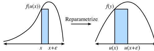
Figure 22.5.2 Visualizing the transformation of a single thin rectangle under the change of variables.
