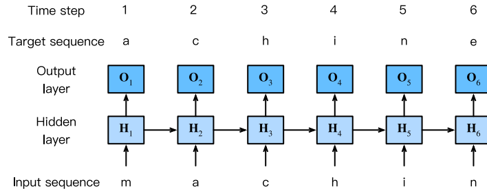
Figure 9.4.2 A character-level language model based on the RNN. The input and target sequences are machin and achine, respectively.
