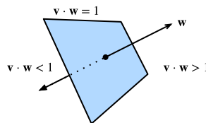
Figure 22.1.7 Hyperplanes in any dimension separate the space into two halves.
