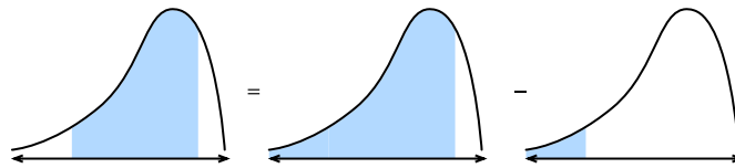
Figure 22.5.1 Visualizing why we may reduce the problem of computing the area under a curve between two points to computing the area to the left of a point.
