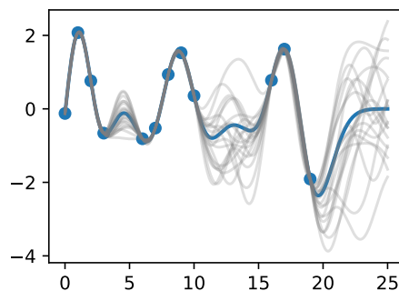
Figure 18.1.4 Posterior samples, alongside posterior mean, which can be used for point predictions, in blue.
