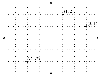
Figure 22.1.1 An illustration of visualizing vectors as points in the plane. The first component of the vector gives the x-coordinate, the second component gives the y-coordinate. Higher dimensions are analogous, although much harder to visualize.
