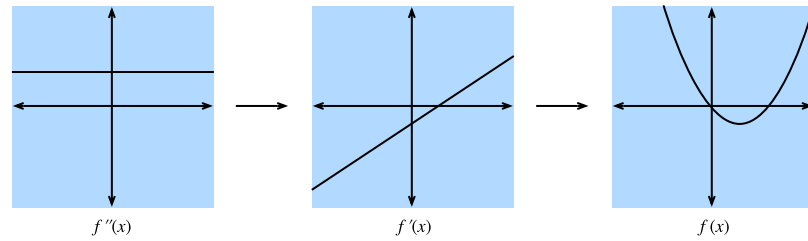
Figure 22.3.1 If we assume the second derivative is a positive constant, then the first derivative is increasing, which implies the function itself has a minimum.
