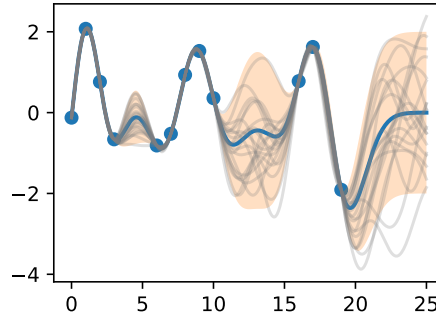
Figure 18.1.5 Posterior samples, including 95% credible set.
