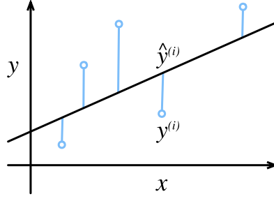
Figure 3.1.1 Fitting a linear regression model to one-dimensional data.
