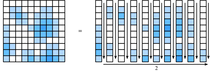
Figure 22.5.3 Illustrating how to decompose a sum over many squares as a sum over first the columns (1), then adding the column sums together (2).
