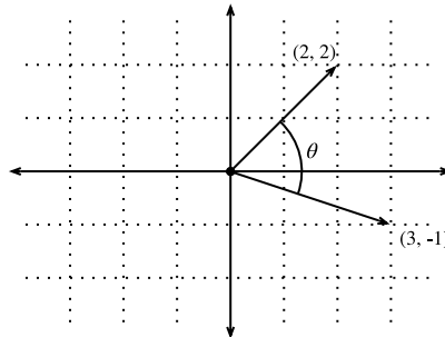
Figure 22.1.4 Between any two vectors in the plane there is a well defined angle \theta . We will see this angle is intimately tied to the dot product.
