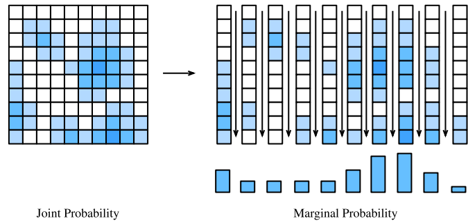
Figure 22.6.1 By summing along the columns of our array of probabilities, we are able to obtain the marginal distribution for just the random variable represented along the x-axis.
