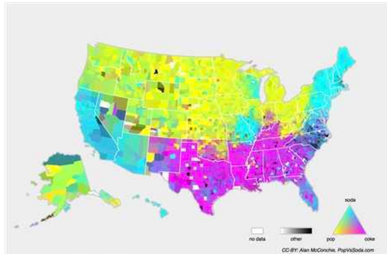
Figure 4.7.3 Concept shift on soft drink names in the United States.
