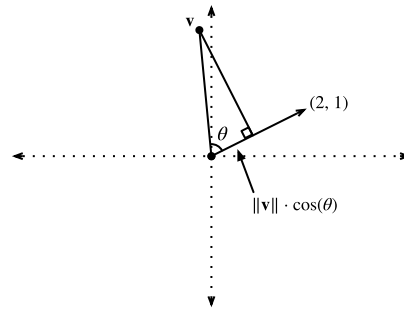
Figure 22.1.5 Recalling trigonometry, we see the formula \|v\| \cos(\theta) is the length of the projection of the vector v onto the direction of w
