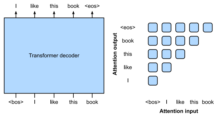
Figure 11.8.6 Left: Pretraining GPT with language modeling. The target sequence is the input sequence shifted by one token. Both <bos> and <eos> are special tokens marking the beginning and end of sequences, respectively. Right: Attention pattern in the Transformer decoder. Each token along the vertical axis attends to only its past tokens along the horizontal axis (causal).
