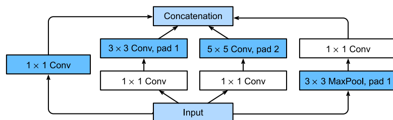
Figure 8.4.1 Structure of the Inception block.
