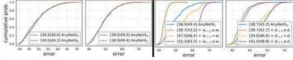
Figure 8.8.2 Comparing error empirical distribution functions of design spaces. AnyNet A is the original design space; AnyNet B ties the bottleneck ratios, AnyNet C also ties group widths, AnyNet D increases the network depth across stages. From left to right: (i) tying bottleneck ratios has no effect on performance, (ii) tying group widths has no effect on performance, (iii) increasing network widths (channels) across stages improves performance, (iv) increasing network depths across stages improves performance. Figure courtesy of Radosavovic et al. (2020).
