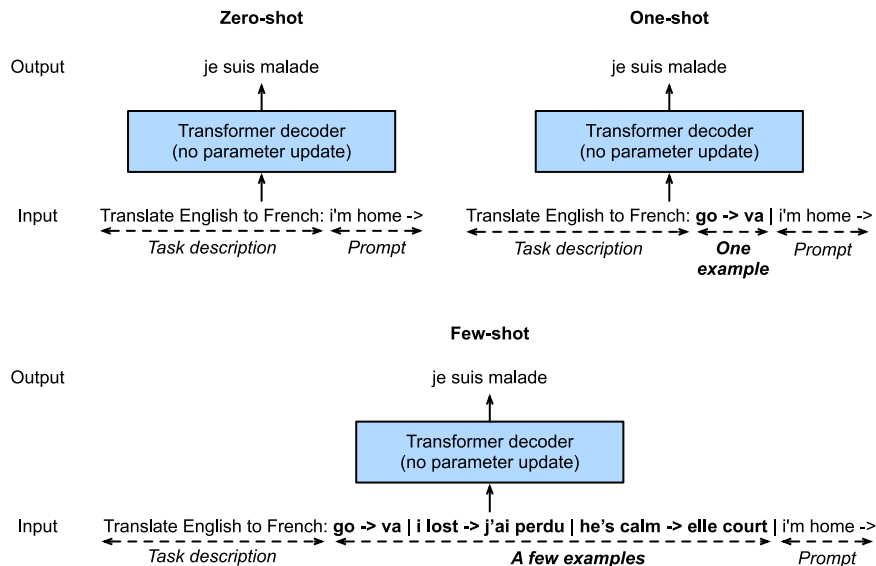
Figure 11.8.7 Zero-shot, one-shot, few-shot in-context learning with language models (Transformer decoders). No parameter update is needed.
