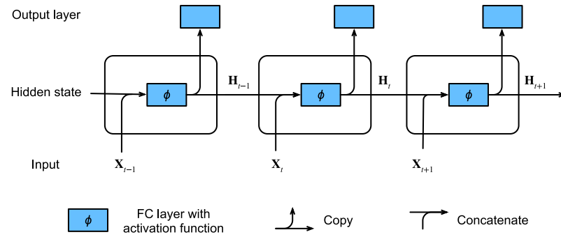
Figure 9.4.1 An RNN with a hidden state.
