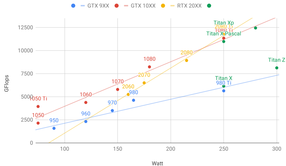
Figure 23.5.2 Floating-point compute power and energy consumption.
