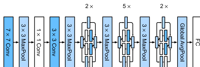
Figure 8.4.2 The GoogLeNet architecture.
