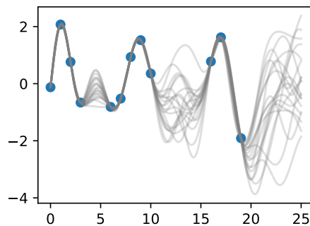
Figure 18.1.3 Sample posterior functions, once we have observed the data.
