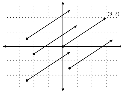
Figure 22.1.2 Any vector can be visualized as an arrow in the plane. In this case, every vector drawn is a representation of the vector (3, 2)^T .
