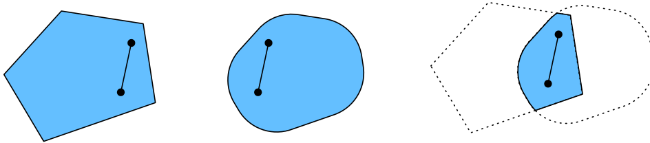
Figure 12.2.2 The intersection between two convex sets is convex.
