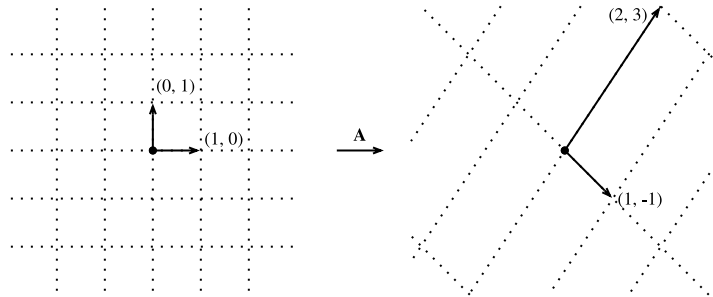
Figure 22.1.8 The matrix \mathbf{A} acting on the given basis vectors. Notice how the entire grid is transported along with it.
