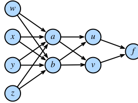
Figure 22.4.1 The function relations above where nodes represent values and edges show functional dependence.
