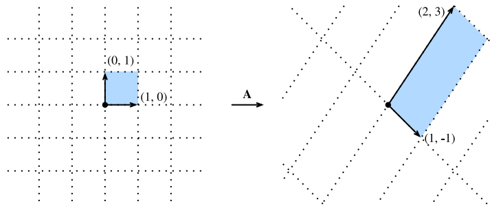
Figure 22.1.9 The matrix \mathbf{A} again distorting the grid. This time, I want to draw particular attention to what happens to the highlighted square.
