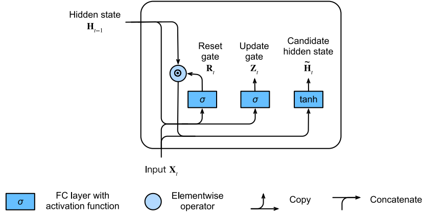
Figure 10.2.2 Computing the candidate hidden state in a GRU model.
