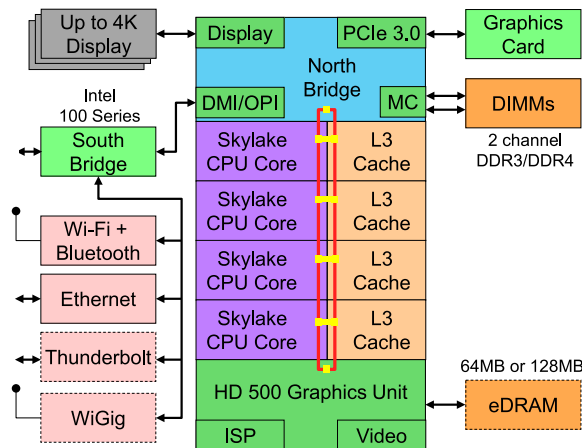
Figure 13.4.3 Intel Skylake consumer quad-core CPU.
