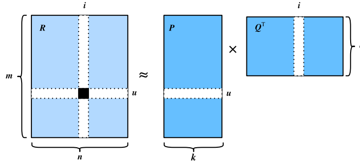
Figure 21.3.1 Illustration of matrix factorization model
