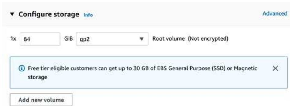
Figure 23.3.7 Modify the hard disk size.
