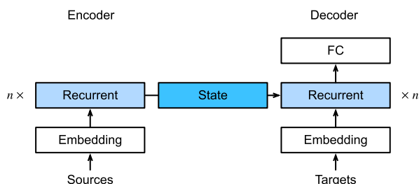
Figure 11.4.1 Sequence to Sequence Model. The state, as generated by the encoder, is the only piece of information shared between the encoder and the decoder.
