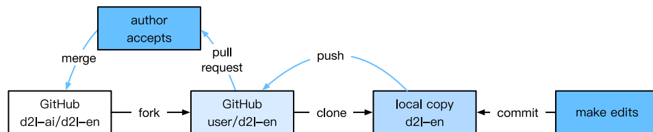
Figure 23.6.2 Contributing to the book.
