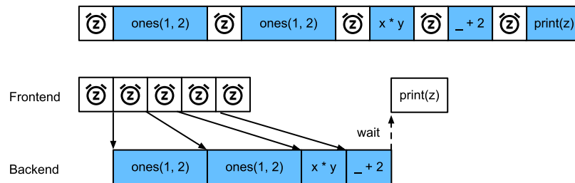
Figure 13.2.3 Interactions of the frontend and backend.
