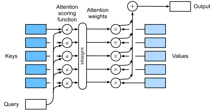
Figure 11.3.1 Computing the output of attention pooling as a weighted average of values, where weights are computed with the attention scoring function a and the softmax operation.
