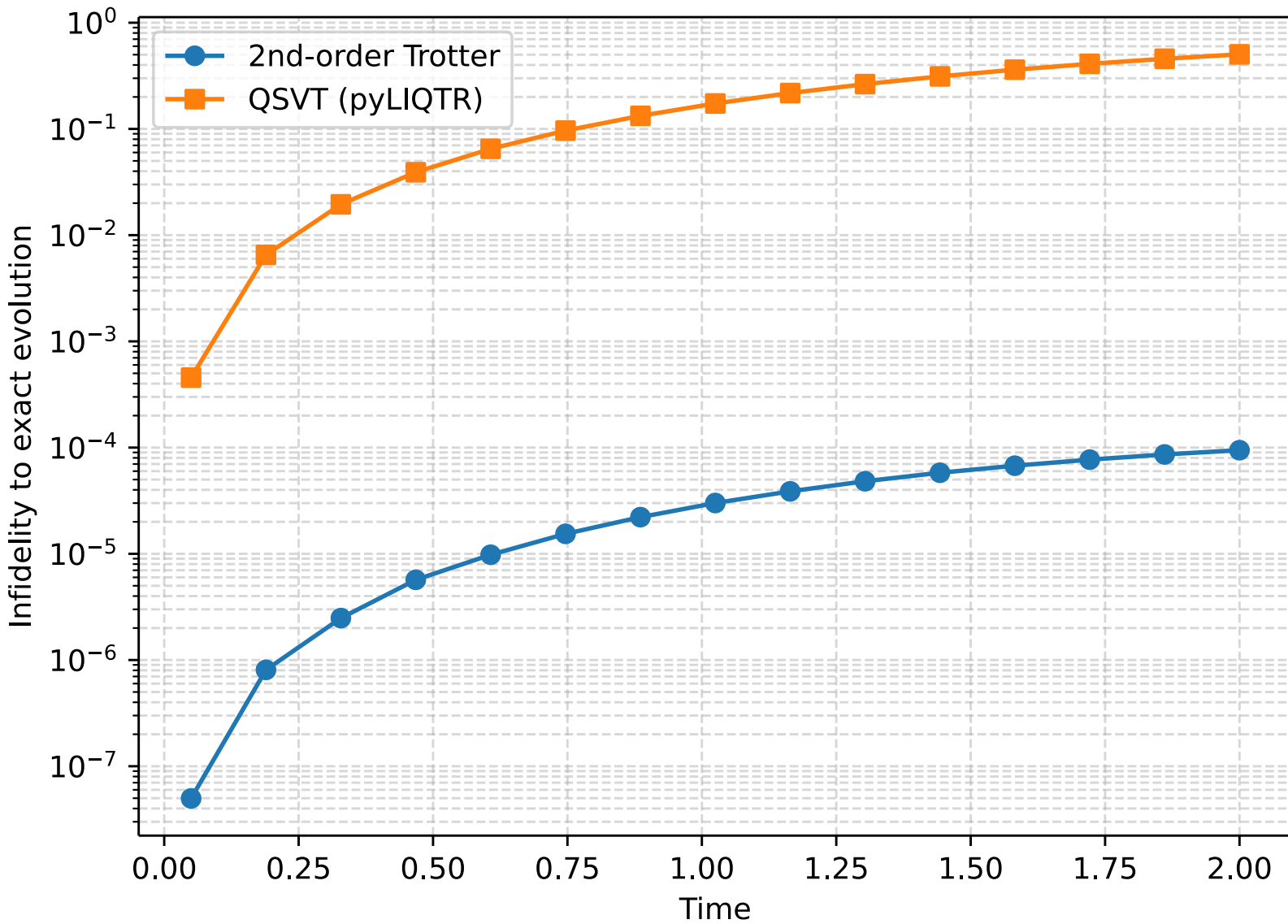
State evolution error vs time
