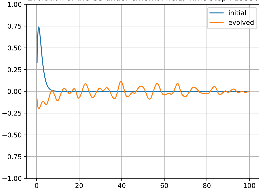
Evolution of the GS under external field, Time step : 19350
