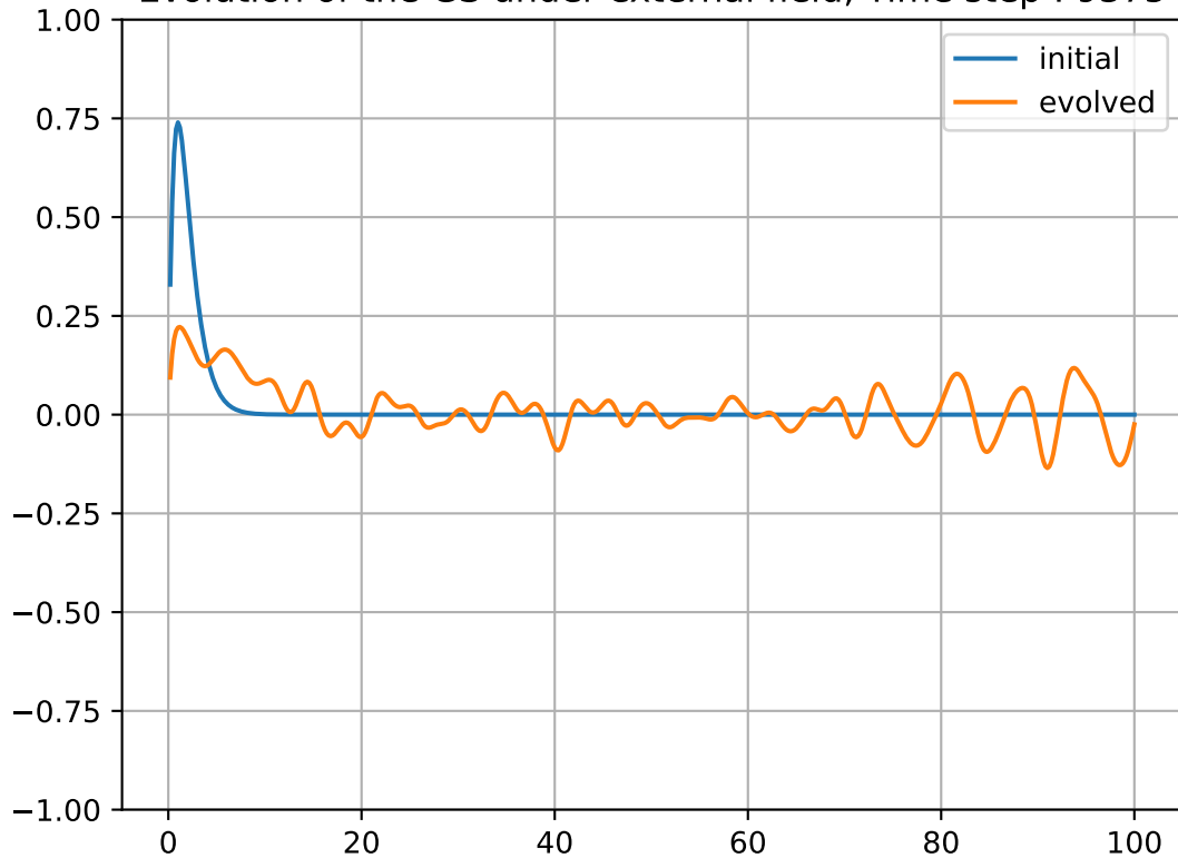
Evolution of the GS under external field, Time step : 9375
