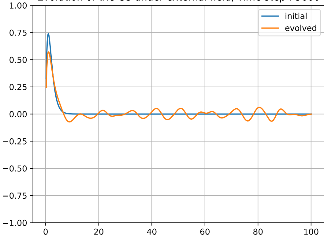
Evolution of the GS under external field, Time step : 5600
