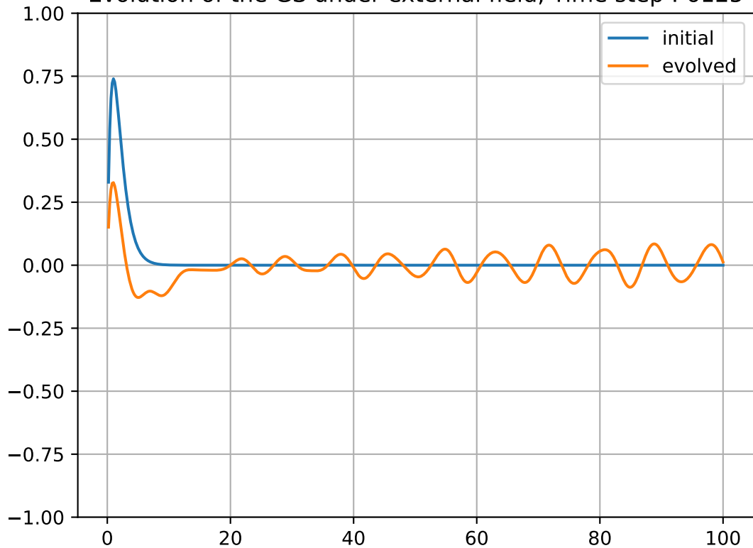
Evolution of the GS under external field, Time step : 6125
