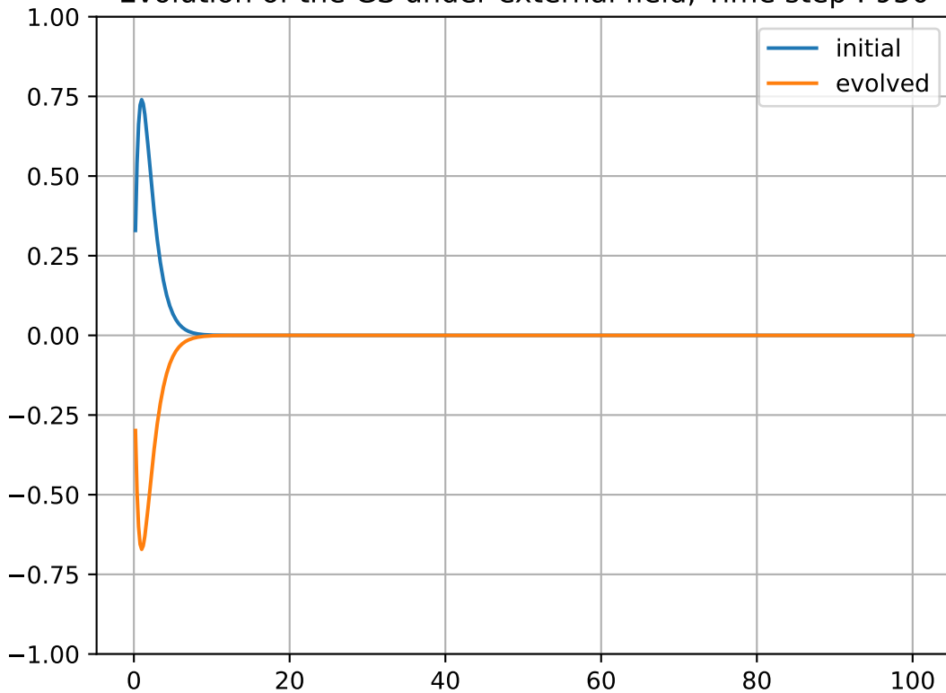
Evolution of the GS under external field, Time step : 950
