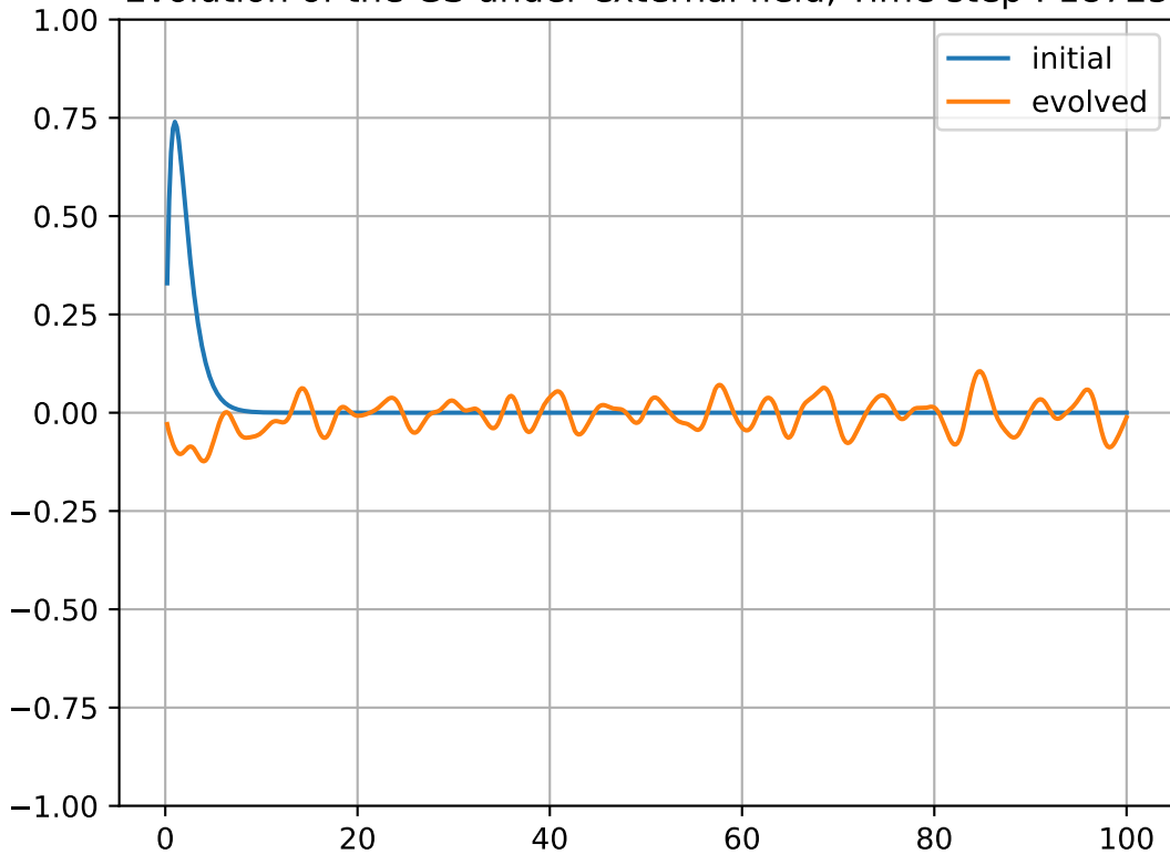
Evolution of the GS under external field, Time step : 18725
