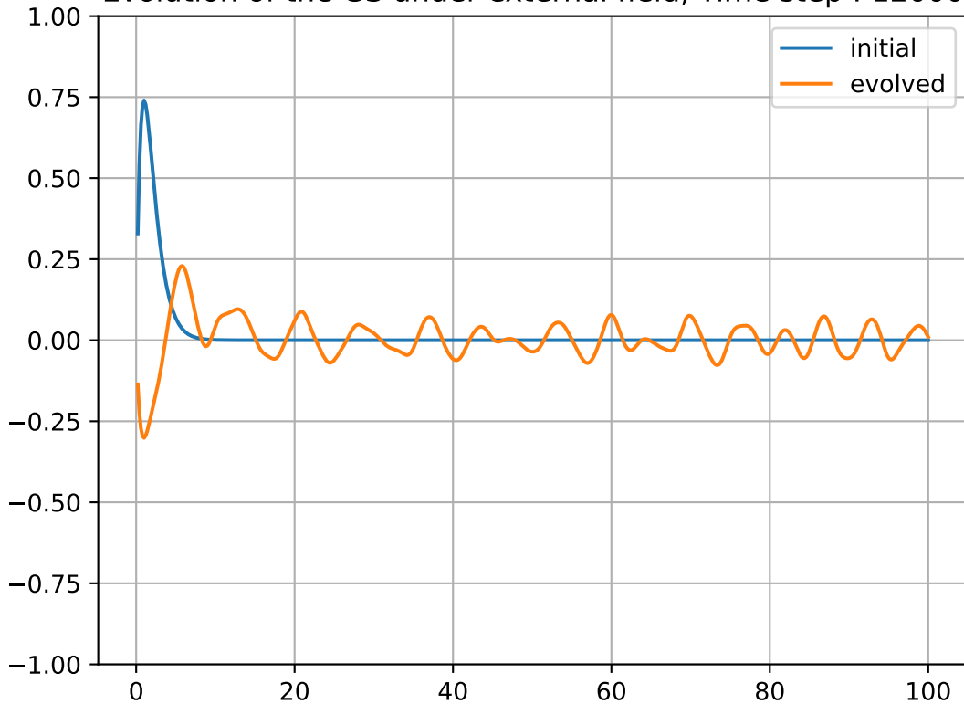
Evolution of the GS under external field, Time step : 12000
