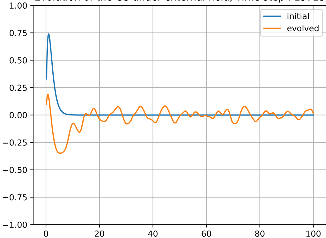
Evolution of the GS under external field, Time step : 15725
