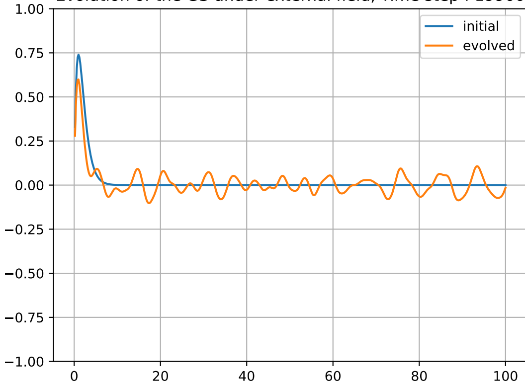
Evolution of the GS under external field, Time step : 19900
