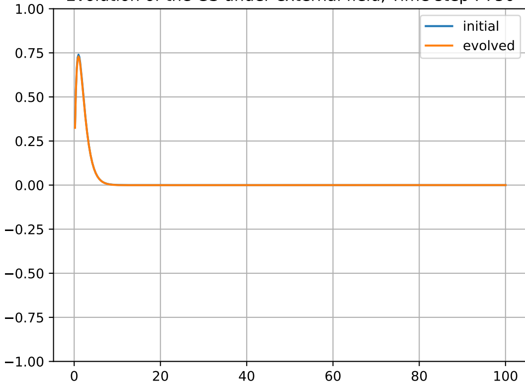
Evolution of the GS under external field, Time step : 750
