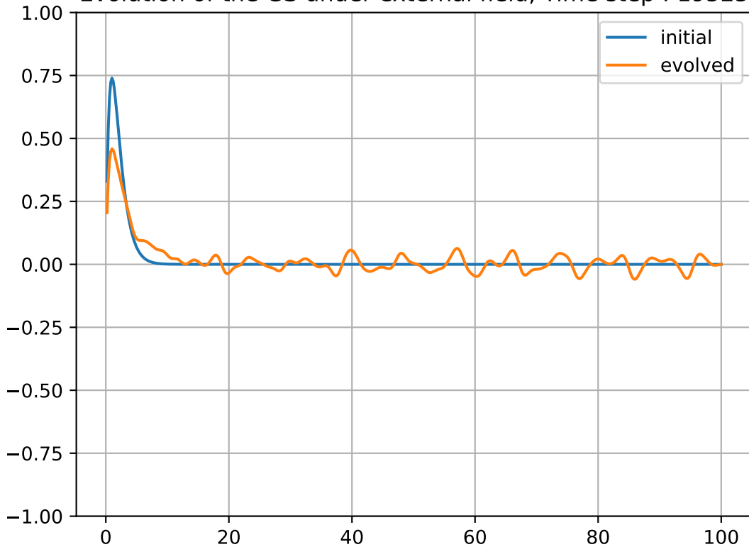
Evolution of the GS under external field, Time step : 19525
