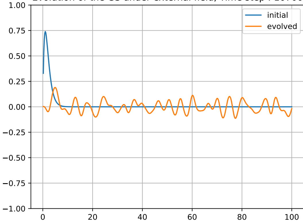
Evolution of the GS under external field, Time step : 10700
