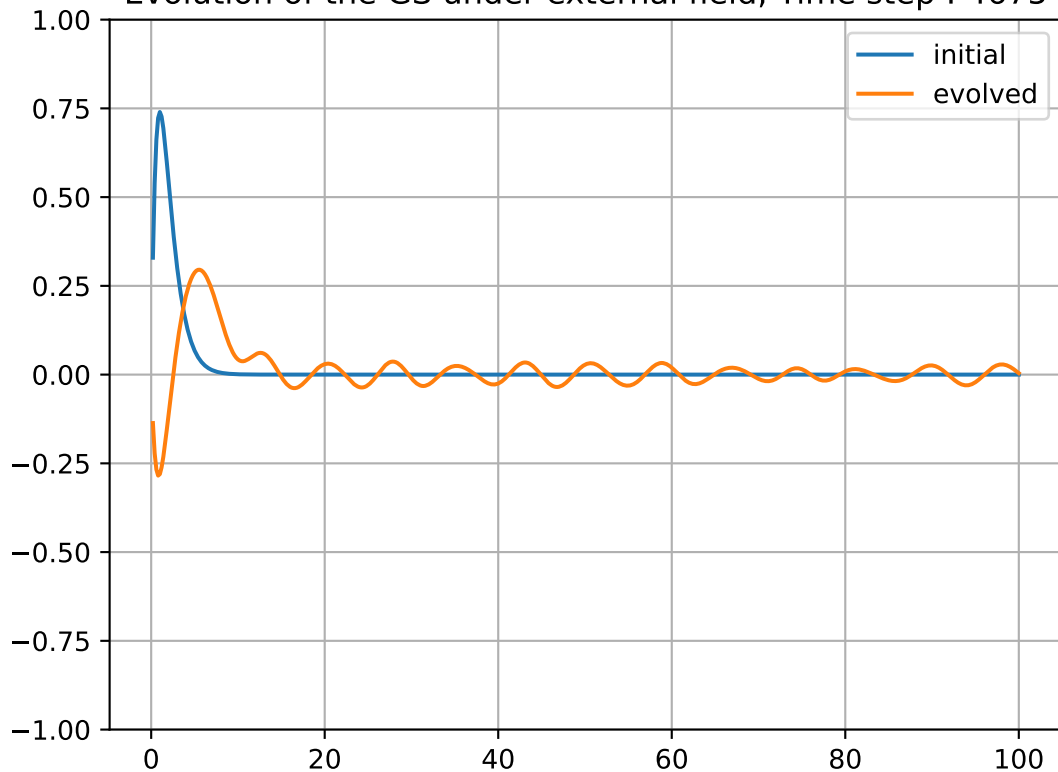
Evolution of the GS under external field, Time step : 4675
