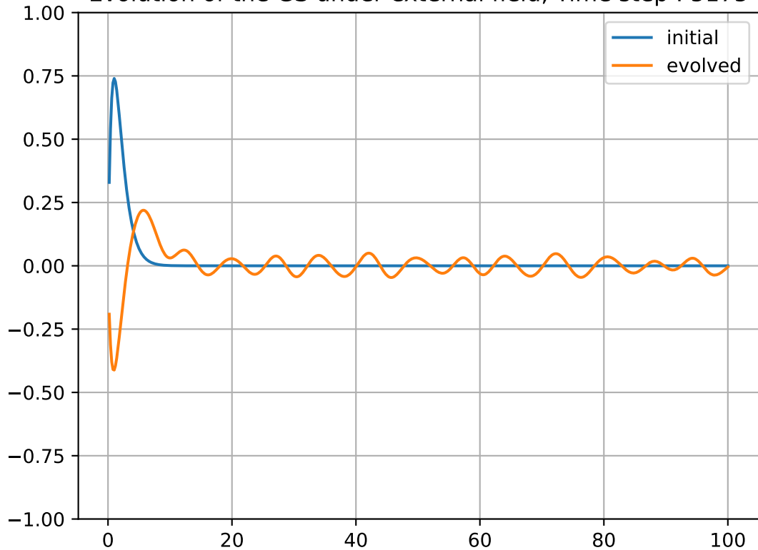
Evolution of the GS under external field, Time step : 5175
