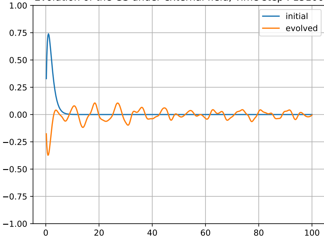
Evolution of the GS under external field, Time step : 15100
