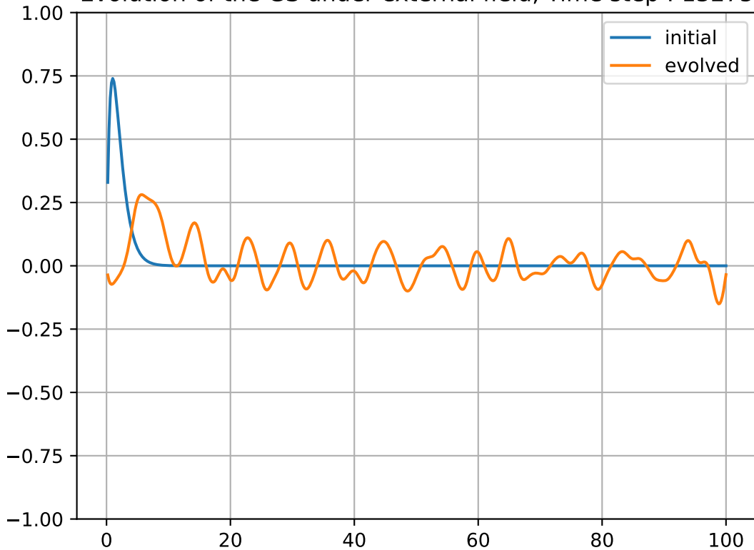
Evolution of the GS under external field, Time step : 13275
