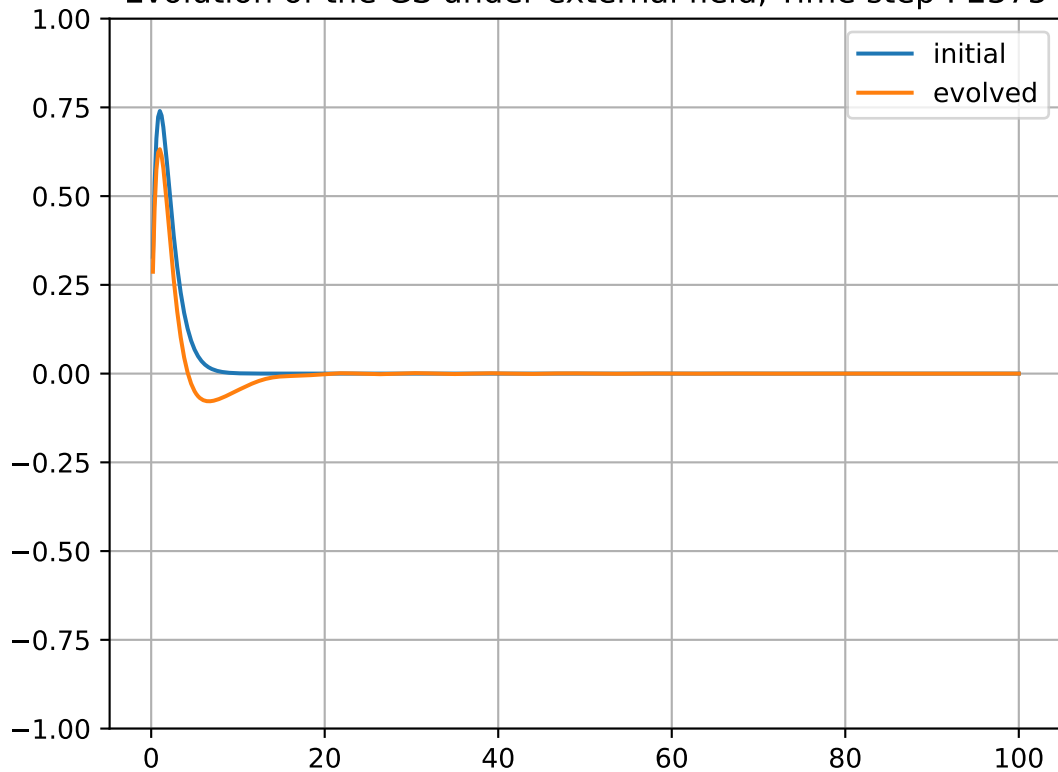
Evolution of the GS under external field, Time step : 2375
