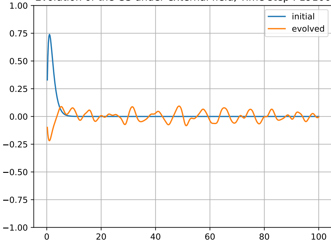
Evolution of the GS under external field, Time step : 19100
