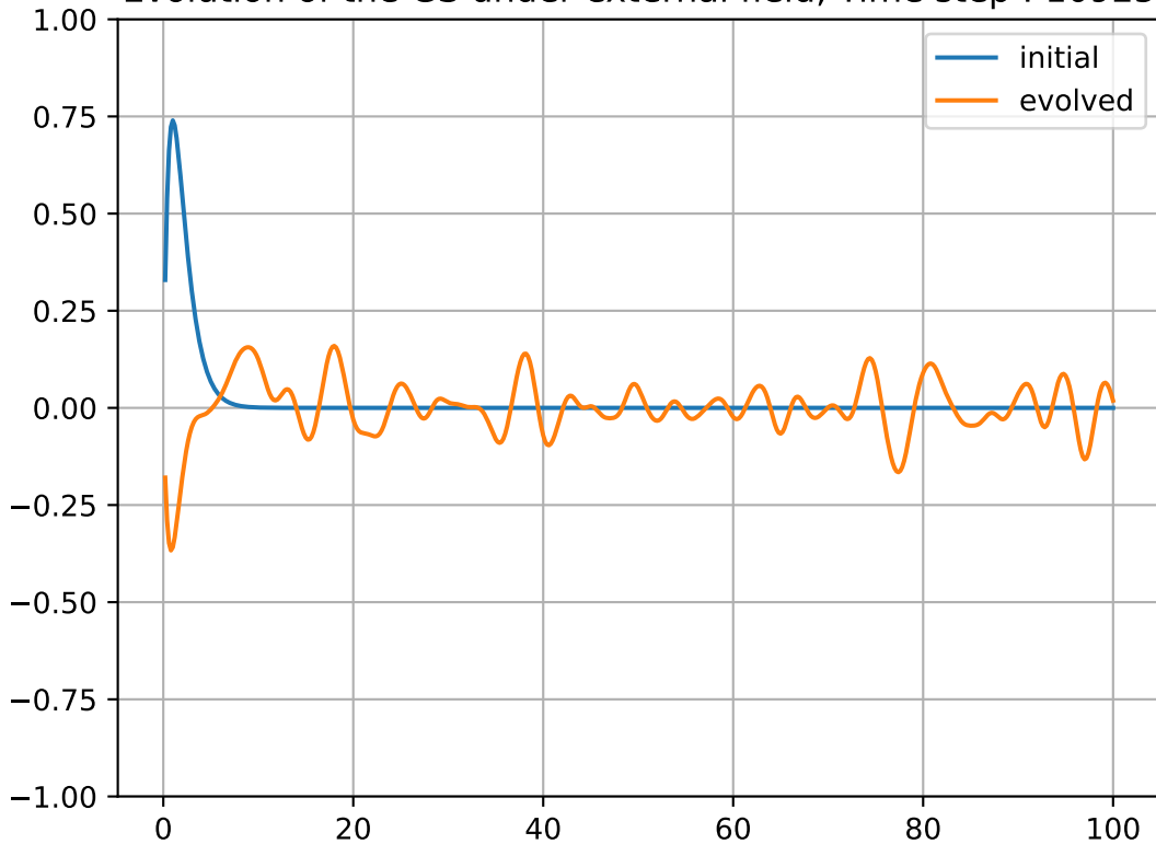
Evolution of the GS under external field, Time step : 10925
