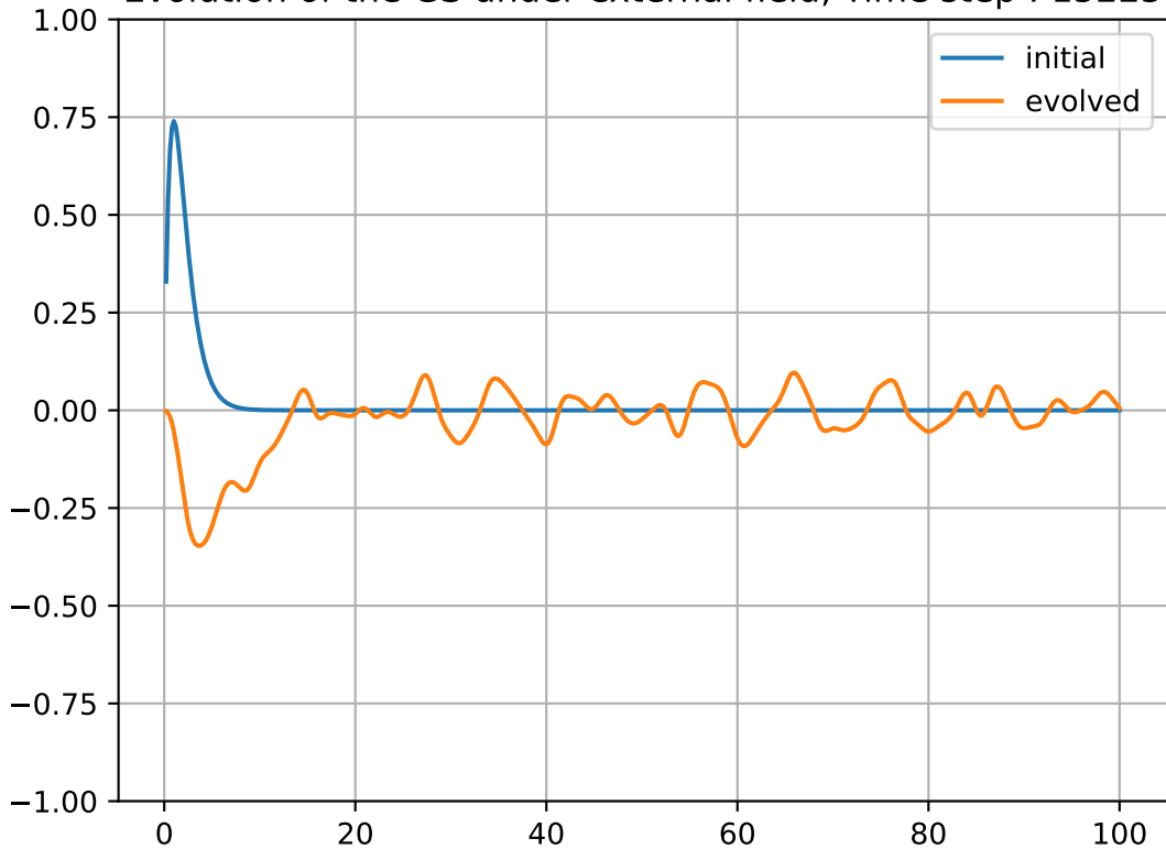
Evolution of the GS under external field, Time step : 15225
