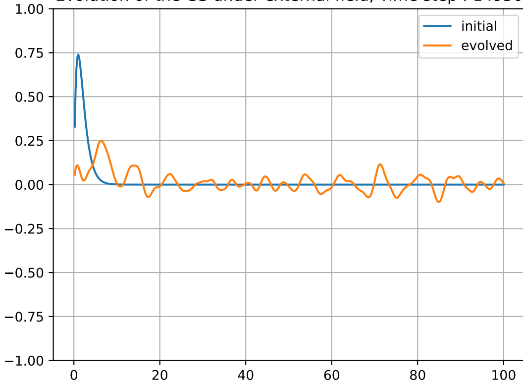
Evolution of the GS under external field, Time step : 14950
