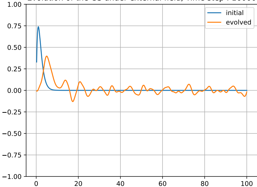
Evolution of the GS under external field, Time step : 16000
