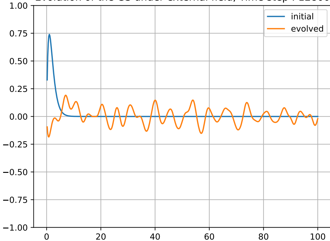
Evolution of the GS under external field, Time step : 12800
