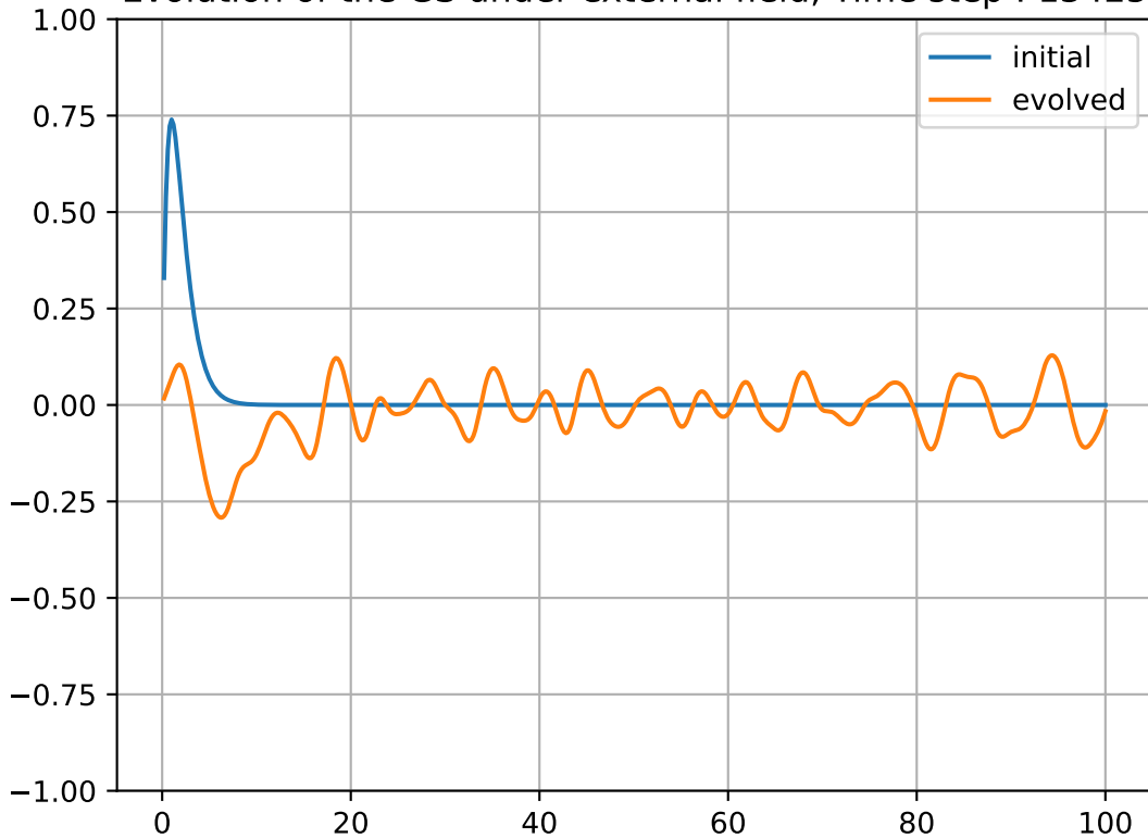
Evolution of the GS under external field, Time step : 13425
