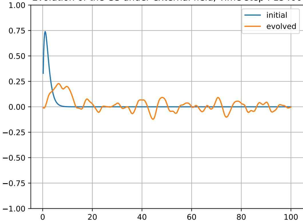
Evolution of the GS under external field, Time step : 15400
