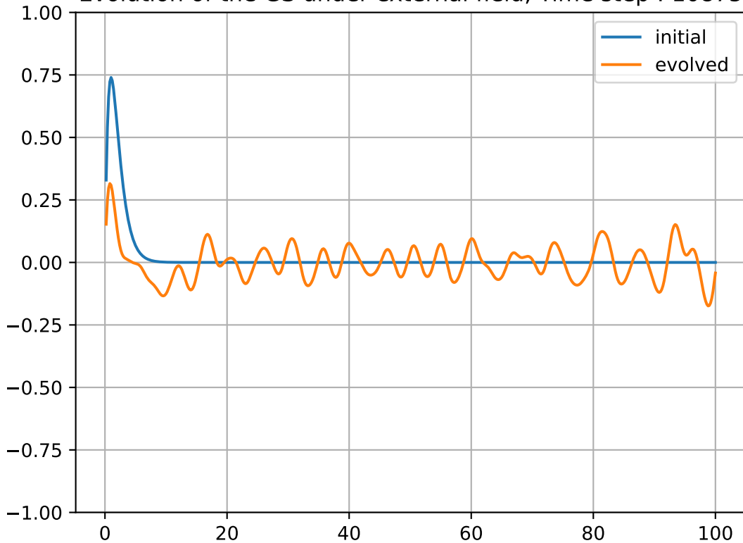
Evolution of the GS under external field, Time step : 10875
