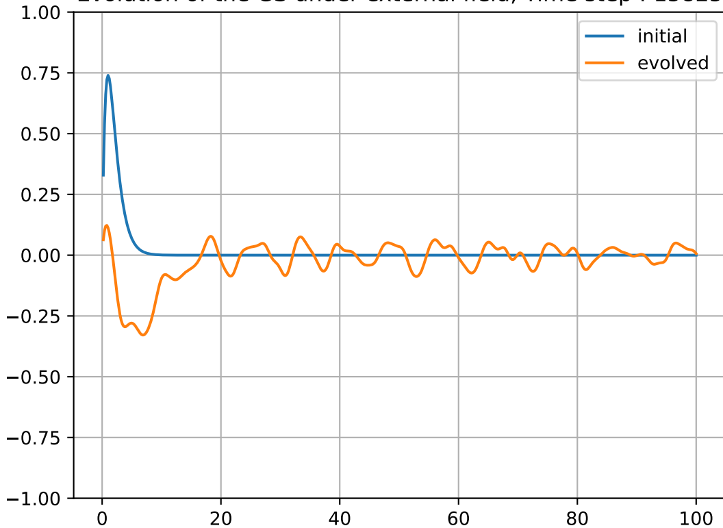
Evolution of the GS under external field, Time step : 15825
