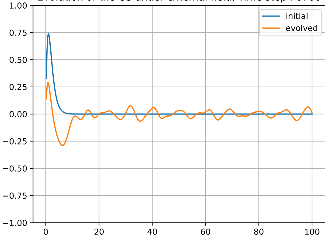
Evolution of the GS under external field, Time step : 6700
