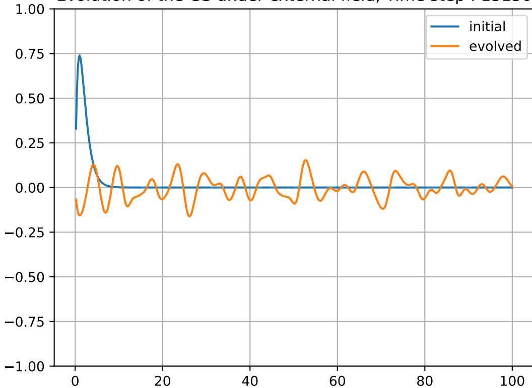
Evolution of the GS under external field, Time step : 13150
