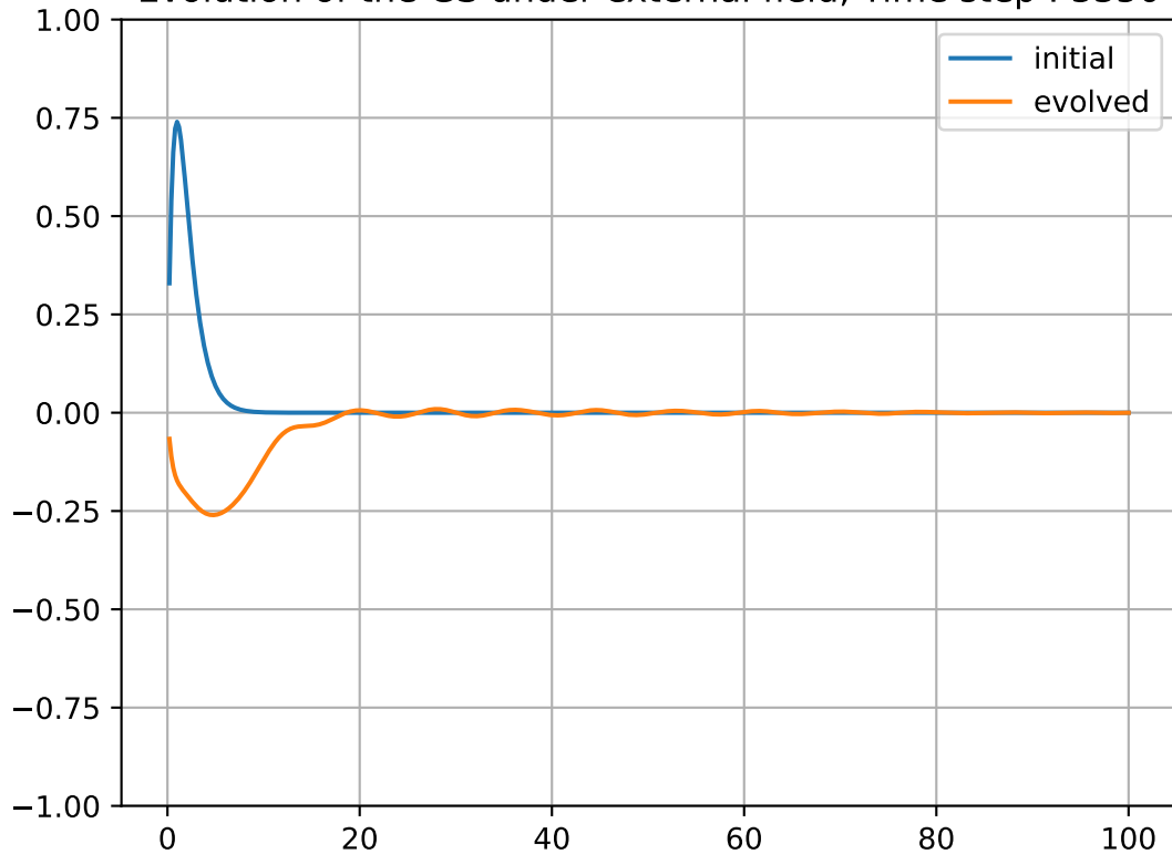
Evolution of the GS under external field, Time step : 3350
