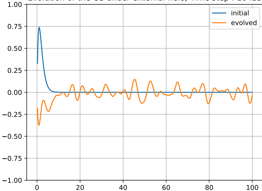
Evolution of the GS under external field, Time step : 10425
