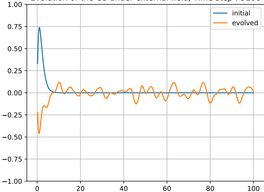
Evolution of the GS under external field, Time step : 9100
