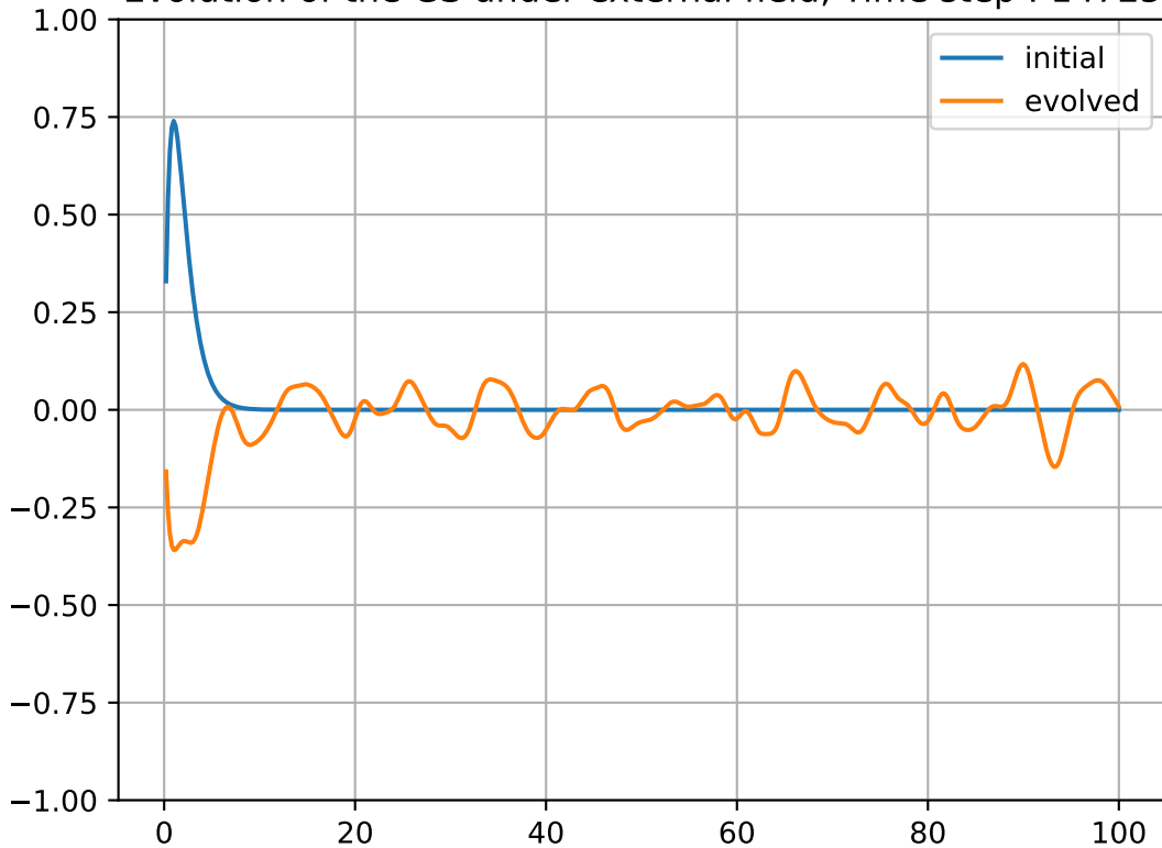
Evolution of the GS under external field, Time step : 14725
