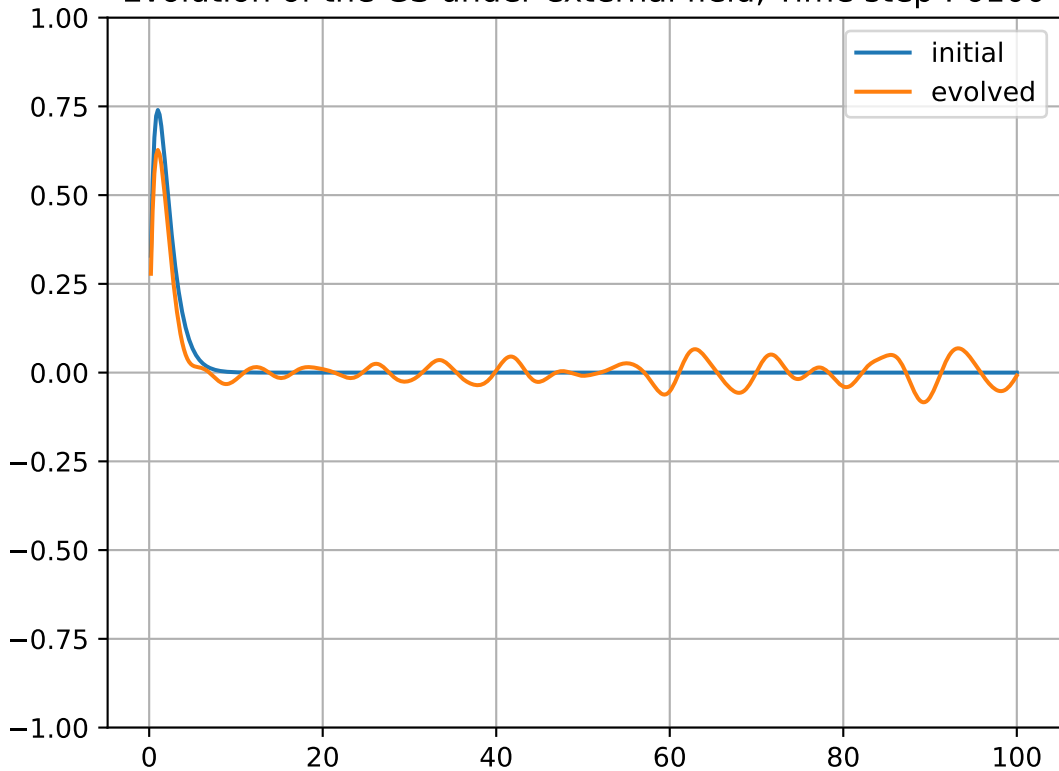
Evolution of the GS under external field, Time step : 6100
