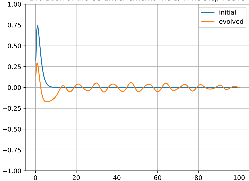
Evolution of the GS under external field, Time step : 5375
