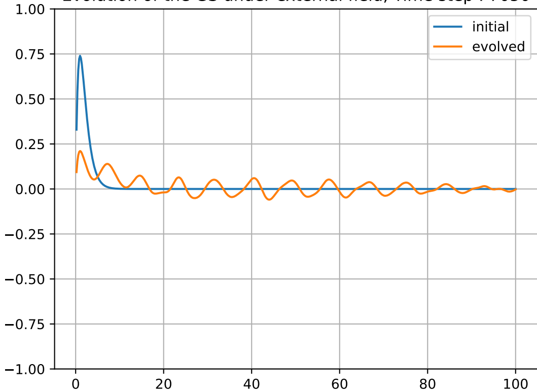
Evolution of the GS under external field, Time step : 7050
