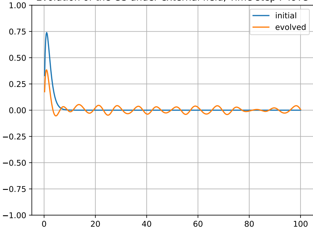
Evolution of the GS under external field, Time step : 4975
