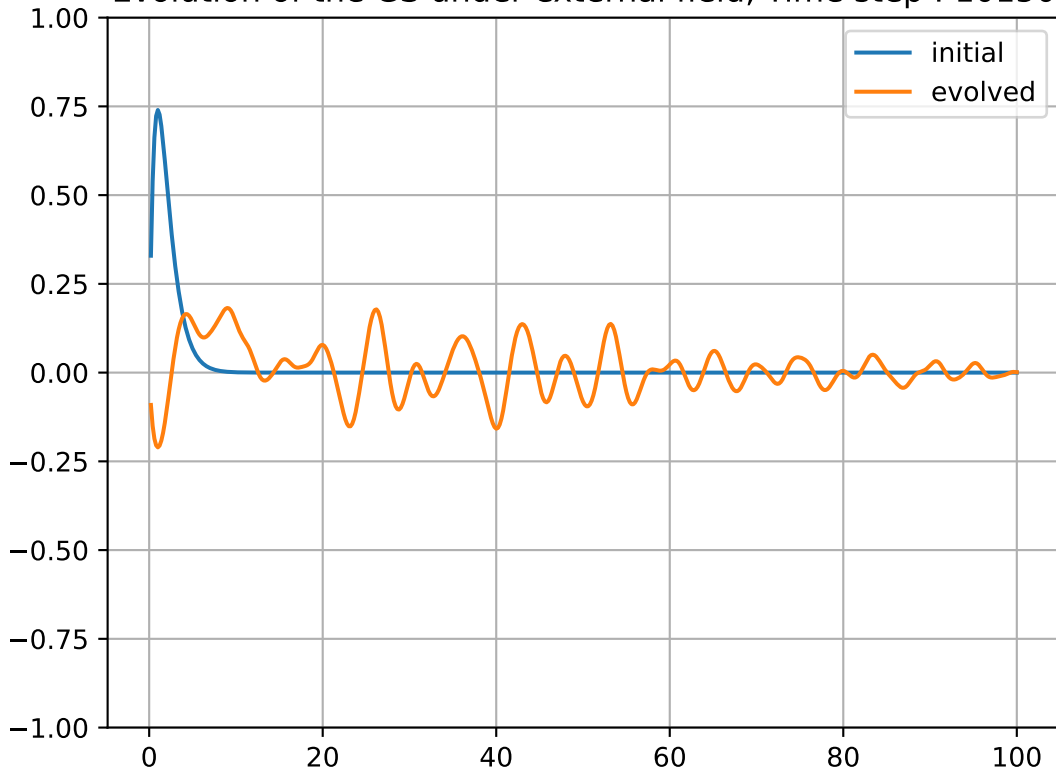
Evolution of the GS under external field, Time step : 10150
