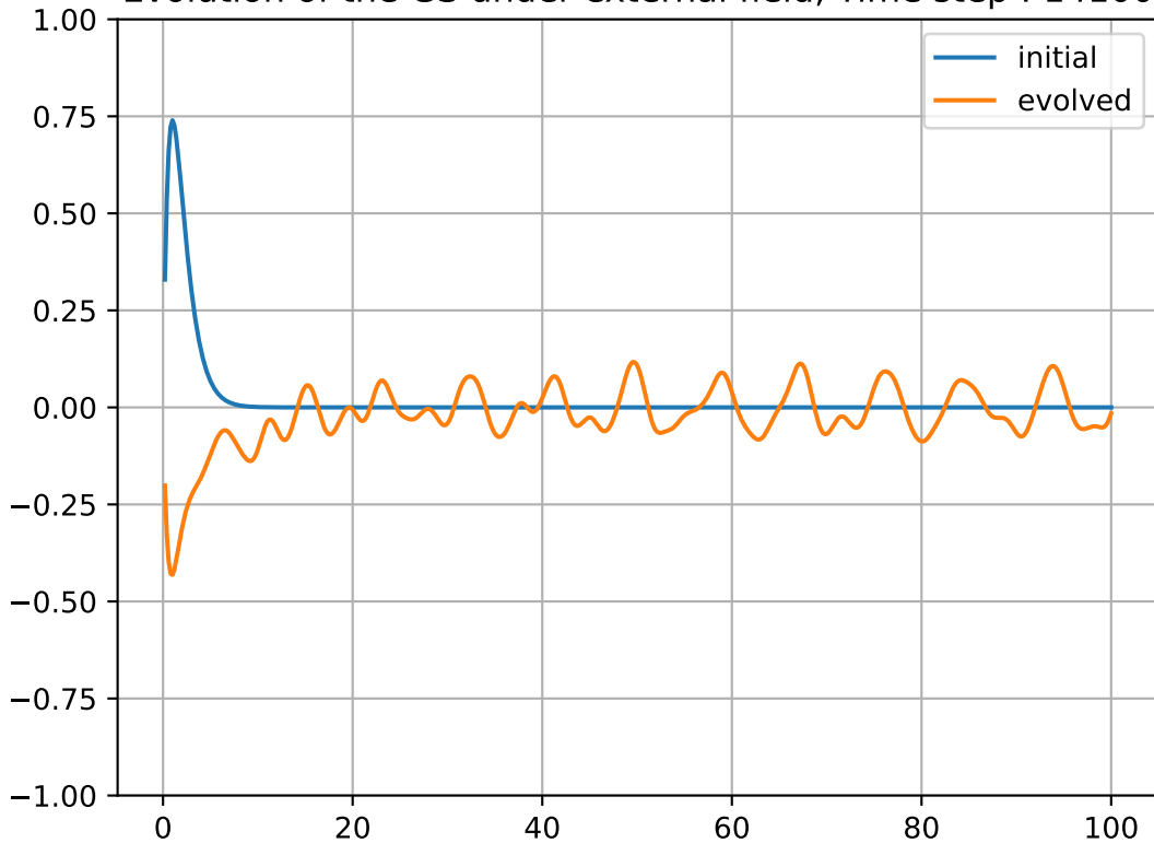
Evolution of the GS under external field, Time step : 14100
