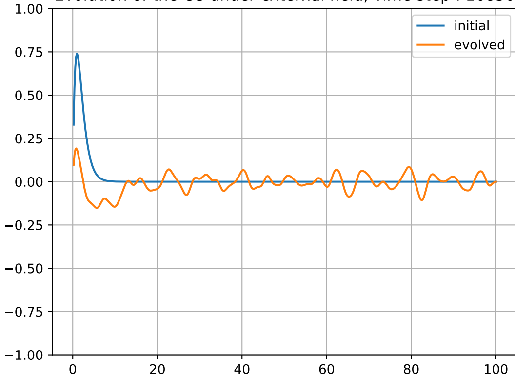
Evolution of the GS under external field, Time step : 16850
