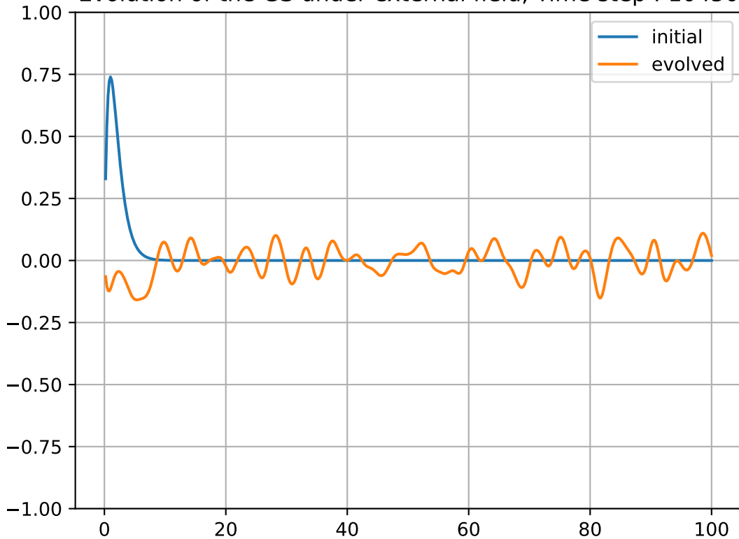
Evolution of the GS under external field, Time step : 10450
