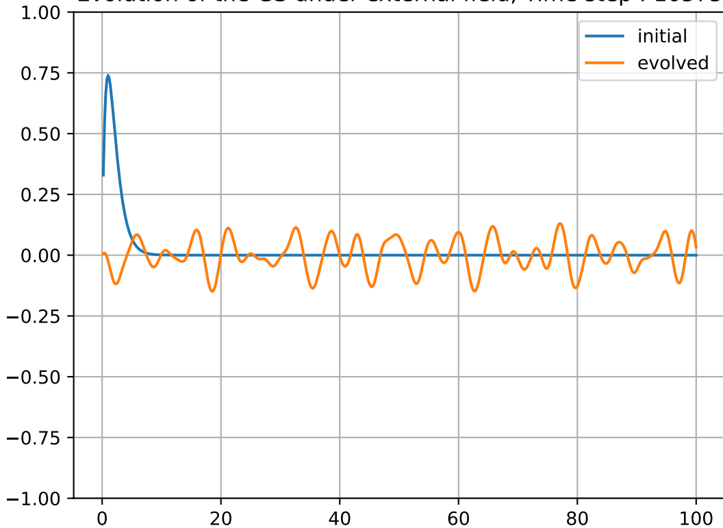
Evolution of the GS under external field, Time step : 10575
