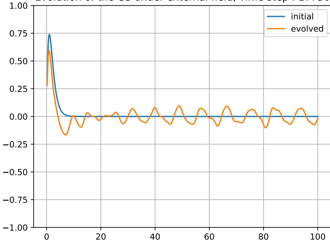
Evolution of the GS under external field, Time step : 17750
