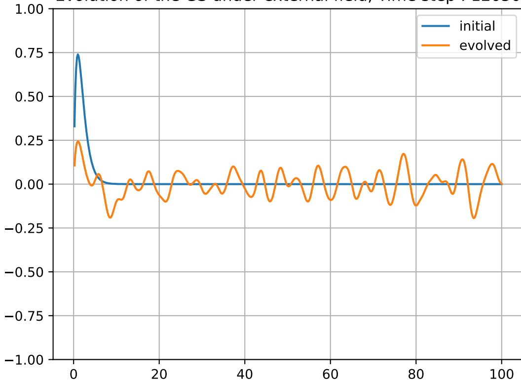
Evolution of the GS under external field, Time step : 12050
