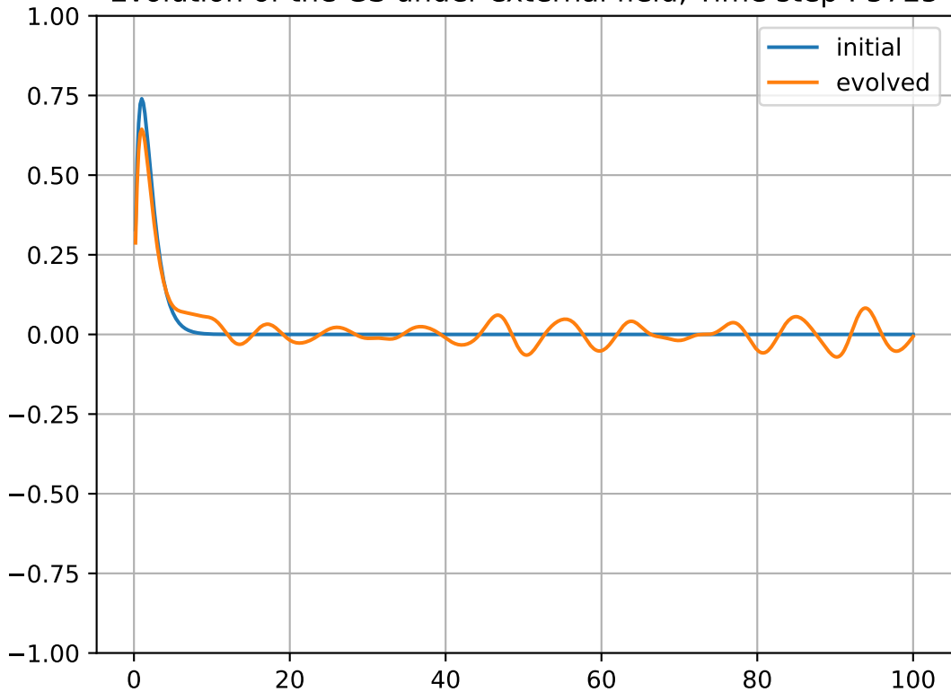
Evolution of the GS under external field, Time step : 5725
