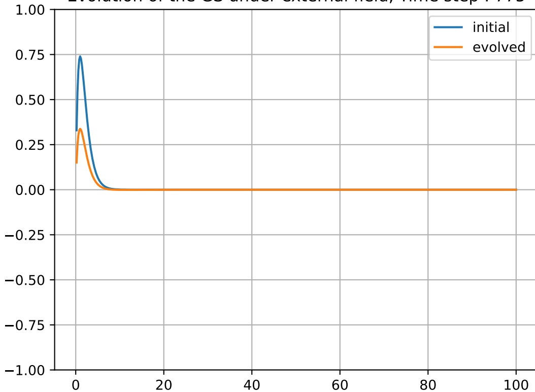
Evolution of the GS under external field, Time step : 775
