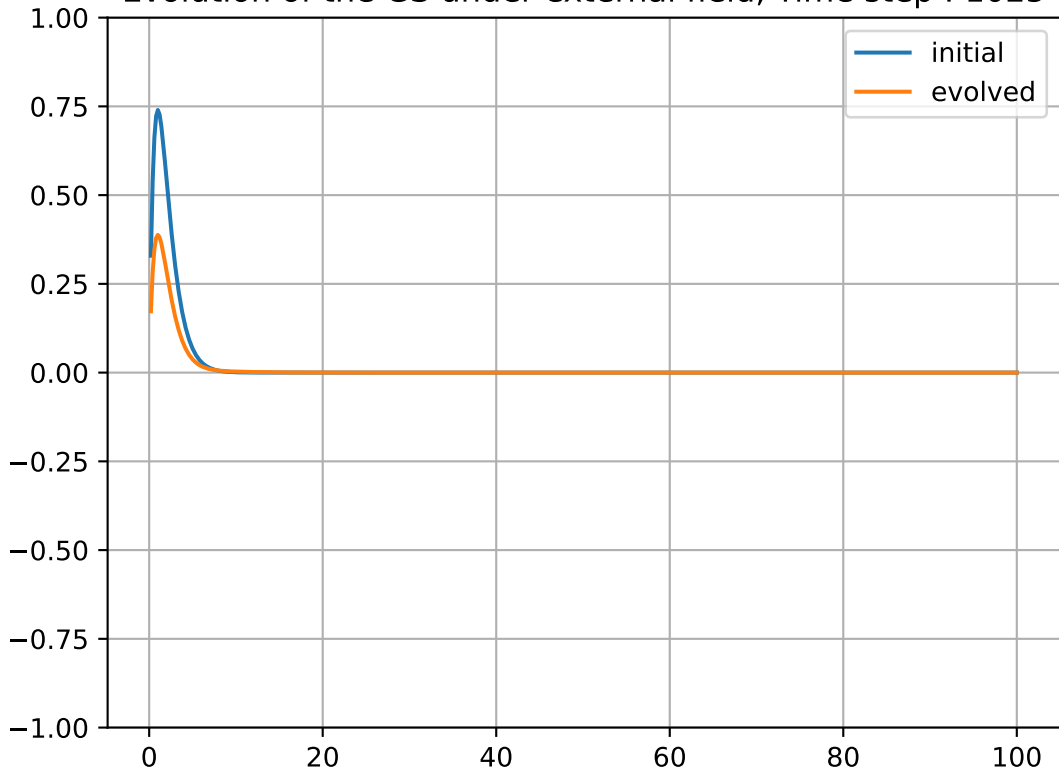
Evolution of the GS under external field, Time step : 1025
