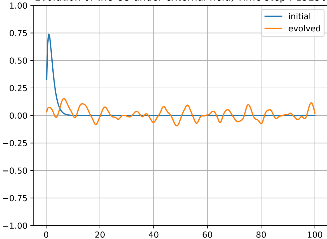
Evolution of the GS under external field, Time step : 15150
