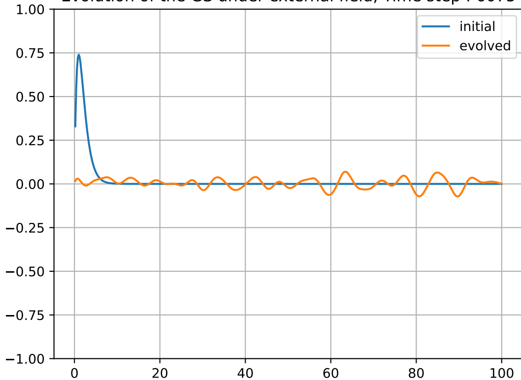
Evolution of the GS under external field, Time step : 6075
