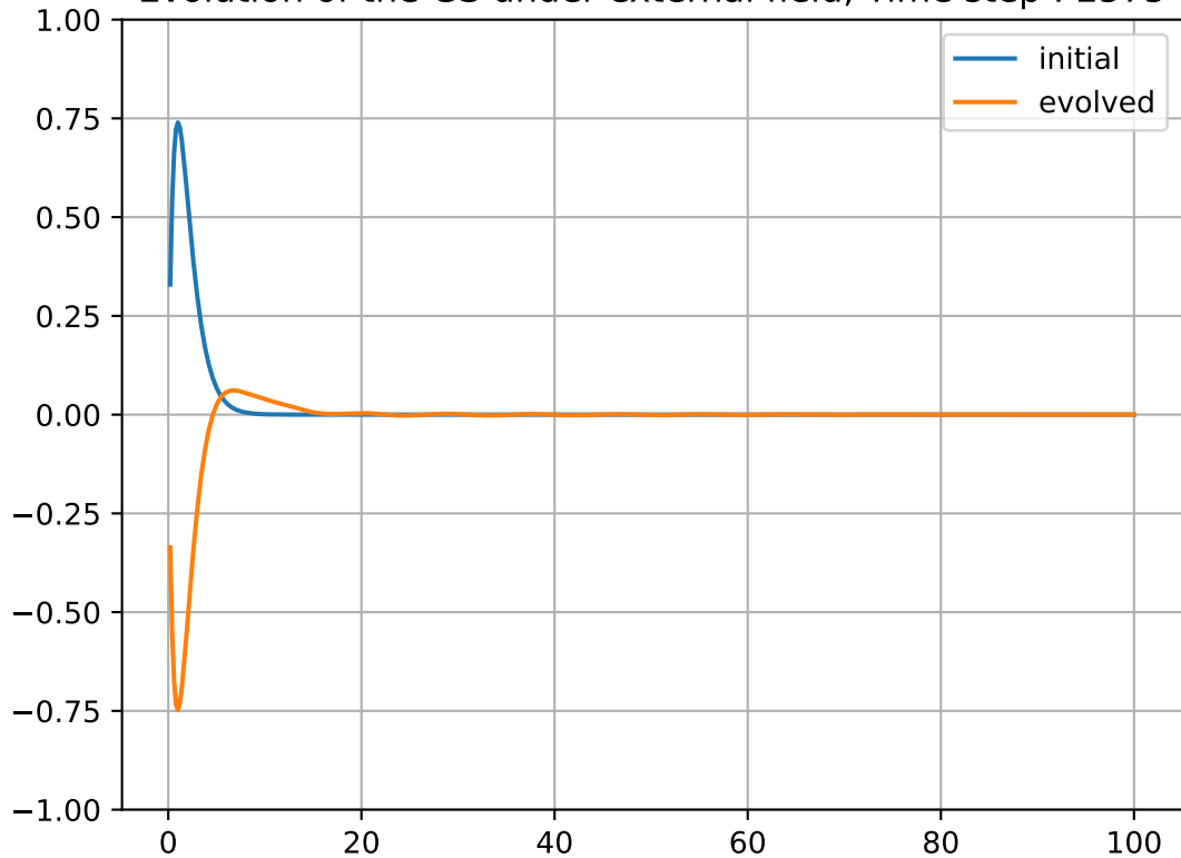
Evolution of the GS under external field, Time step : 2575
