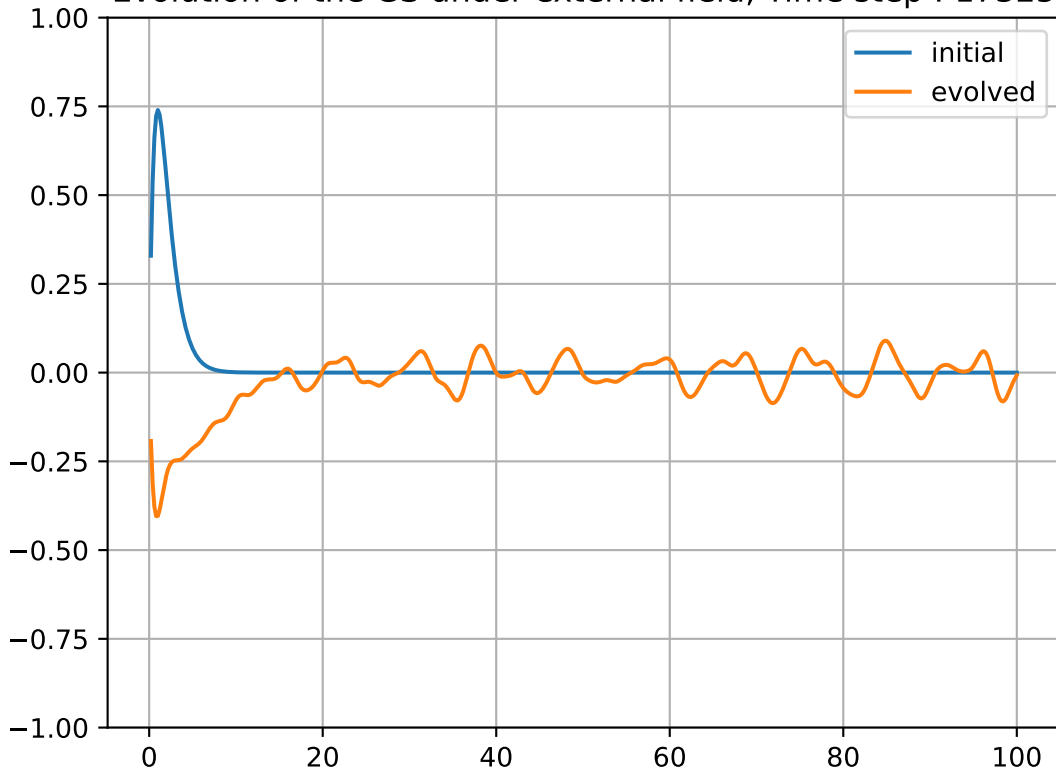
Evolution of the GS under external field, Time step : 17325
