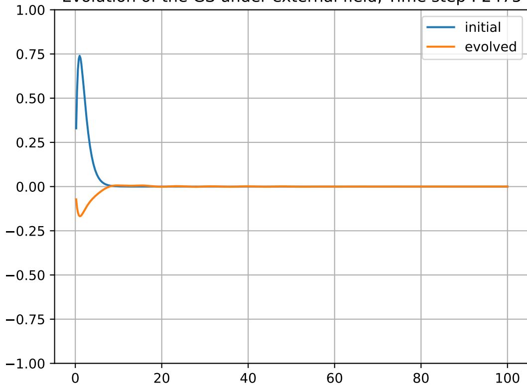
Evolution of the GS under external field, Time step : 2475
