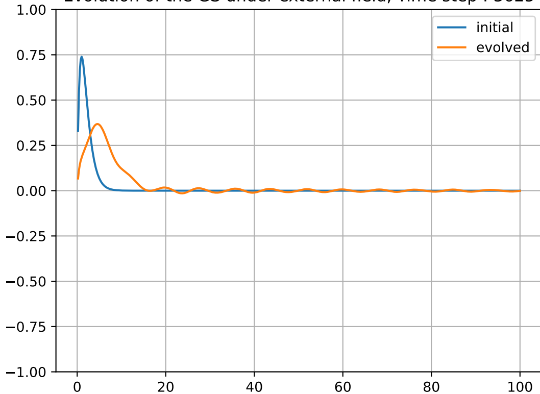
Evolution of the GS under external field, Time step : 3625
