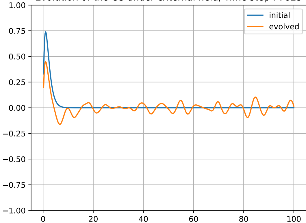
Evolution of the GS under external field, Time step : 7825
