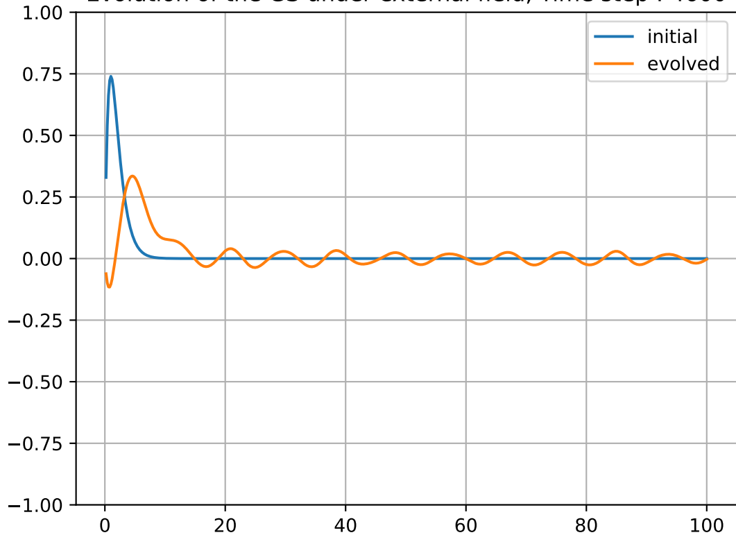
Evolution of the GS under external field, Time step : 4600
