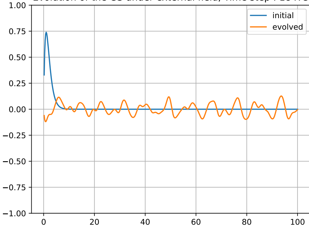
Evolution of the GS under external field, Time step : 18475
