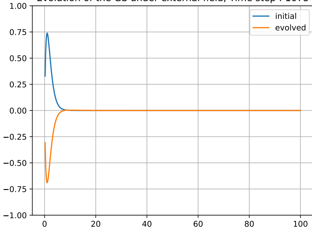
Evolution of the GS under external field, Time step : 1075
