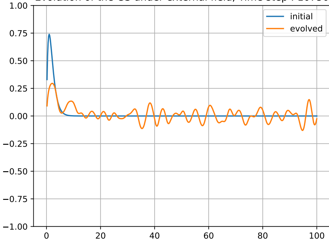
Evolution of the GS under external field, Time step : 10750
