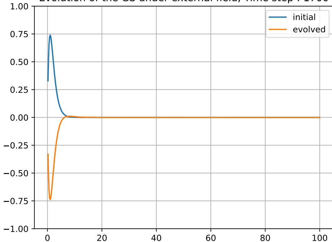
Evolution of the GS under external field, Time step : 1700
