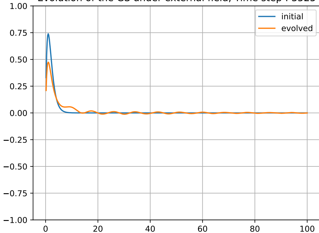
Evolution of the GS under external field, Time step : 3525
