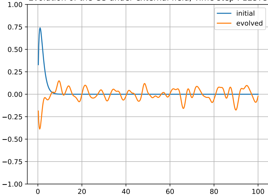
Evolution of the GS under external field, Time step : 12375
