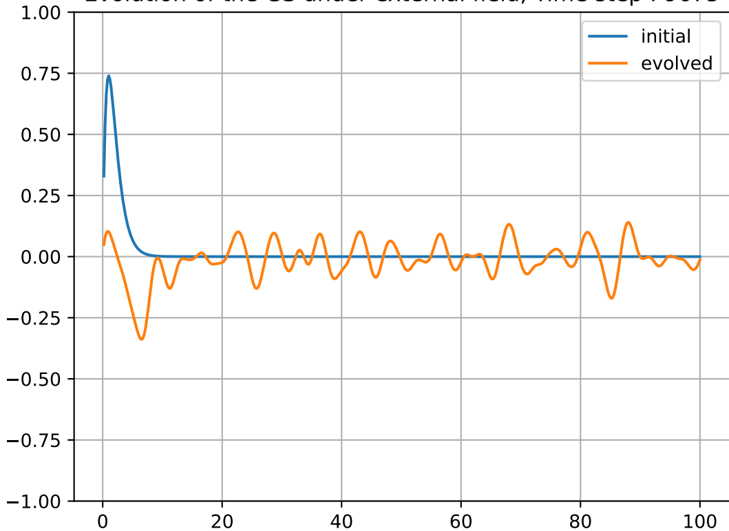
Evolution of the GS under external field, Time step : 9675
