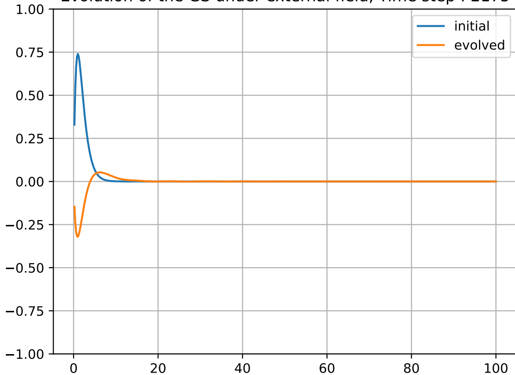
Evolution of the GS under external field, Time step : 2175
