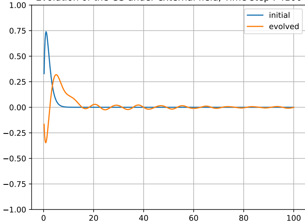
Evolution of the GS under external field, Time step : 4100
