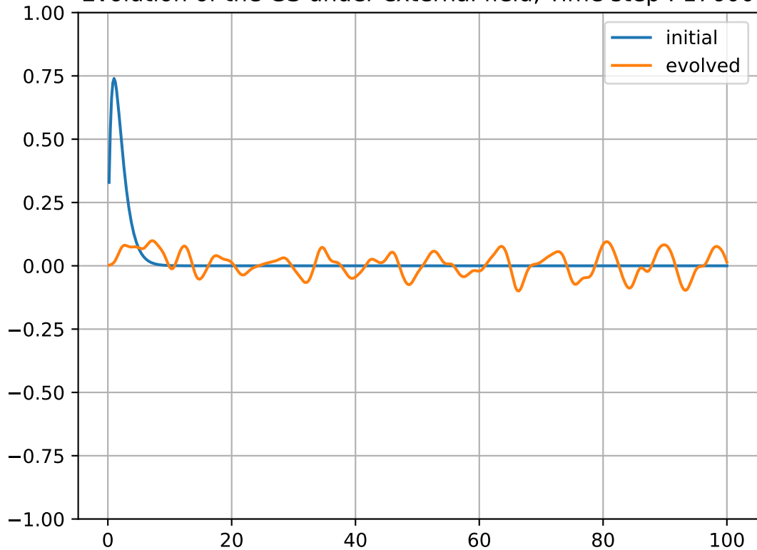
Evolution of the GS under external field, Time step : 17600
