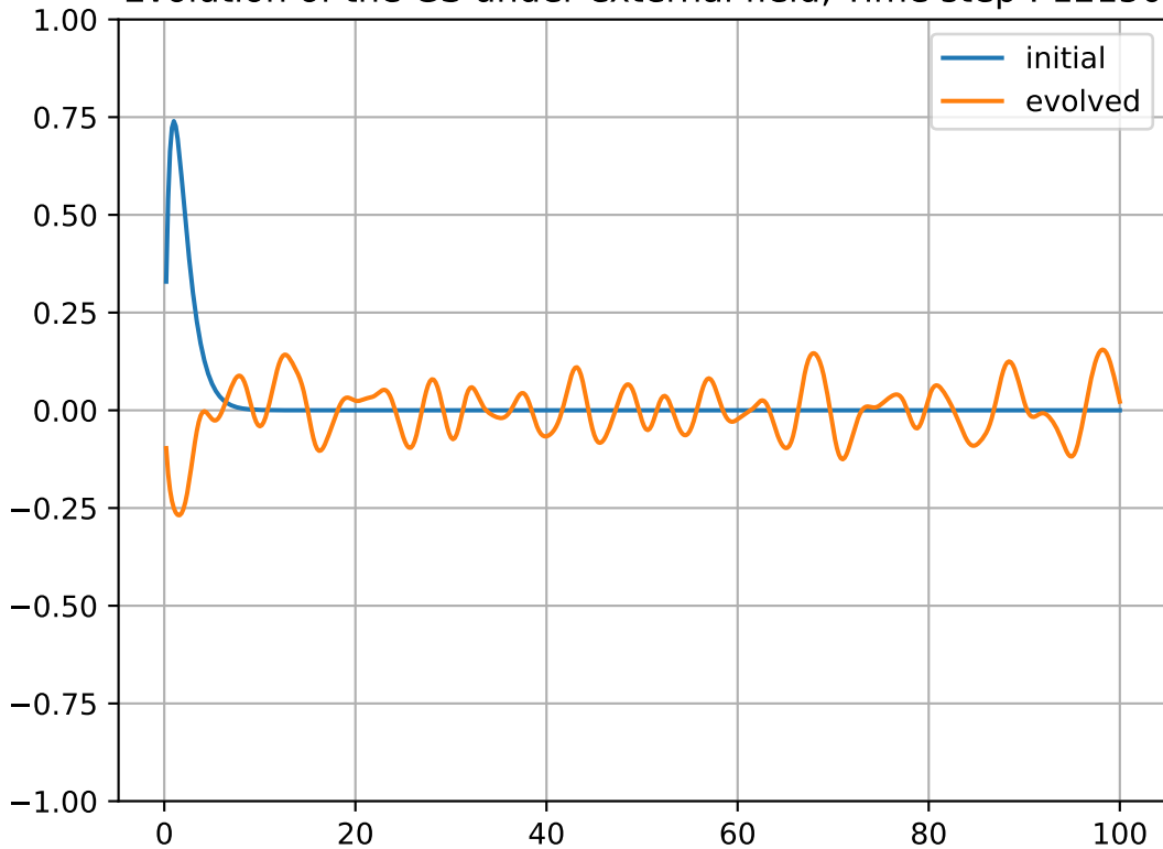
Evolution of the GS under external field, Time step : 12150
