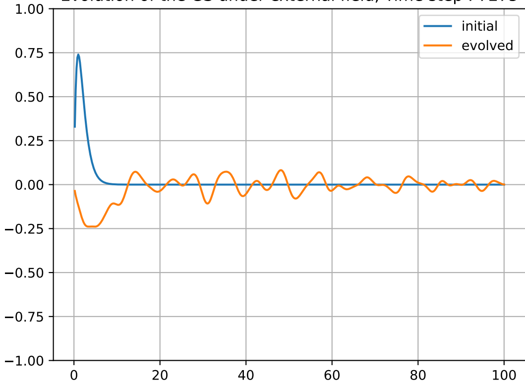
Evolution of the GS under external field, Time step : 7275
