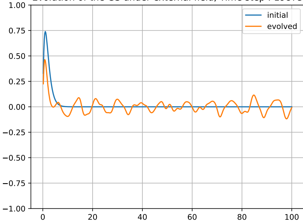
Evolution of the GS under external field, Time step : 19875
