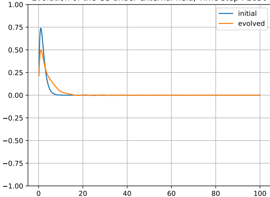
Evolution of the GS under external field, Time step : 2650
