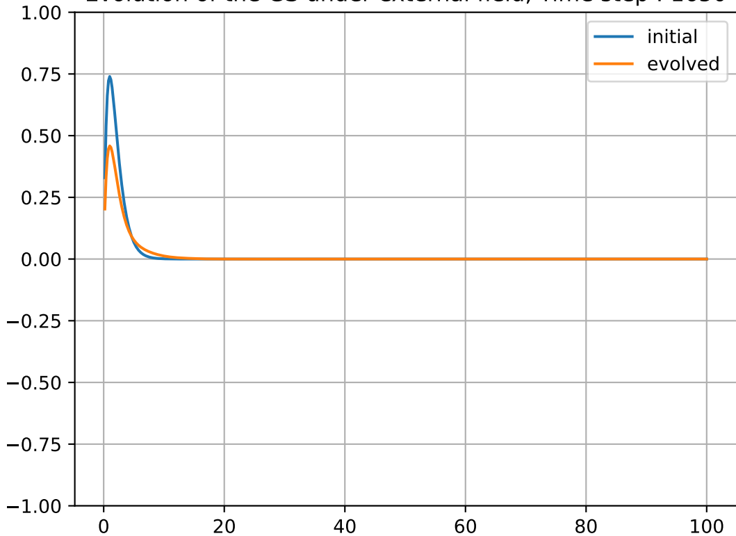
Evolution of the GS under external field, Time step : 1650
