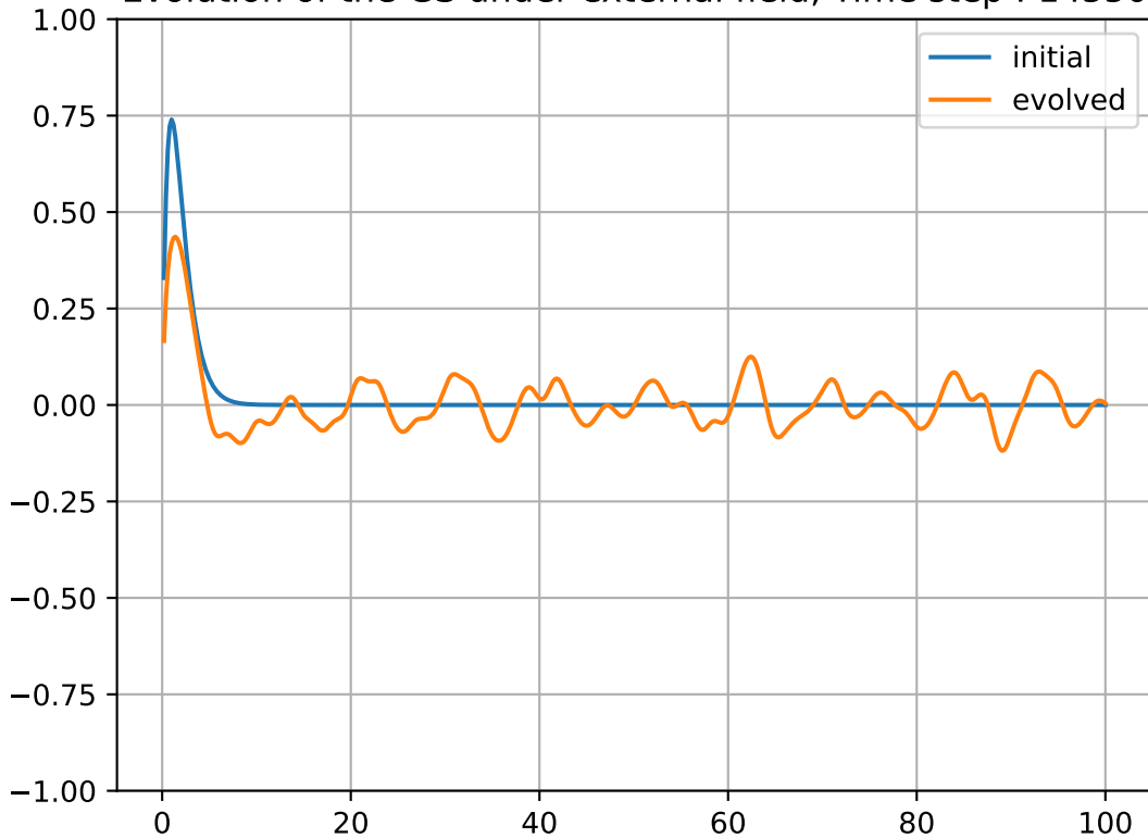
Evolution of the GS under external field, Time step : 14550
