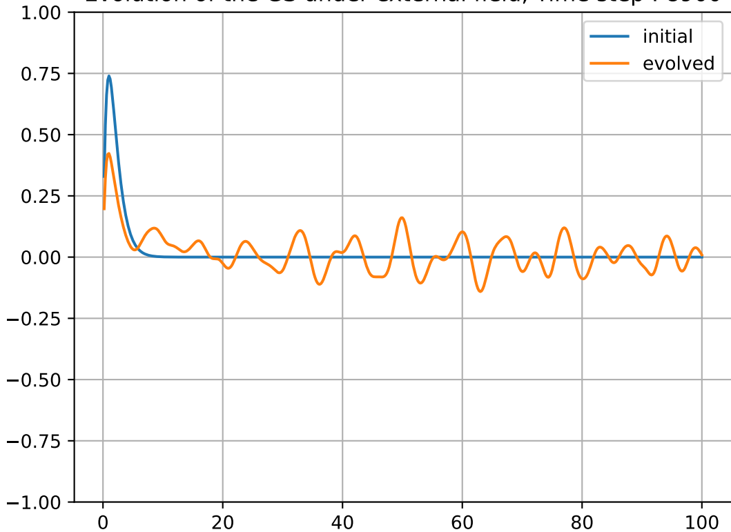
Evolution of the GS under external field, Time step : 8900
