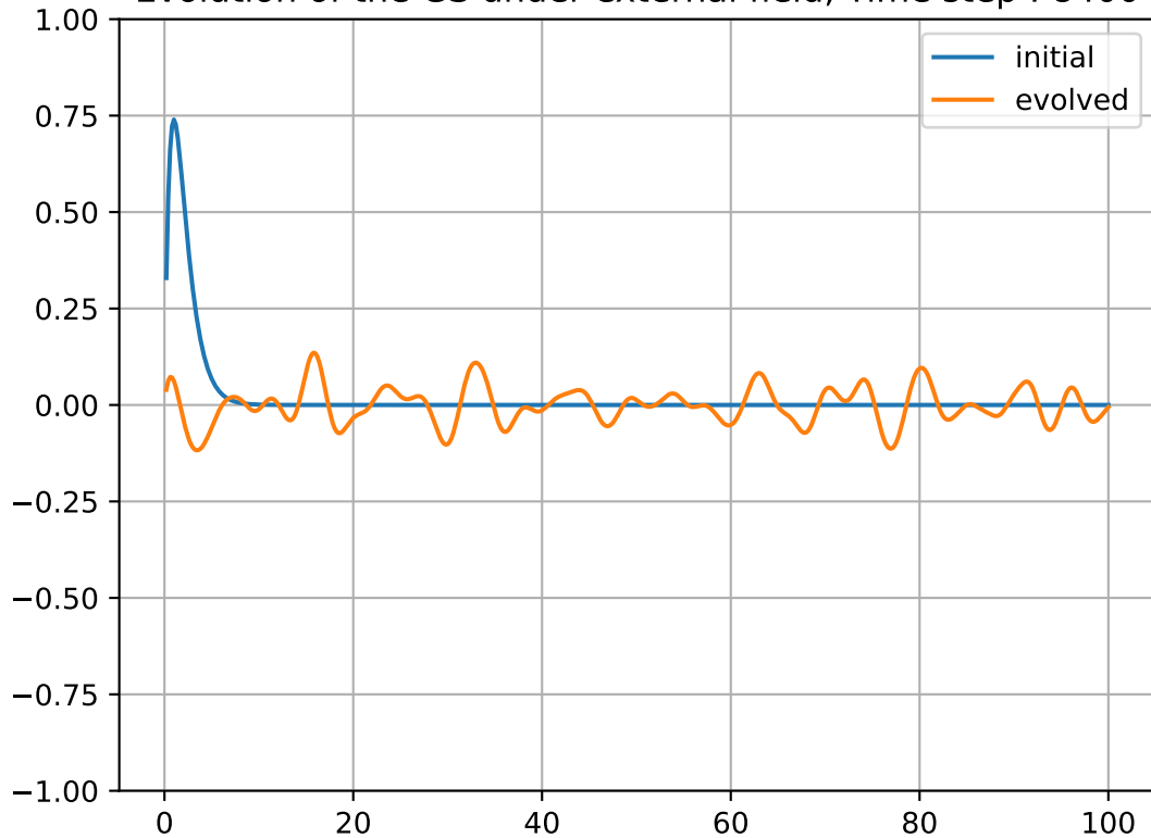
Evolution of the GS under external field, Time step : 8400
