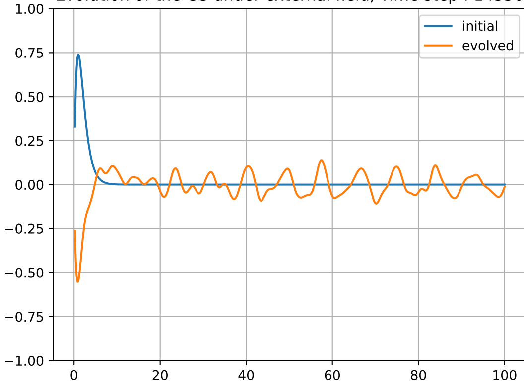
Evolution of the GS under external field, Time step : 14350
