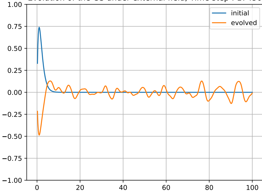
Evolution of the GS under external field, Time step : 17450
