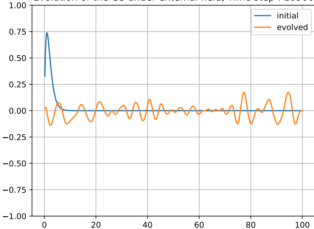
Evolution of the GS under external field, Time step : 10900
