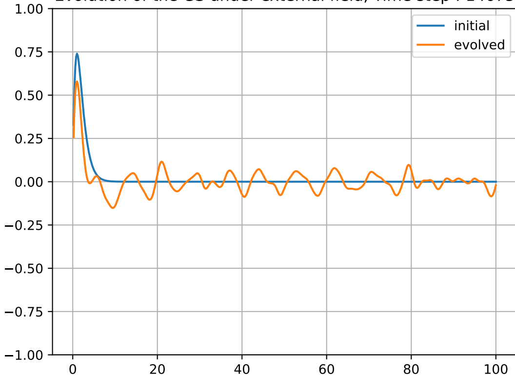
Evolution of the GS under external field, Time step : 14675
