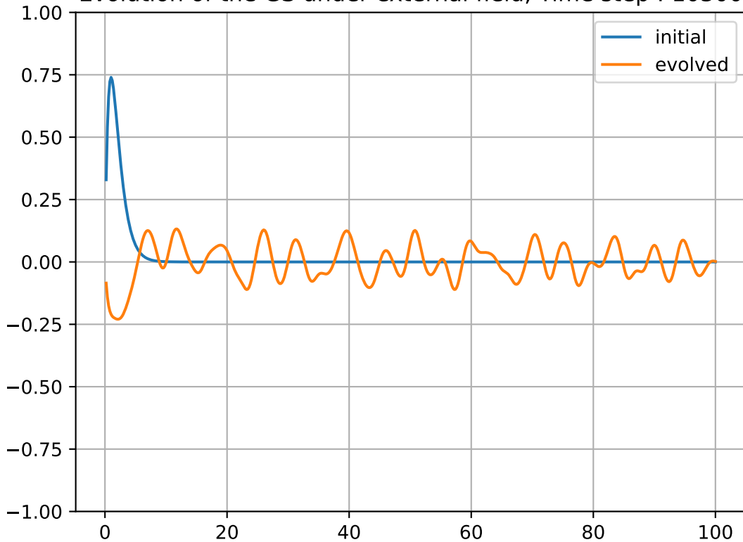
Evolution of the GS under external field, Time step : 10300
