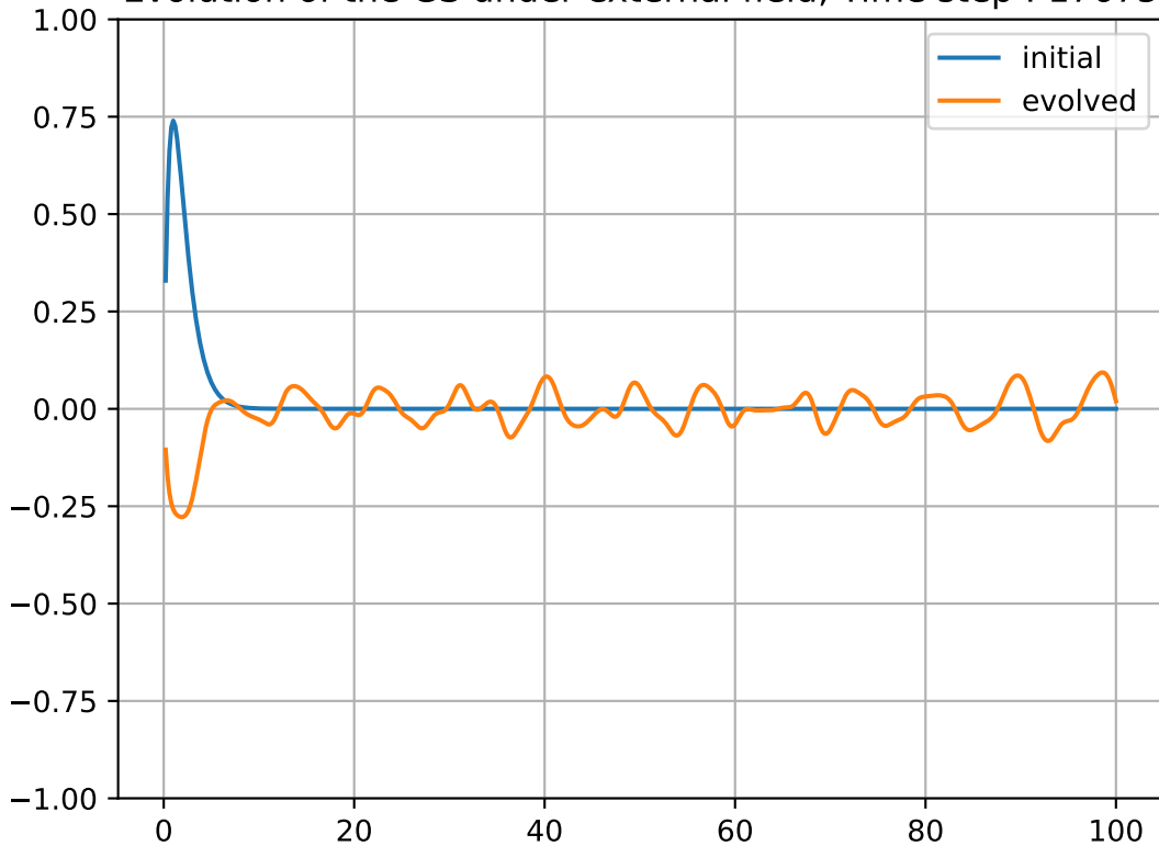
Evolution of the GS under external field, Time step : 17675
