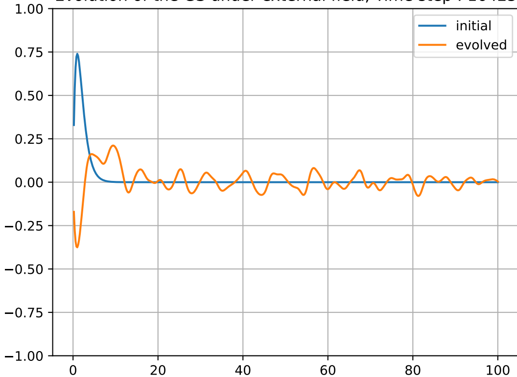
Evolution of the GS under external field, Time step : 16425
