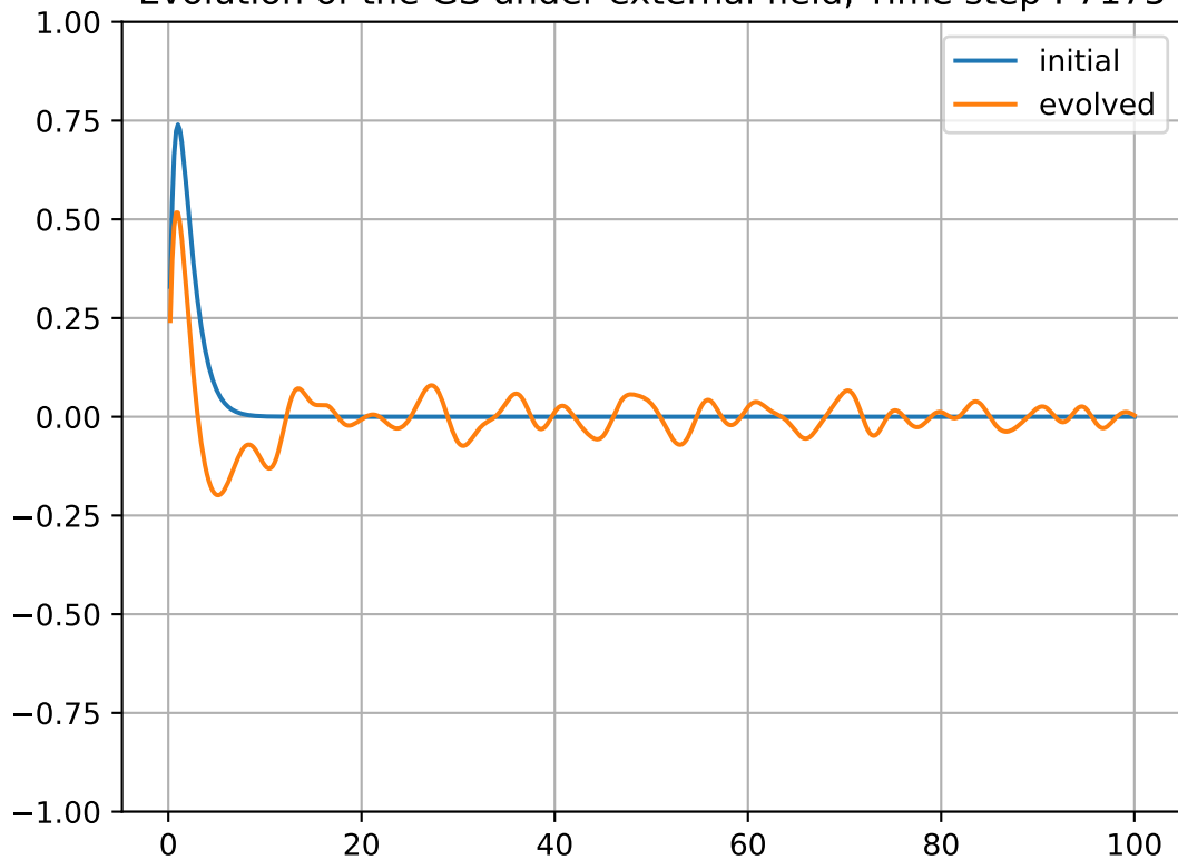
Evolution of the GS under external field, Time step : 7175
