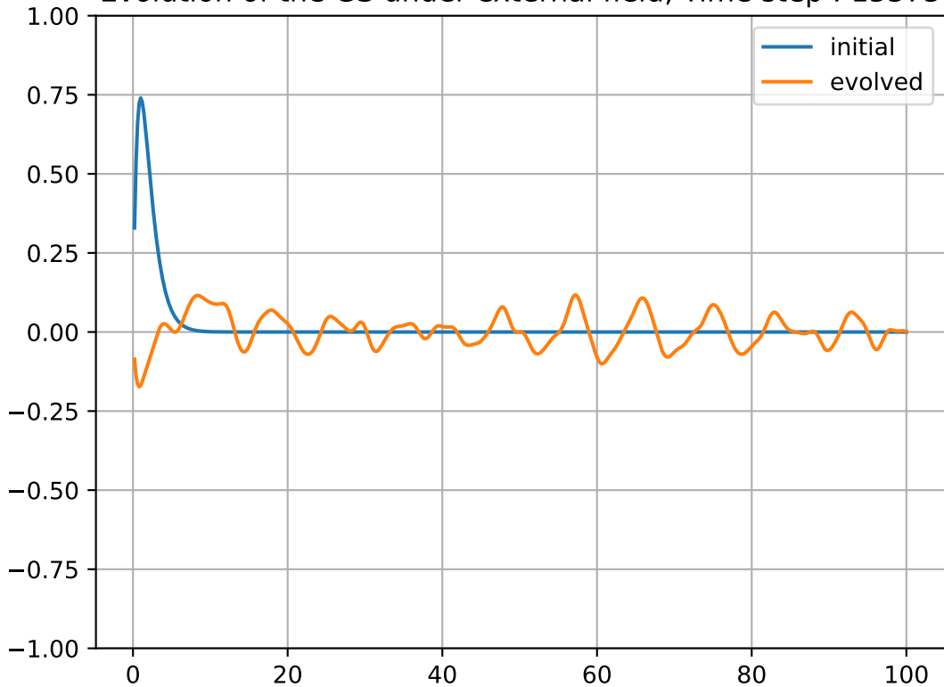
Evolution of the GS under external field, Time step : 15375
