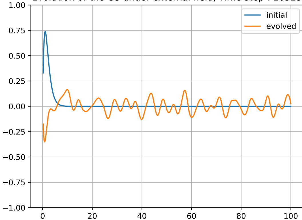
Evolution of the GS under external field, Time step : 10525
