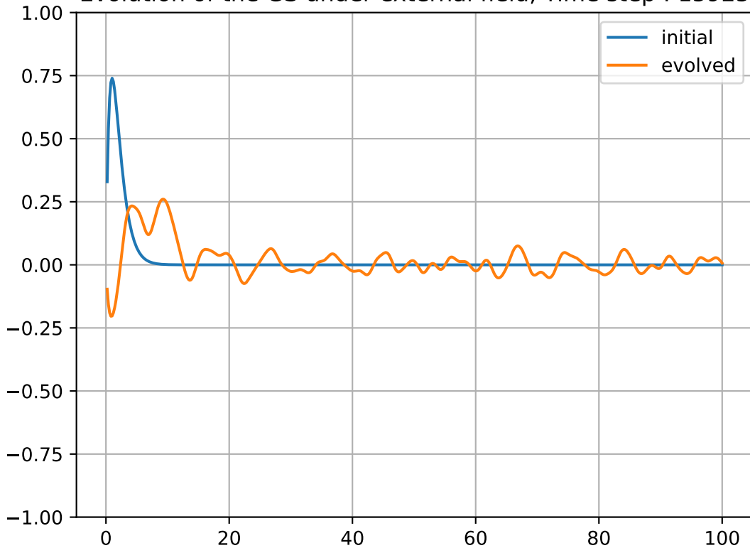
Evolution of the GS under external field, Time step : 15925
