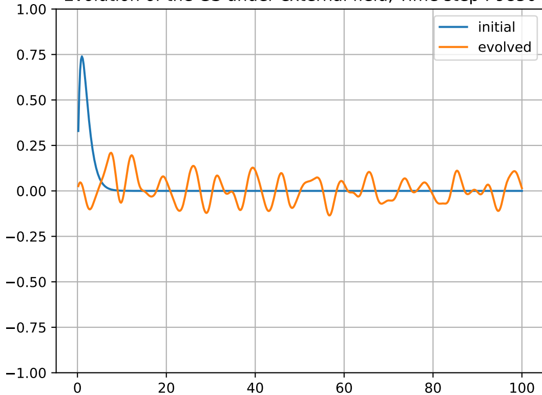
Evolution of the GS under external field, Time step : 9850
