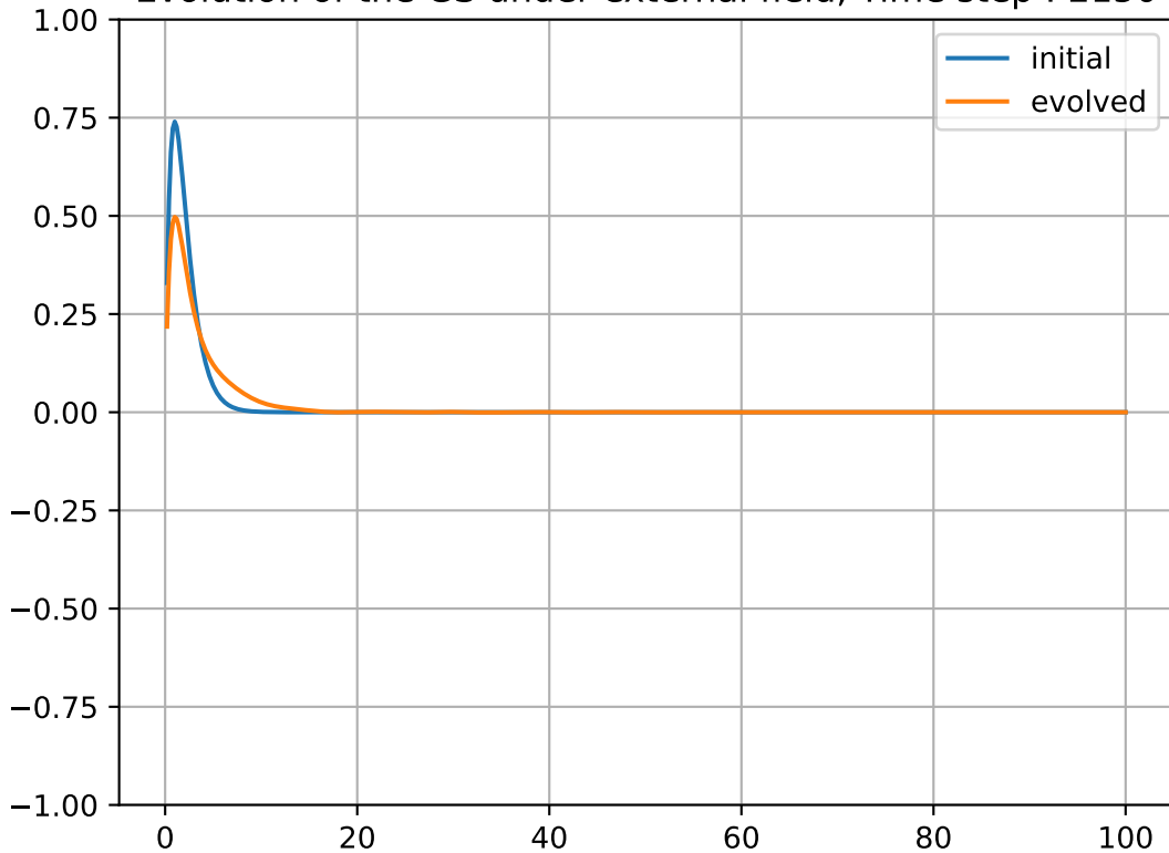
Evolution of the GS under external field, Time step : 2150
