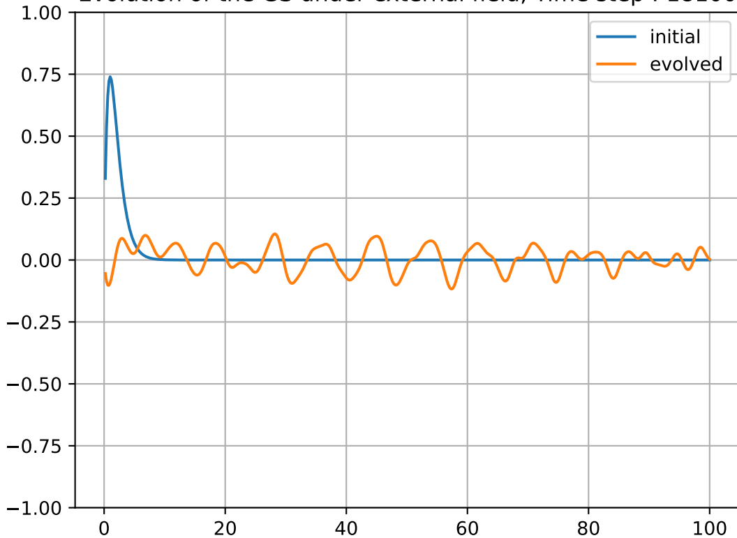
Evolution of the GS under external field, Time step : 18100
