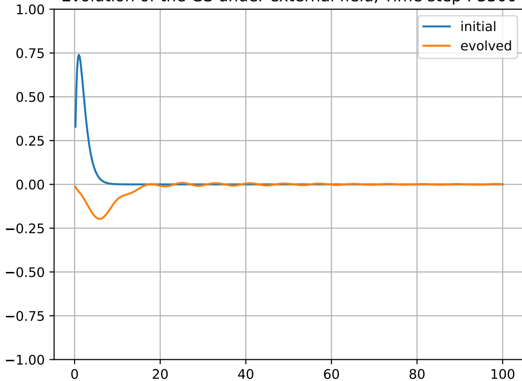
Evolution of the GS under external field, Time step : 3300
