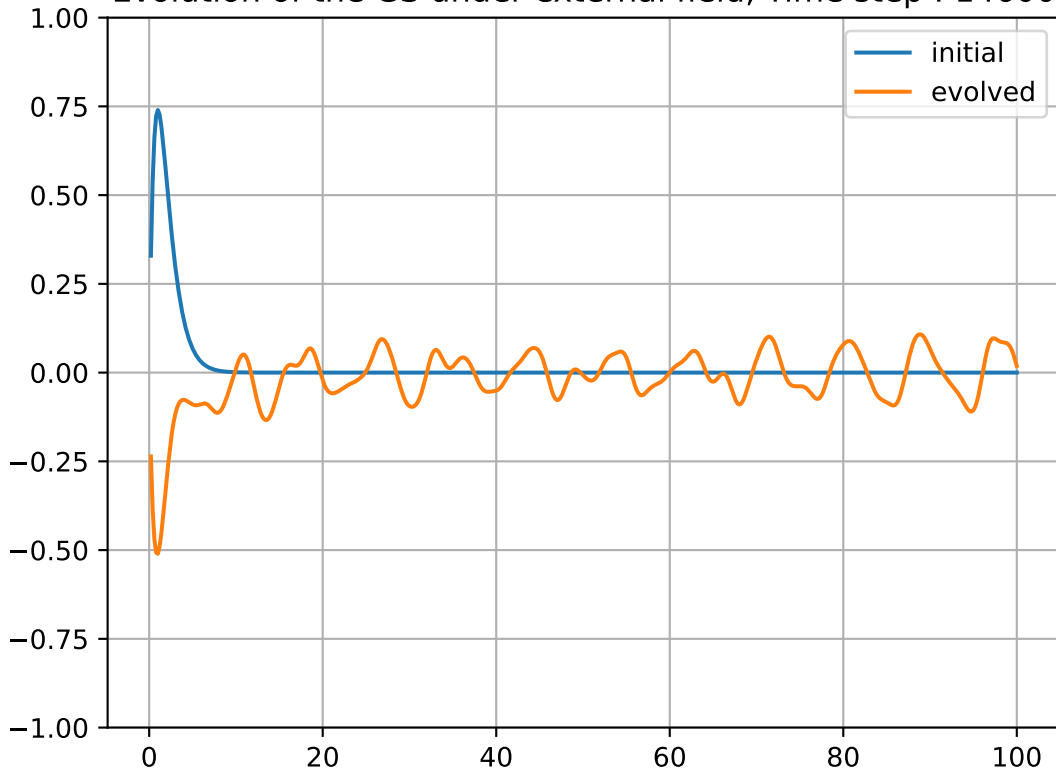
Evolution of the GS under external field, Time step : 14600
