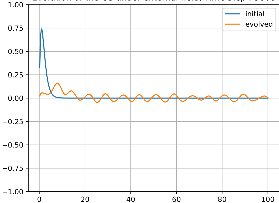
Evolution of the GS under external field, Time step : 5000
