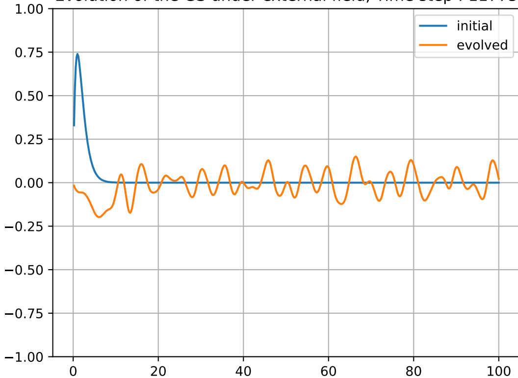
Evolution of the GS under external field, Time step : 11775
