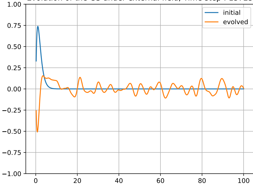
Evolution of the GS under external field, Time step : 13725
