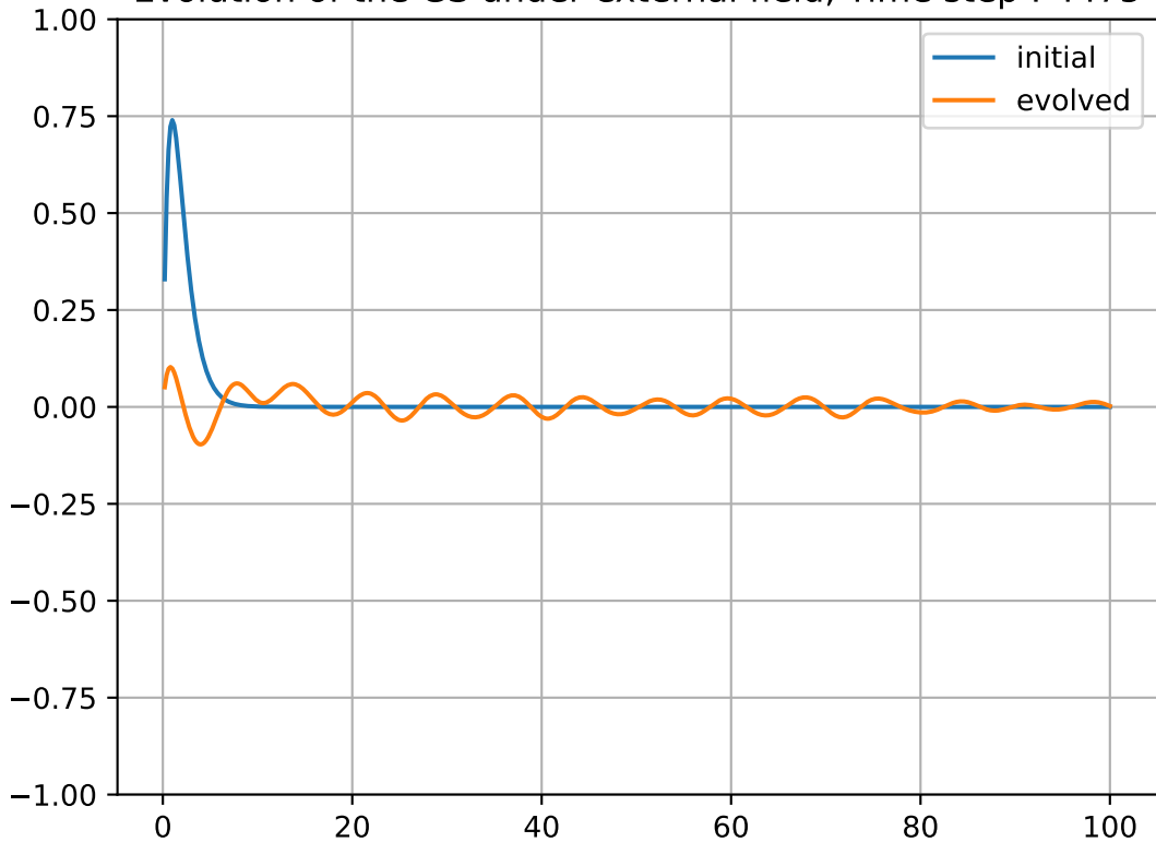
Evolution of the GS under external field, Time step : 4475
