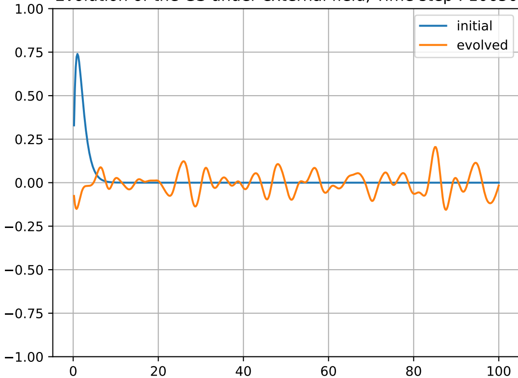
Evolution of the GS under external field, Time step : 10650
