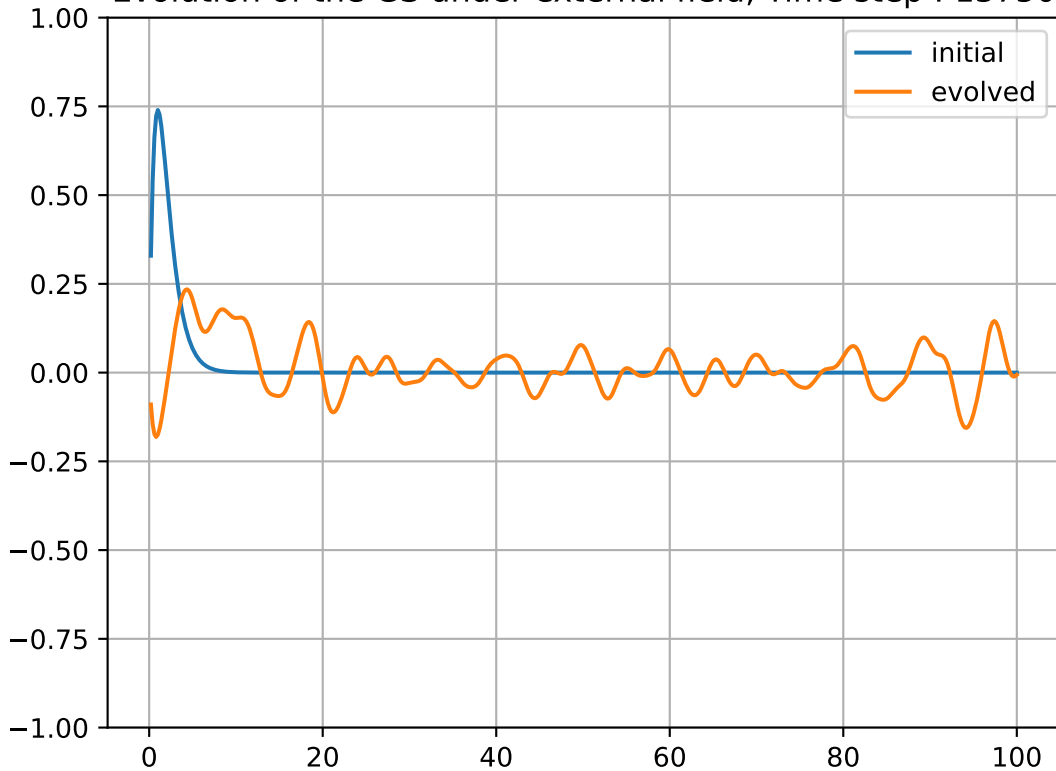
Evolution of the GS under external field, Time step : 13750
