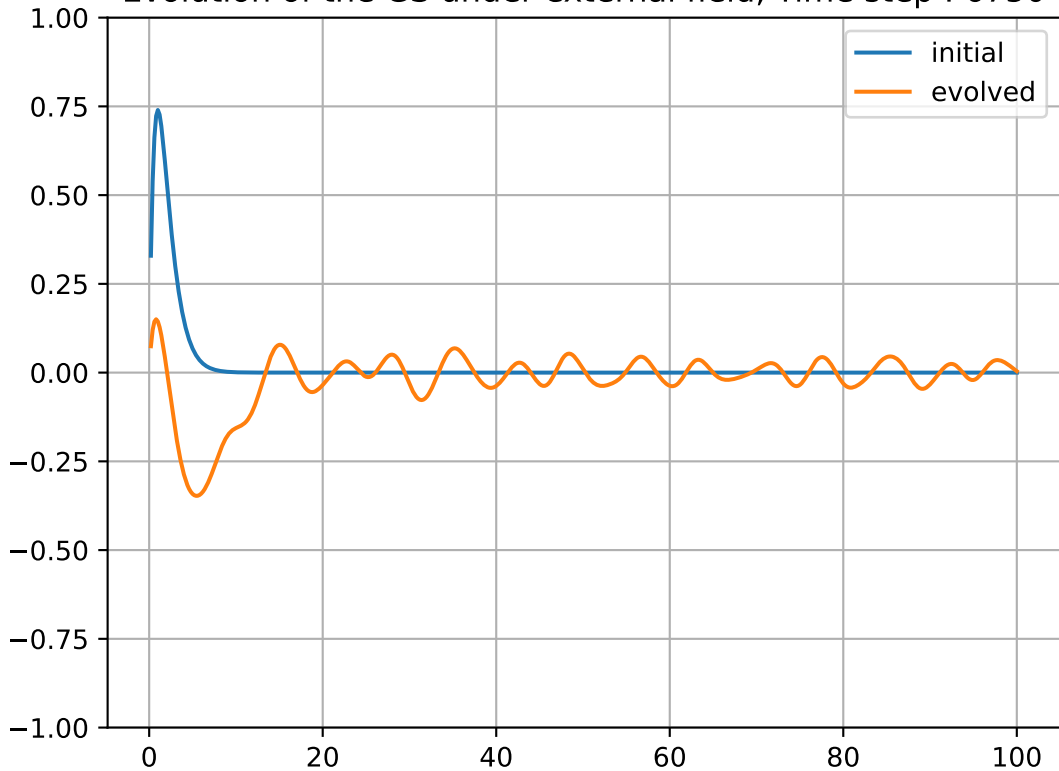
Evolution of the GS under external field, Time step : 6750
