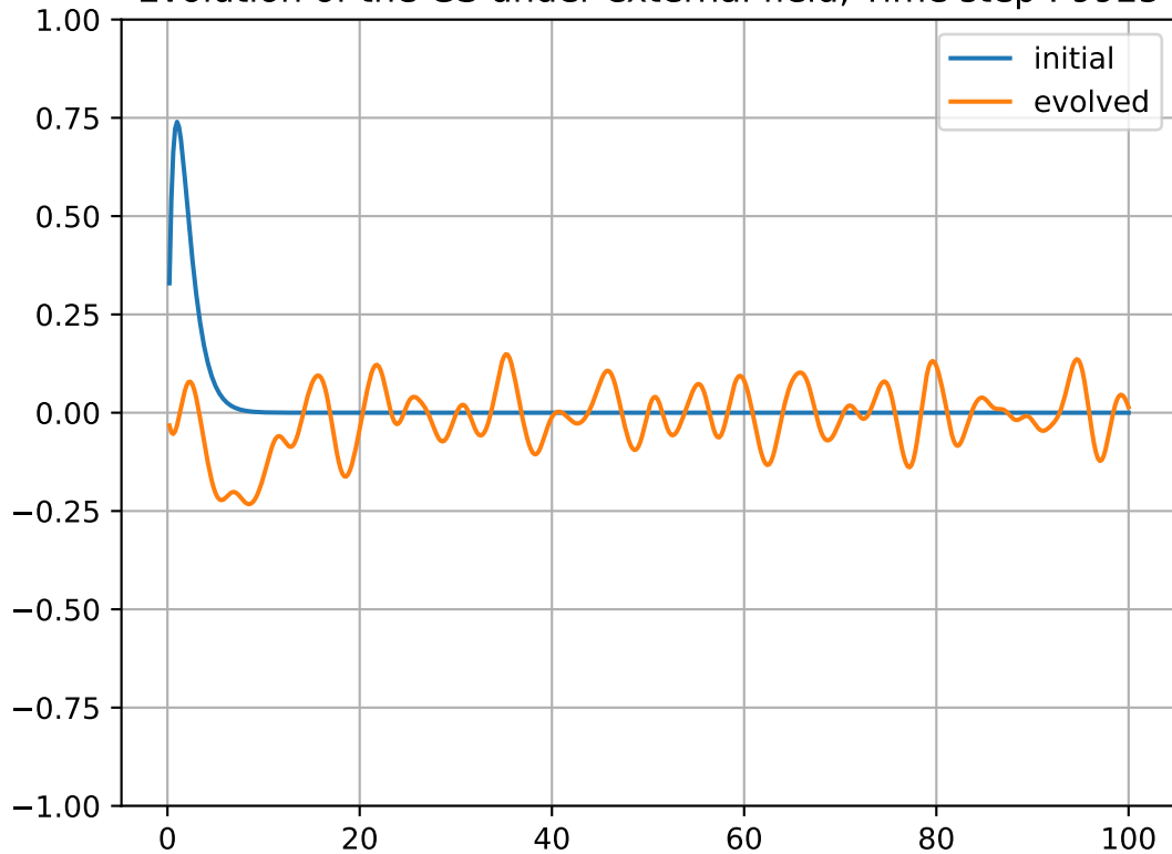
Evolution of the GS under external field, Time step : 9925
