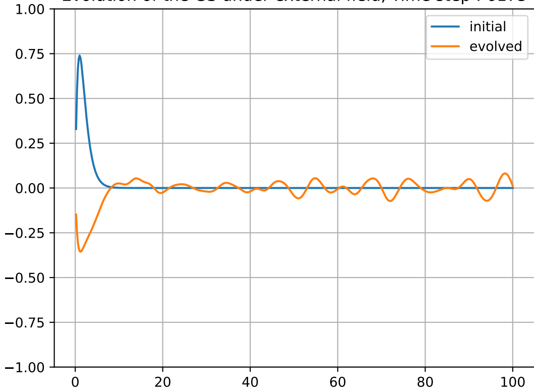
Evolution of the GS under external field, Time step : 6175
