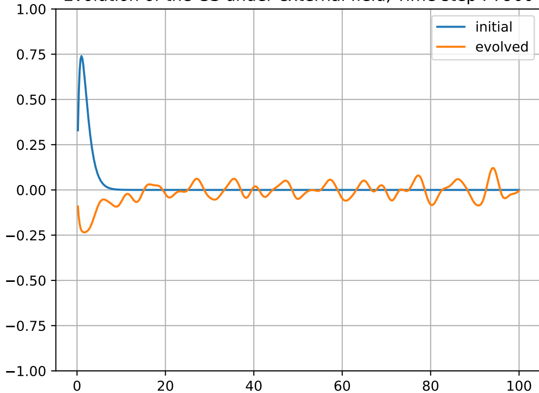
Evolution of the GS under external field, Time step : 7900
