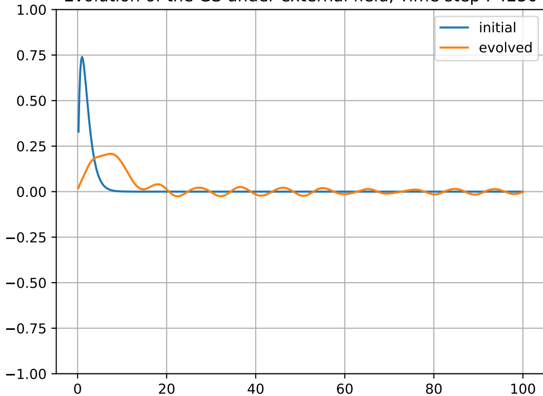
Evolution of the GS under external field, Time step : 4250
