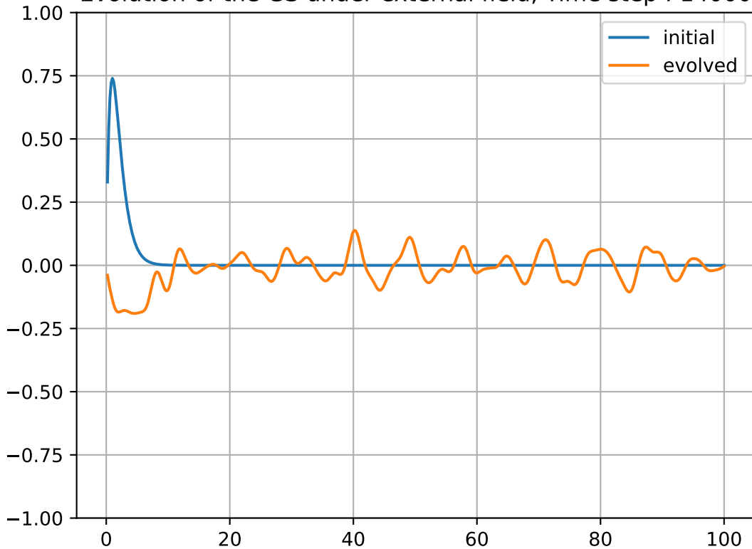
Evolution of the GS under external field, Time step : 14000
