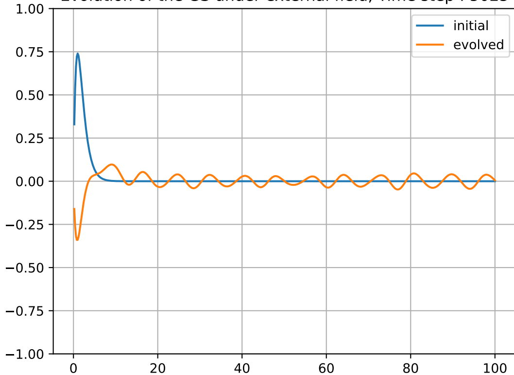
Evolution of the GS under external field, Time step : 5025
