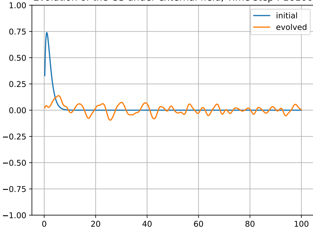
Evolution of the GS under external field, Time step : 16100
