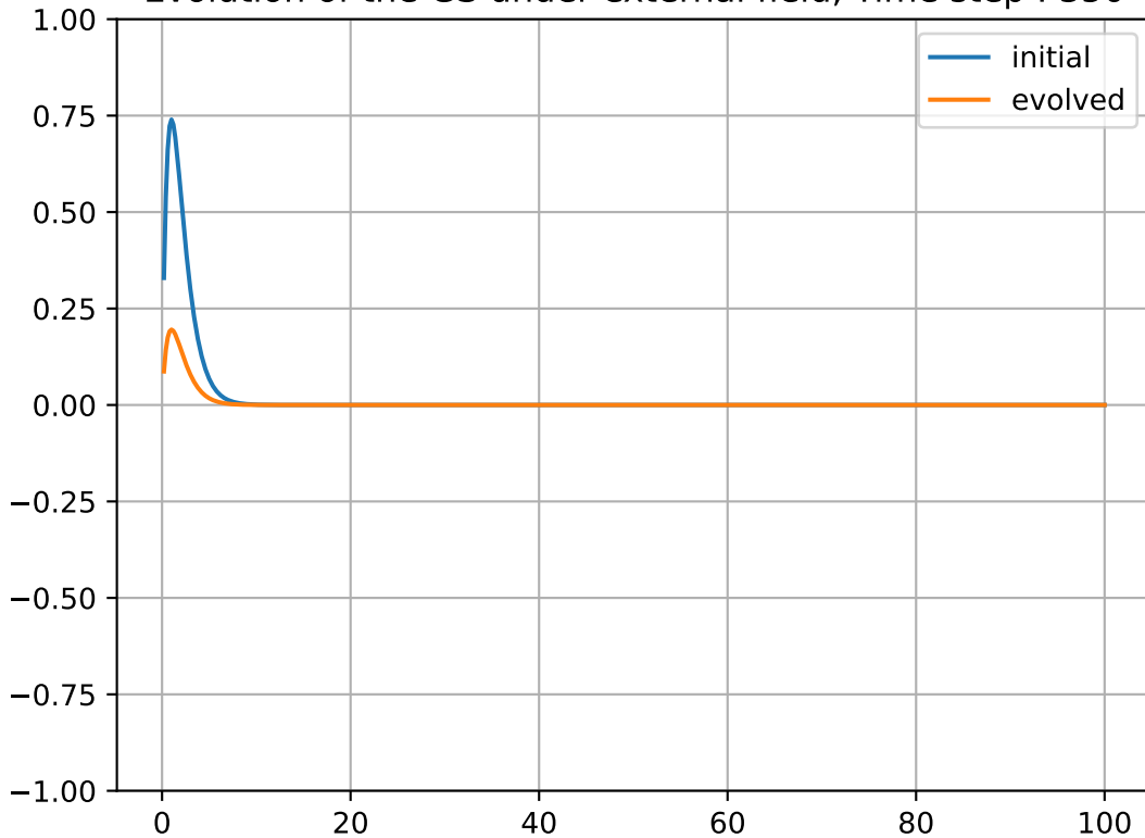
Evolution of the GS under external field, Time step : 350
