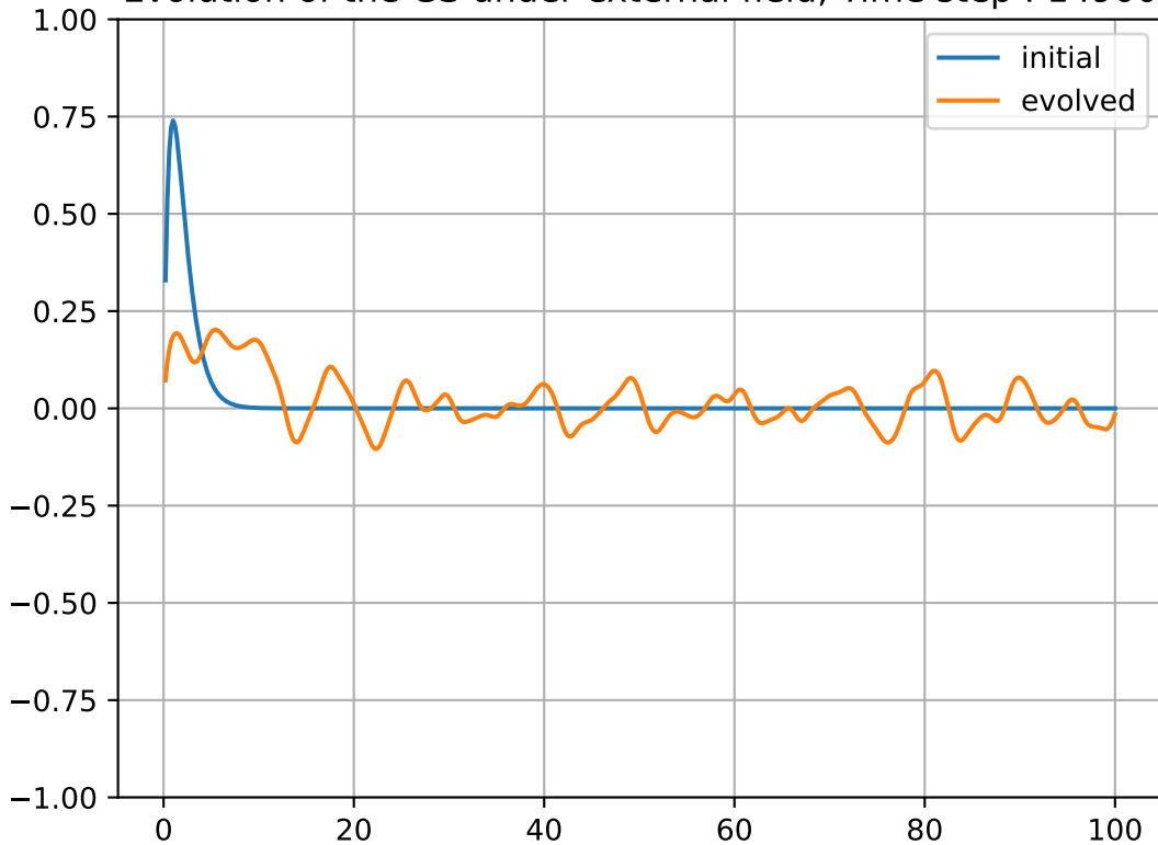
Evolution of the GS under external field, Time step : 14900
