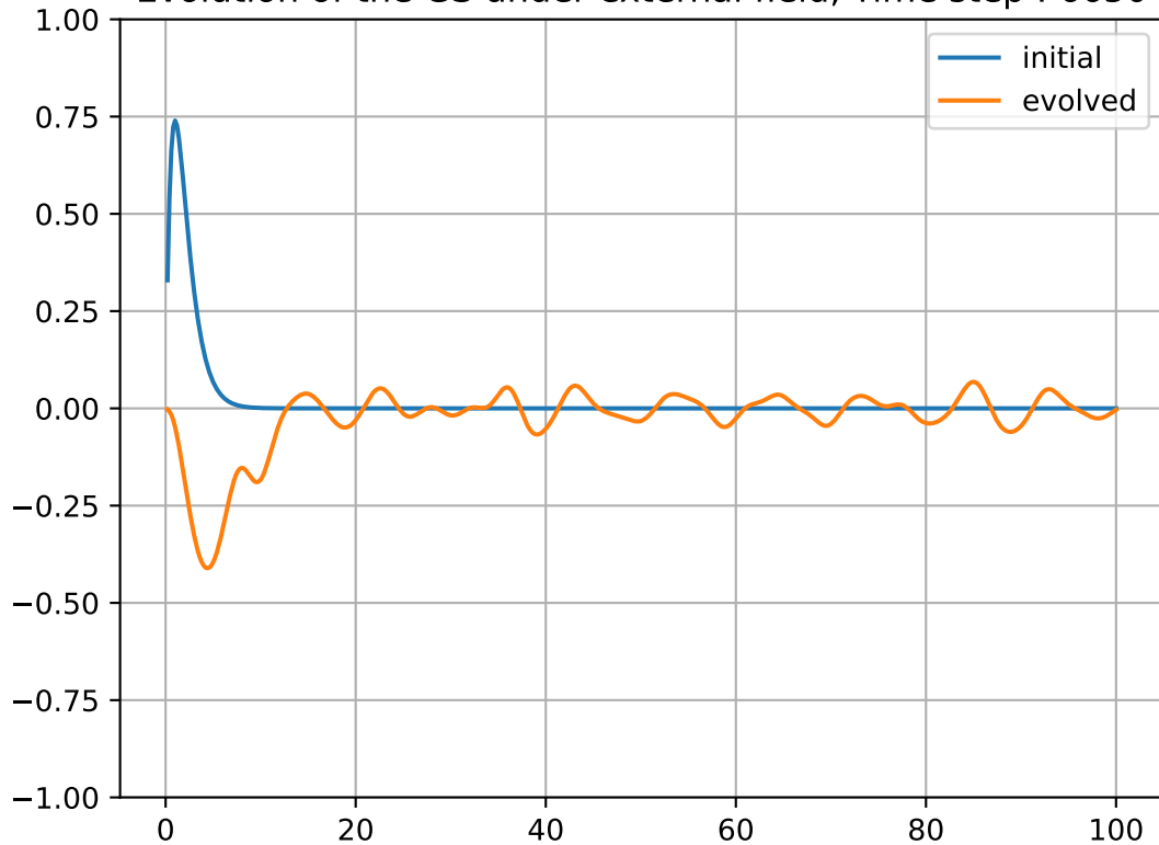
Evolution of the GS under external field, Time step : 6650
