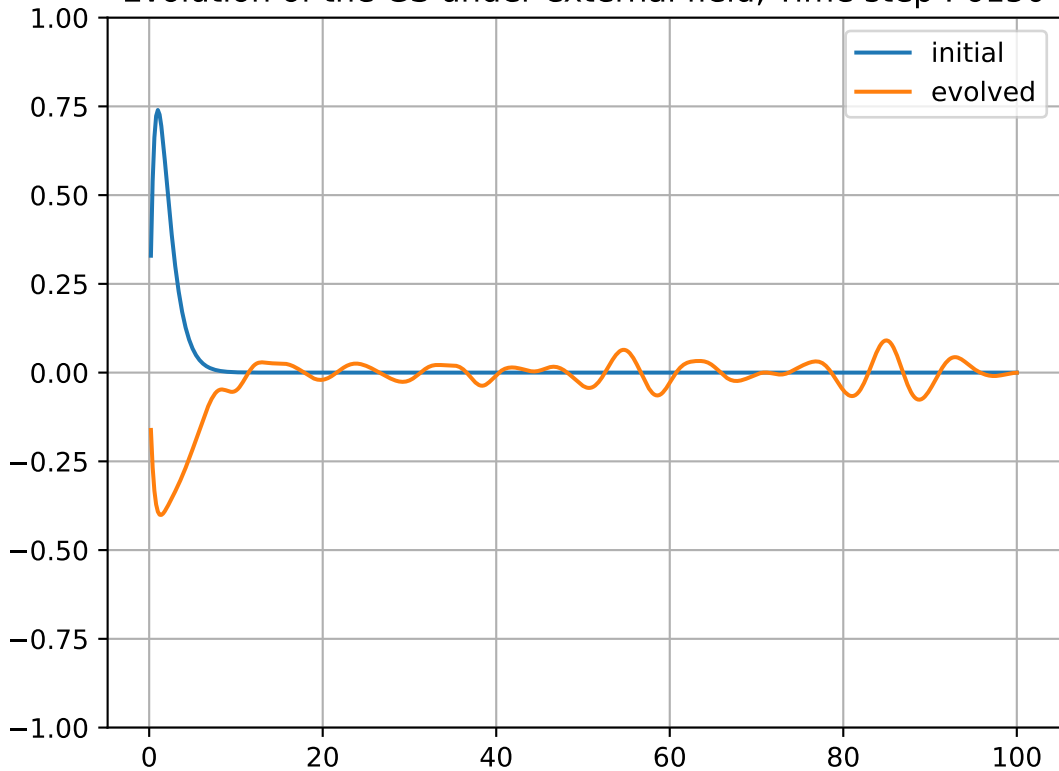
Evolution of the GS under external field, Time step : 6150
