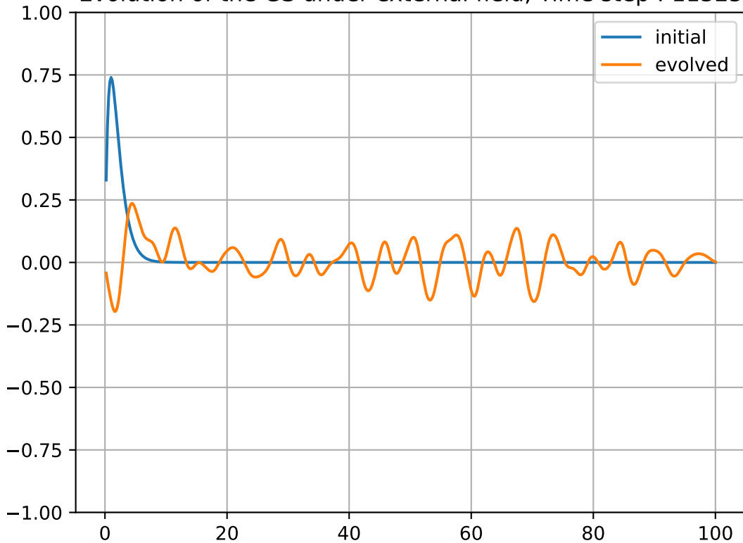
Evolution of the GS under external field, Time step : 11325
