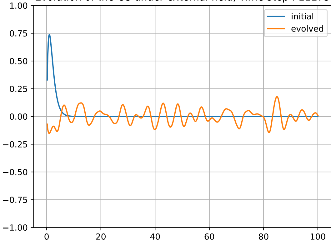
Evolution of the GS under external field, Time step : 11175
