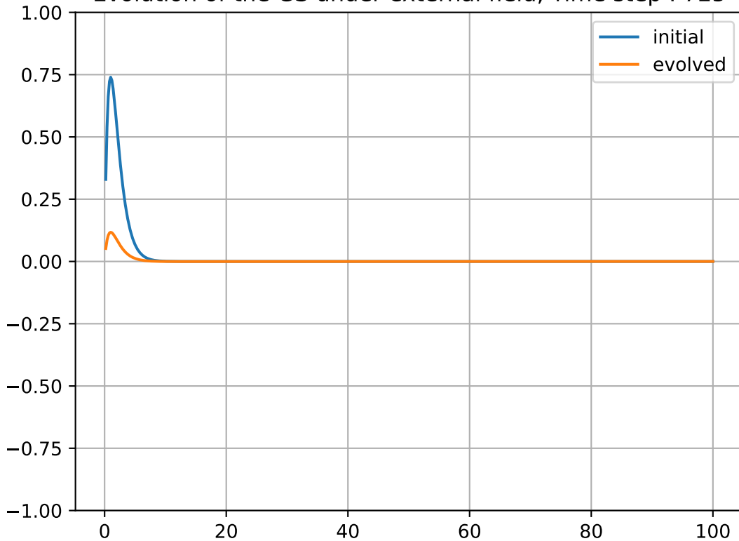
Evolution of the GS under external field, Time step : 725
