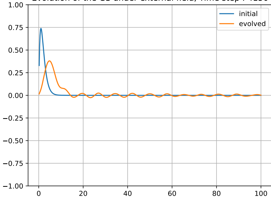
Evolution of the GS under external field, Time step : 4150
