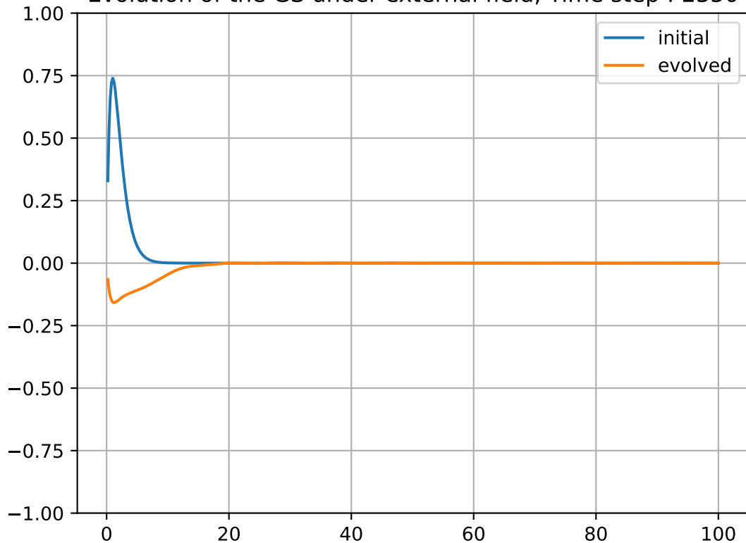
Evolution of the GS under external field, Time step : 2350
