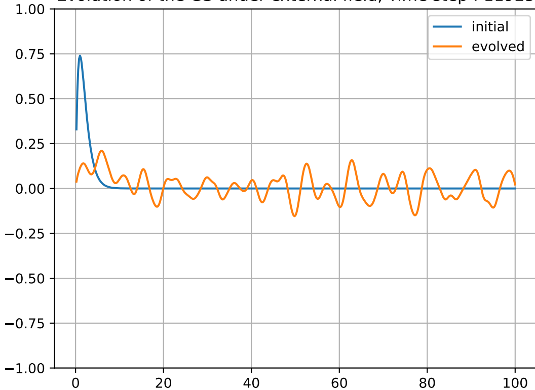
Evolution of the GS under external field, Time step : 11925
