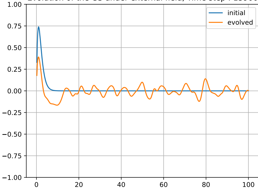
Evolution of the GS under external field, Time step : 13900
