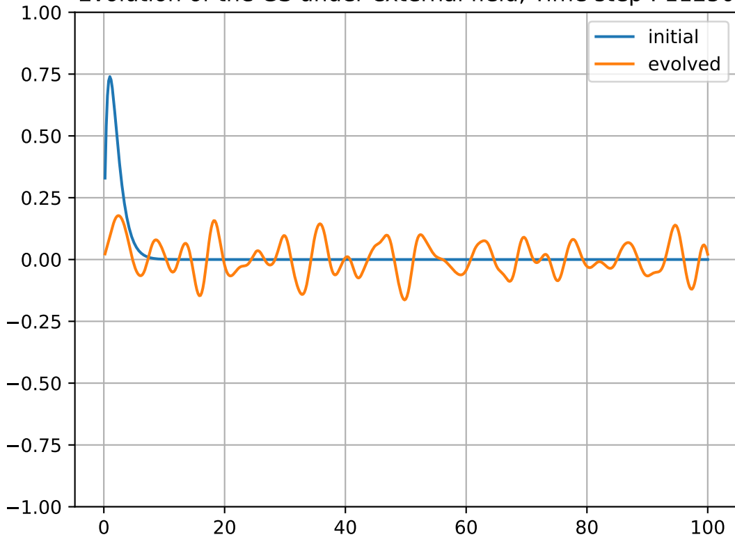
Evolution of the GS under external field, Time step : 11250
