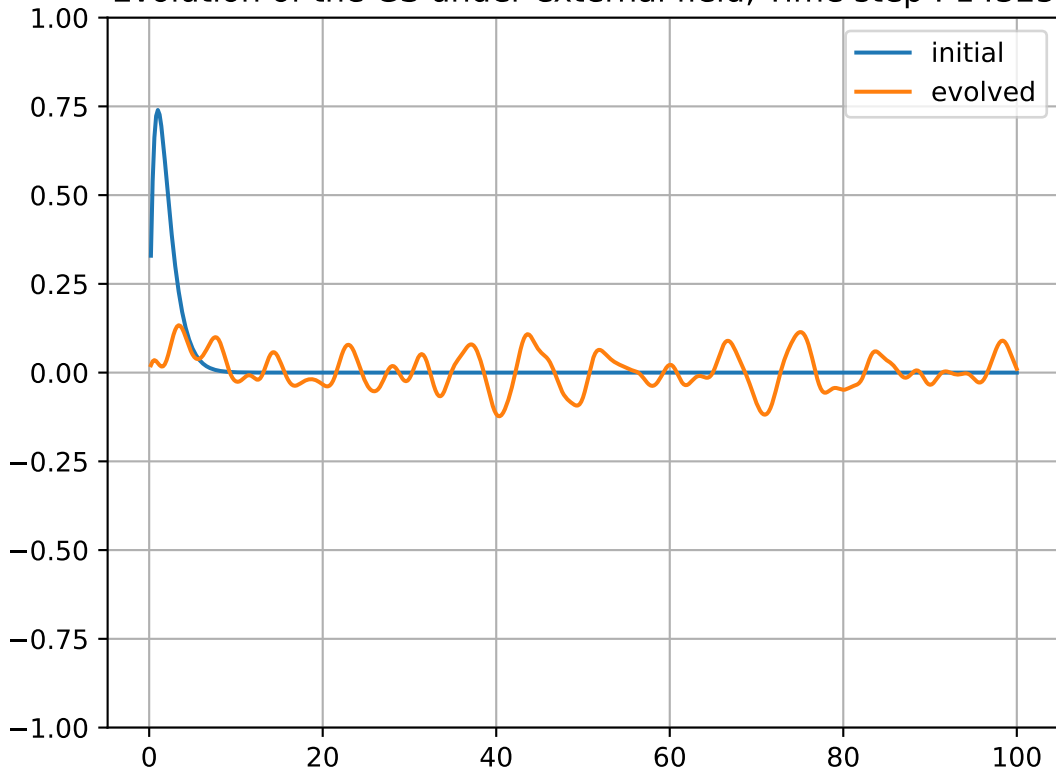
Evolution of the GS under external field, Time step : 14325
