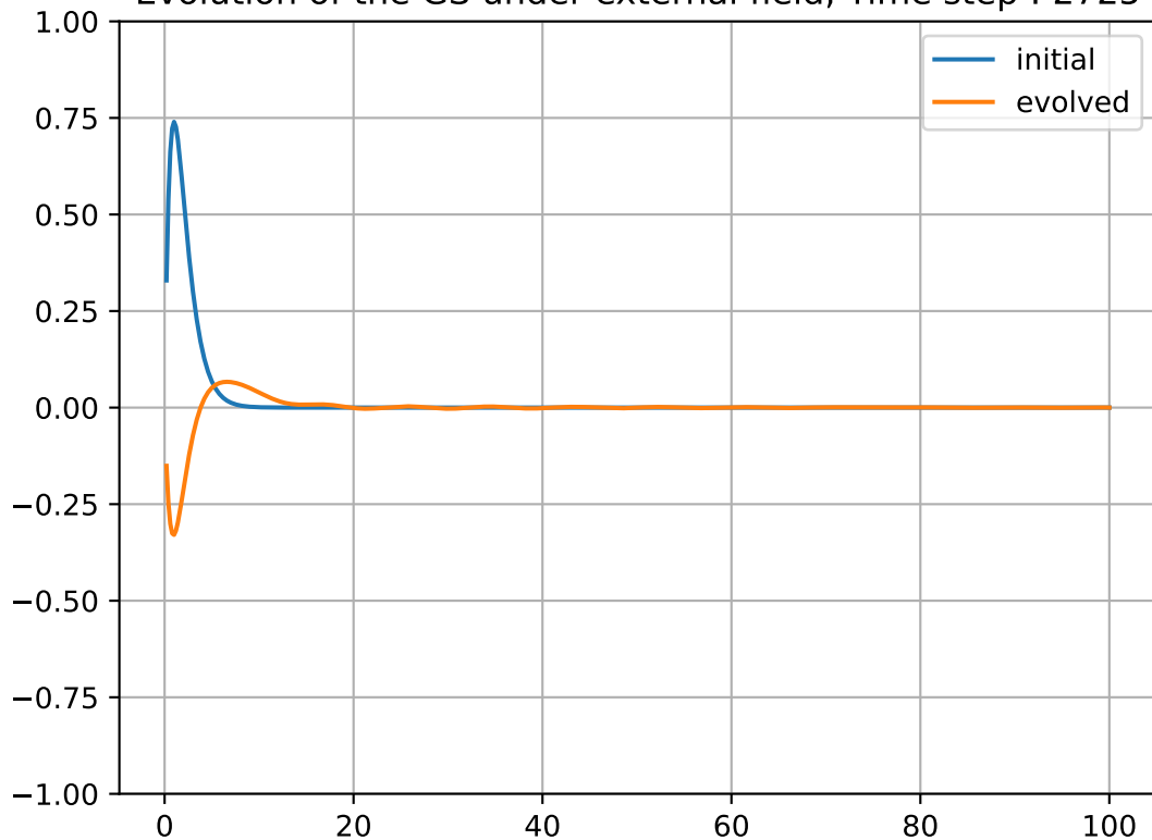
Evolution of the GS under external field, Time step : 2725
