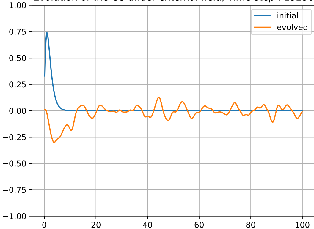
Evolution of the GS under external field, Time step : 15250
