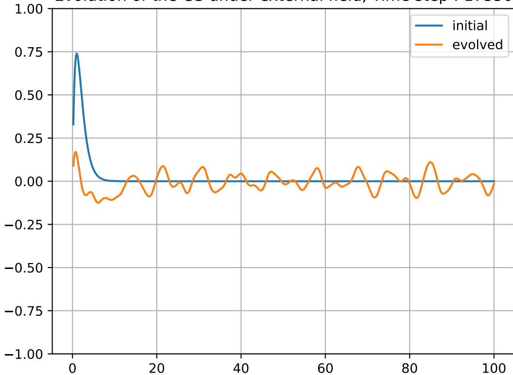
Evolution of the GS under external field, Time step : 17350
