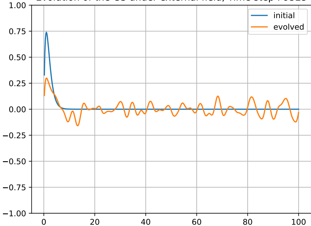
Evolution of the GS under external field, Time step : 9525
