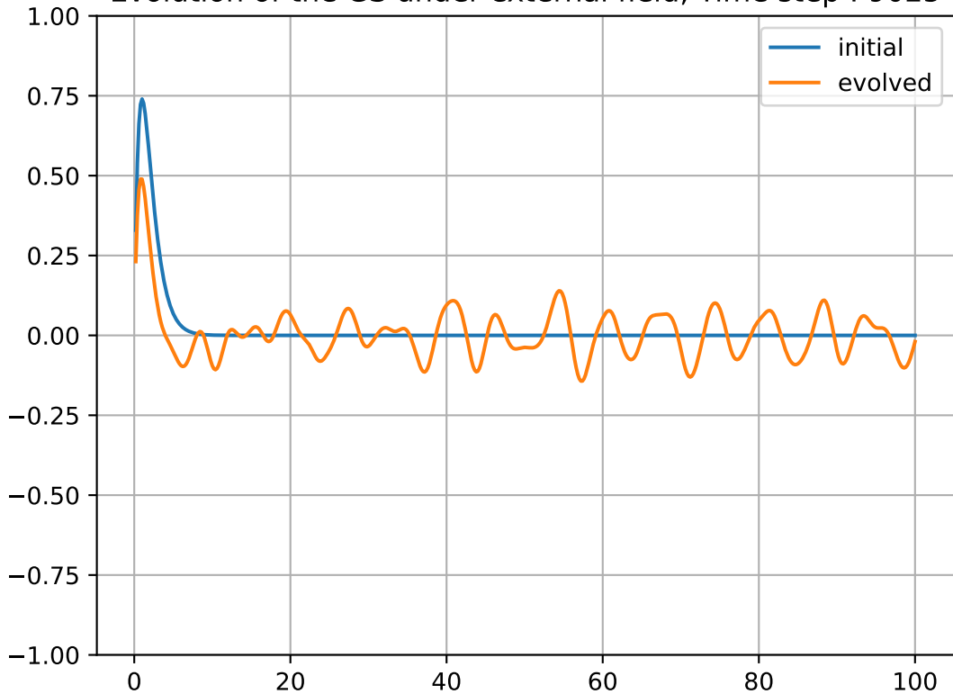
Evolution of the GS under external field, Time step : 9025
