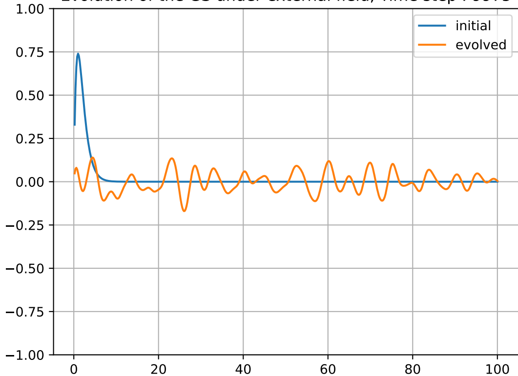
Evolution of the GS under external field, Time step : 9975
