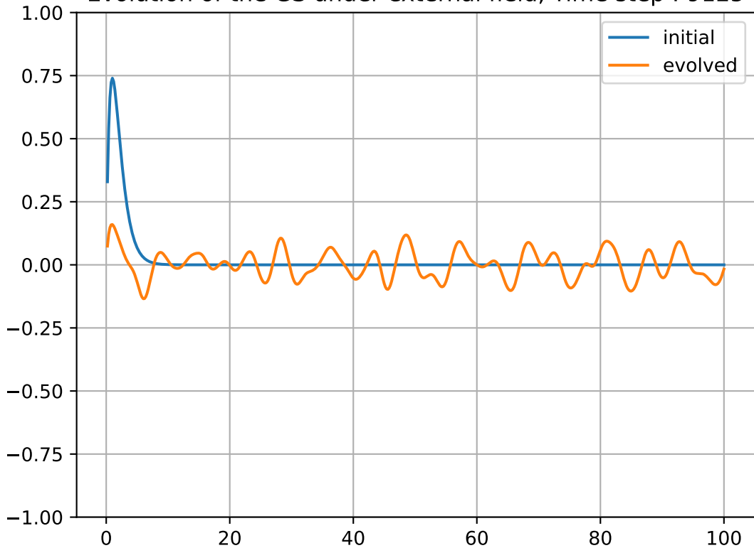
Evolution of the GS under external field, Time step : 9125
