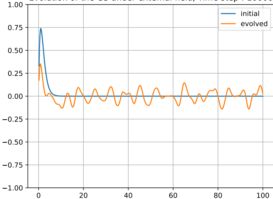
Evolution of the GS under external field, Time step : 10600
