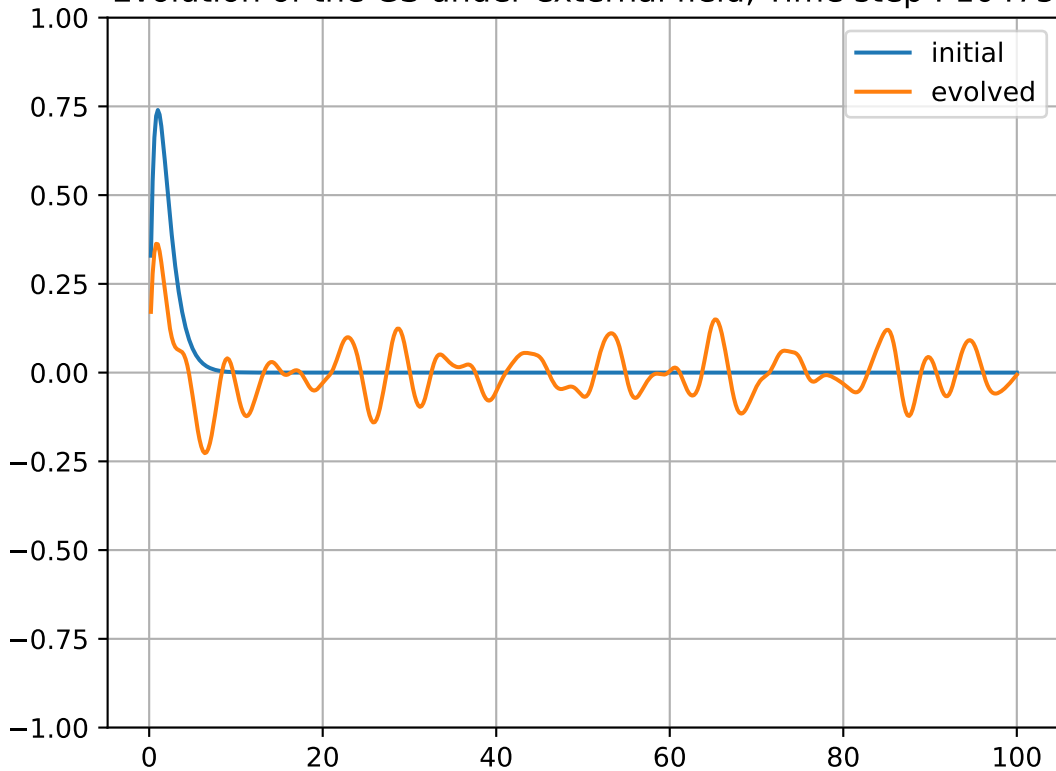
Evolution of the GS under external field, Time step : 10475
