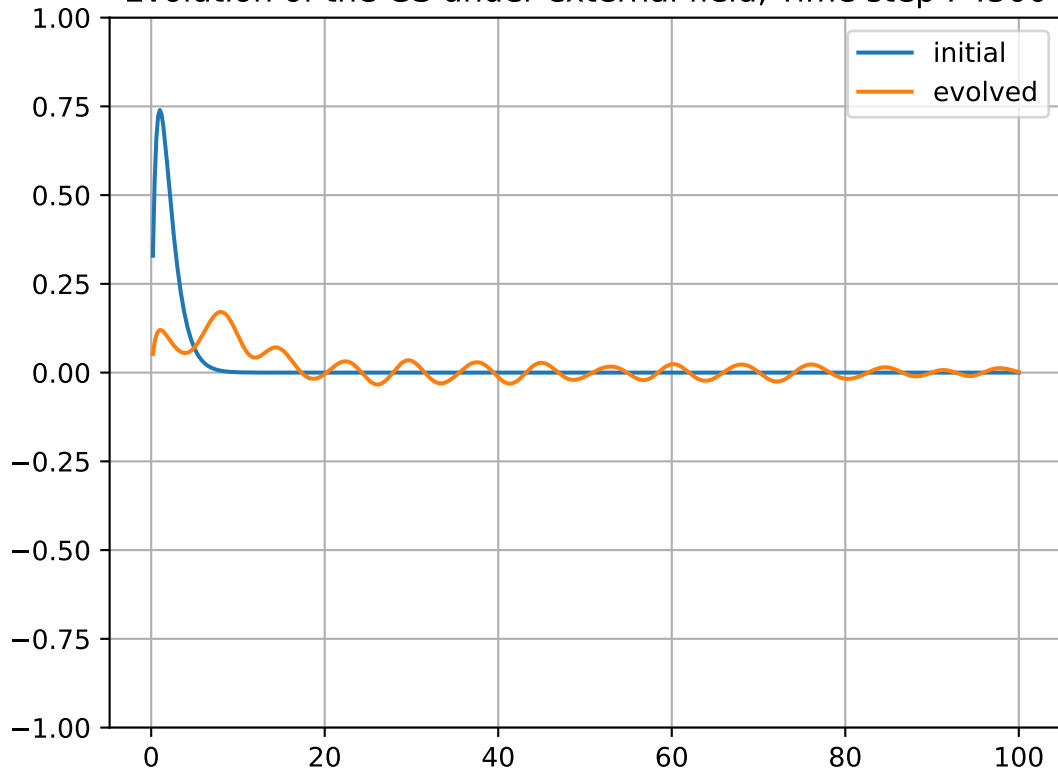
Evolution of the GS under external field, Time step : 4500
