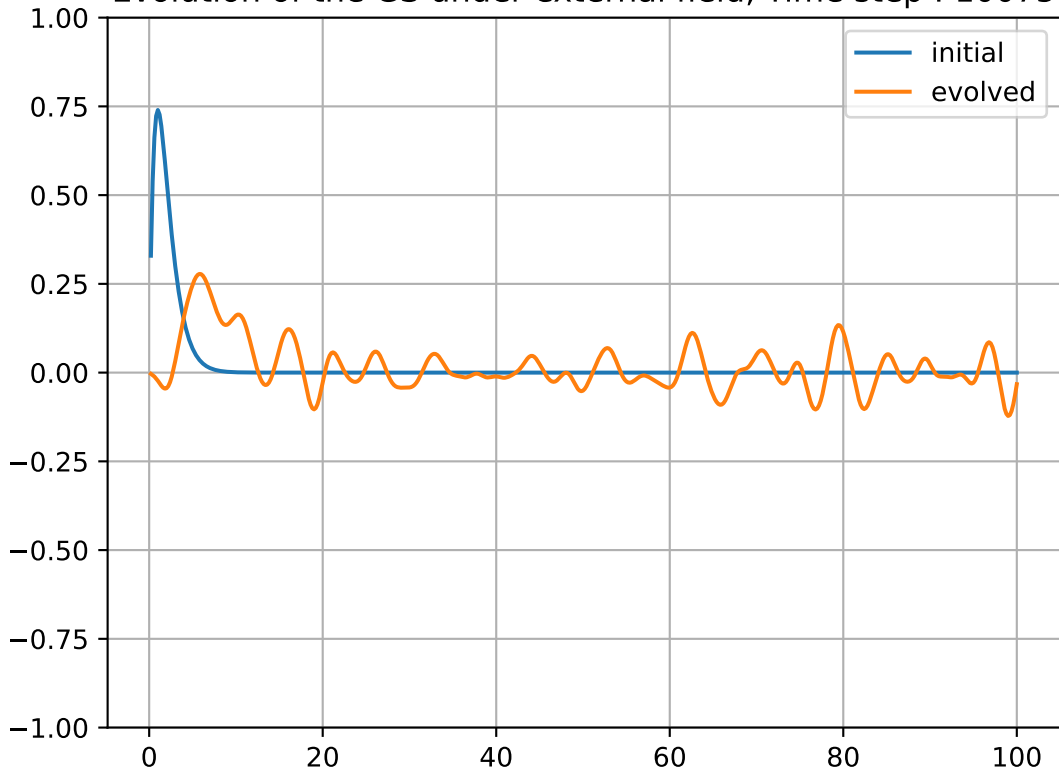
Evolution of the GS under external field, Time step : 10075
