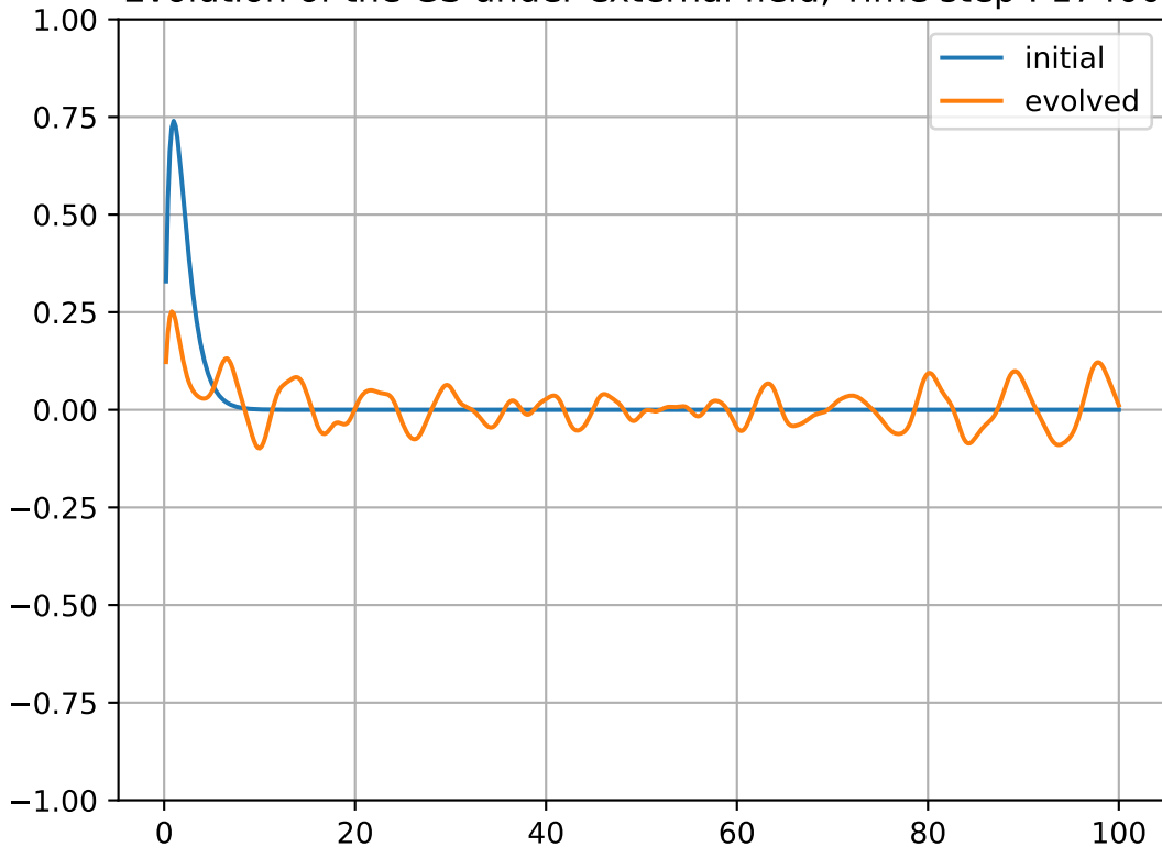
Evolution of the GS under external field, Time step : 17400
