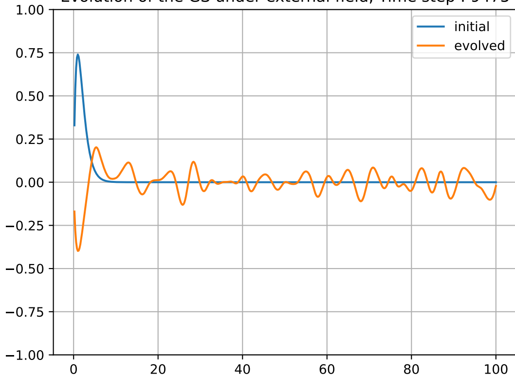
Evolution of the GS under external field, Time step : 9475
