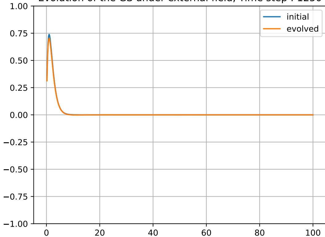
Evolution of the GS under external field, Time step : 1250
