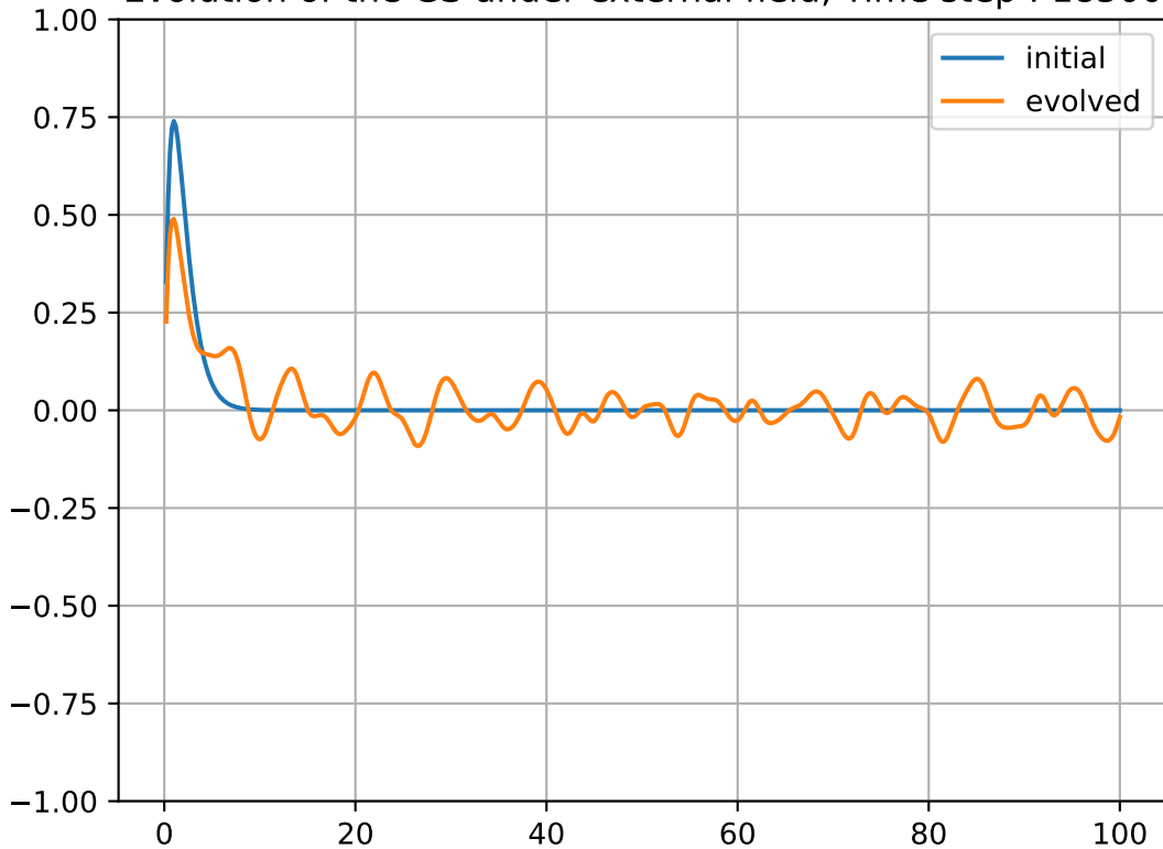
Evolution of the GS under external field, Time step : 18500
