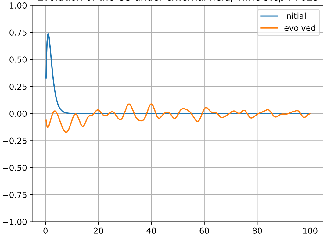
Evolution of the GS under external field, Time step : 7025
