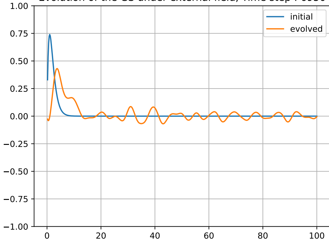
Evolution of the GS under external field, Time step : 6950
