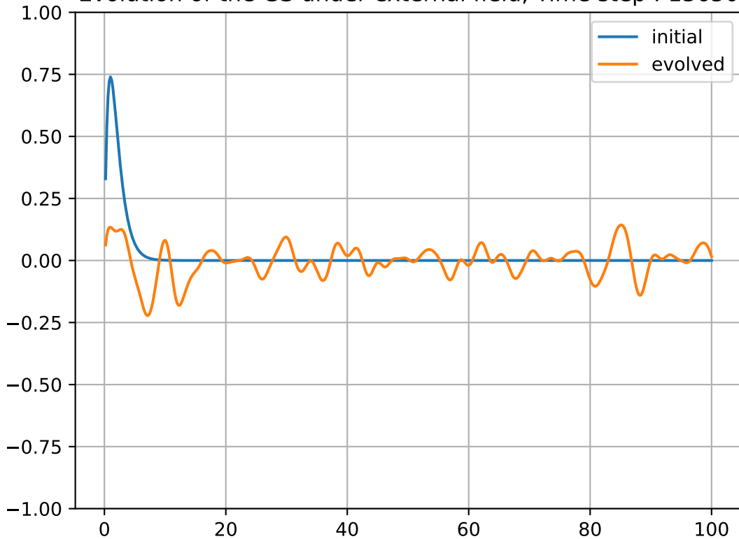
Evolution of the GS under external field, Time step : 13650
