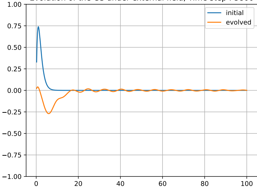
Evolution of the GS under external field, Time step : 3800
