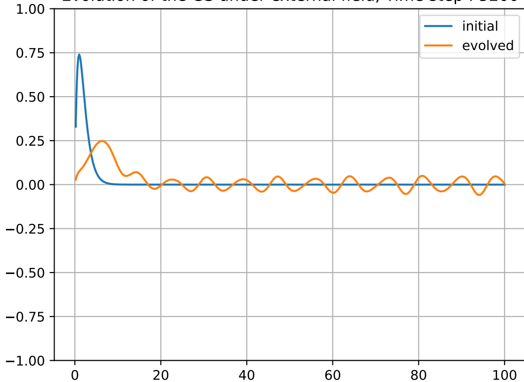
Evolution of the GS under external field, Time step : 5200
