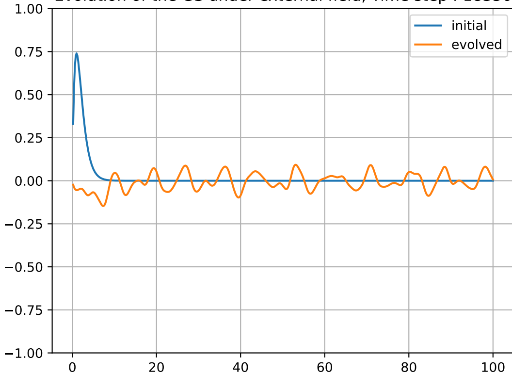
Evolution of the GS under external field, Time step : 18350
