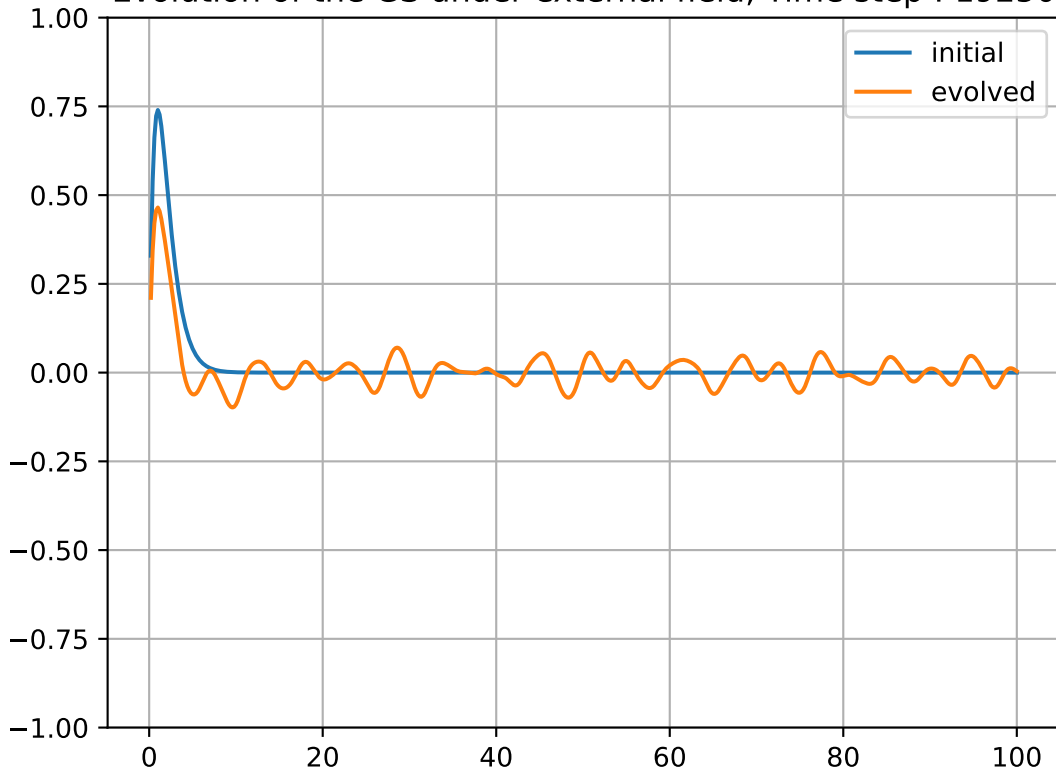
Evolution of the GS under external field, Time step : 19250
