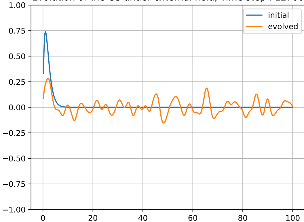
Evolution of the GS under external field, Time step : 12700
