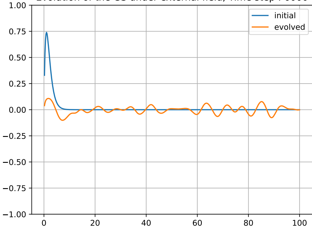
Evolution of the GS under external field, Time step : 6000
