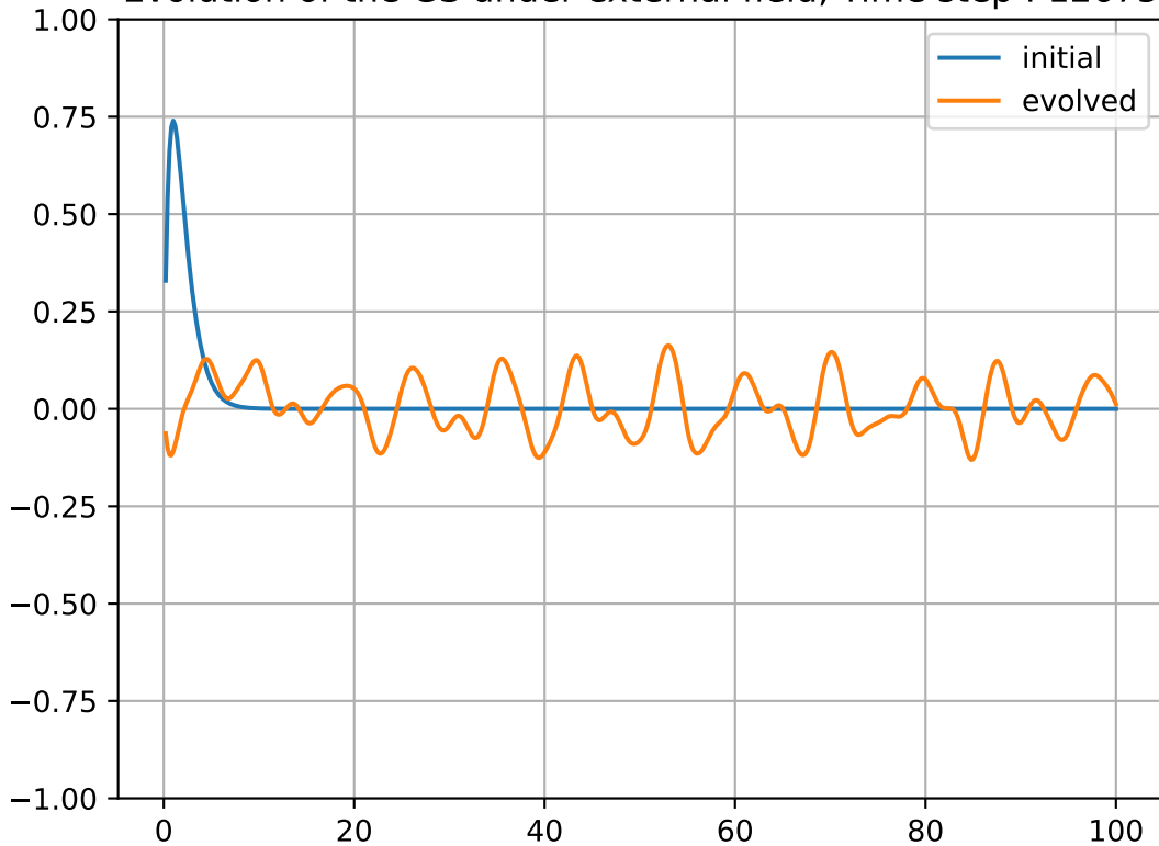
Evolution of the GS under external field, Time step : 12675
