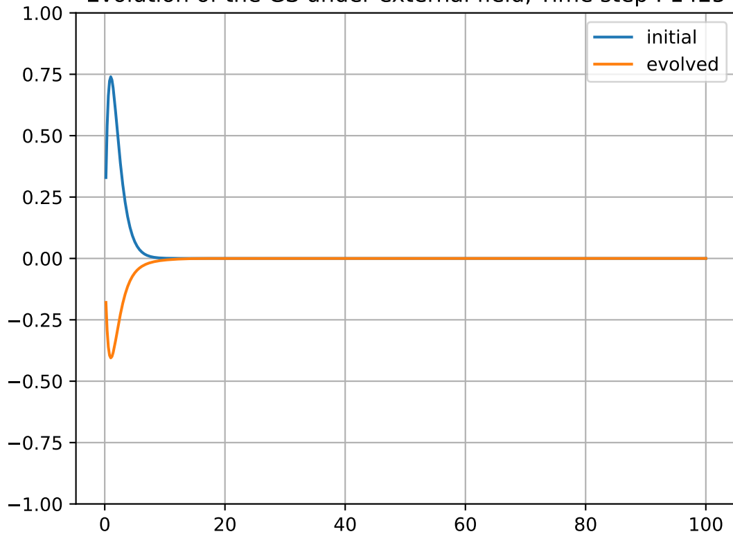
Evolution of the GS under external field, Time step : 1425
