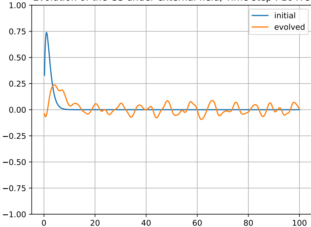
Evolution of the GS under external field, Time step : 16475
