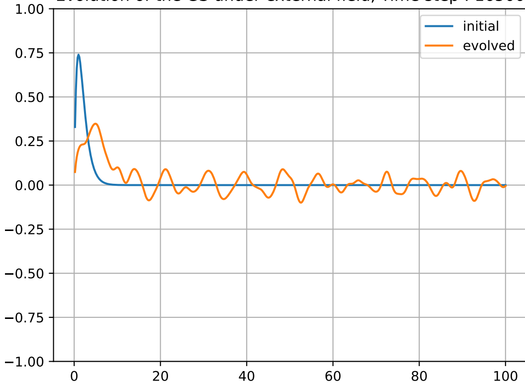
Evolution of the GS under external field, Time step : 16500
