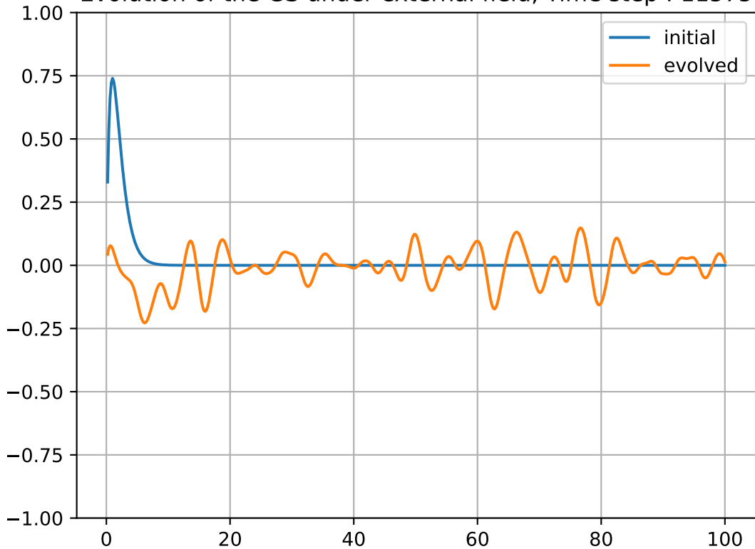
Evolution of the GS under external field, Time step : 11575
