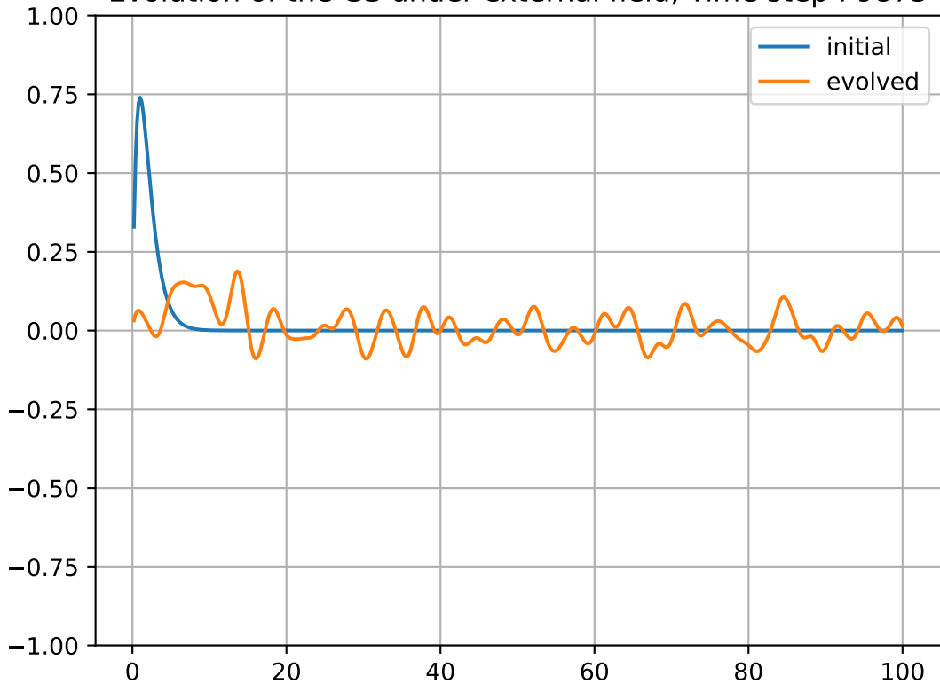
Evolution of the GS under external field, Time step : 9875
