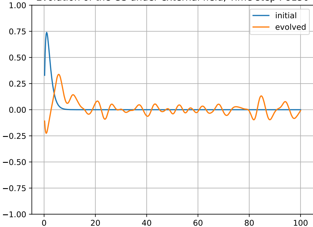
Evolution of the GS under external field, Time step : 8150
