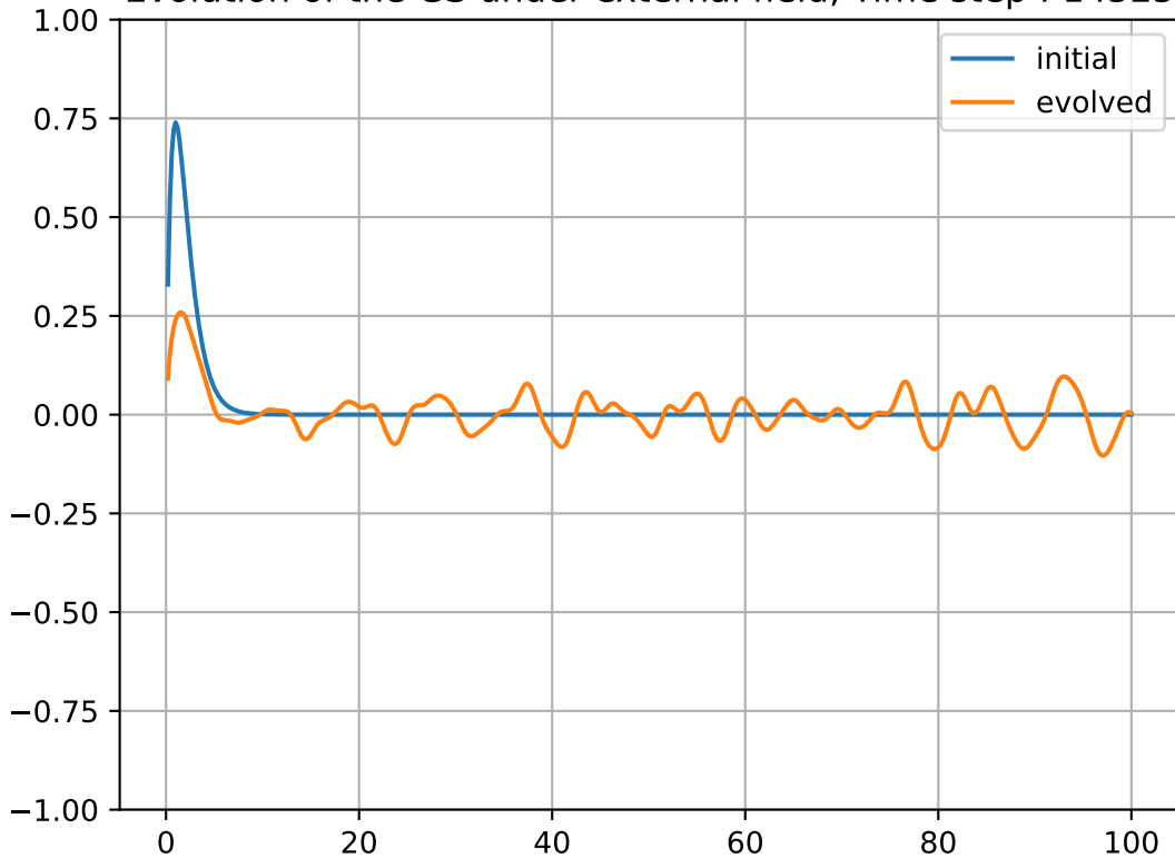
Evolution of the GS under external field, Time step : 14525
