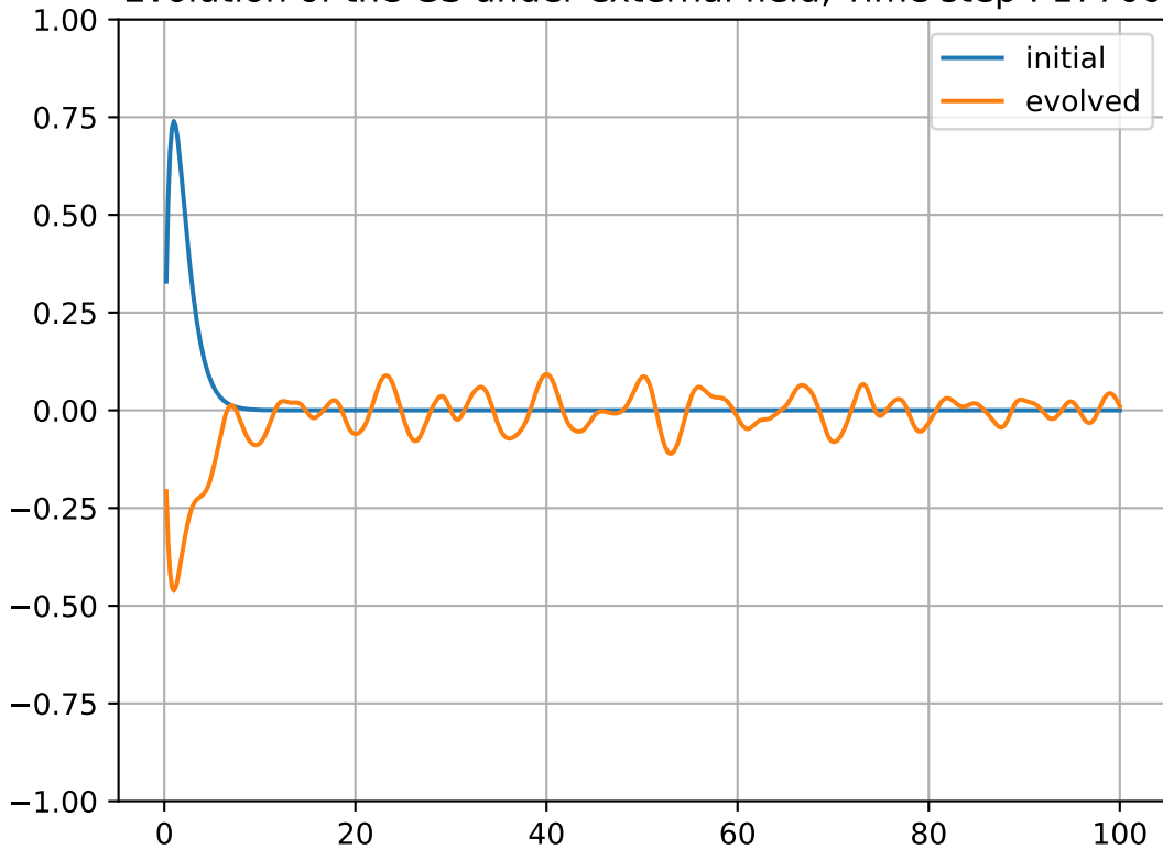
Evolution of the GS under external field, Time step : 17700
