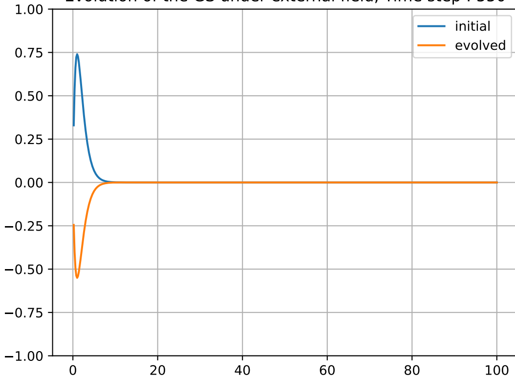
Evolution of the GS under external field, Time step : 550
