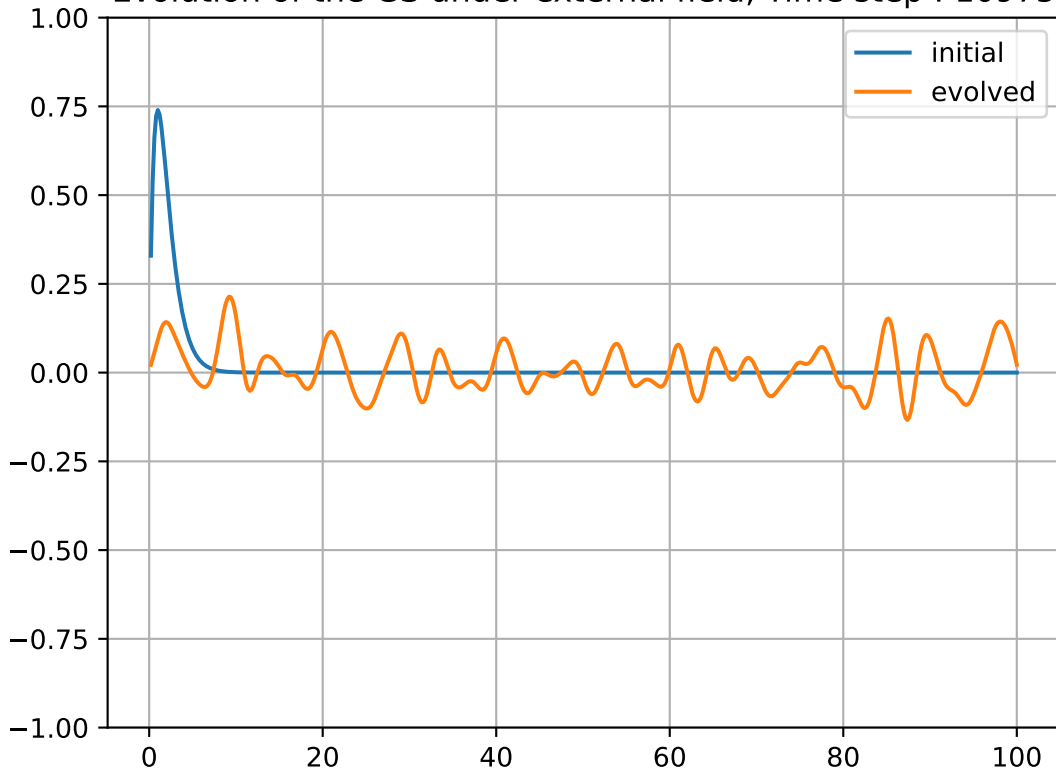
Evolution of the GS under external field, Time step : 10975
