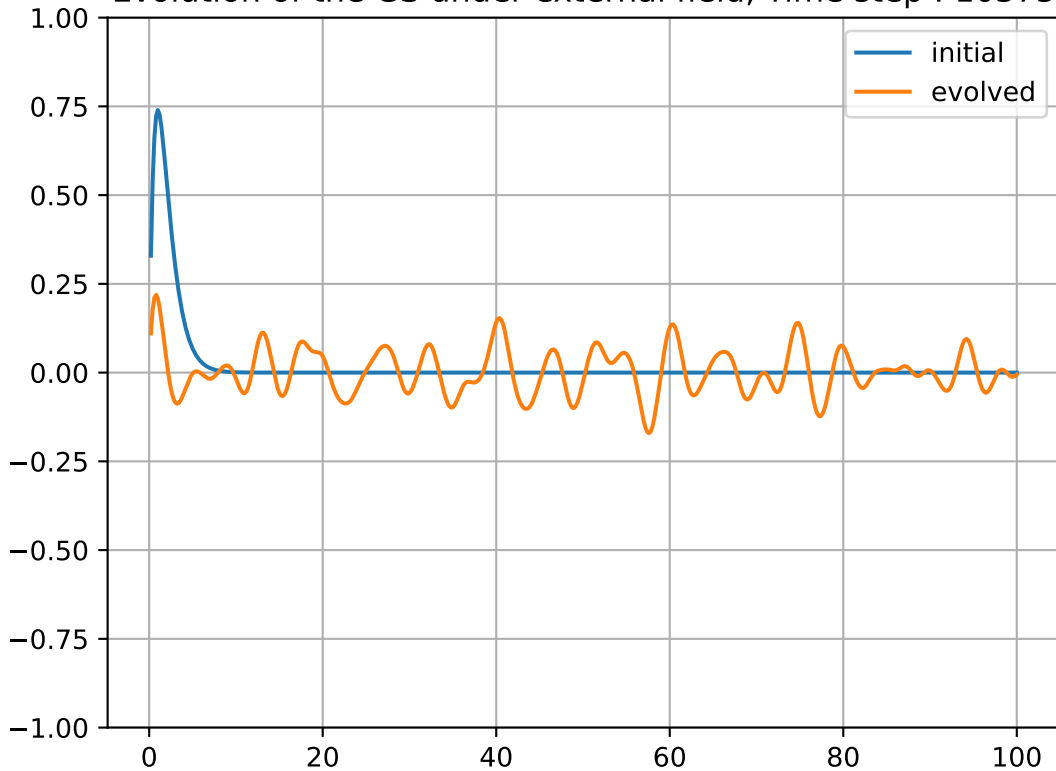
Evolution of the GS under external field, Time step : 10375
