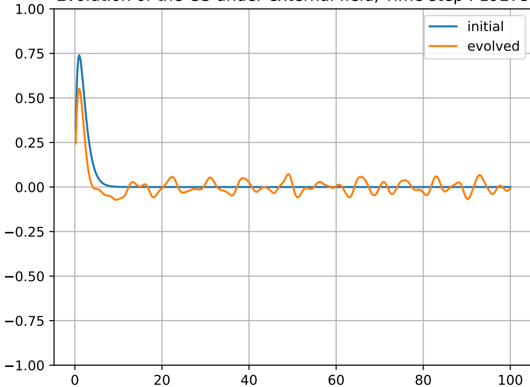
Evolution of the GS under external field, Time step : 19275
