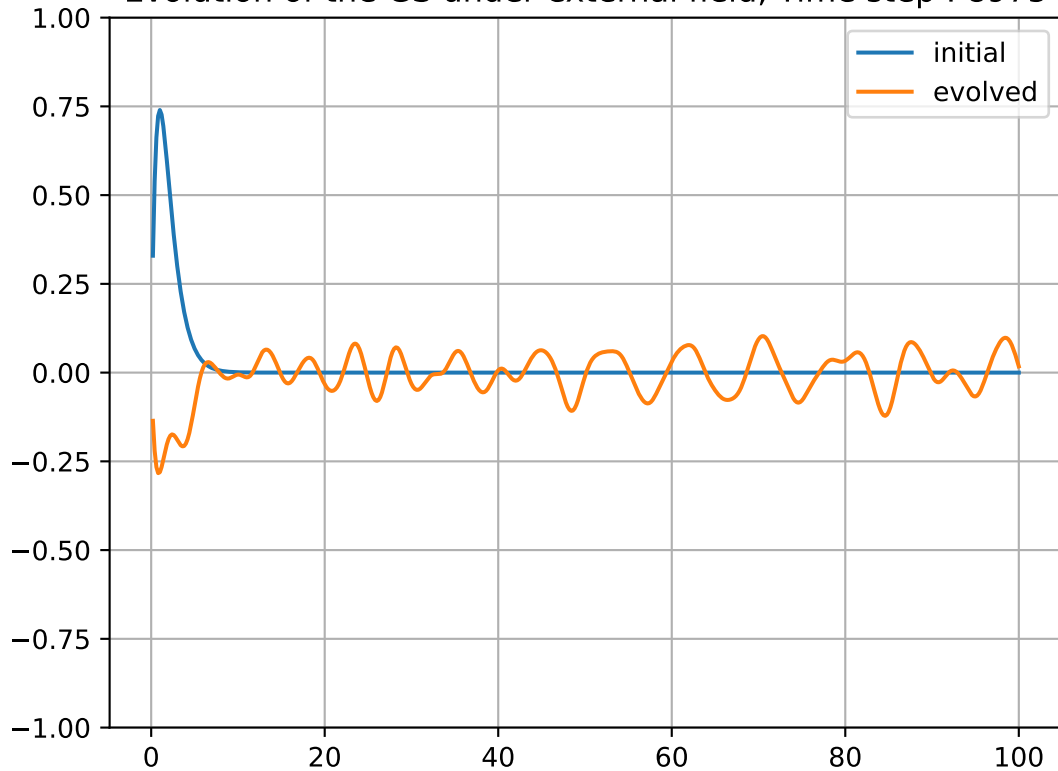
Evolution of the GS under external field, Time step : 8975
