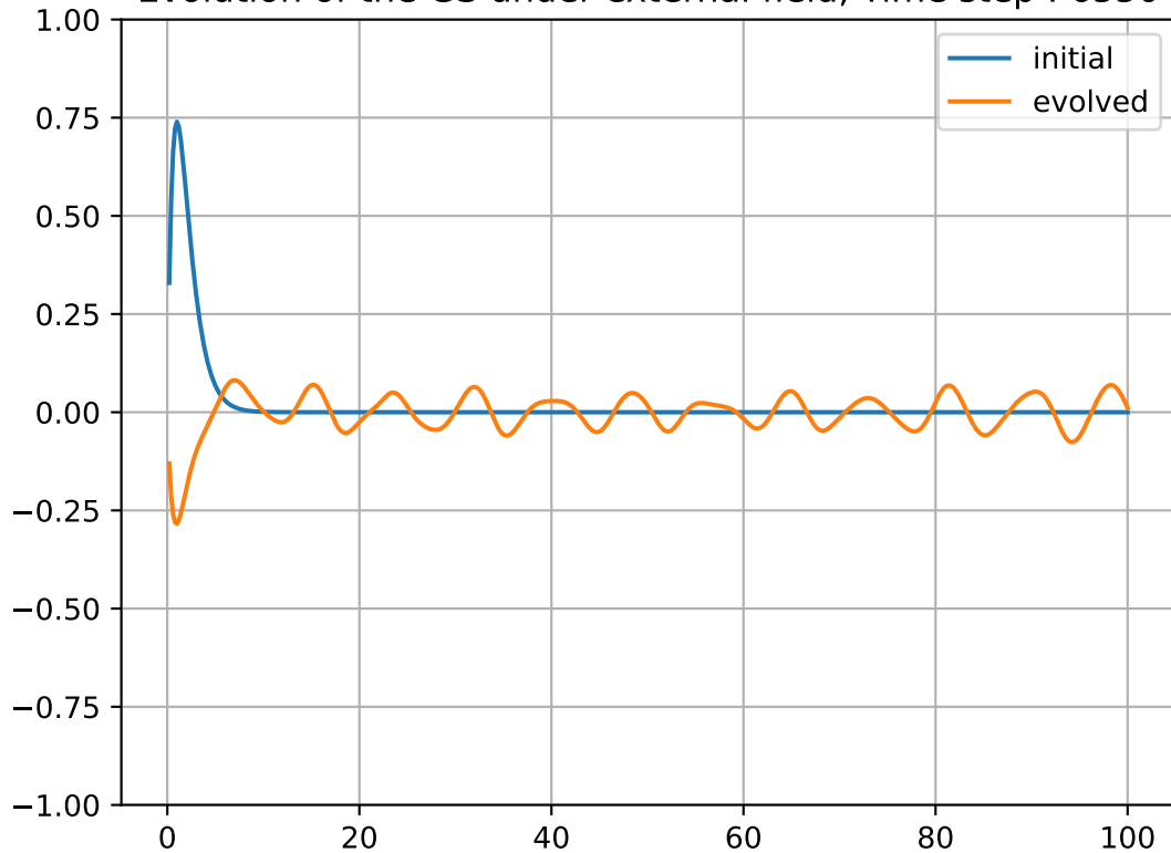
Evolution of the GS under external field, Time step : 6550
