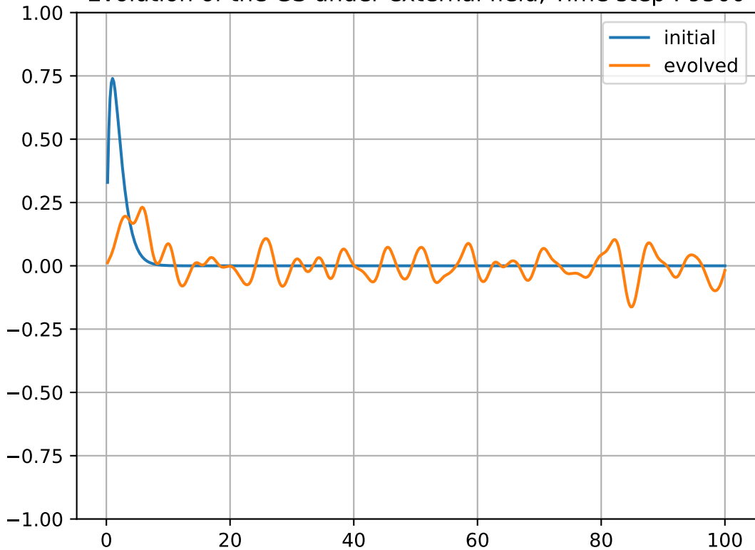
Evolution of the GS under external field, Time step : 9500
