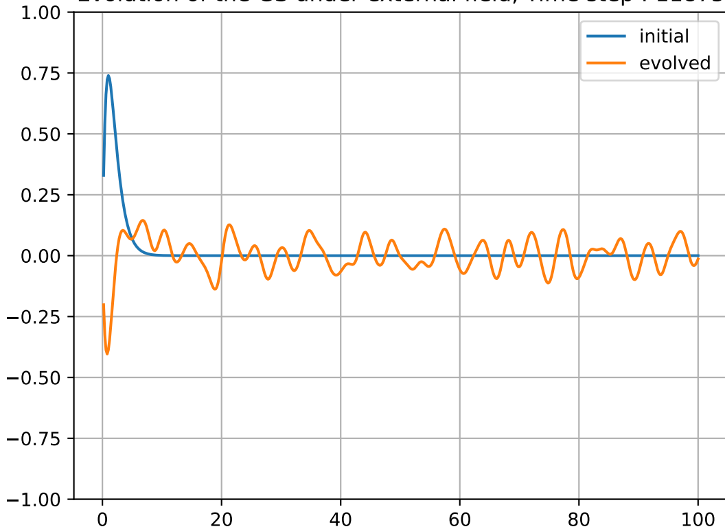
Evolution of the GS under external field, Time step : 11875
