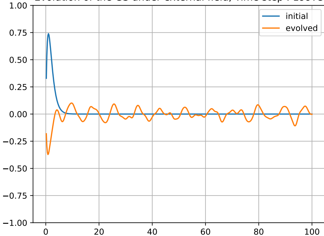
Evolution of the GS under external field, Time step : 19975
