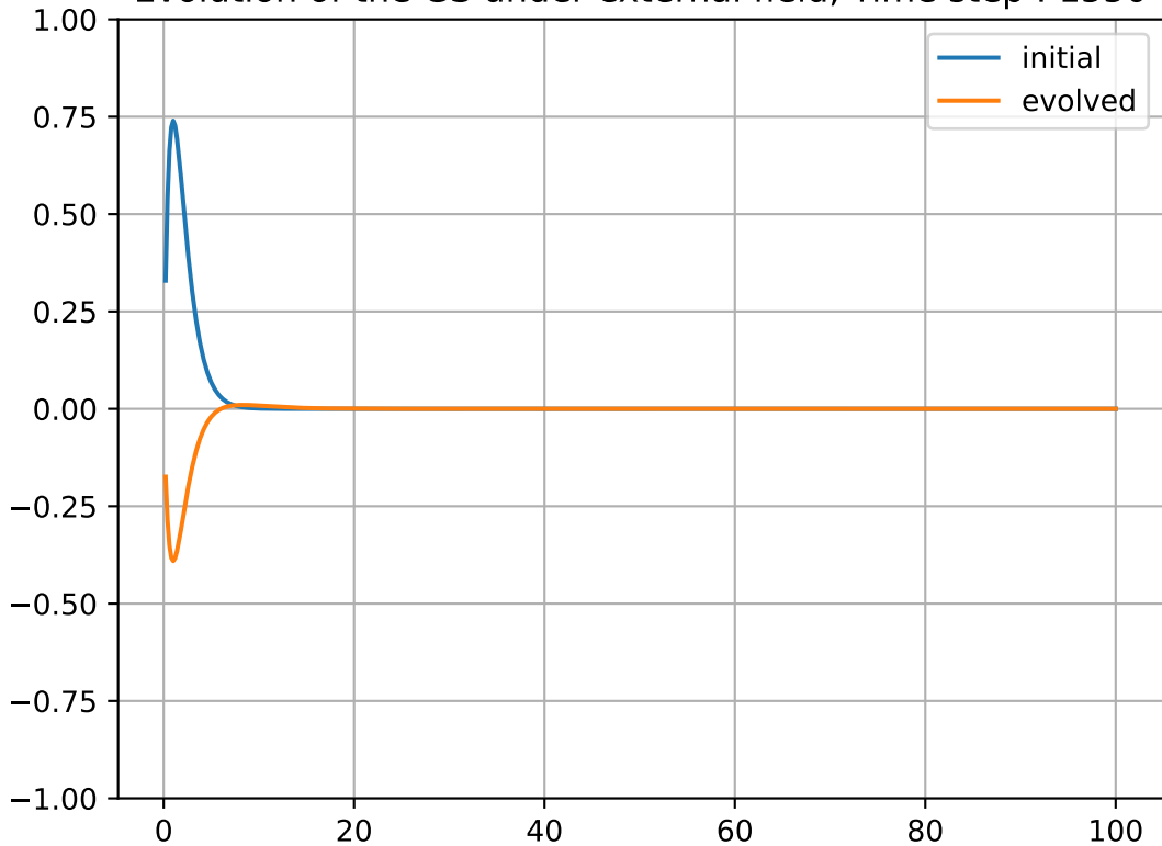
Evolution of the GS under external field, Time step : 1550
