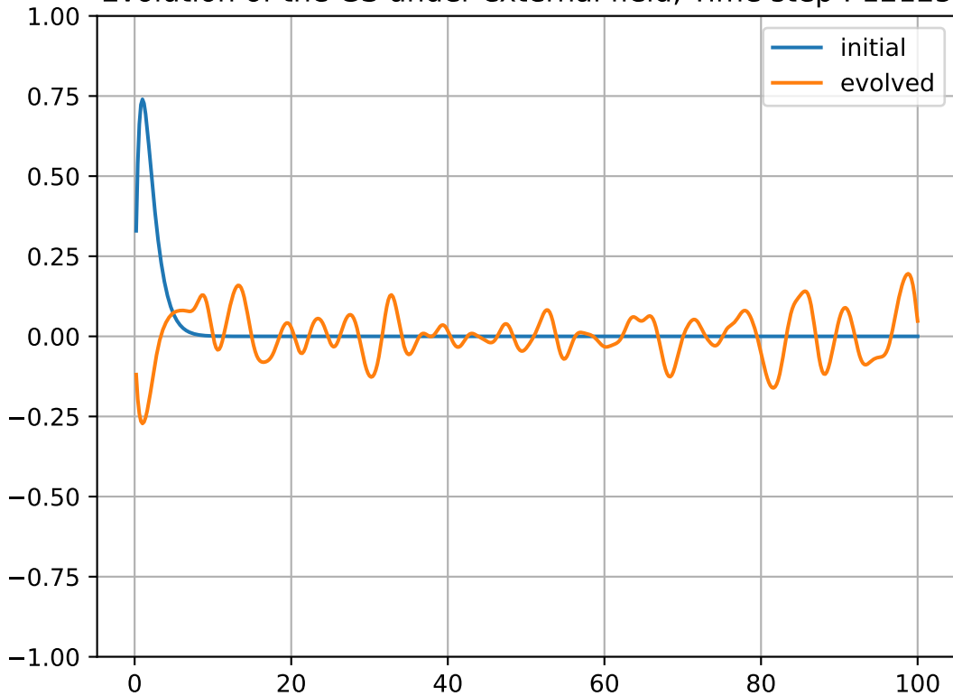
Evolution of the GS under external field, Time step : 12125
