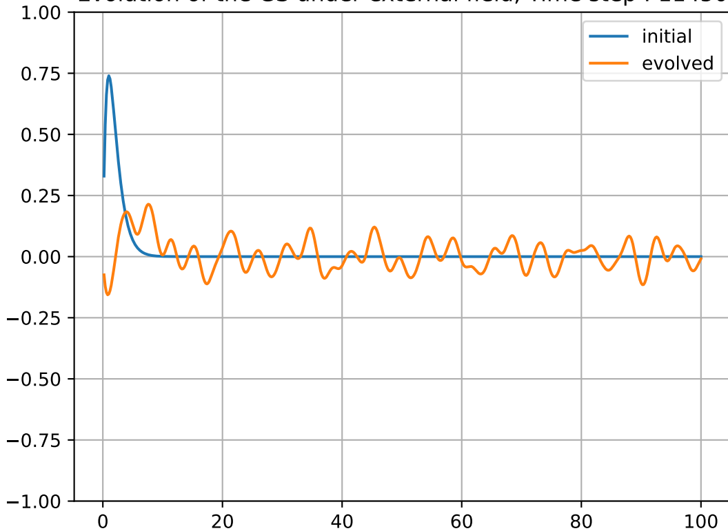
Evolution of the GS under external field, Time step : 11450
