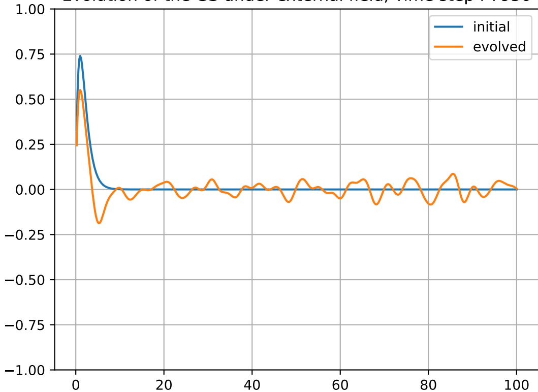
Evolution of the GS under external field, Time step : 7950
