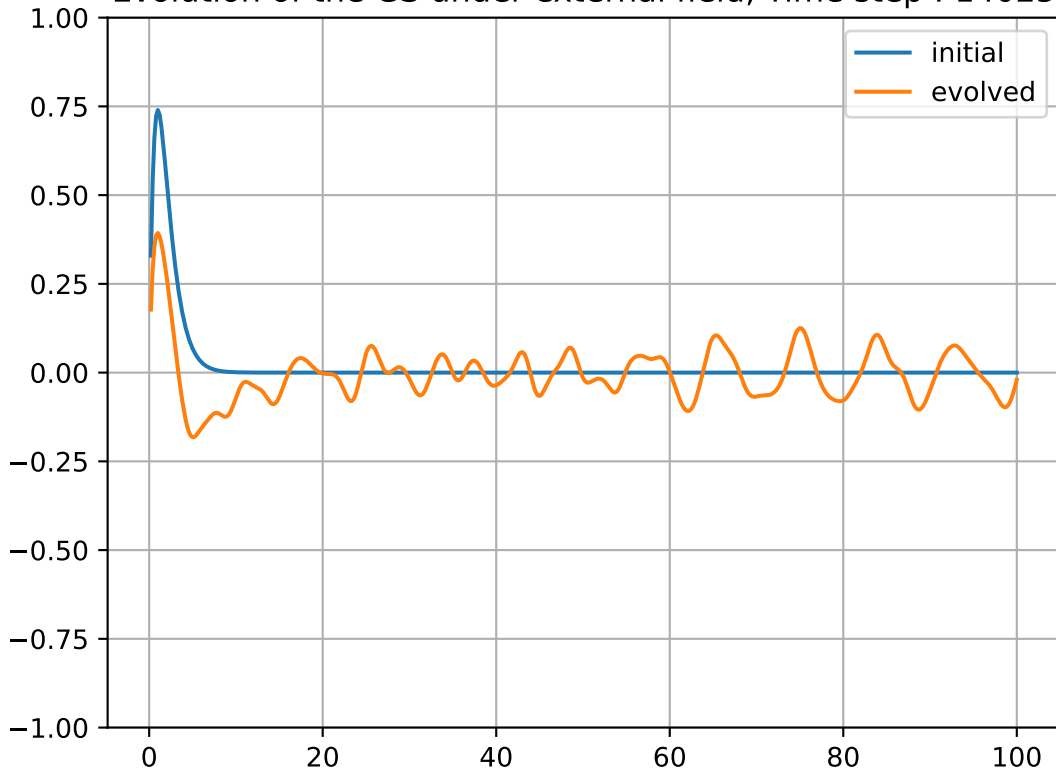
Evolution of the GS under external field, Time step : 14025
