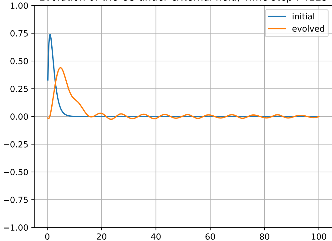
Evolution of the GS under external field, Time step : 4125
