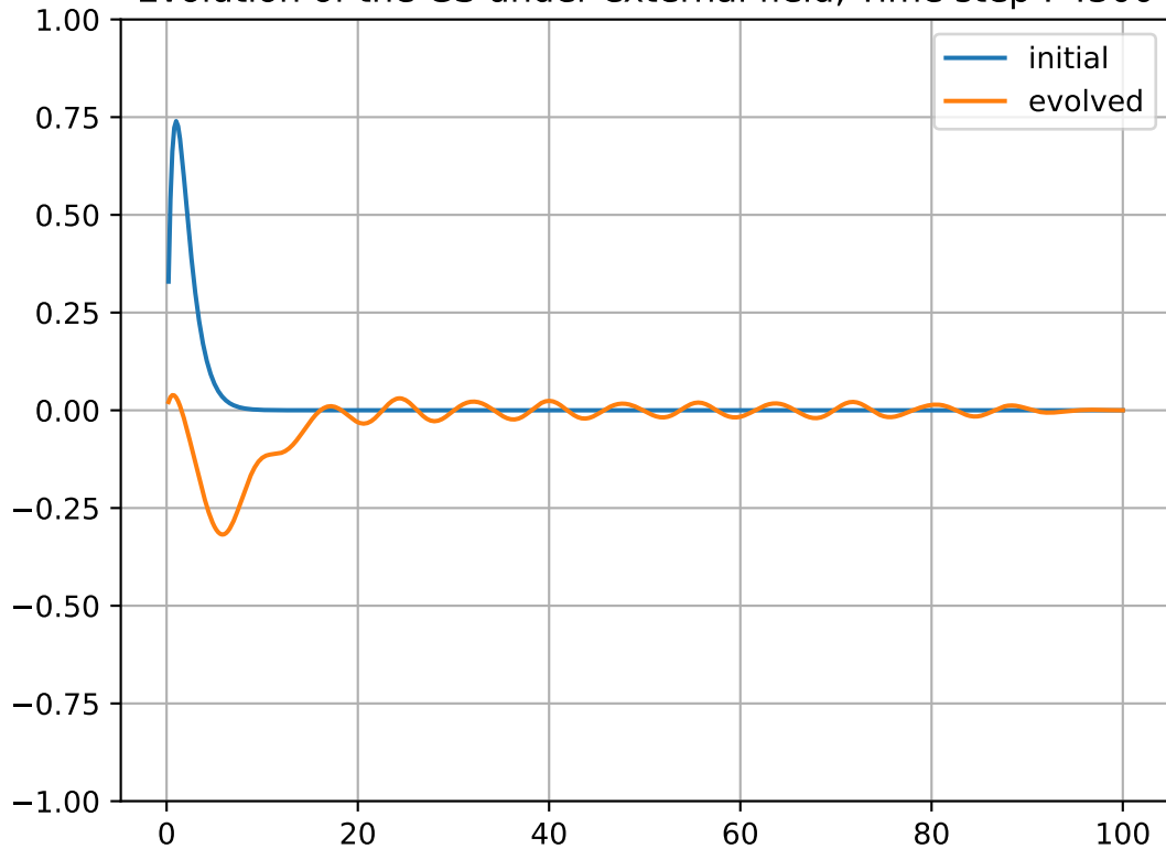
Evolution of the GS under external field, Time step : 4300
