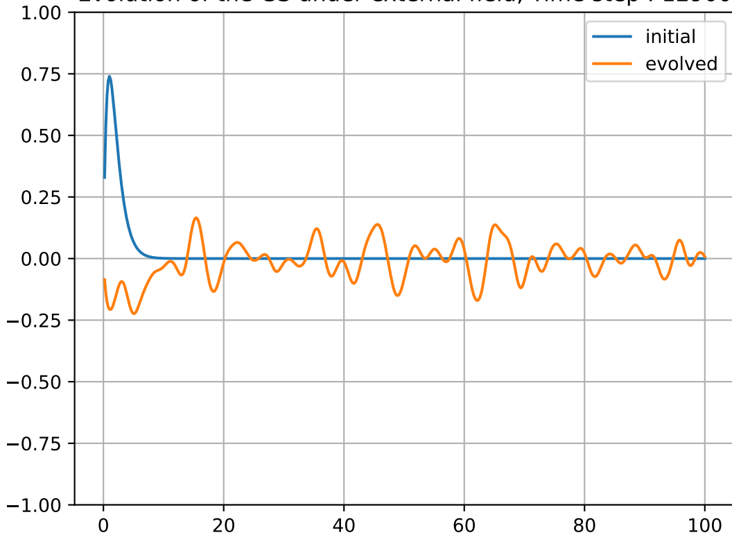
Evolution of the GS under external field, Time step : 12900
