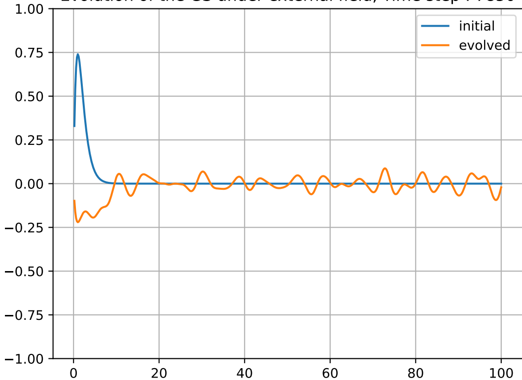
Evolution of the GS under external field, Time step : 7850
