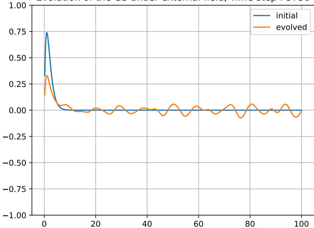
Evolution of the GS under external field, Time step : 5750
