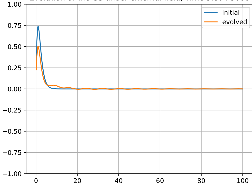
Evolution of the GS under external field, Time step : 3000
