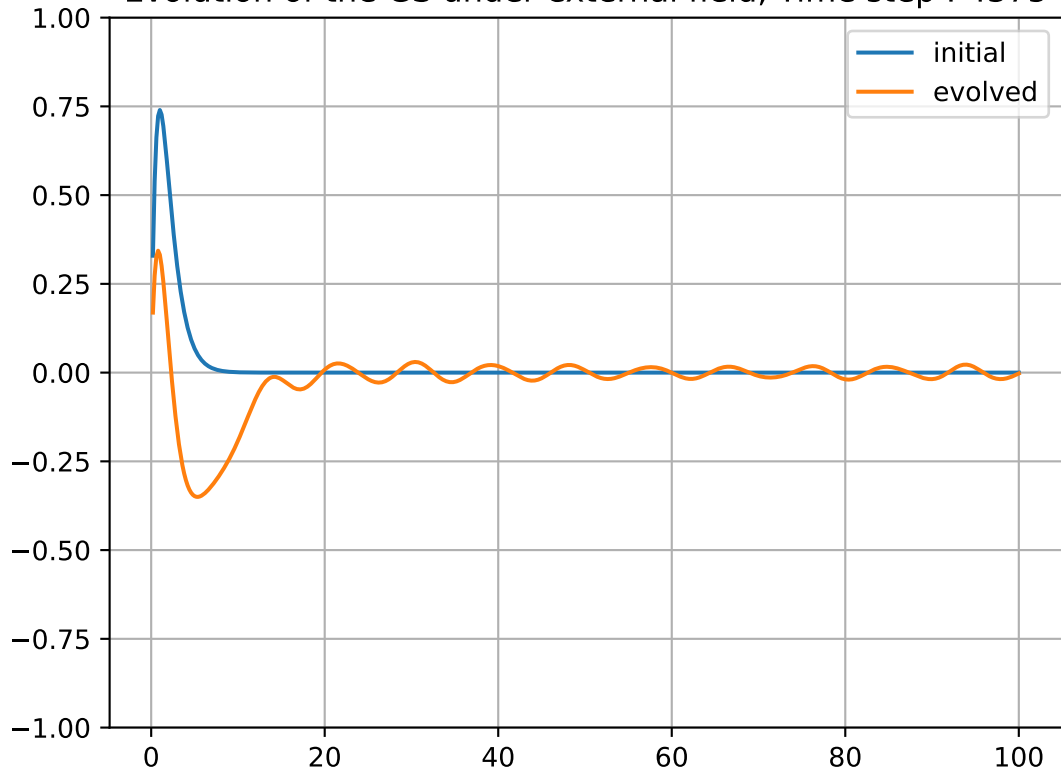
Evolution of the GS under external field, Time step : 4375
