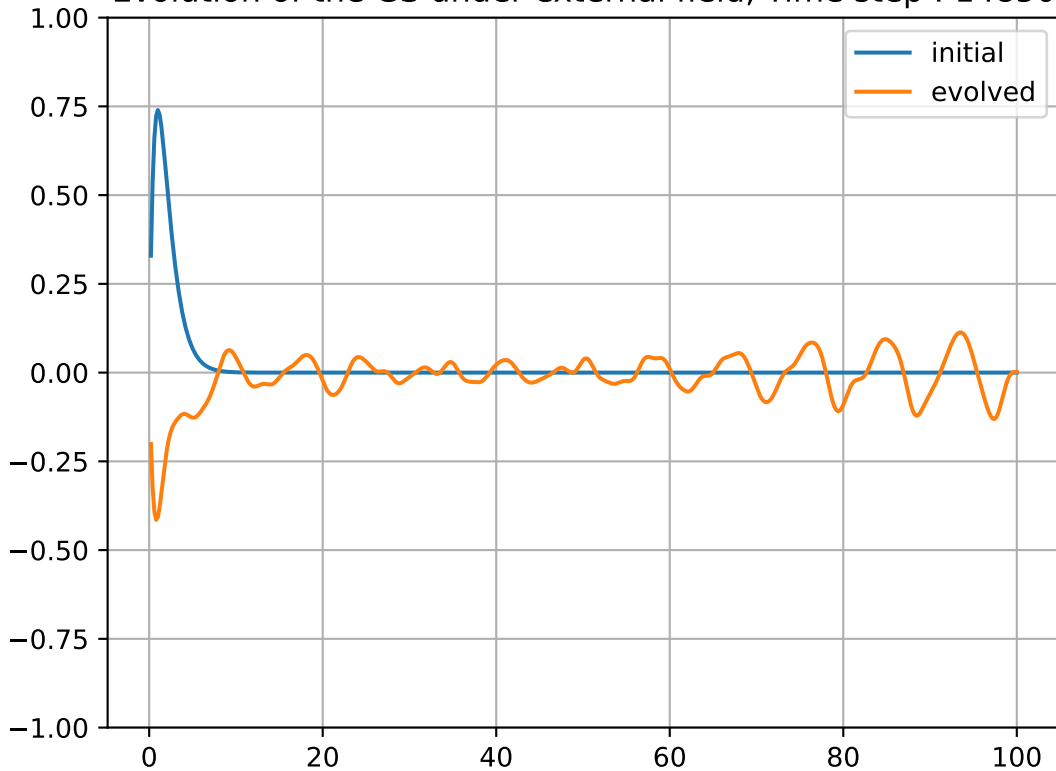
Evolution of the GS under external field, Time step : 14850
