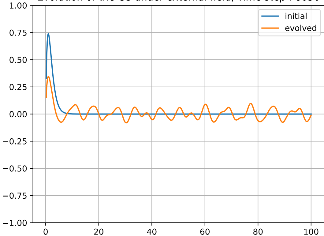
Evolution of the GS under external field, Time step : 8050
