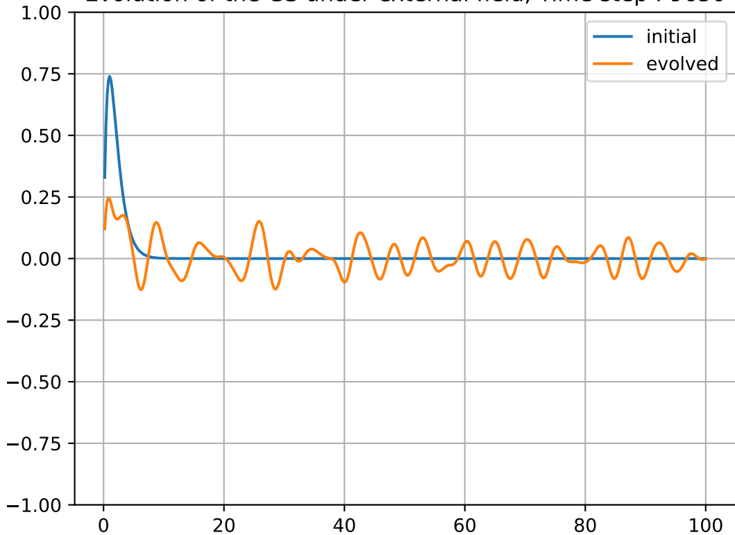
Evolution of the GS under external field, Time step : 9650
