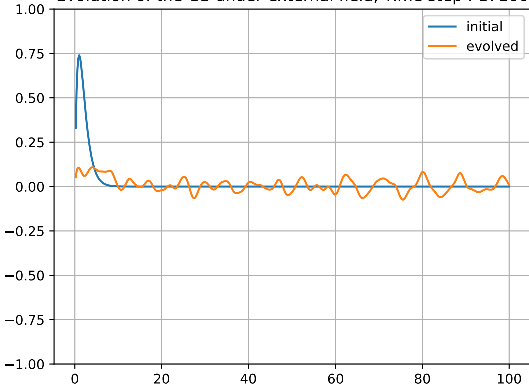
Evolution of the GS under external field, Time step : 17100
