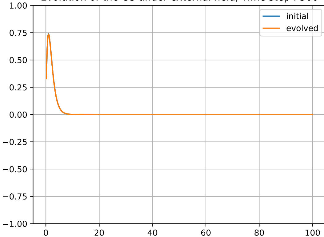
Evolution of the GS under external field, Time step : 500
