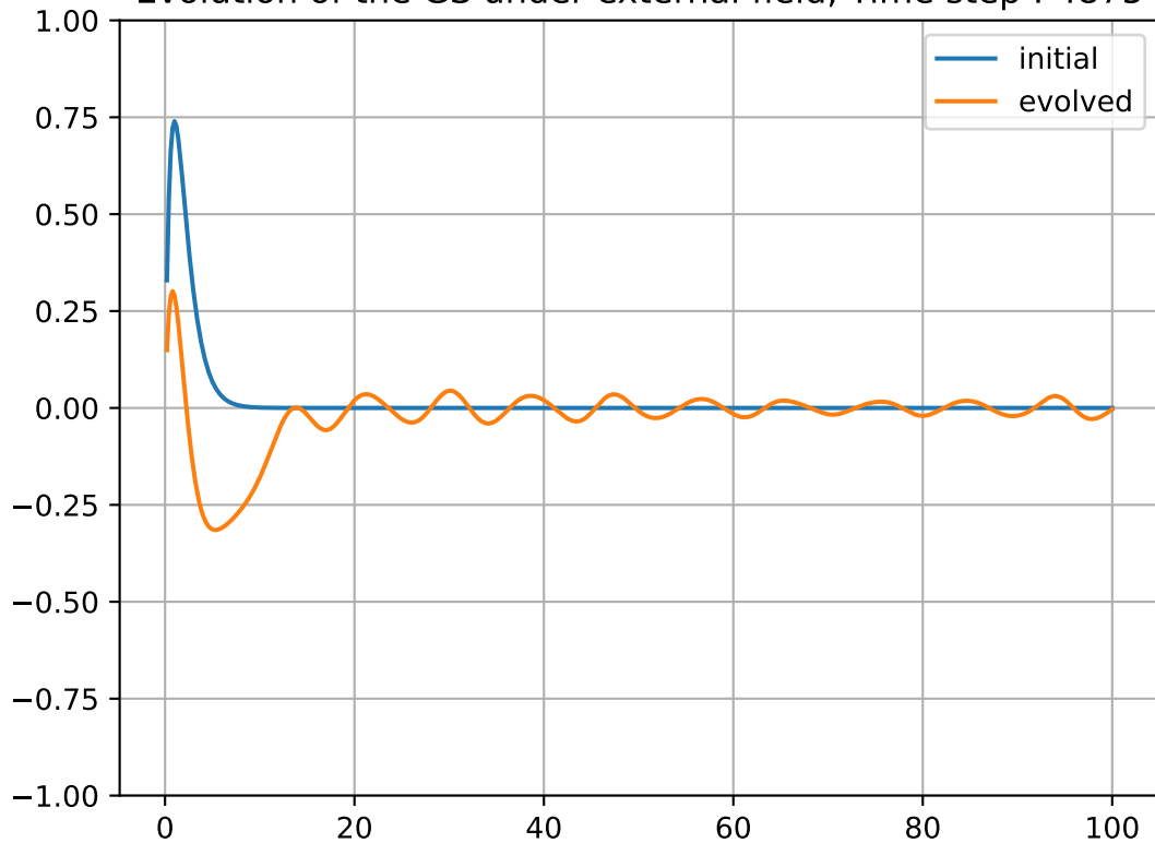
Evolution of the GS under external field, Time step : 4875
