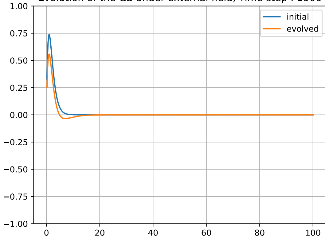
Evolution of the GS under external field, Time step : 1900
