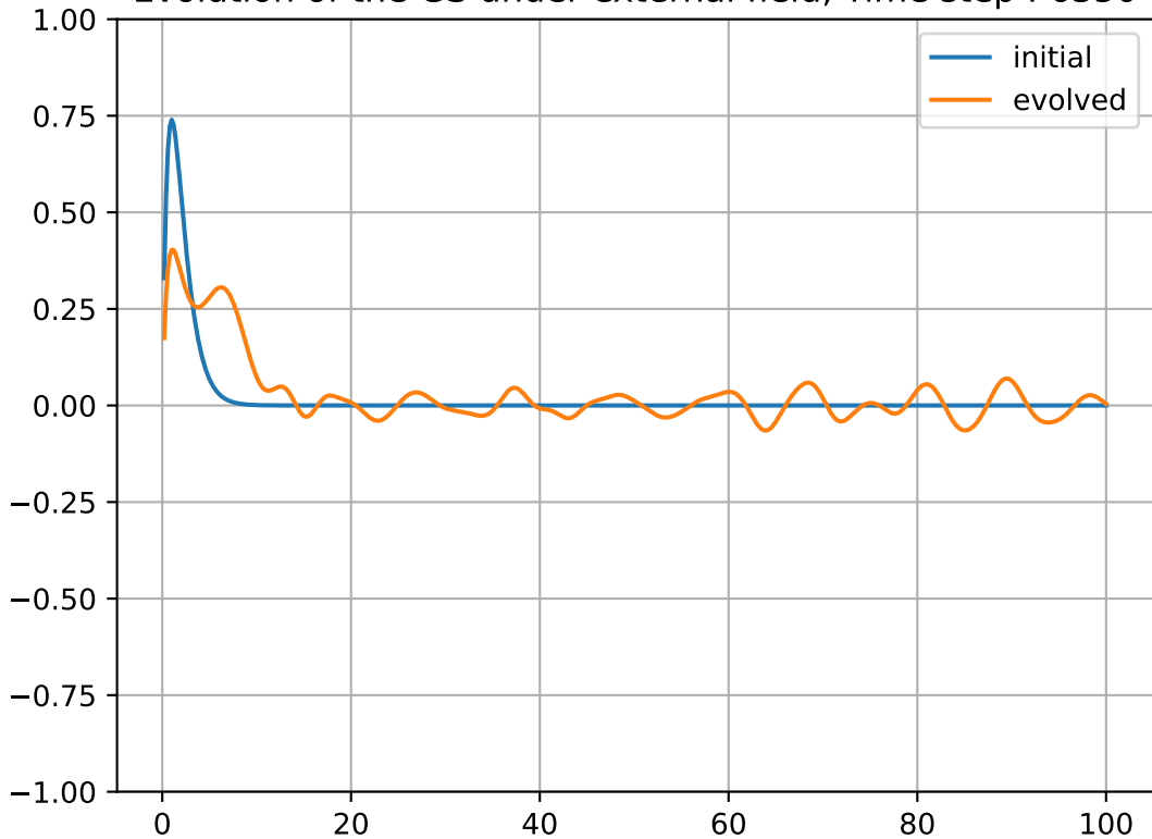
Evolution of the GS under external field, Time step : 6350
