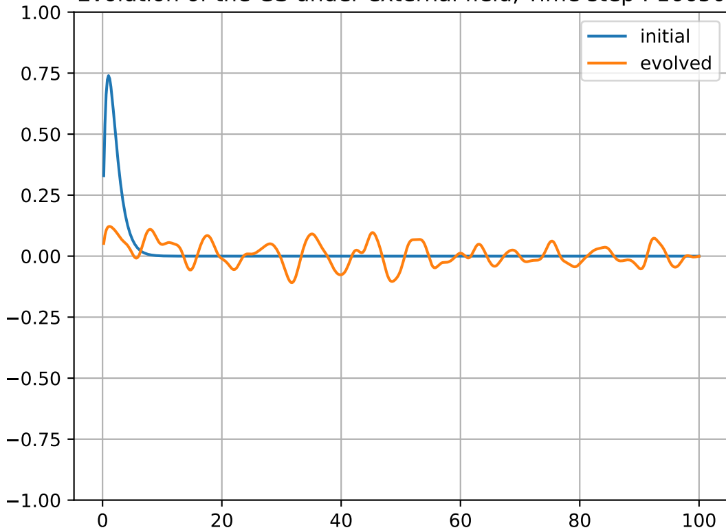
Evolution of the GS under external field, Time step : 16650
