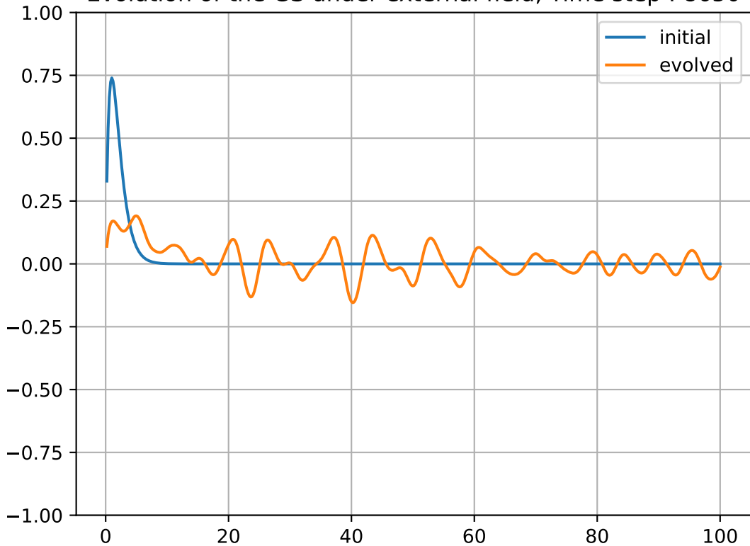
Evolution of the GS under external field, Time step : 8650
