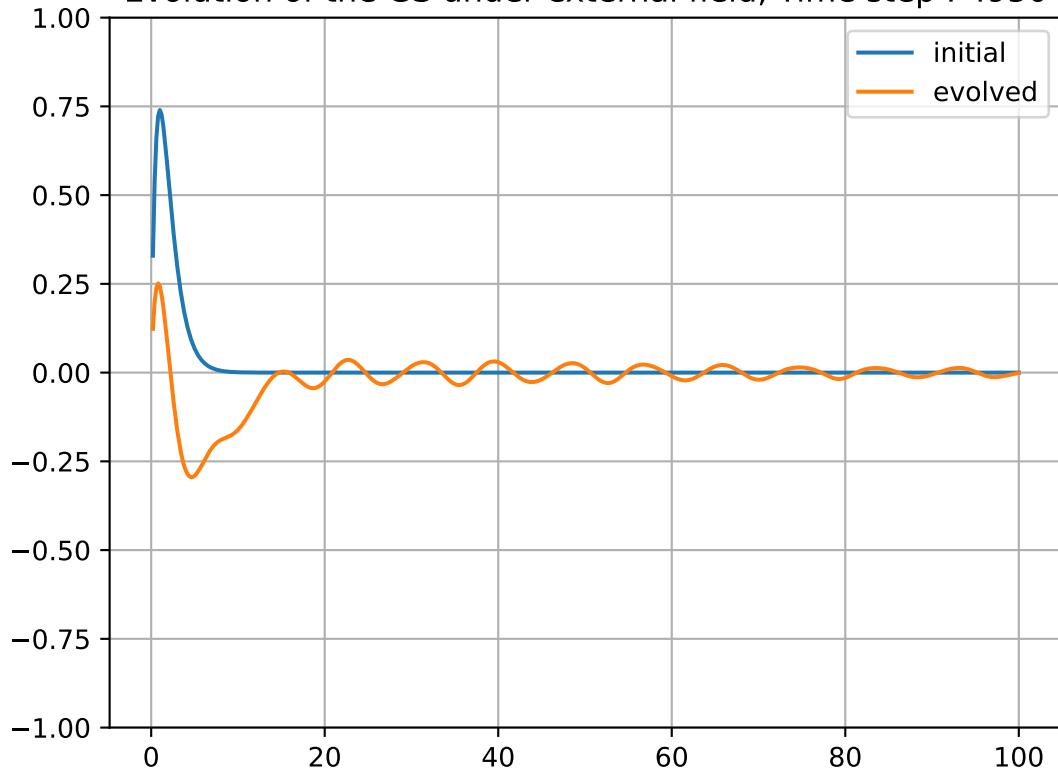
Evolution of the GS under external field, Time step : 4950
