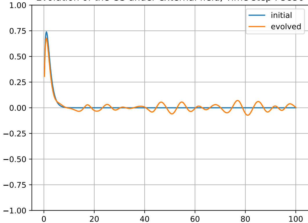
Evolution of the GS under external field, Time step : 5850
