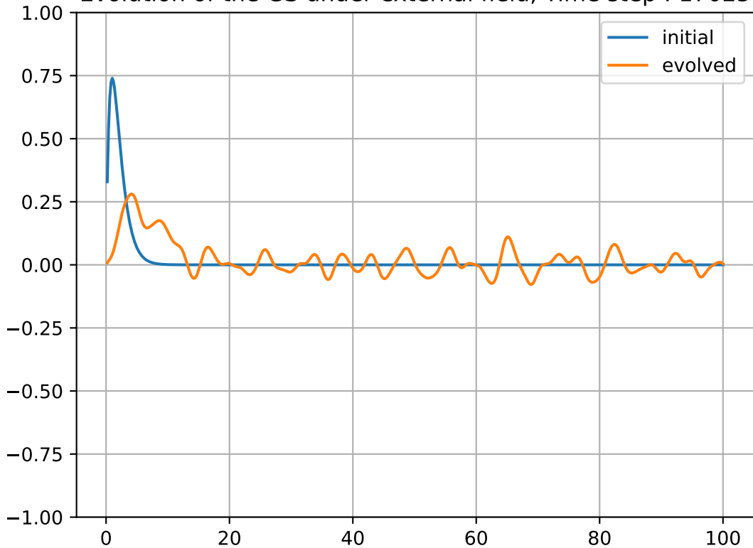
Evolution of the GS under external field, Time step : 17025
