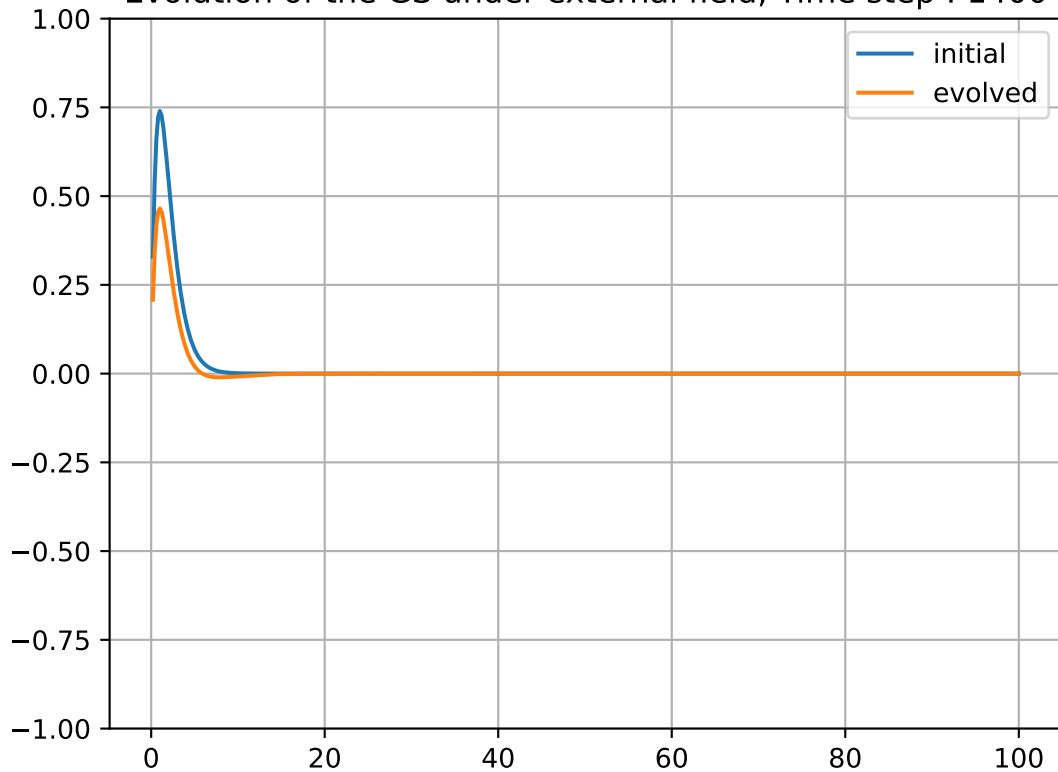
Evolution of the GS under external field, Time step : 1400
