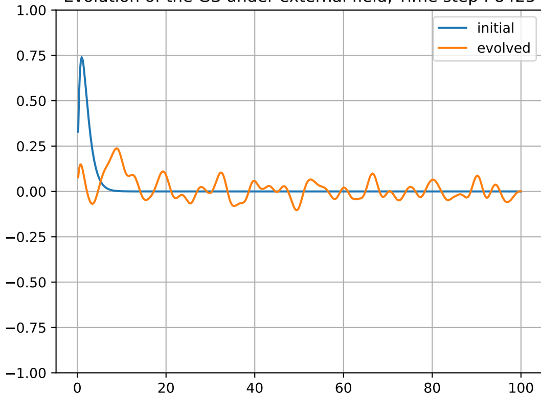
Evolution of the GS under external field, Time step : 8425
