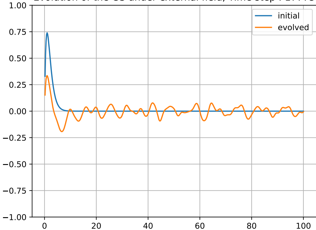
Evolution of the GS under external field, Time step : 17775
