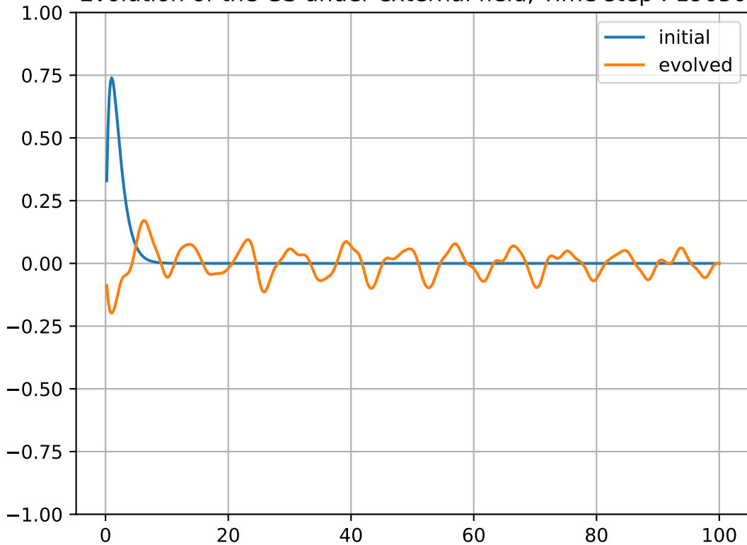
Evolution of the GS under external field, Time step : 19050
