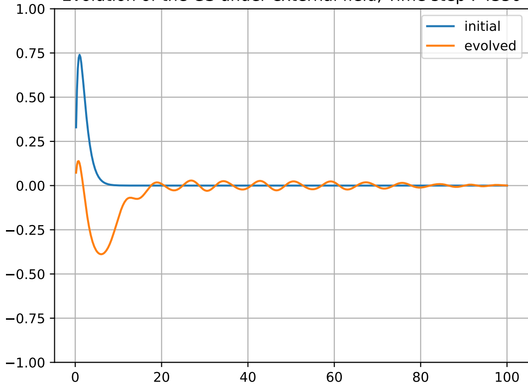
Evolution of the GS under external field, Time step : 4350
