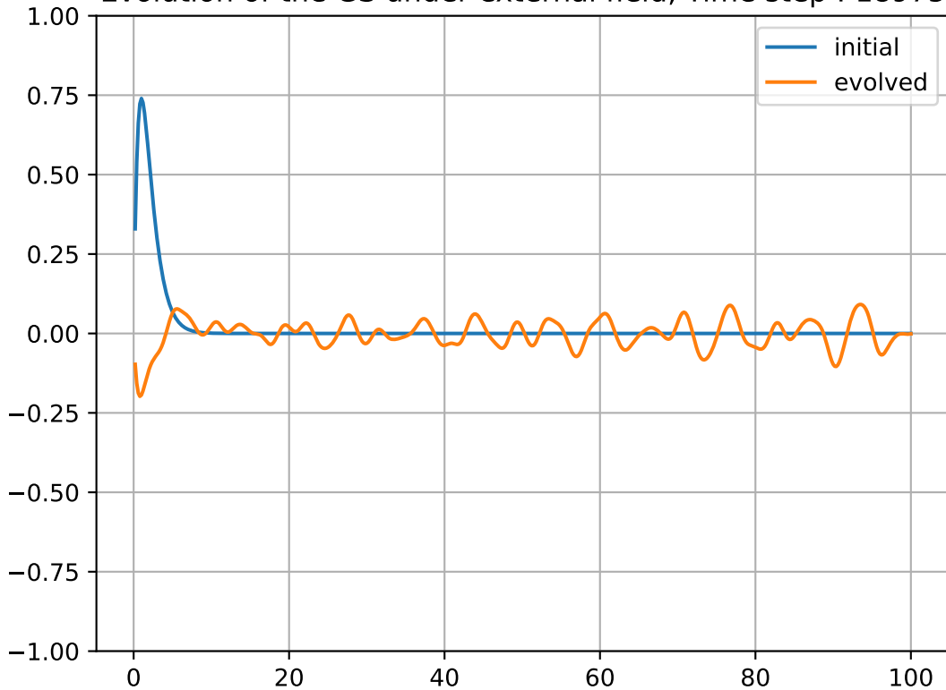
Evolution of the GS under external field, Time step : 18975
