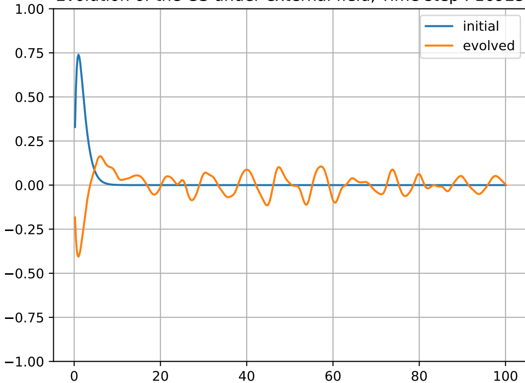
Evolution of the GS under external field, Time step : 16925
