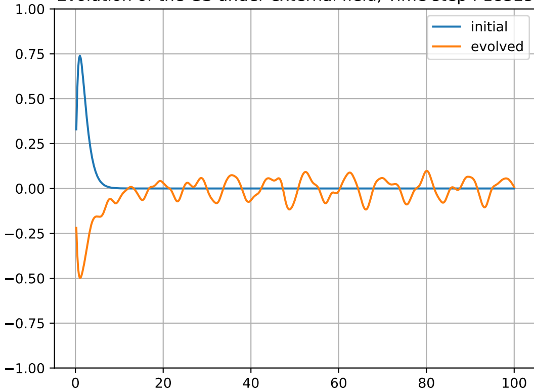
Evolution of the GS under external field, Time step : 18325
