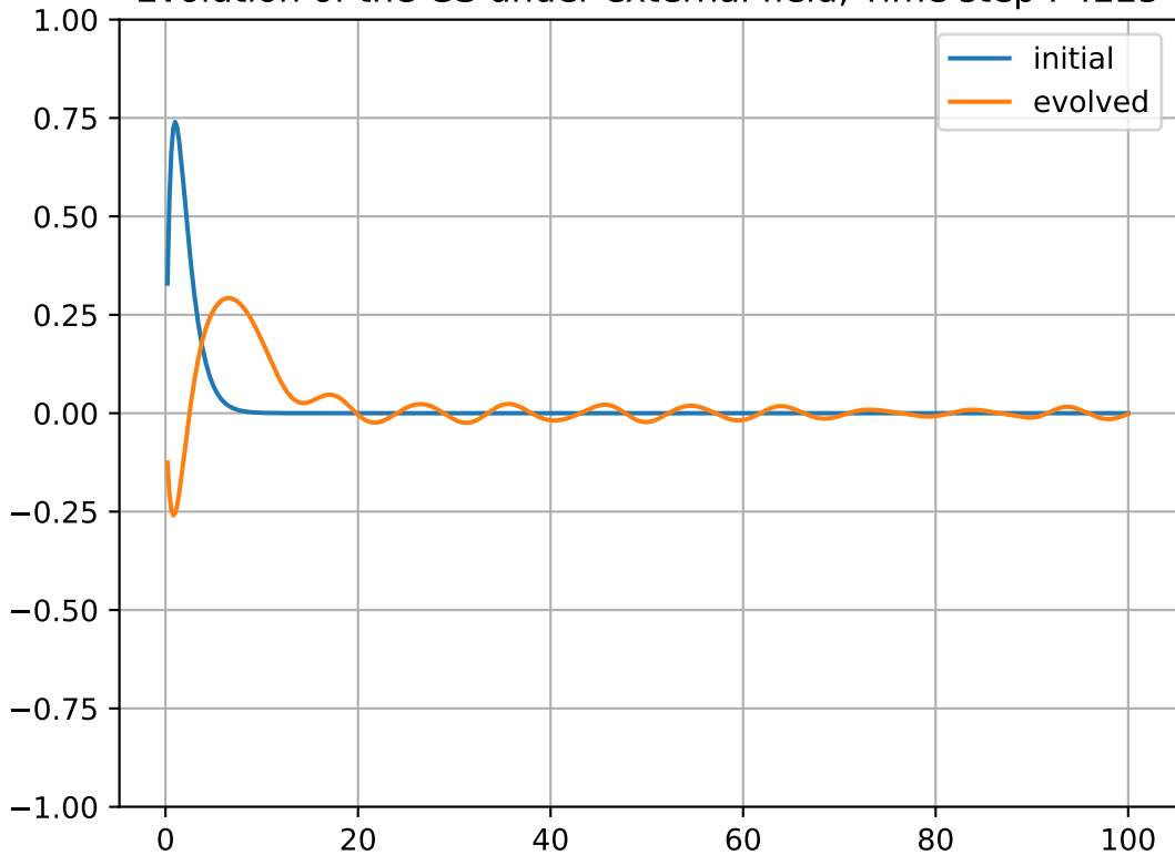
Evolution of the GS under external field, Time step : 4225
