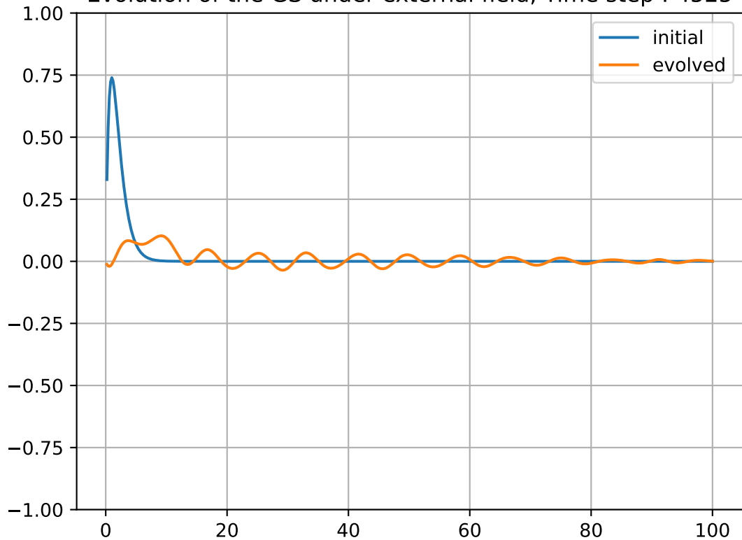
Evolution of the GS under external field, Time step : 4525
