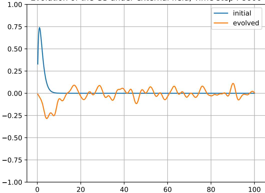
Evolution of the GS under external field, Time step : 8600
