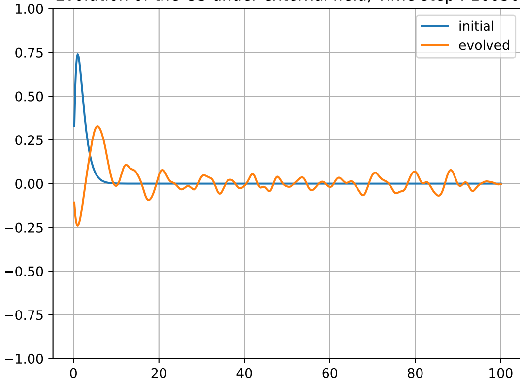
Evolution of the GS under external field, Time step : 16050
