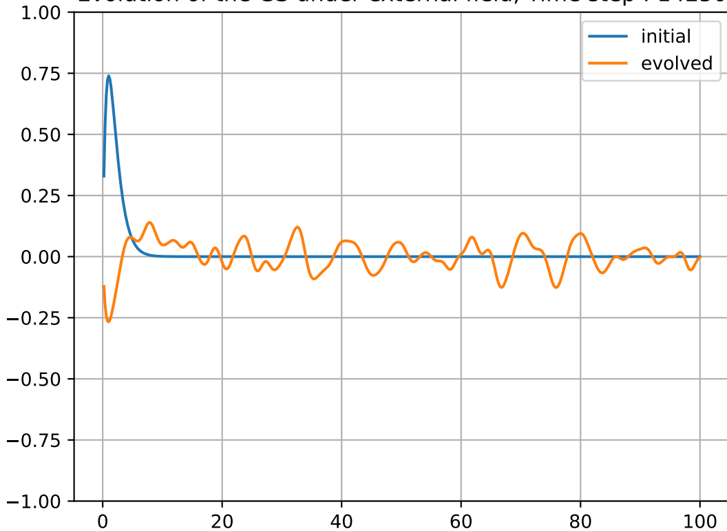
Evolution of the GS under external field, Time step : 14250
