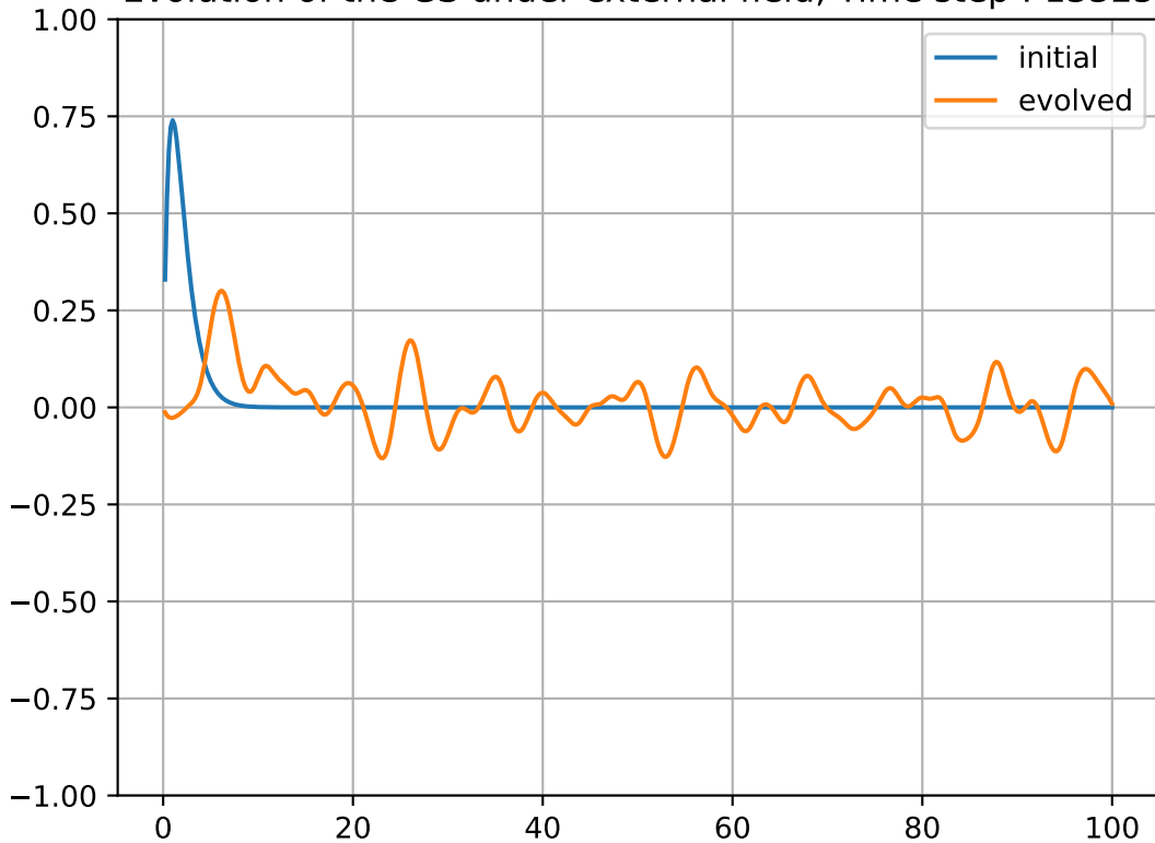
Evolution of the GS under external field, Time step : 13325
