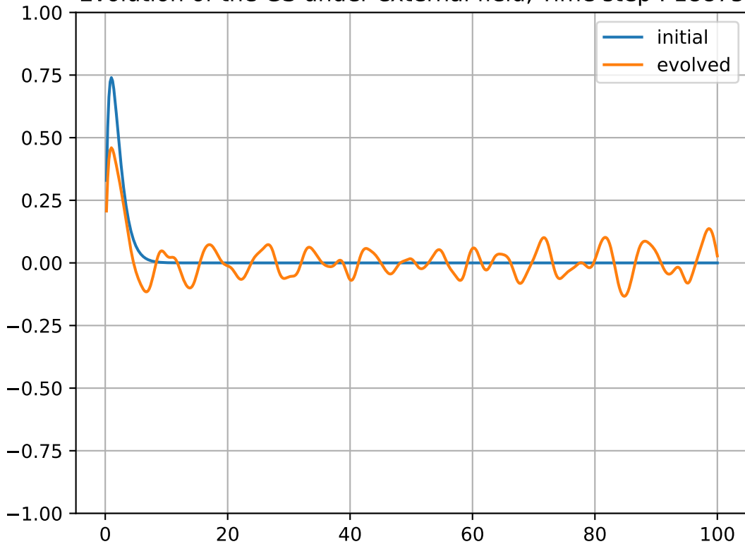
Evolution of the GS under external field, Time step : 18875
