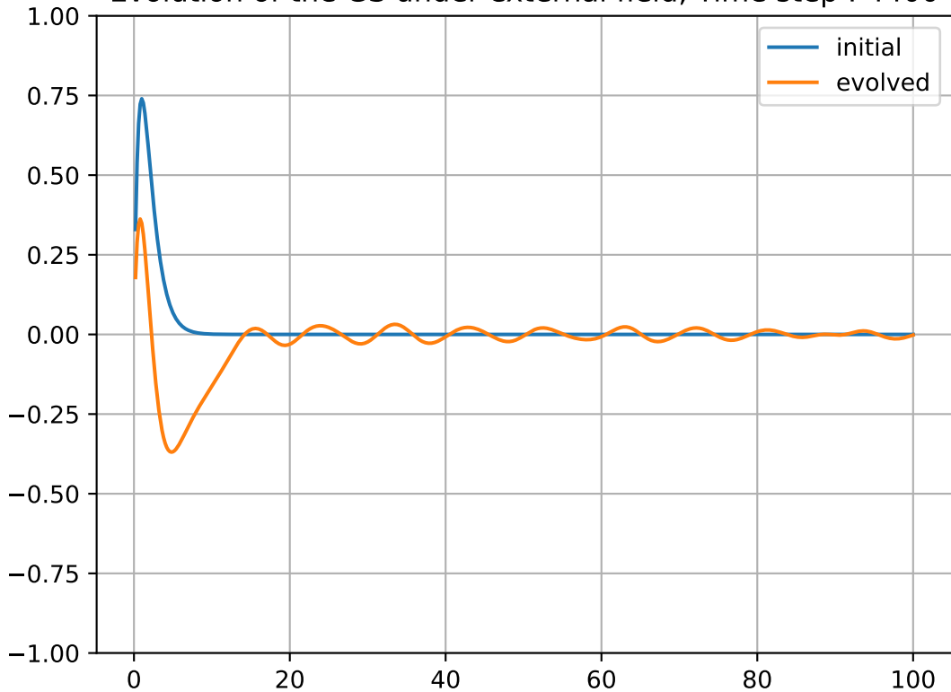
Evolution of the GS under external field, Time step : 4400
