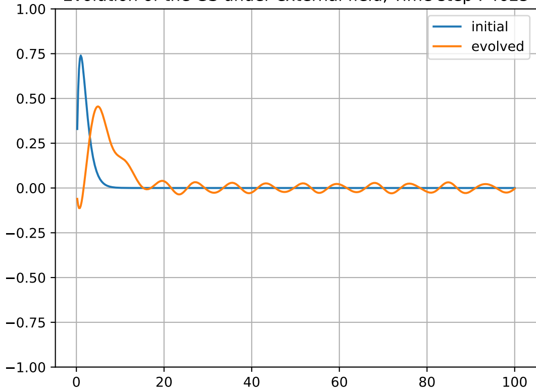
Evolution of the GS under external field, Time step : 4625
