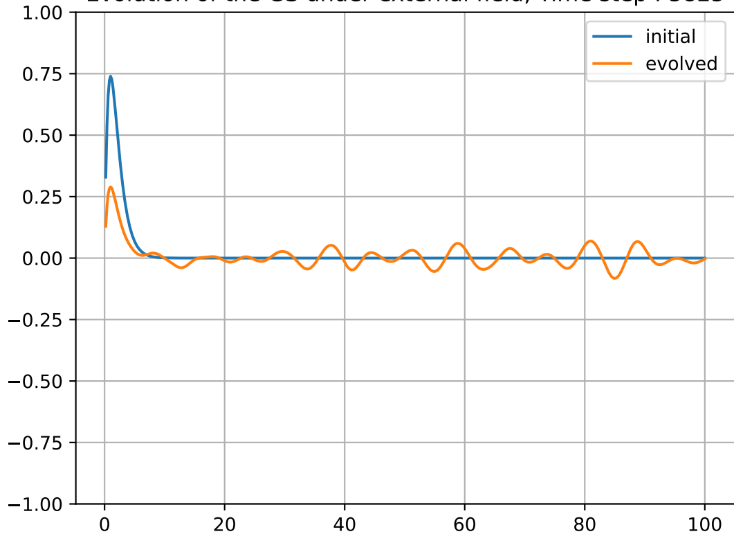
Evolution of the GS under external field, Time step : 5825
