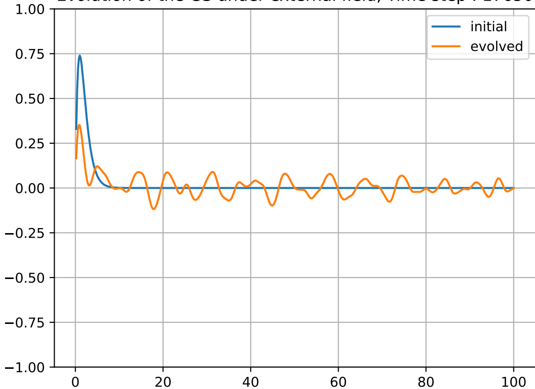
Evolution of the GS under external field, Time step : 17650
