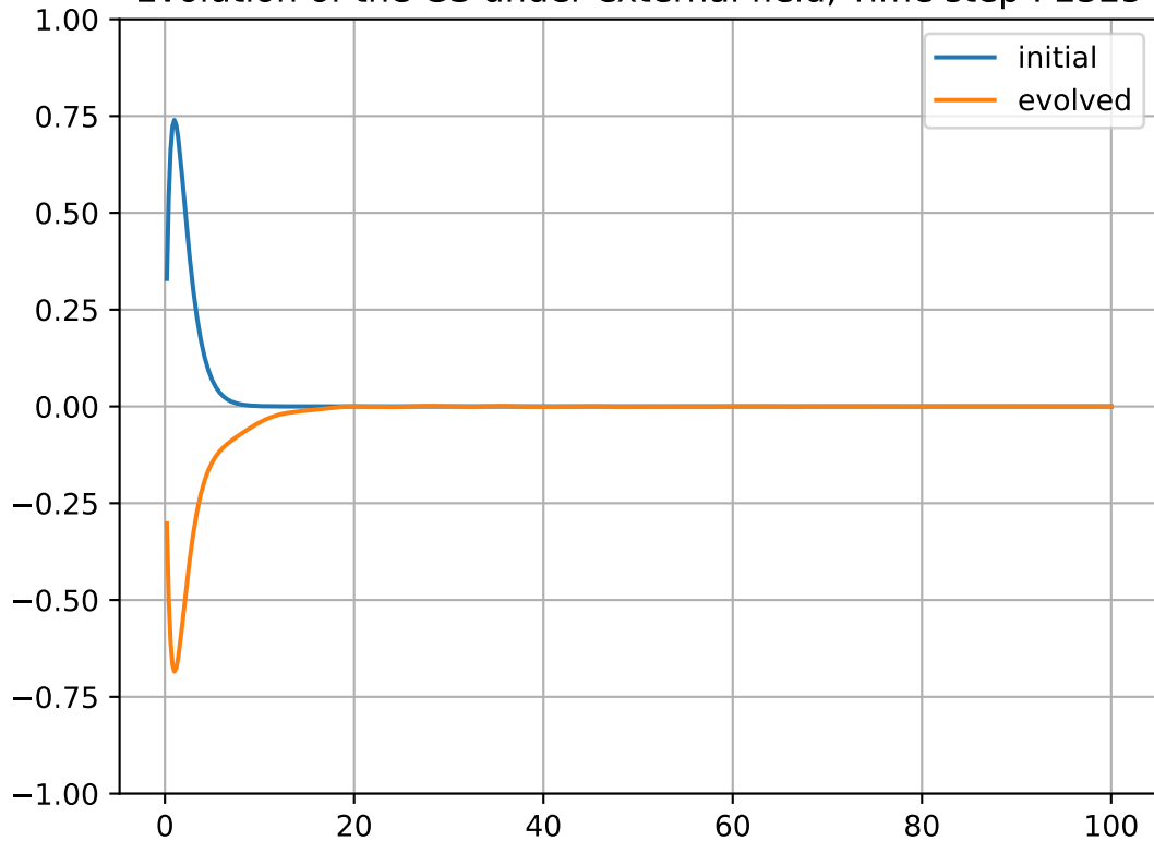
Evolution of the GS under external field, Time step : 2325
