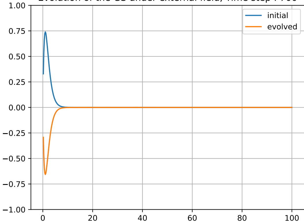
Evolution of the GS under external field, Time step : 700
