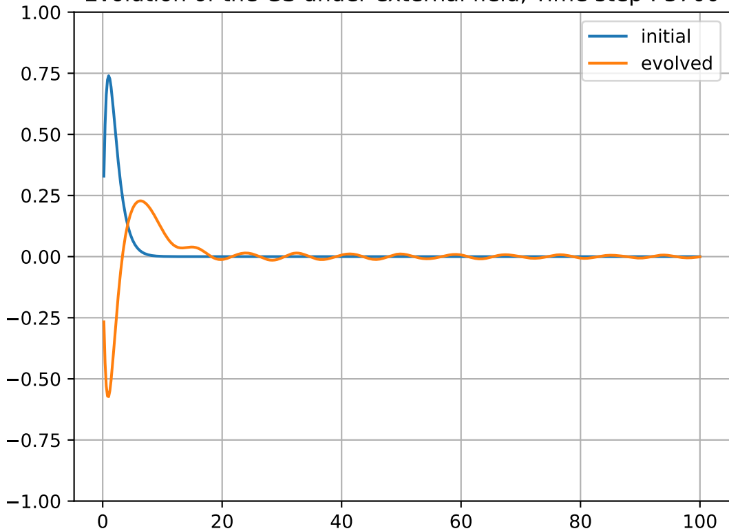
Evolution of the GS under external field, Time step : 3700
