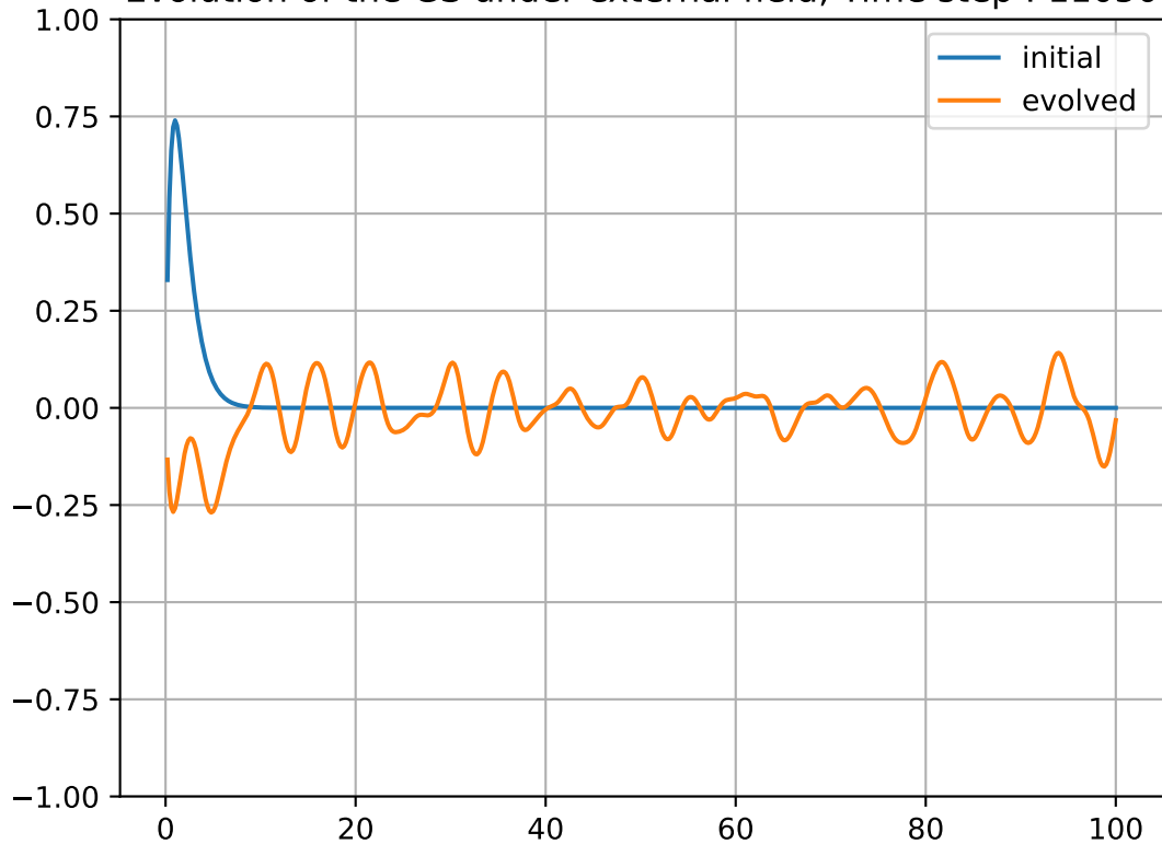
Evolution of the GS under external field, Time step : 11050
