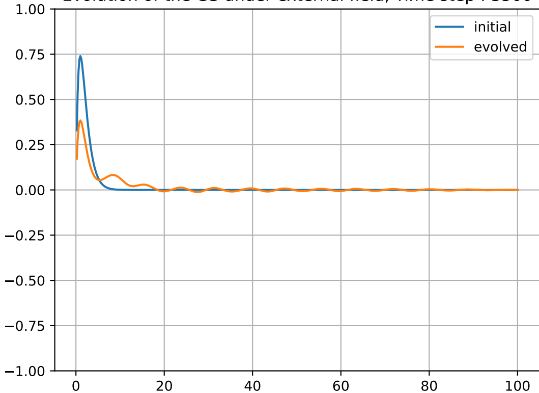
Evolution of the GS under external field, Time step : 3500
