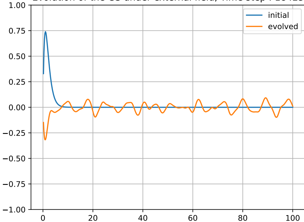
Evolution of the GS under external field, Time step : 18425
