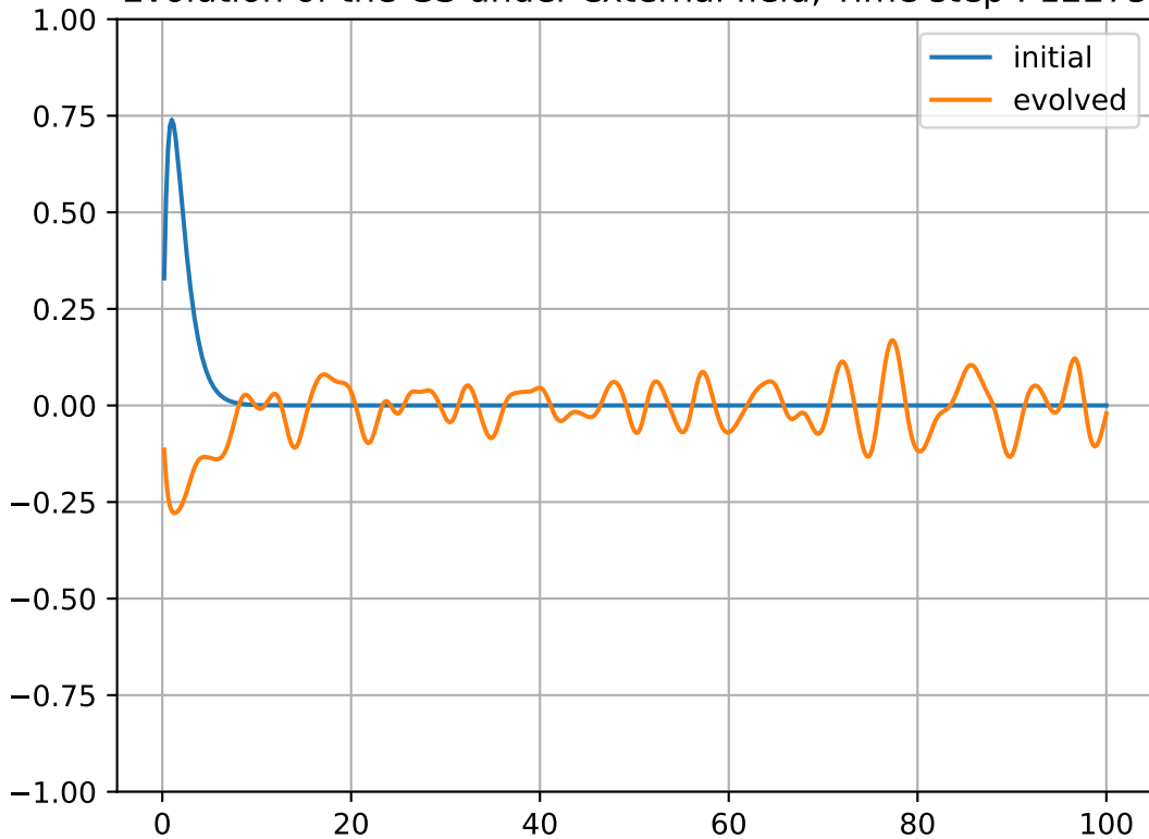
Evolution of the GS under external field, Time step : 12275
