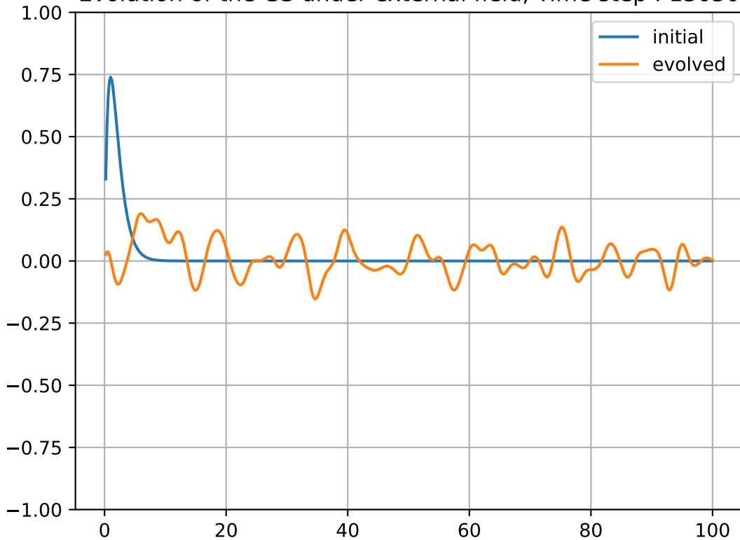
Evolution of the GS under external field, Time step : 13050
