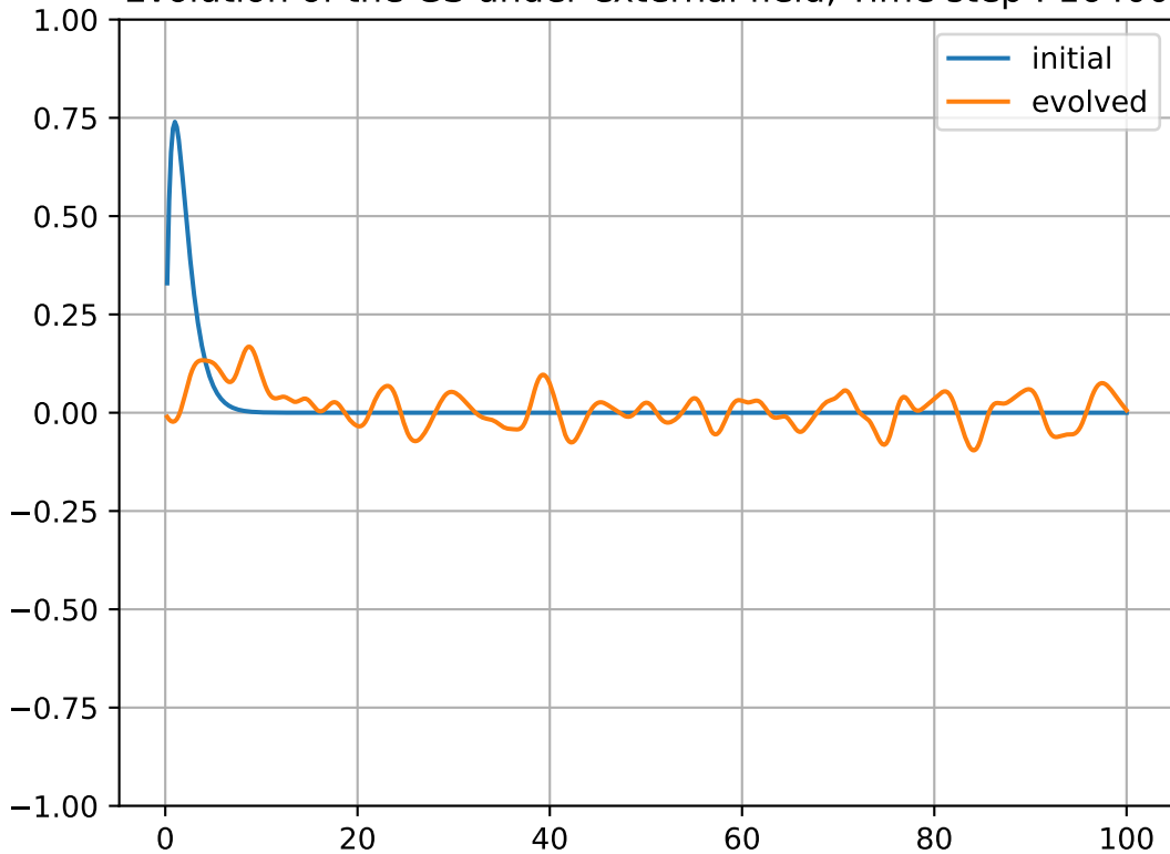
Evolution of the GS under external field, Time step : 16400
