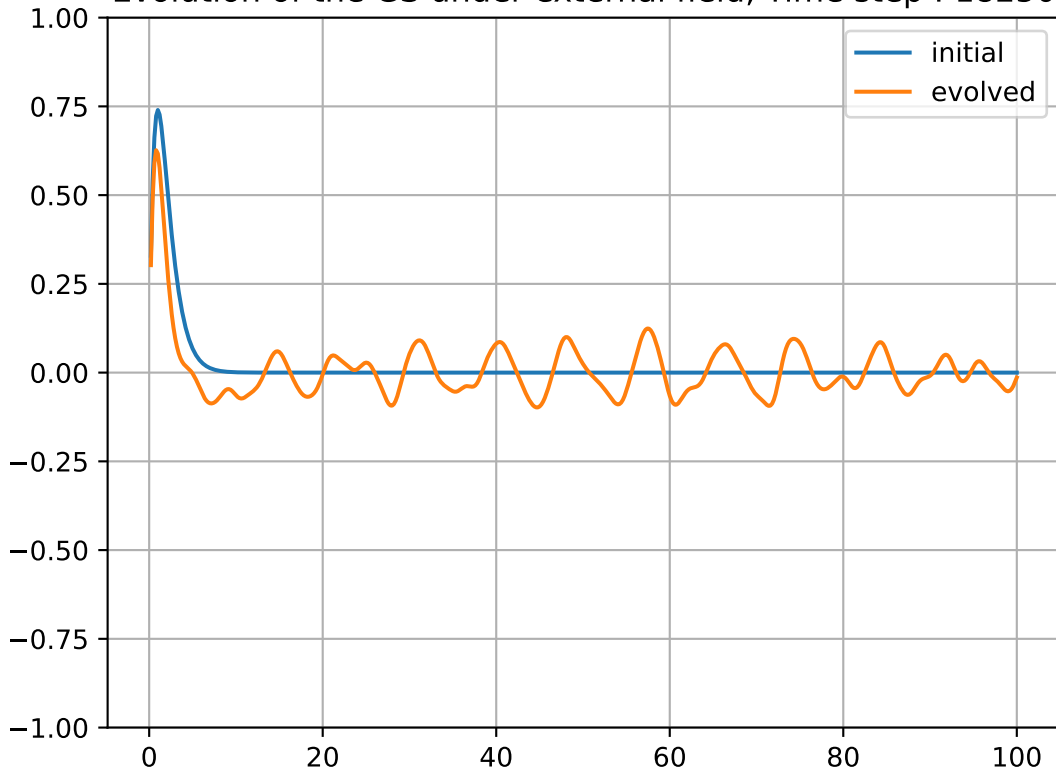
Evolution of the GS under external field, Time step : 18250
