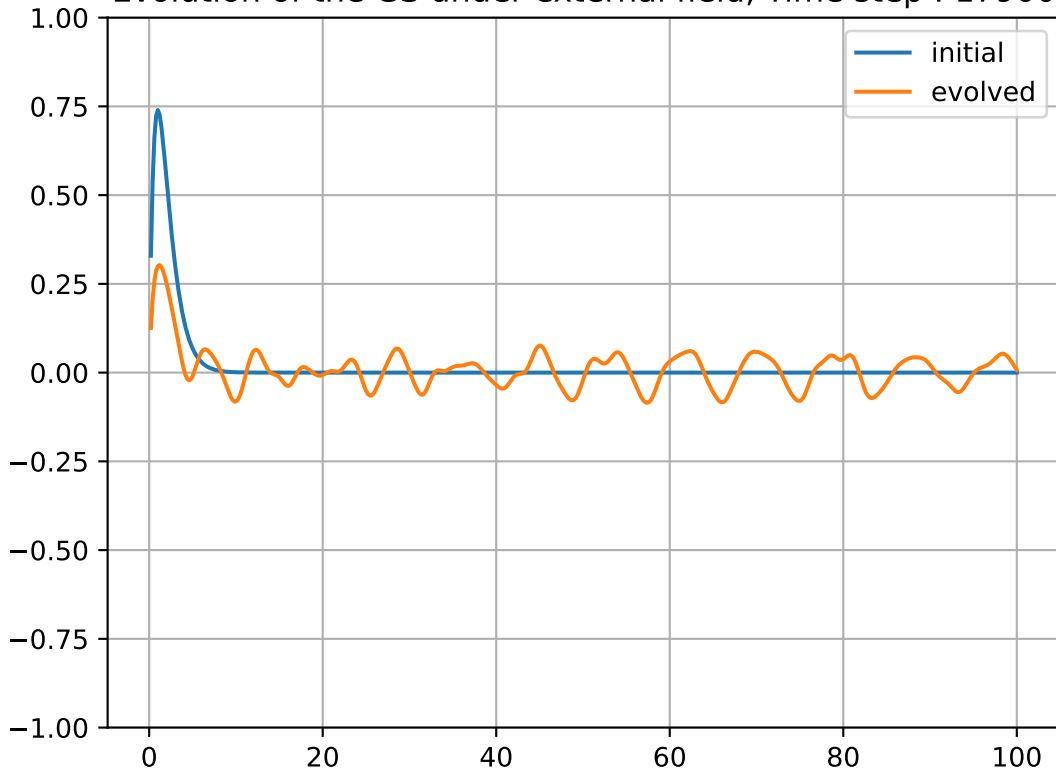
Evolution of the GS under external field, Time step : 17900
