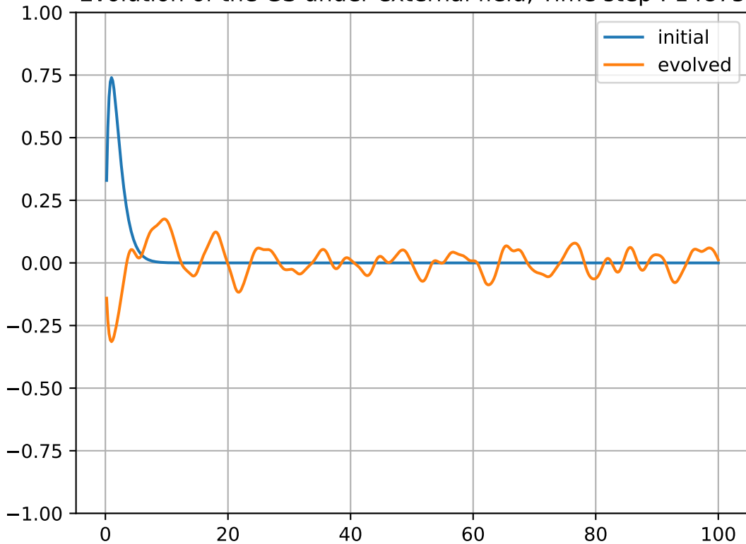
Evolution of the GS under external field, Time step : 14875
