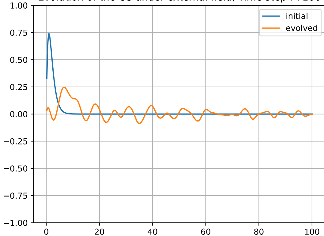
Evolution of the GS under external field, Time step : 7100
