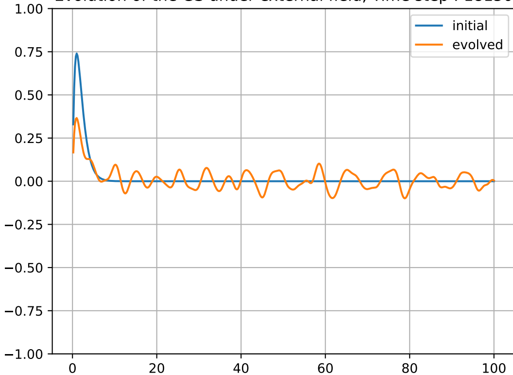
Evolution of the GS under external field, Time step : 18150
