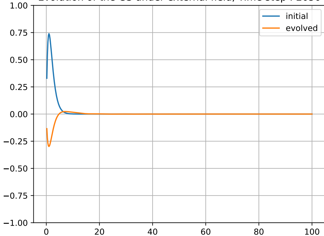
Evolution of the GS under external field, Time step : 2050
