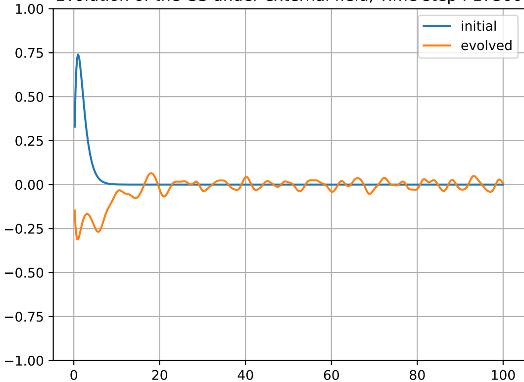
Evolution of the GS under external field, Time step : 17300
