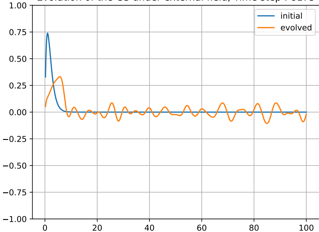
Evolution of the GS under external field, Time step : 8175
