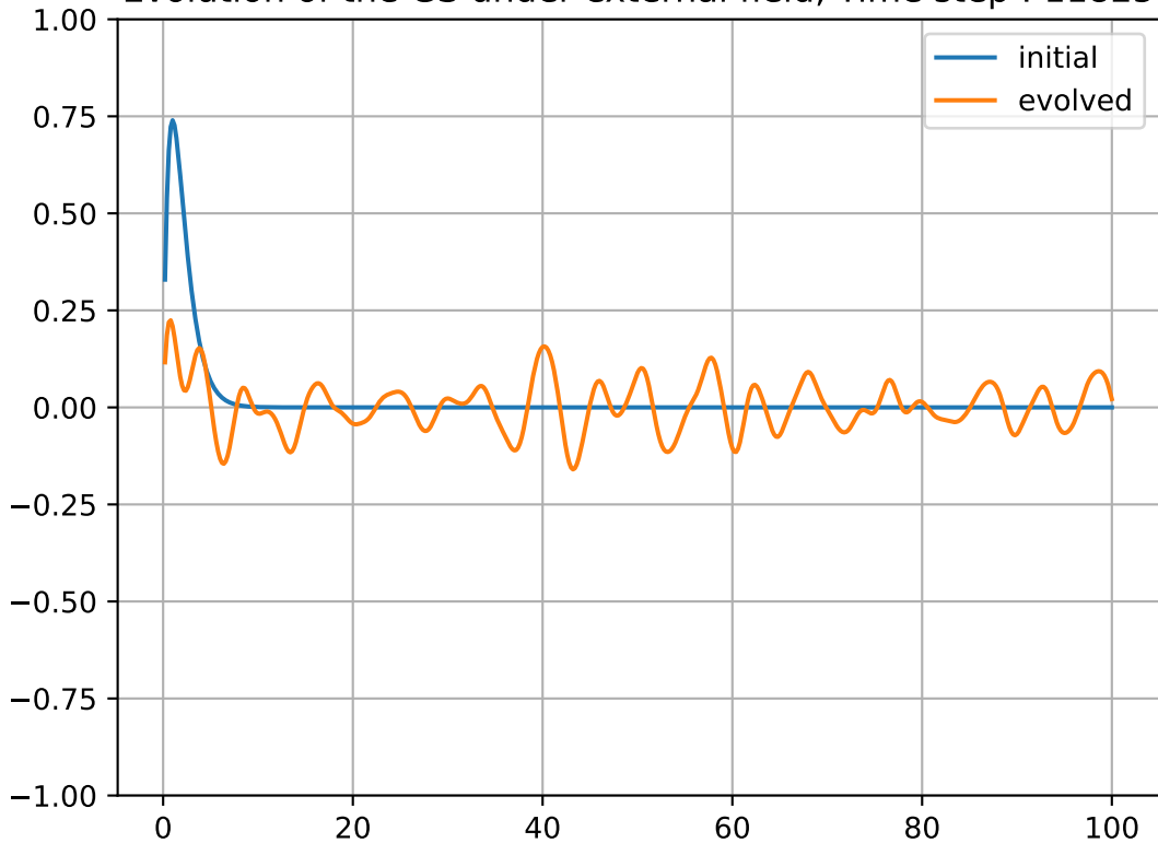
Evolution of the GS under external field, Time step : 11825
