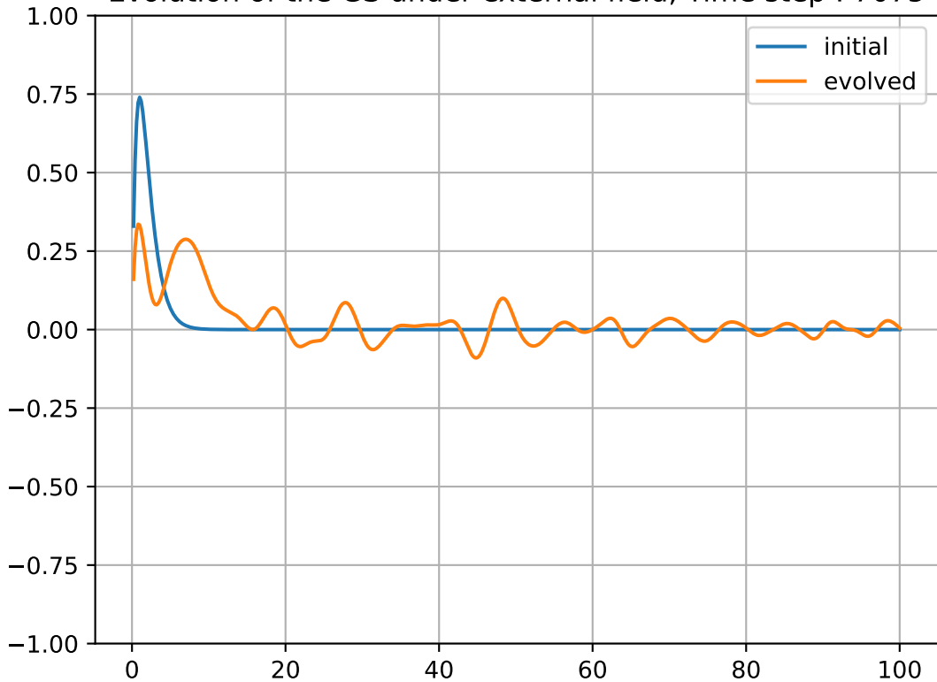
Evolution of the GS under external field, Time step : 7075
