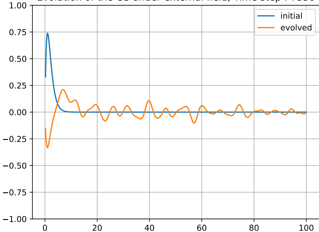
Evolution of the GS under external field, Time step : 7350
