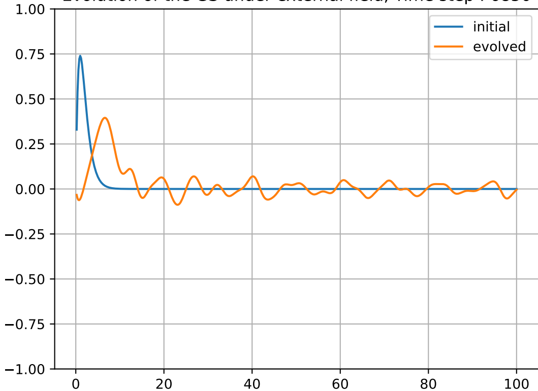
Evolution of the GS under external field, Time step : 6850
