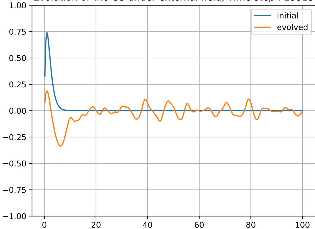
Evolution of the GS under external field, Time step : 15325
