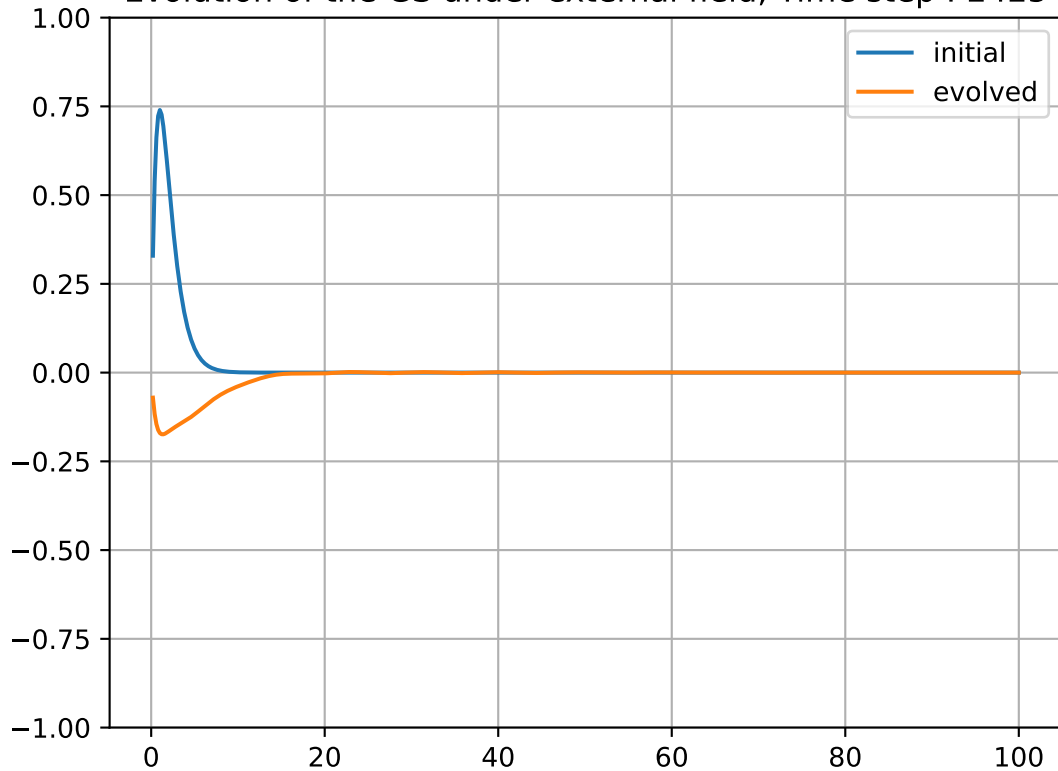
Evolution of the GS under external field, Time step : 2425
