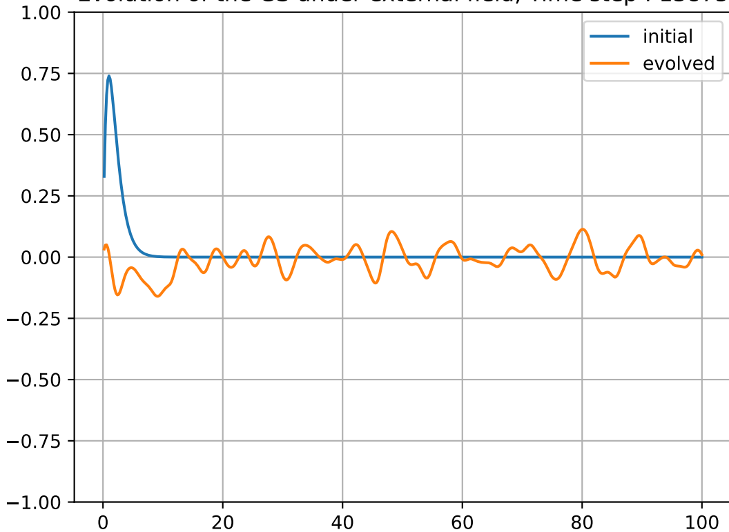
Evolution of the GS under external field, Time step : 13875
