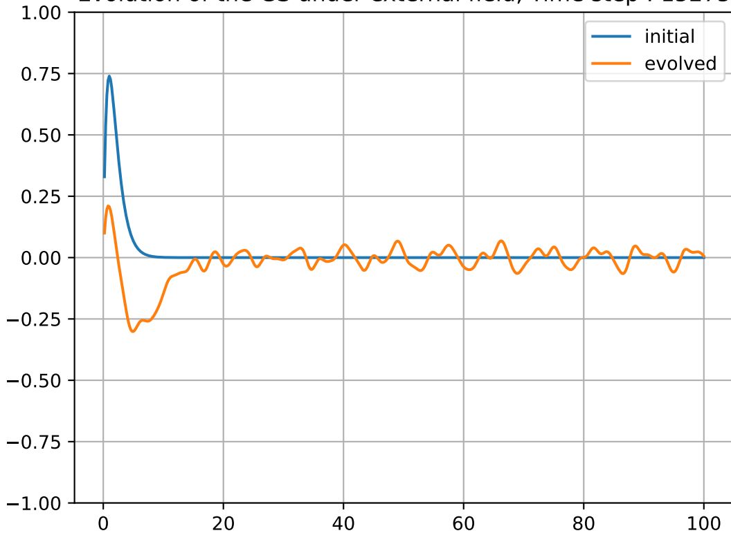
Evolution of the GS under external field, Time step : 15275
