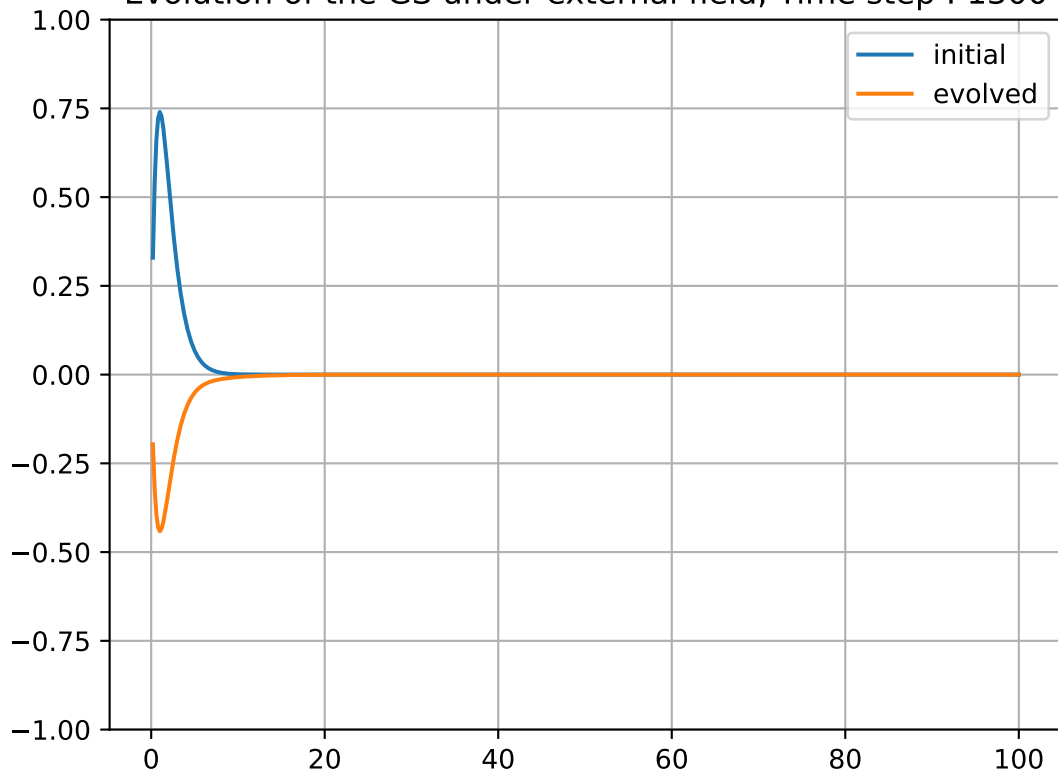
Evolution of the GS under external field, Time step : 1300
