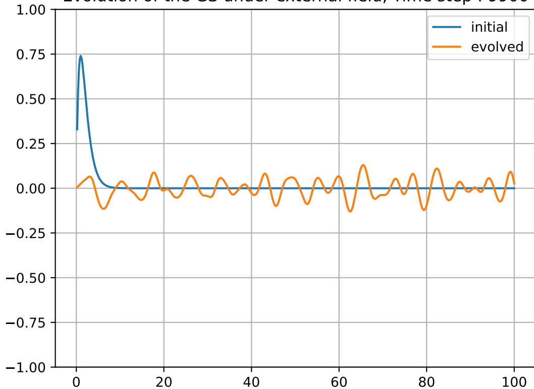
Evolution of the GS under external field, Time step : 9900
