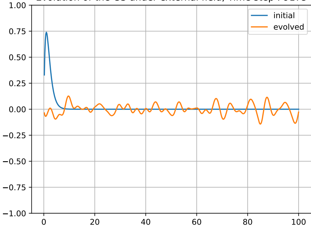
Evolution of the GS under external field, Time step : 9175
