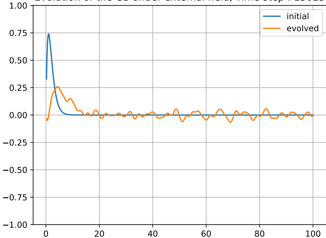
Evolution of the GS under external field, Time step : 15025
