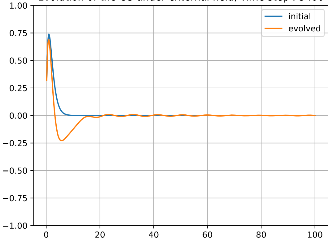
Evolution of the GS under external field, Time step : 3400
