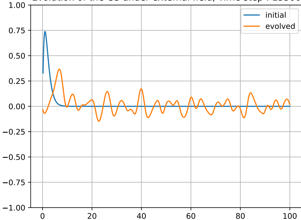
Evolution of the GS under external field, Time step : 13300
