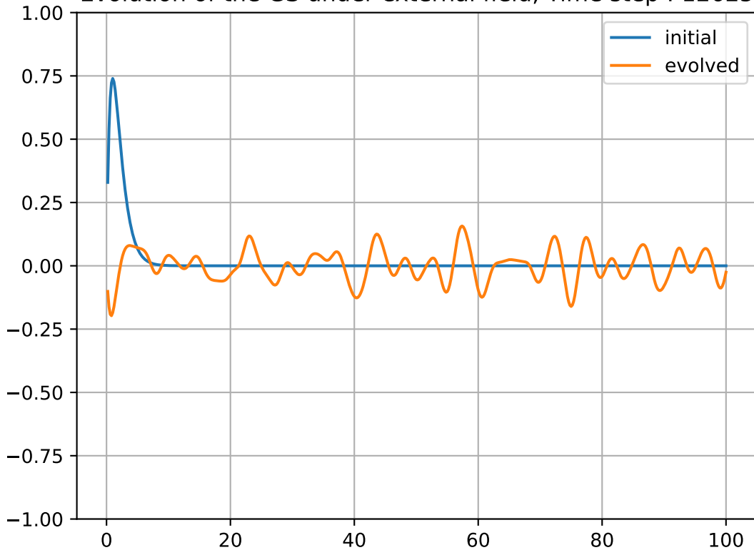
Evolution of the GS under external field, Time step : 12625
