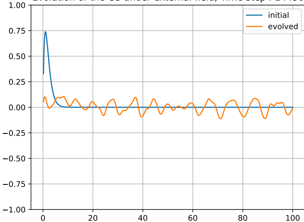
Evolution of the GS under external field, Time step : 14450
