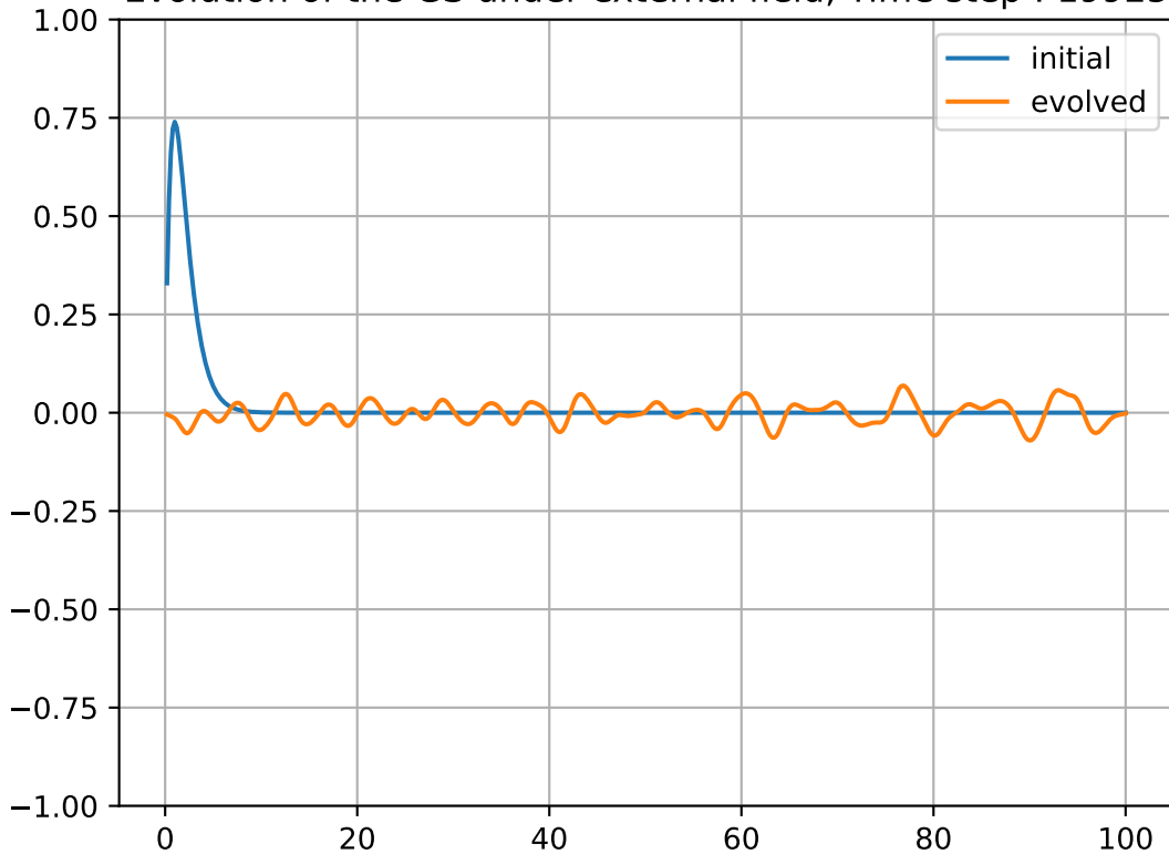
Evolution of the GS under external field, Time step : 19925
