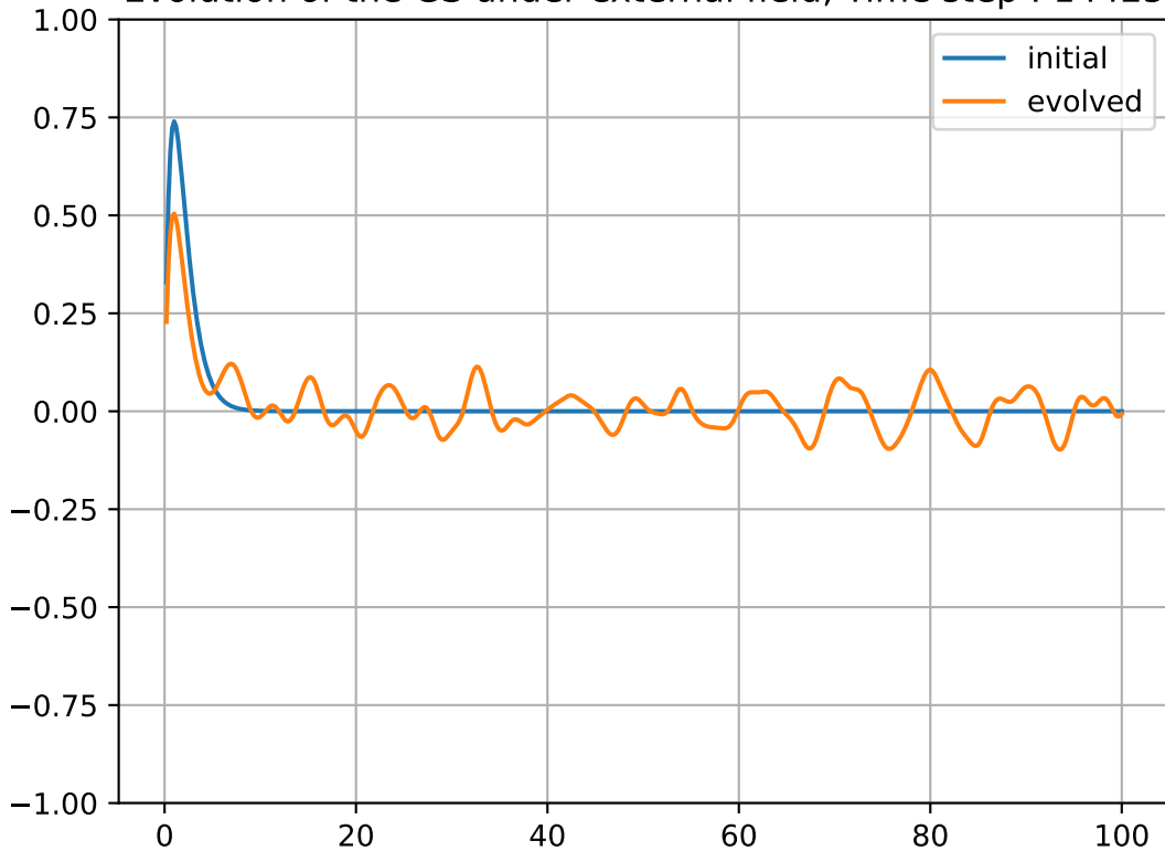
Evolution of the GS under external field, Time step : 14425
