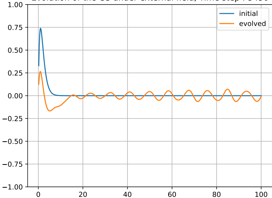
Evolution of the GS under external field, Time step : 5450
