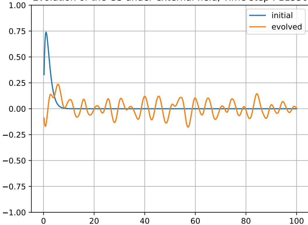
Evolution of the GS under external field, Time step : 11350
