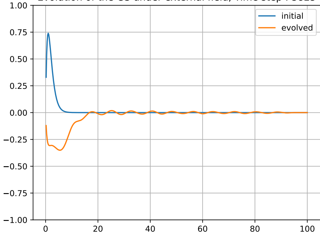
Evolution of the GS under external field, Time step : 3825
