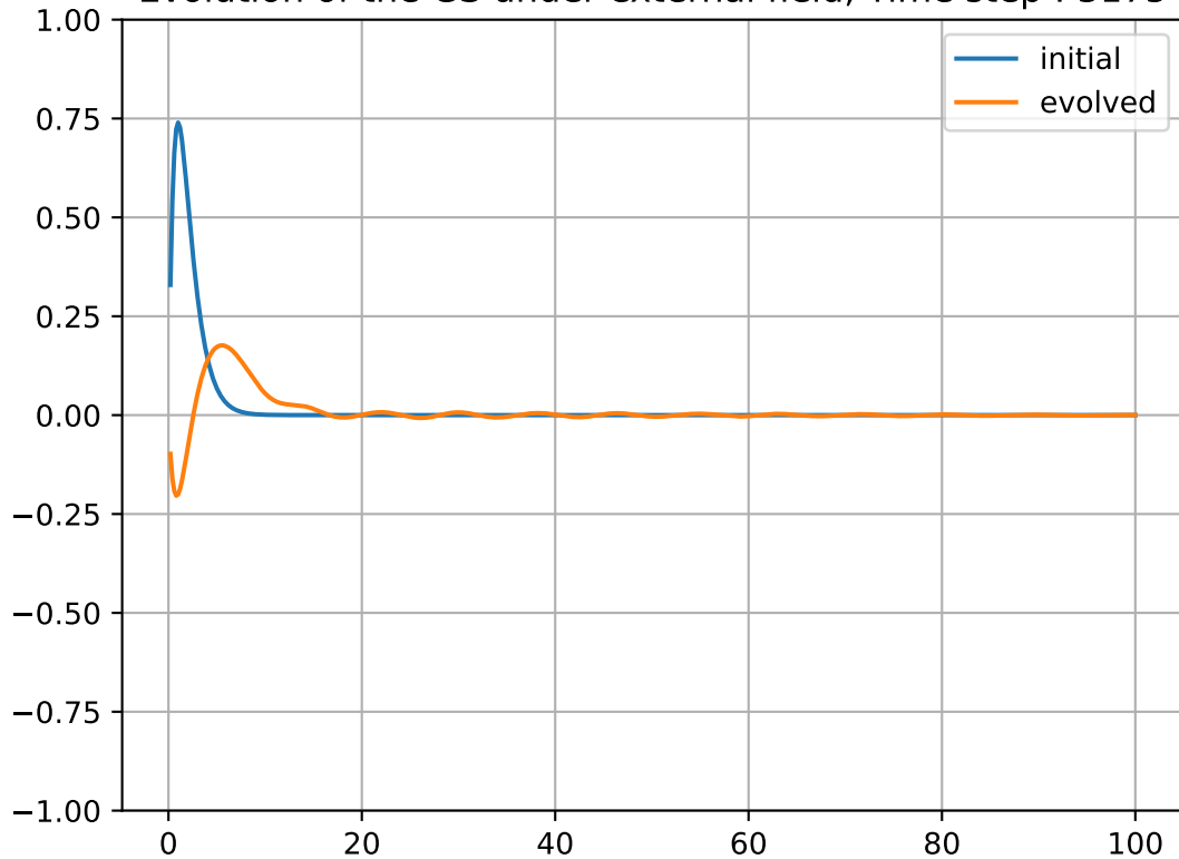
Evolution of the GS under external field, Time step : 3175
