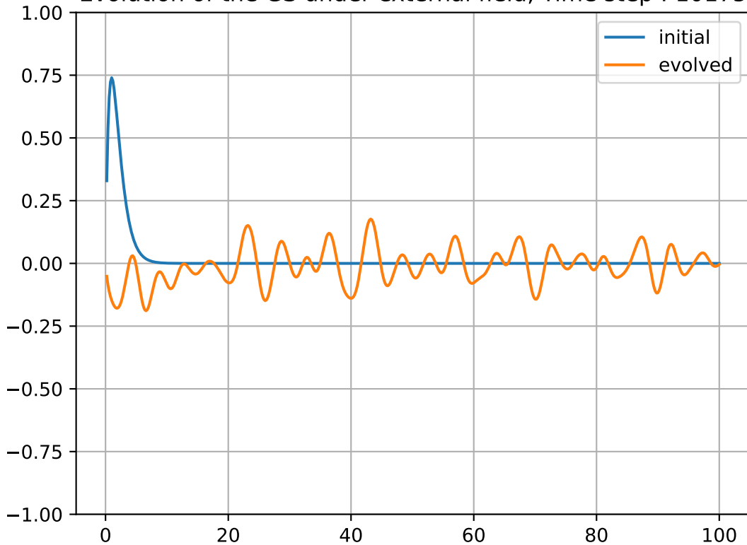
Evolution of the GS under external field, Time step : 10175
