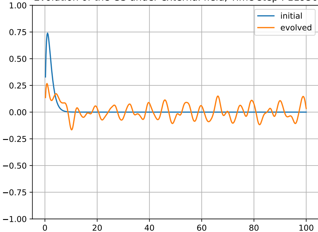
Evolution of the GS under external field, Time step : 11950
