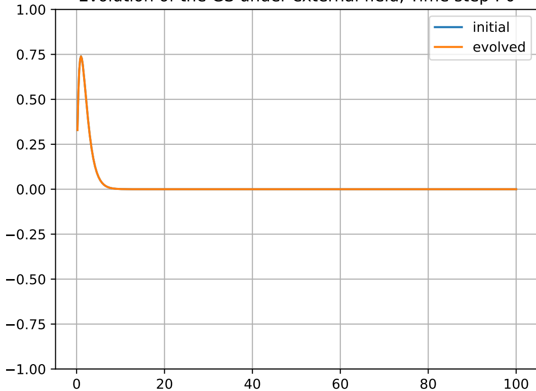
Evolution of the GS under external field, Time step : 0
