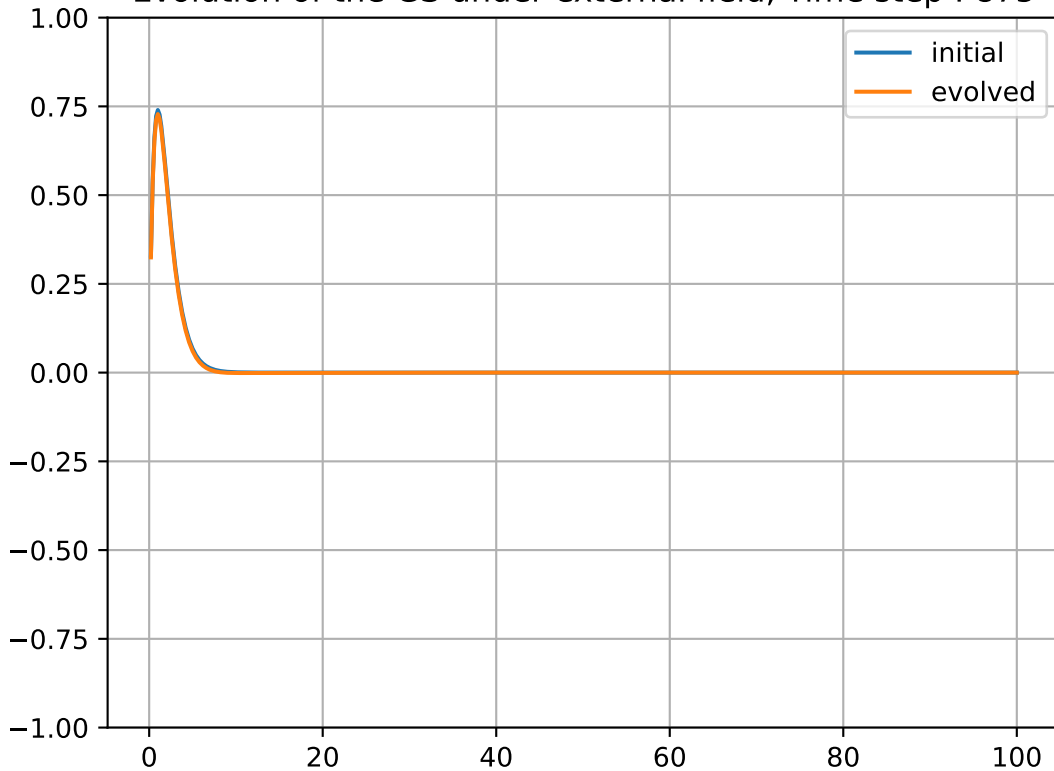
Evolution of the GS under external field, Time step : 875
