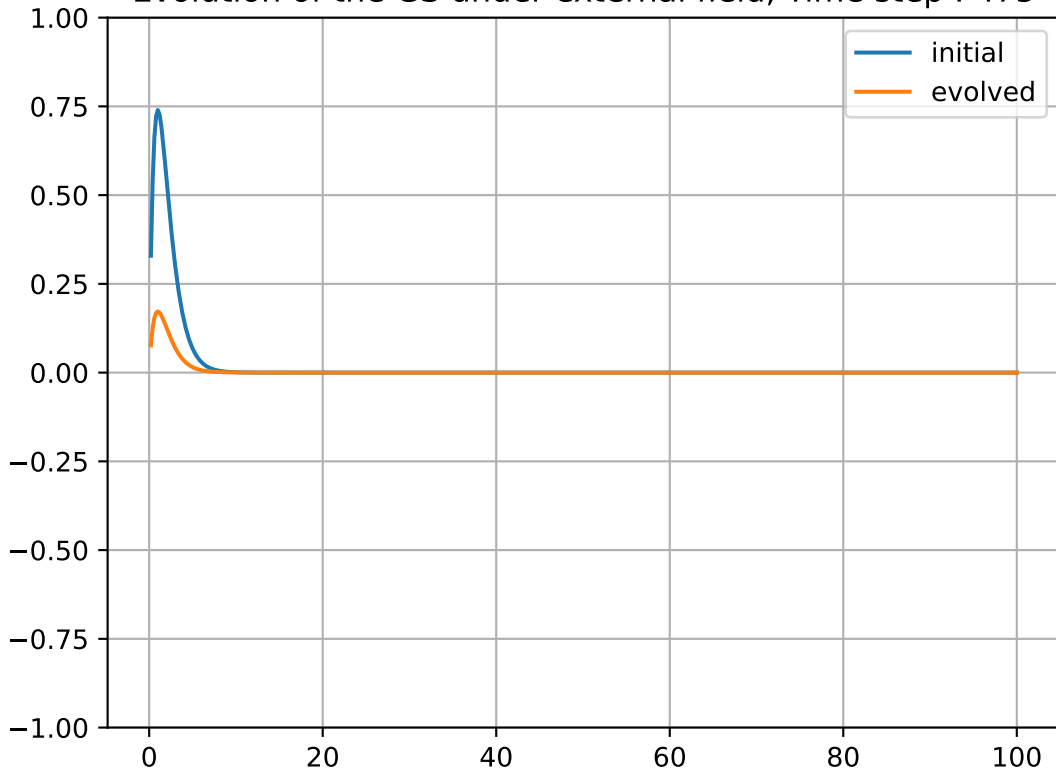
Evolution of the GS under external field, Time step : 475
