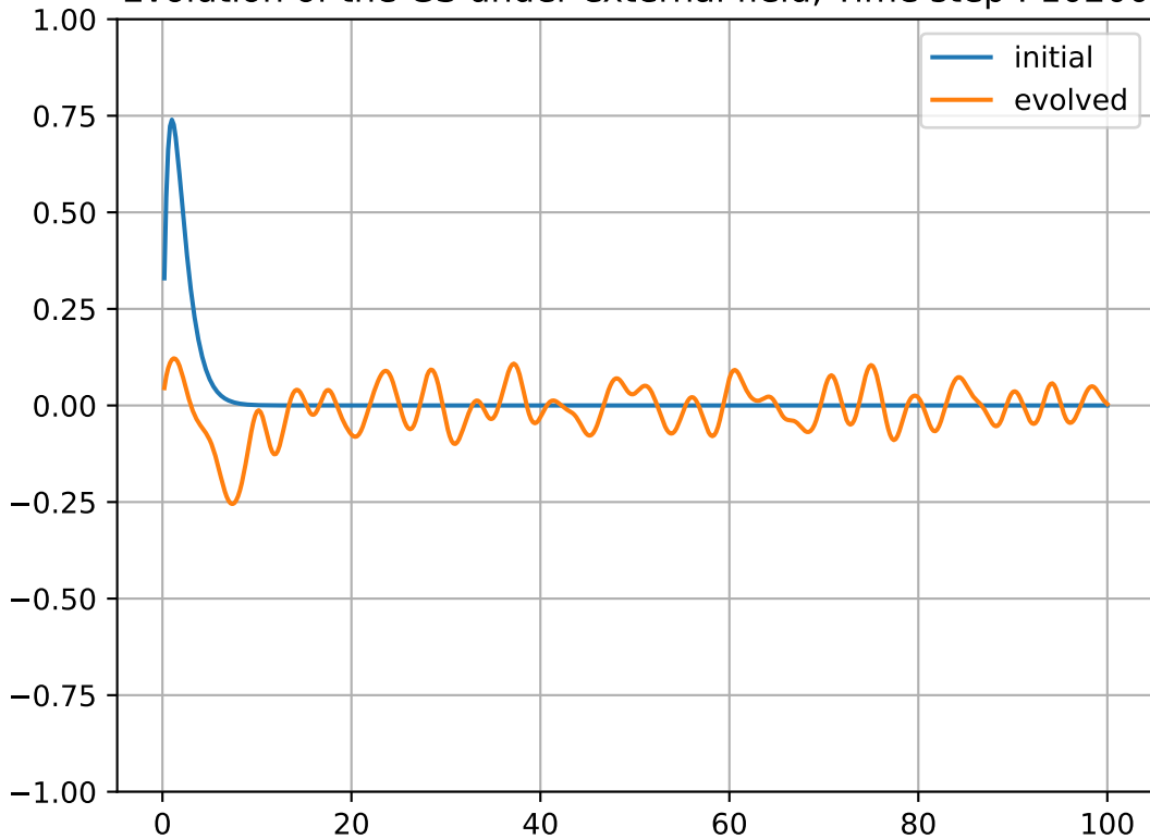
Evolution of the GS under external field, Time step : 10200
