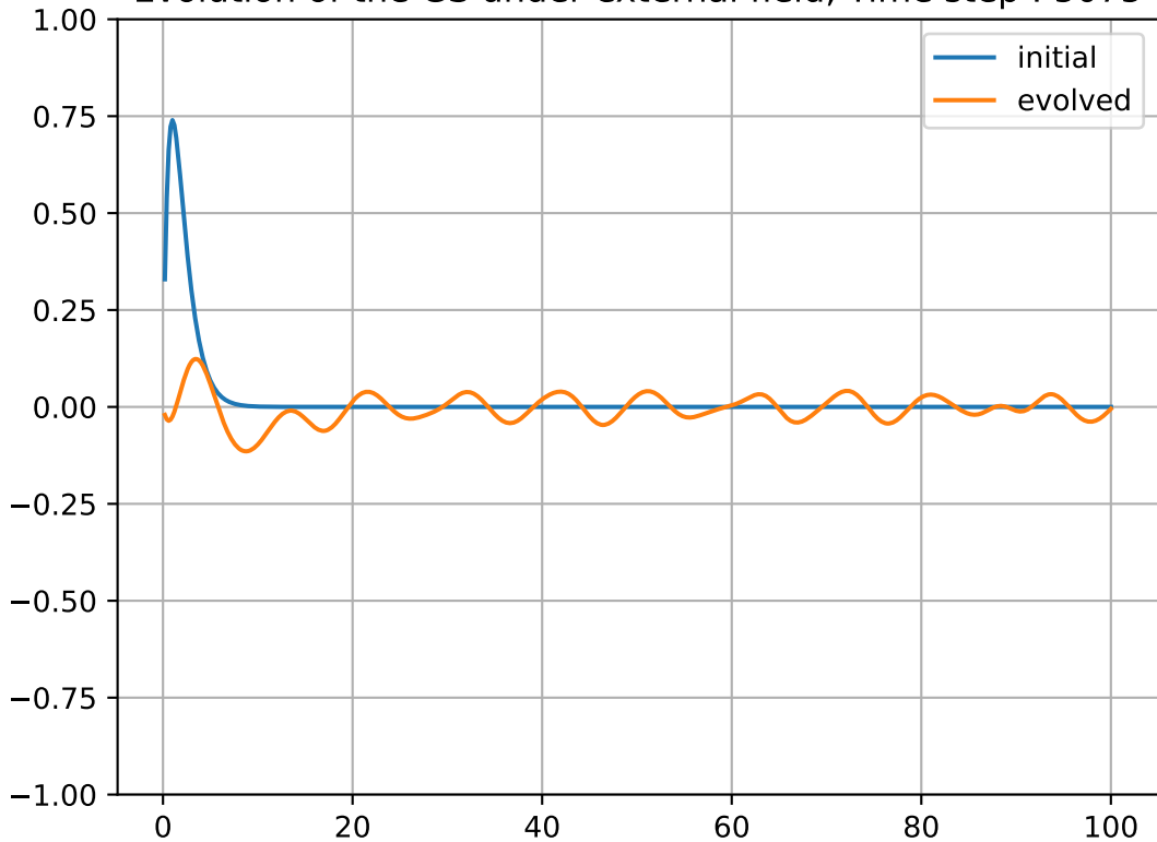
Evolution of the GS under external field, Time step : 5075
