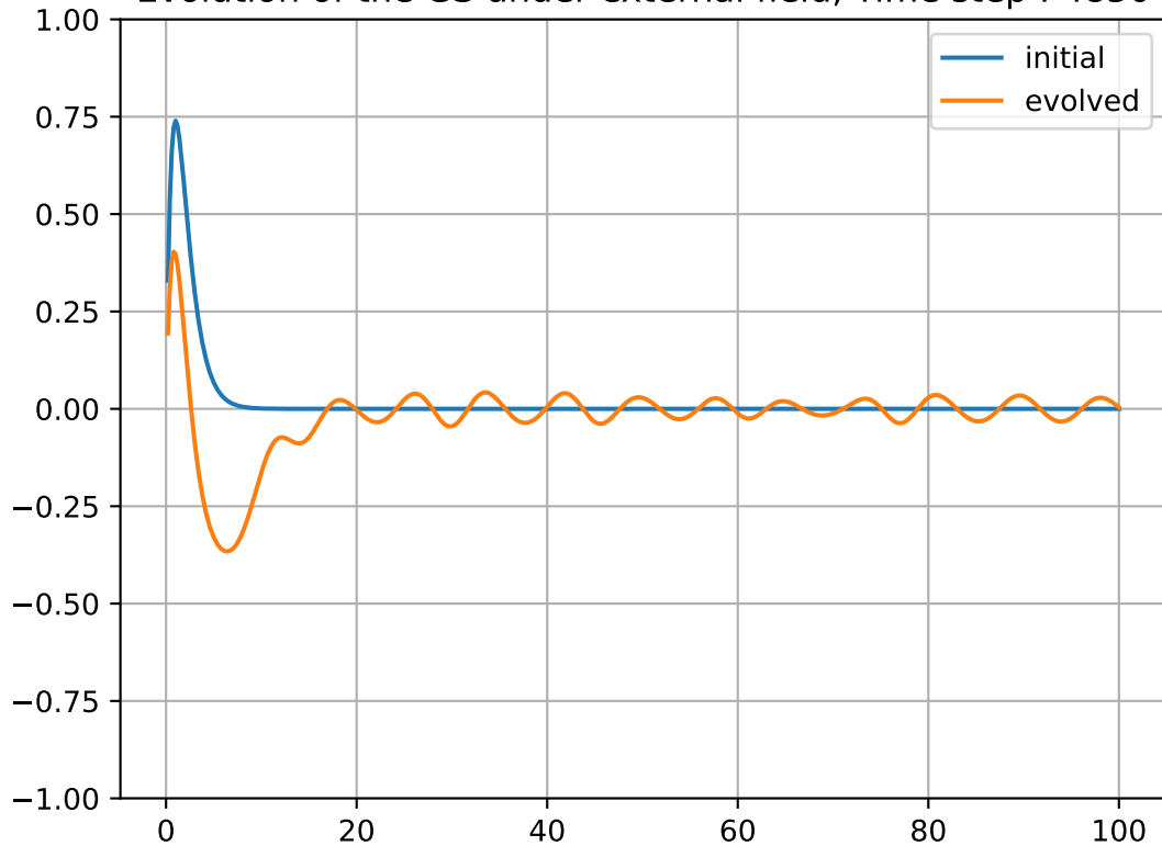
Evolution of the GS under external field, Time step : 4850
