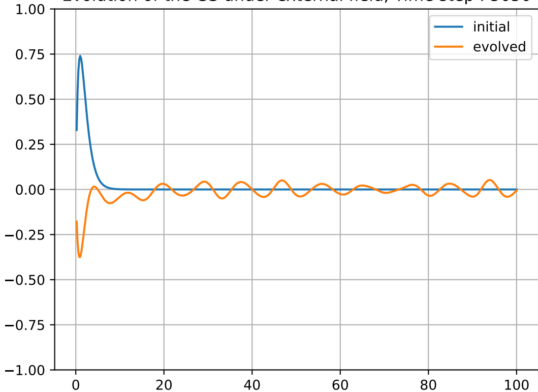
Evolution of the GS under external field, Time step : 5050
