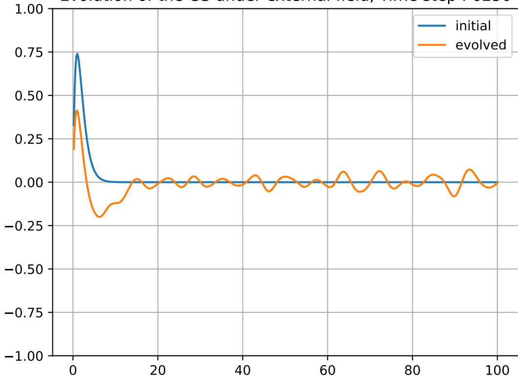
Evolution of the GS under external field, Time step : 6250
