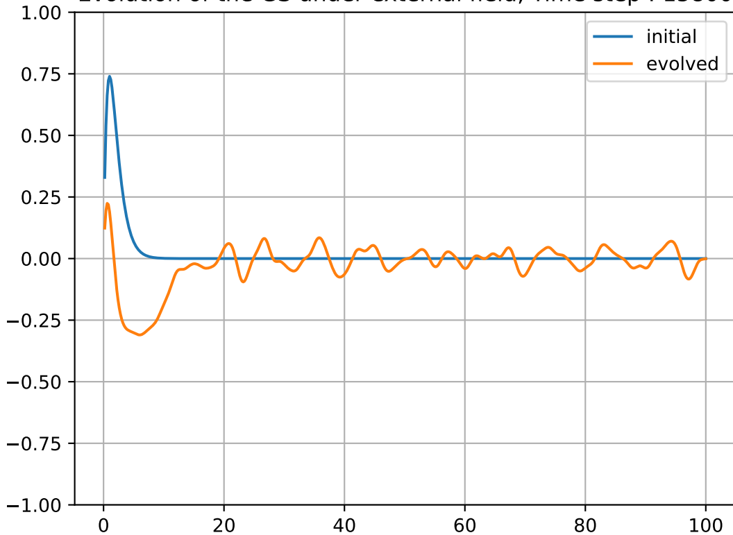
Evolution of the GS under external field, Time step : 15800
