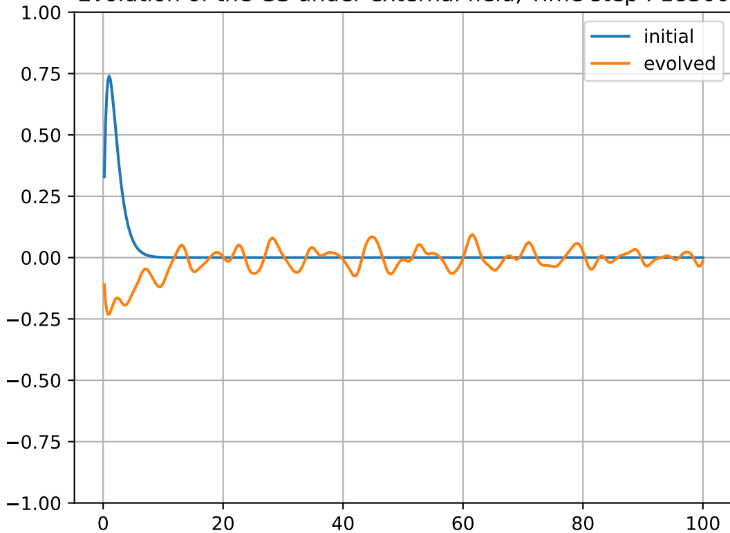
Evolution of the GS under external field, Time step : 18300
