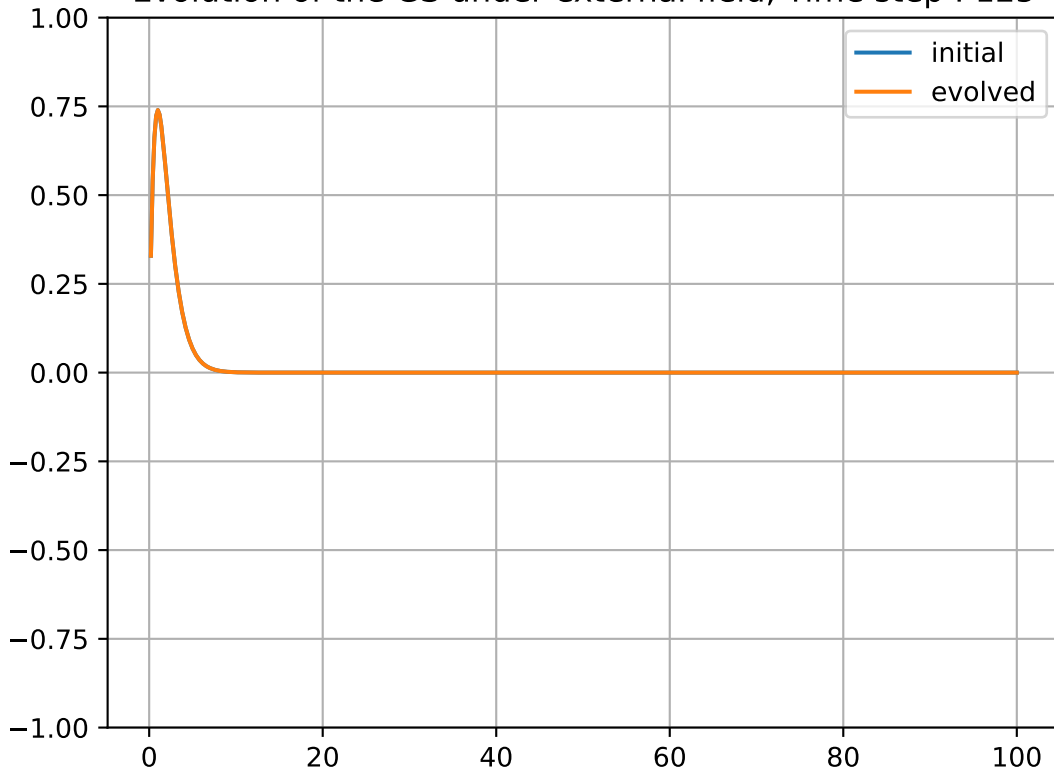
Evolution of the GS under external field, Time step : 125
