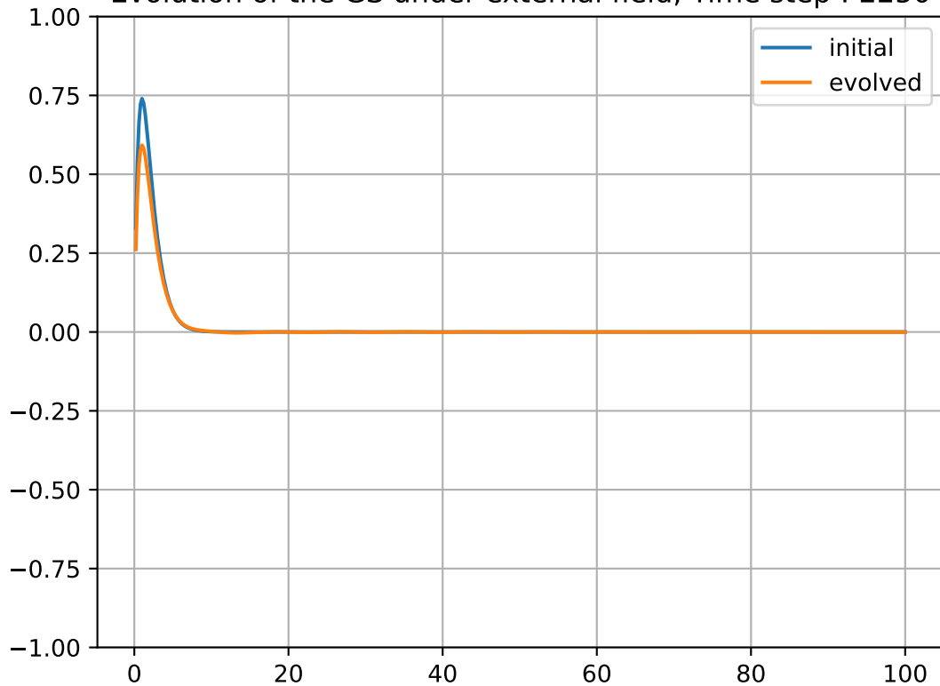
Evolution of the GS under external field, Time step : 2250
