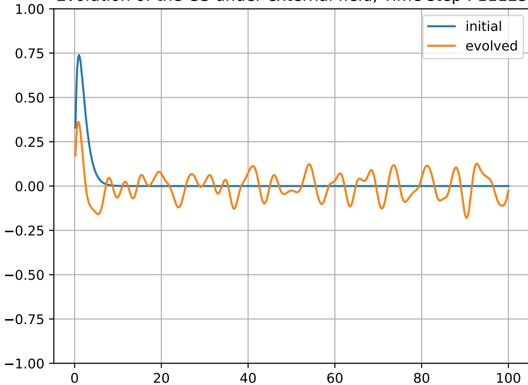
Evolution of the GS under external field, Time step : 11125
