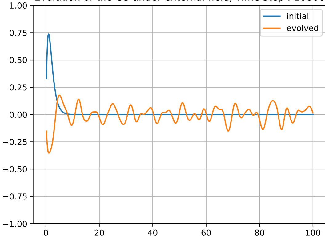
Evolution of the GS under external field, Time step : 10800
