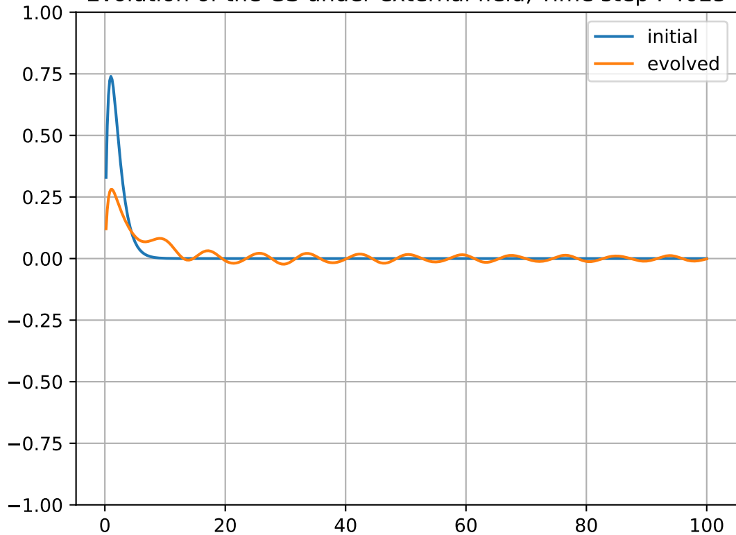
Evolution of the GS under external field, Time step : 4025
