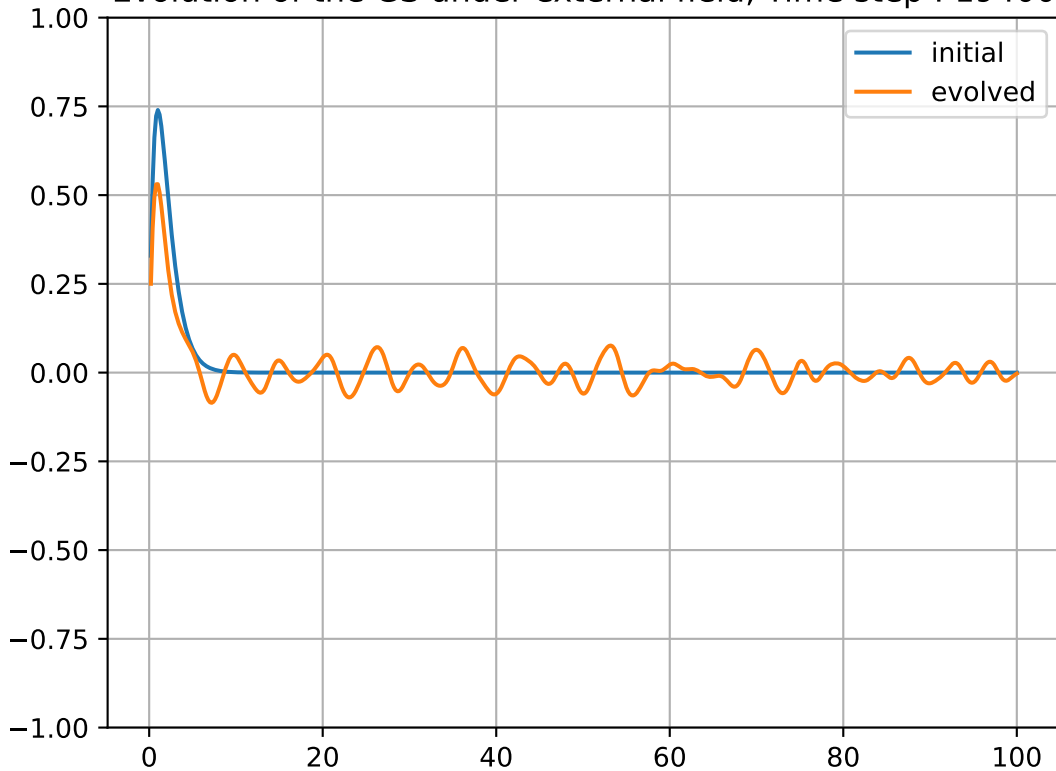
Evolution of the GS under external field, Time step : 19400
