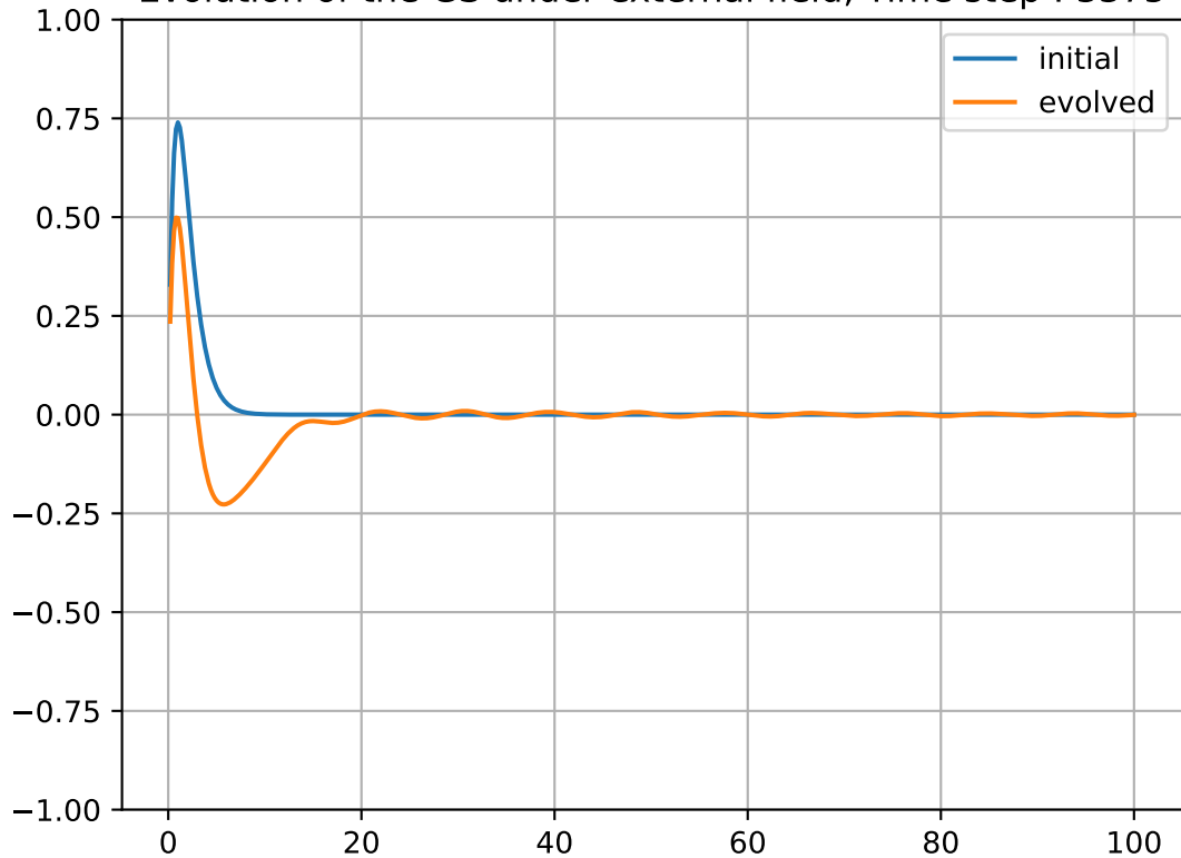
Evolution of the GS under external field, Time step : 3375
