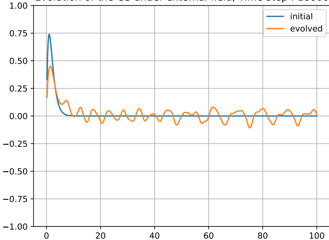
Evolution of the GS under external field, Time step : 18000
