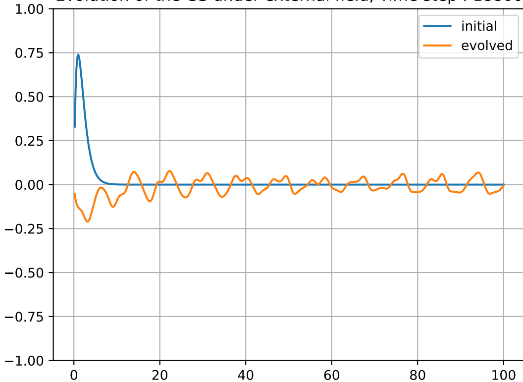
Evolution of the GS under external field, Time step : 18800
