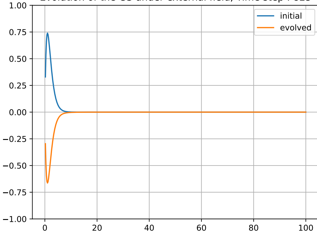
Evolution of the GS under external field, Time step : 825
