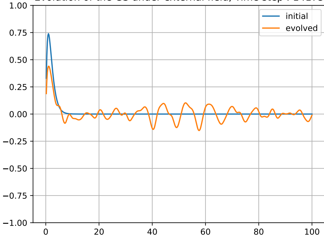
Evolution of the GS under external field, Time step : 14175
