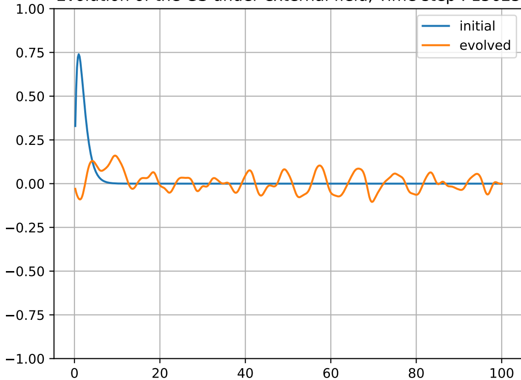
Evolution of the GS under external field, Time step : 15625
