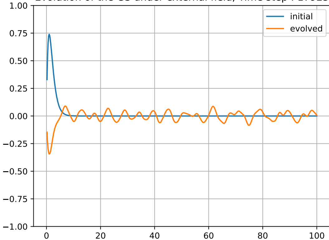
Evolution of the GS under external field, Time step : 17925
