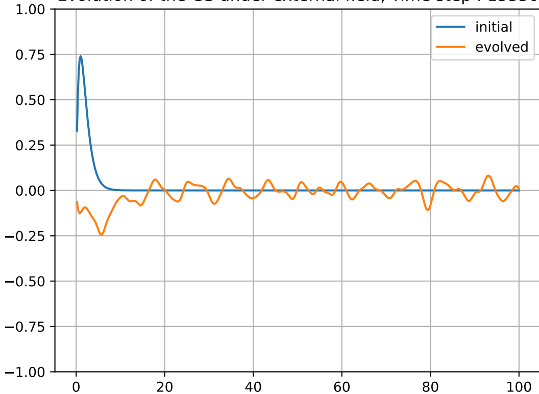
Evolution of the GS under external field, Time step : 15350
