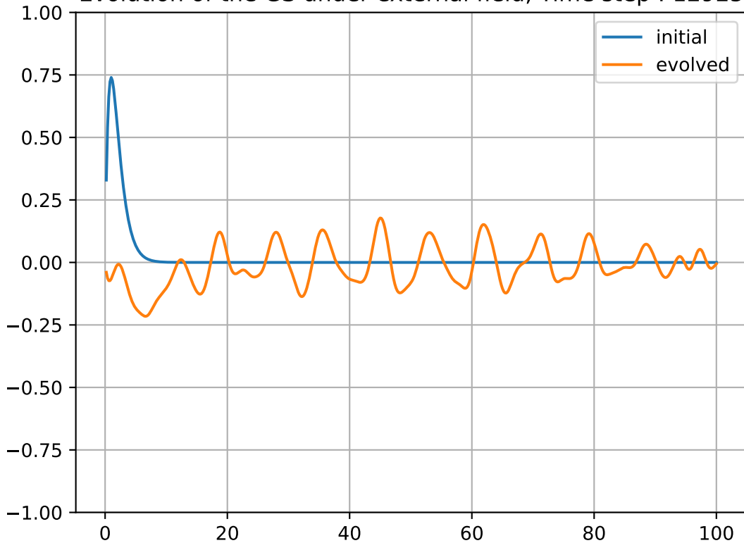
Evolution of the GS under external field, Time step : 12925
