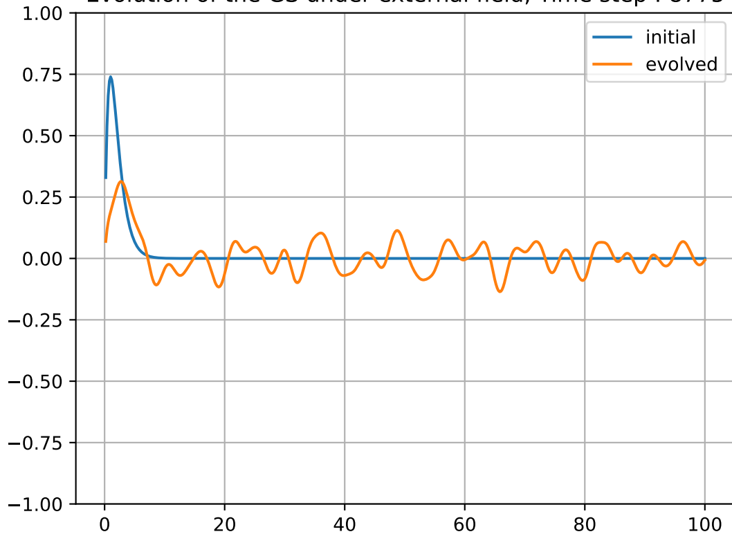
Evolution of the GS under external field, Time step : 8775
