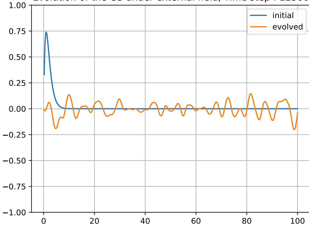
Evolution of the GS under external field, Time step : 12300
