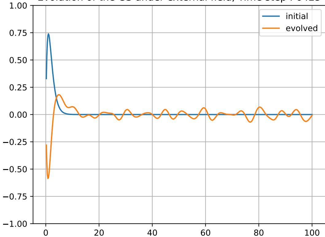
Evolution of the GS under external field, Time step : 6425
