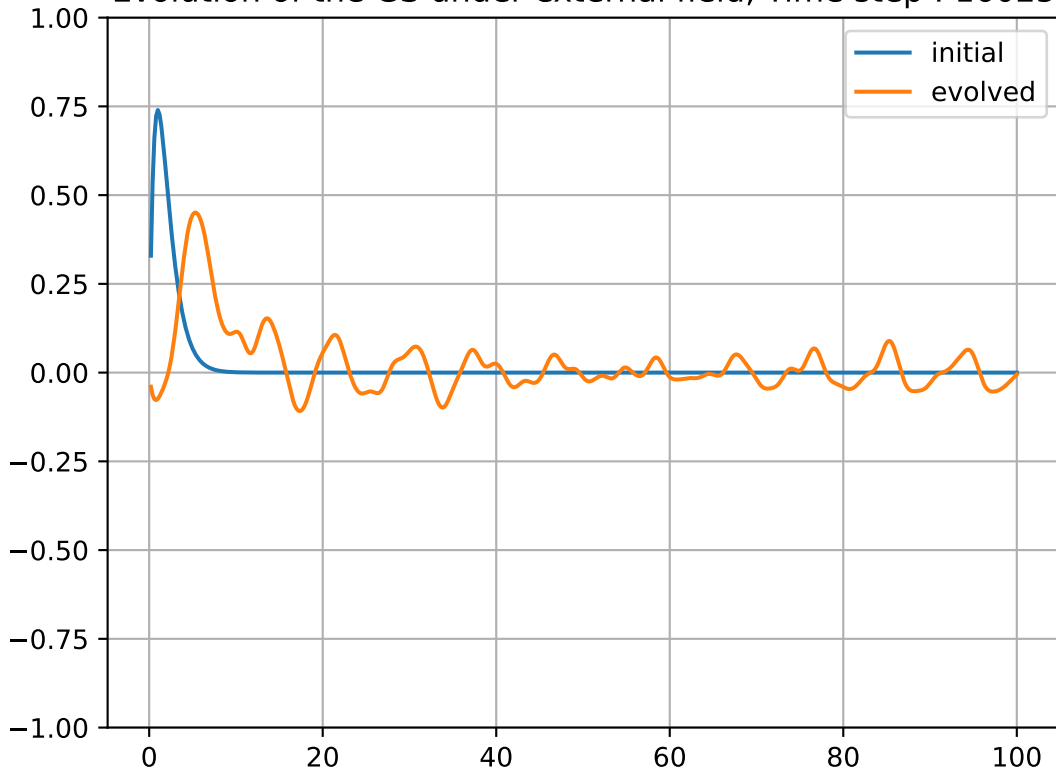
Evolution of the GS under external field, Time step : 16025
