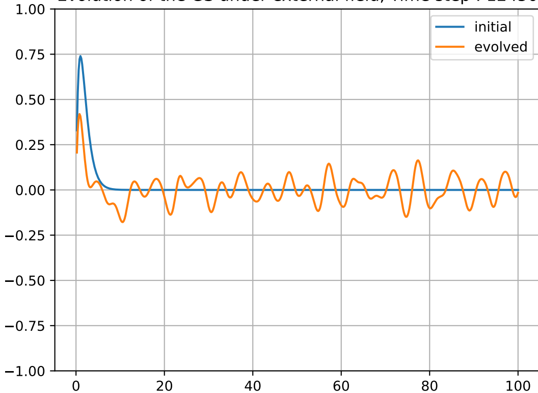
Evolution of the GS under external field, Time step : 12450
