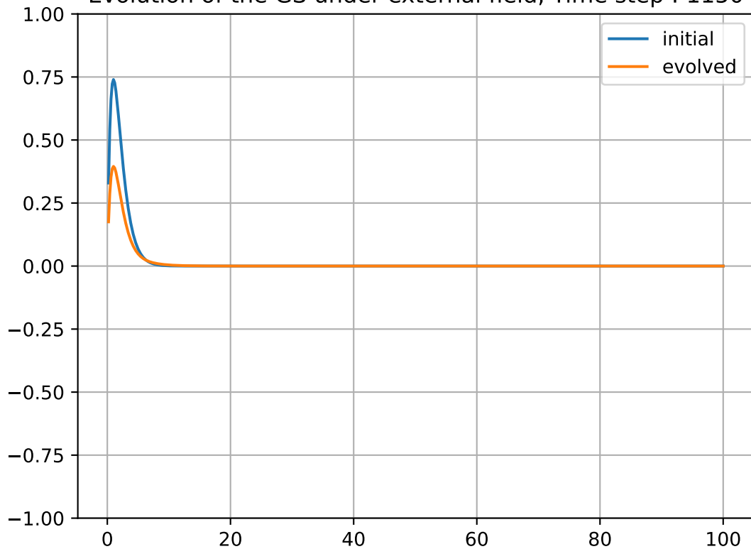
Evolution of the GS under external field, Time step : 1150
