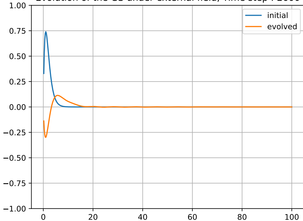
Evolution of the GS under external field, Time step : 2600
