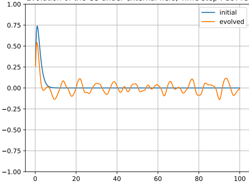
Evolution of the GS under external field, Time step : 18775
