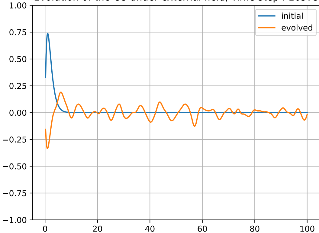
Evolution of the GS under external field, Time step : 16575
