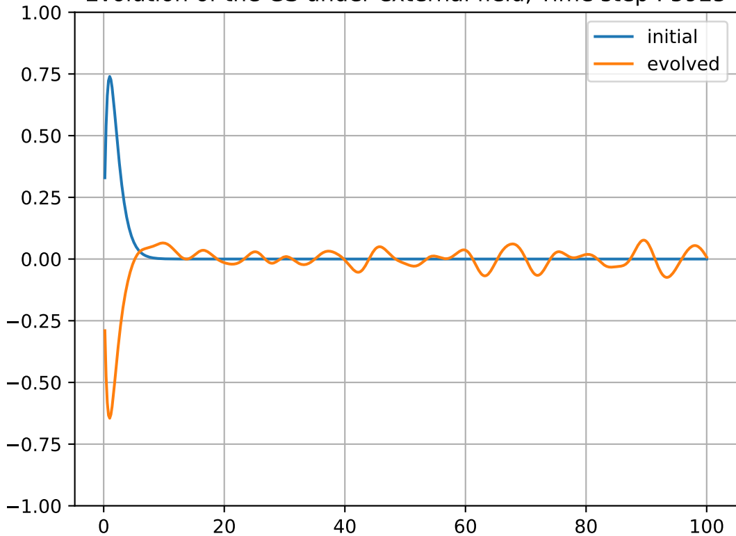
Evolution of the GS under external field, Time step : 5925
