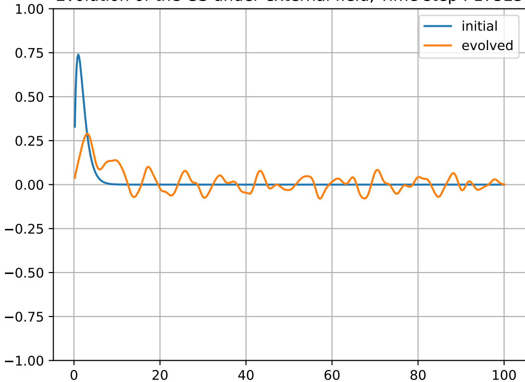
Evolution of the GS under external field, Time step : 17525
