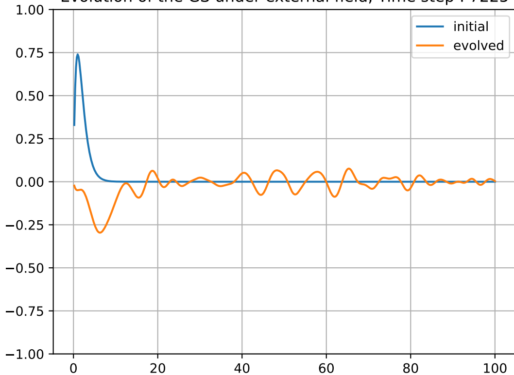
Evolution of the GS under external field, Time step : 7225
