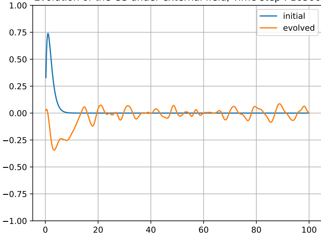
Evolution of the GS under external field, Time step : 16300
