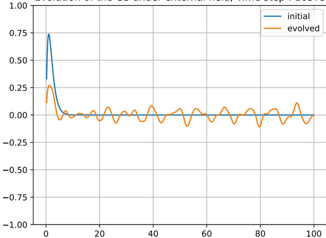
Evolution of the GS under external field, Time step : 16375
