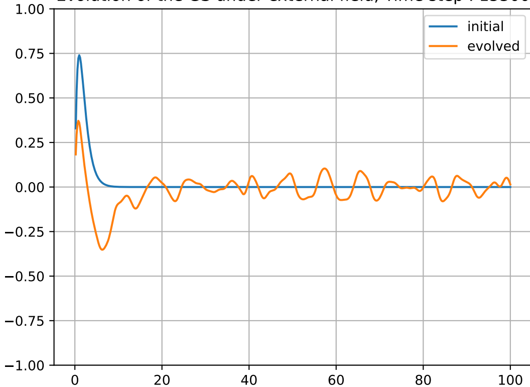
Evolution of the GS under external field, Time step : 15300
