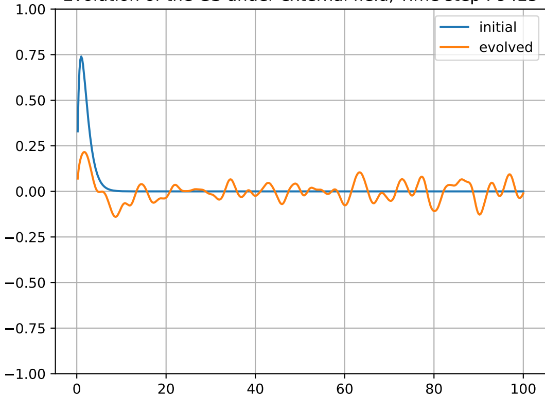
Evolution of the GS under external field, Time step : 9425
