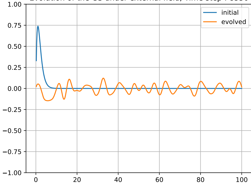
Evolution of the GS under external field, Time step : 8550
