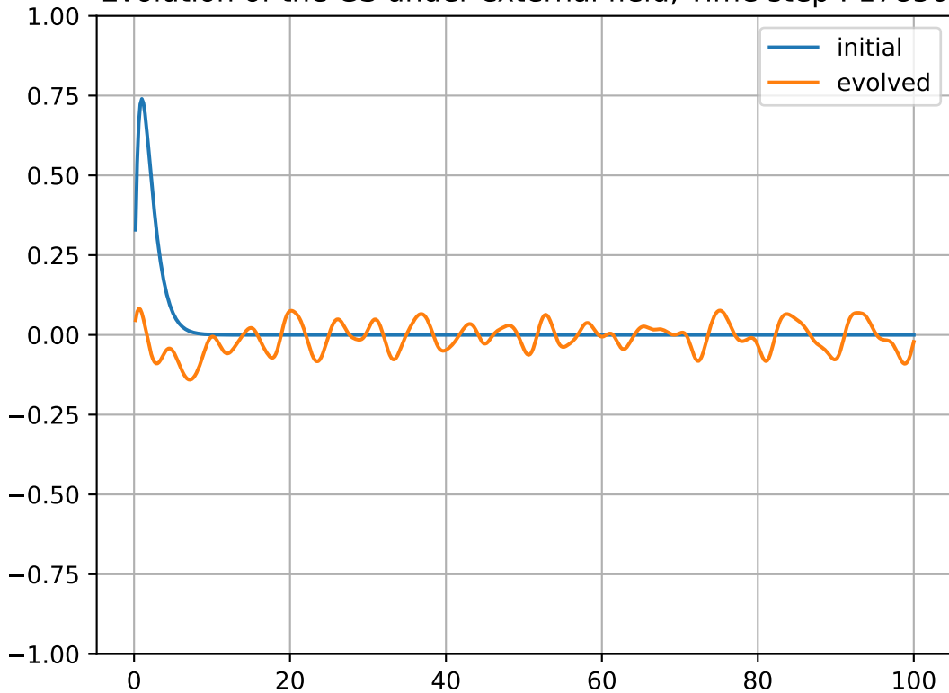
Evolution of the GS under external field, Time step : 17850
