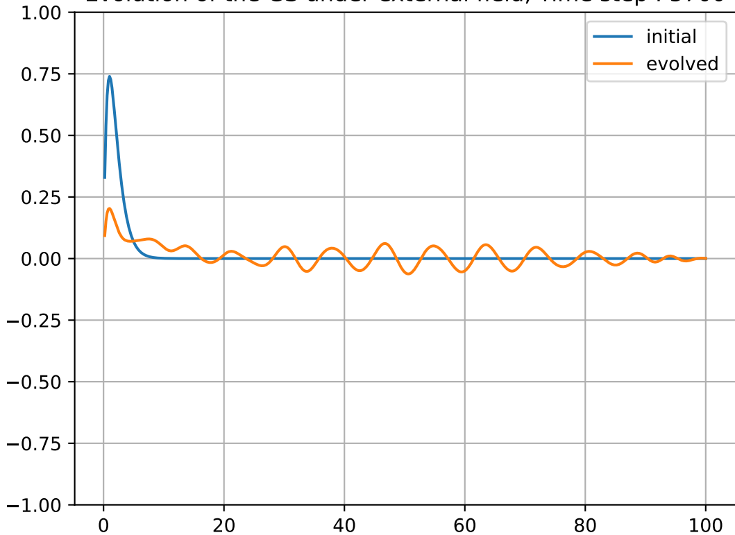
Evolution of the GS under external field, Time step : 5700
