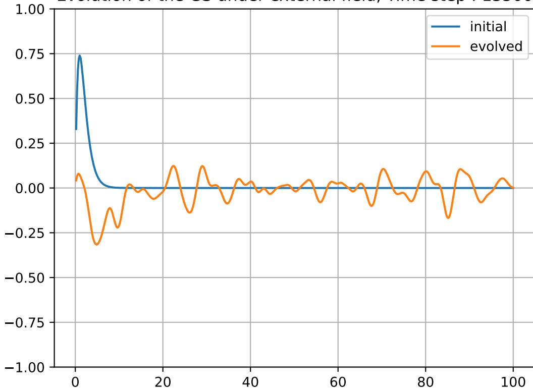
Evolution of the GS under external field, Time step : 13500
