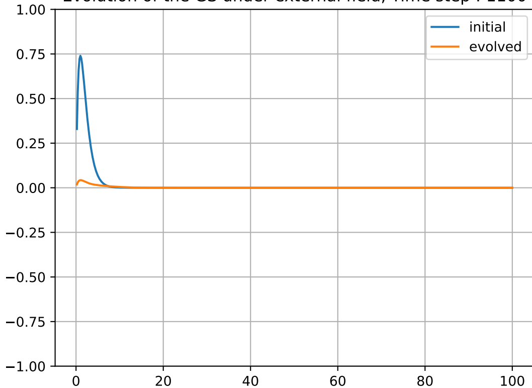
Evolution of the GS under external field, Time step : 1100
