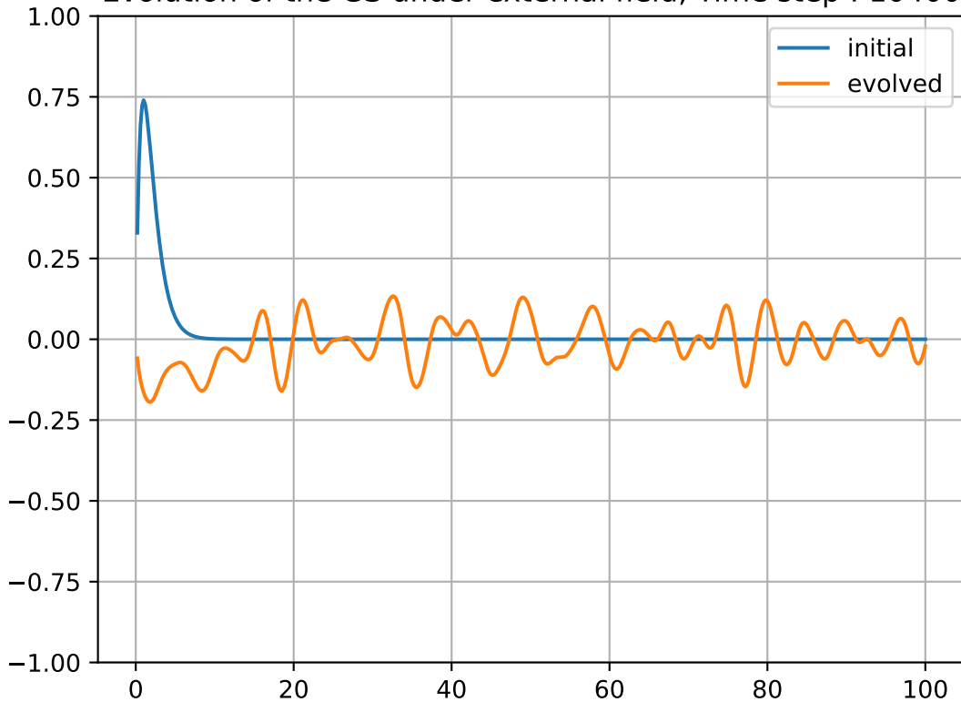
Evolution of the GS under external field, Time step : 10400
