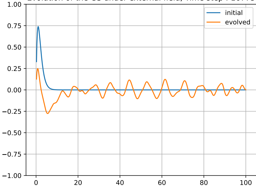
Evolution of the GS under external field, Time step : 16775
