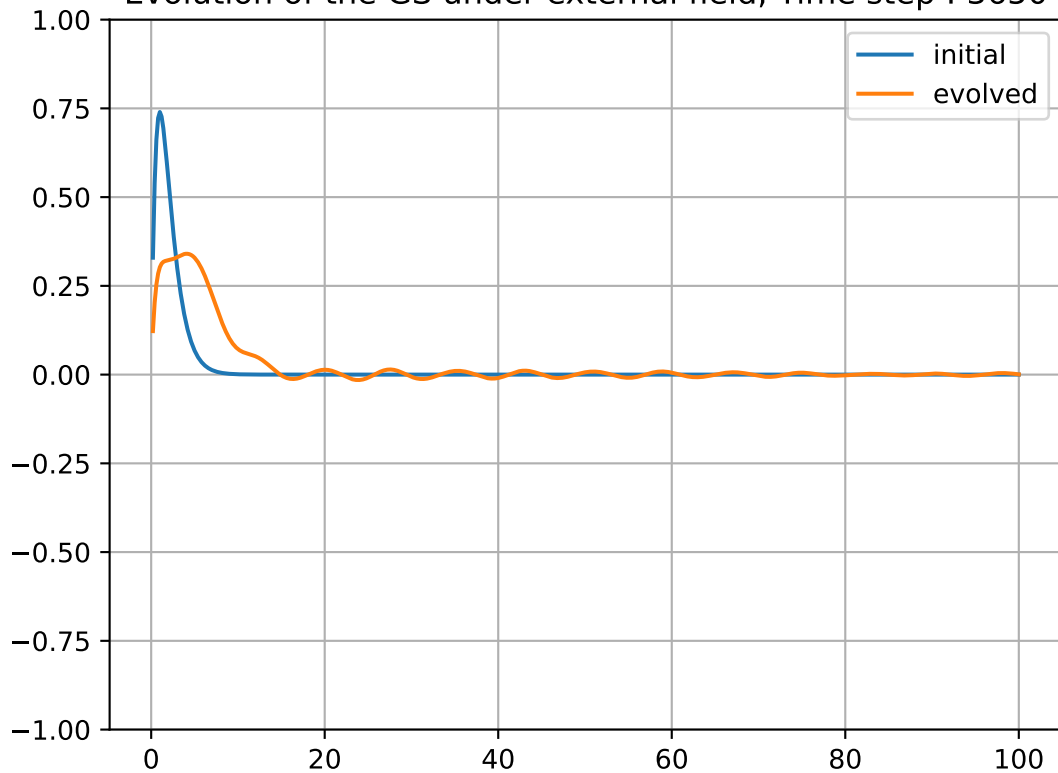
Evolution of the GS under external field, Time step : 3650
