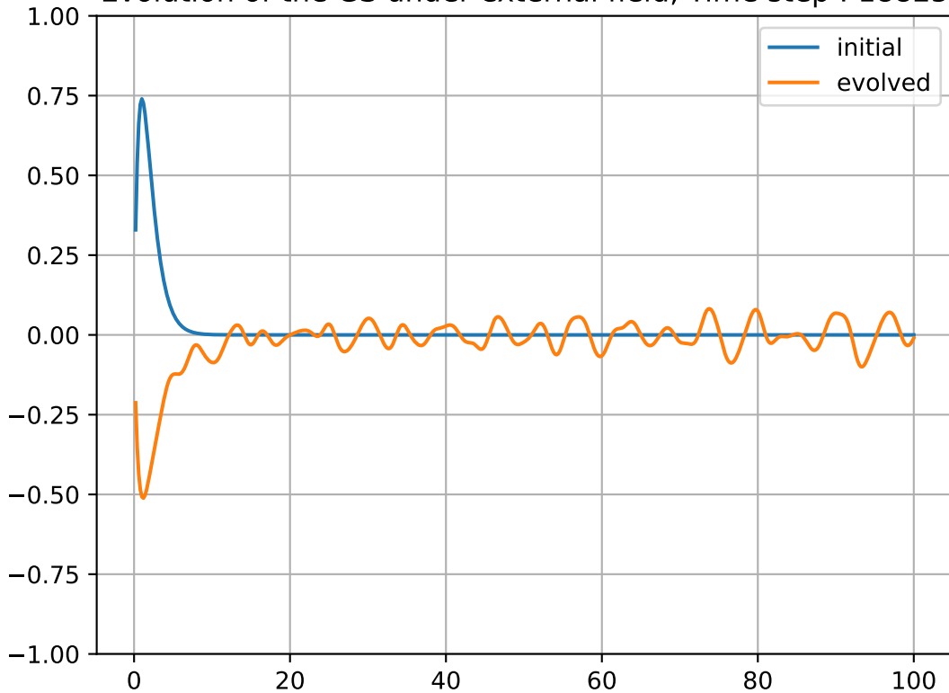
Evolution of the GS under external field, Time step : 18825
