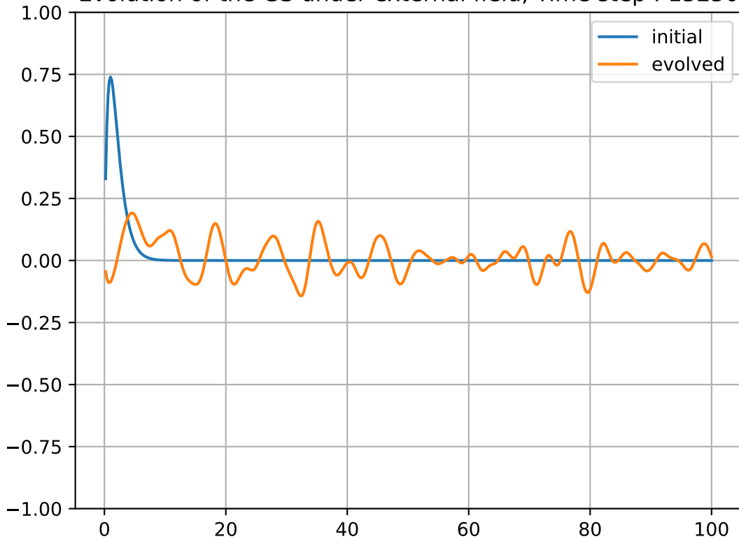
Evolution of the GS under external field, Time step : 13250
