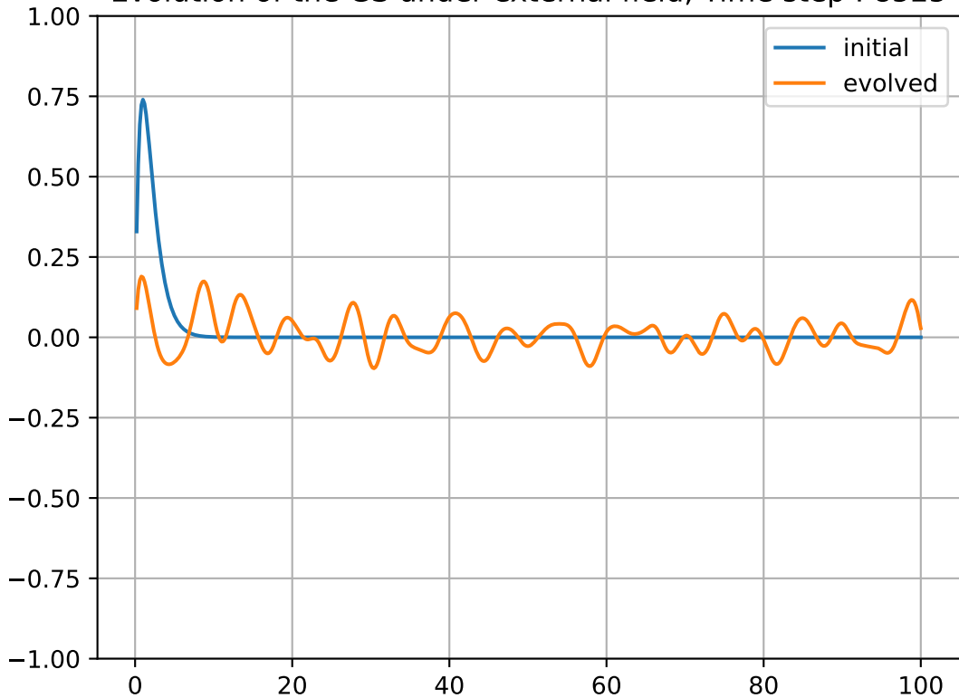
Evolution of the GS under external field, Time step : 8525
