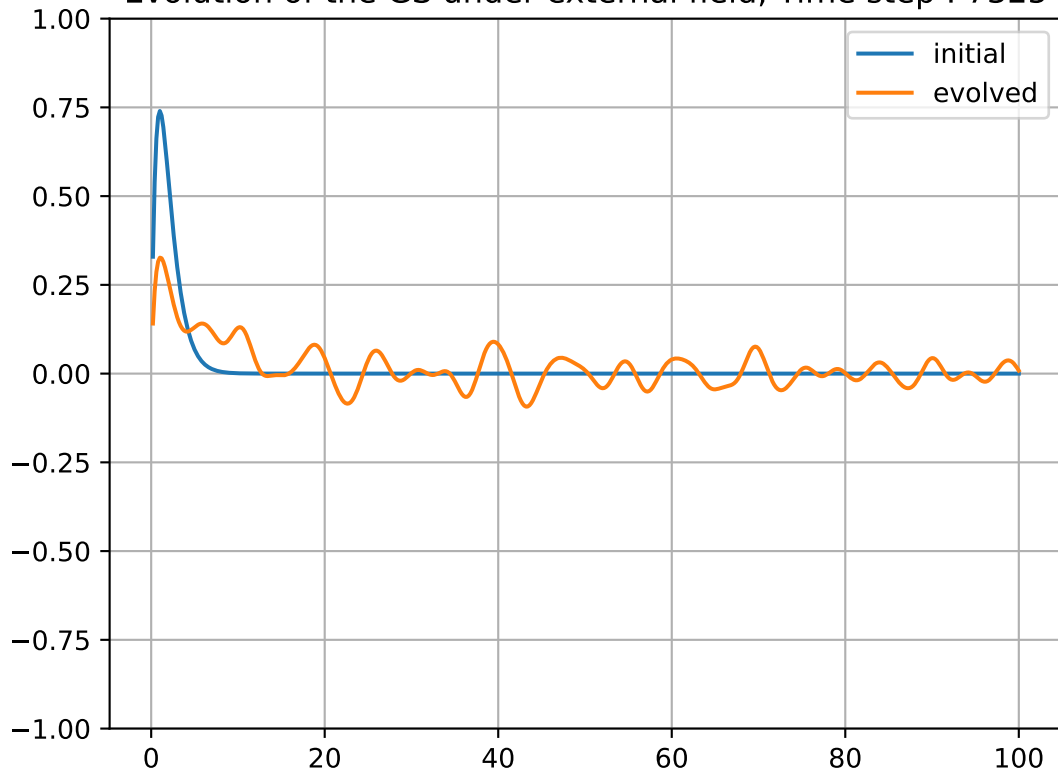
Evolution of the GS under external field, Time step : 7325
