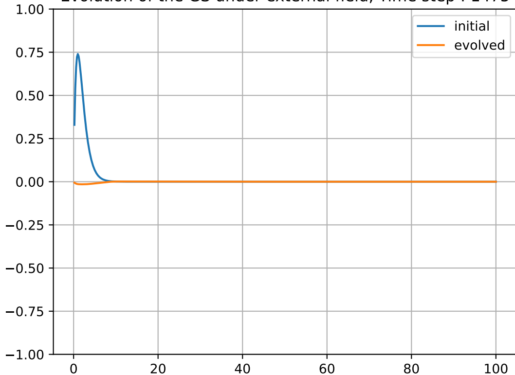
Evolution of the GS under external field, Time step : 1475
