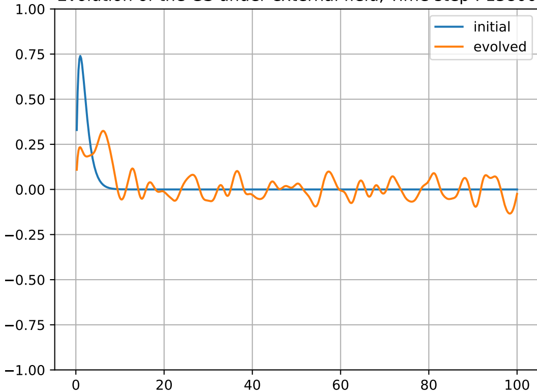
Evolution of the GS under external field, Time step : 13800
