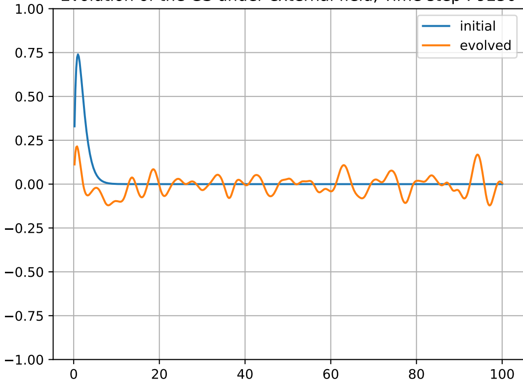
Evolution of the GS under external field, Time step : 9250
