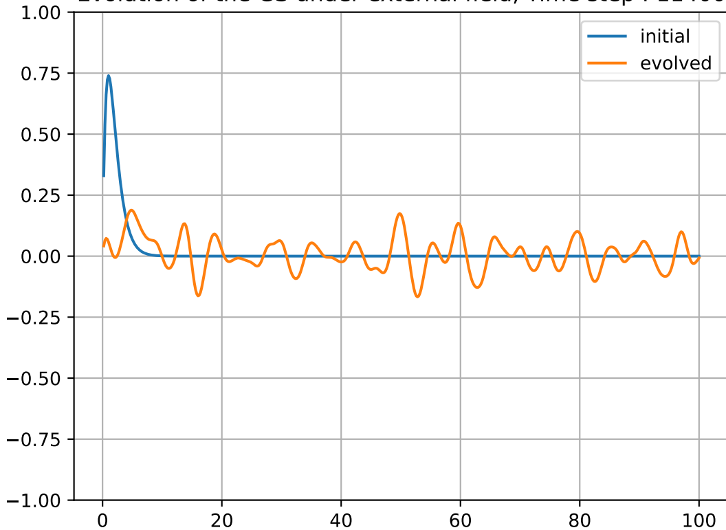
Evolution of the GS under external field, Time step : 11400
