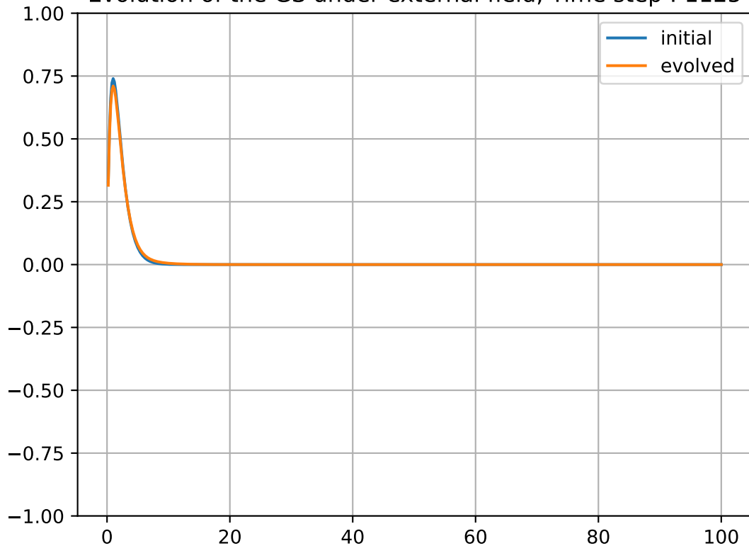
Evolution of the GS under external field, Time step : 1125
