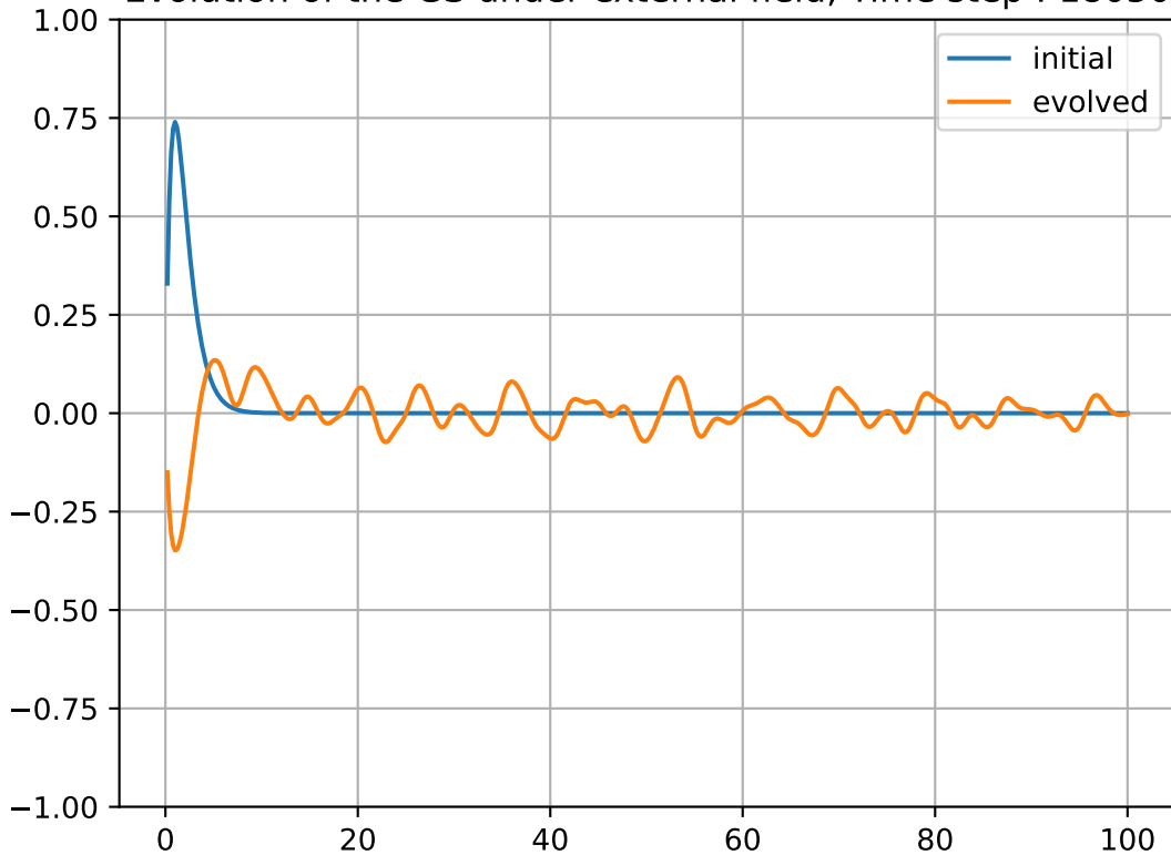
Evolution of the GS under external field, Time step : 18050
