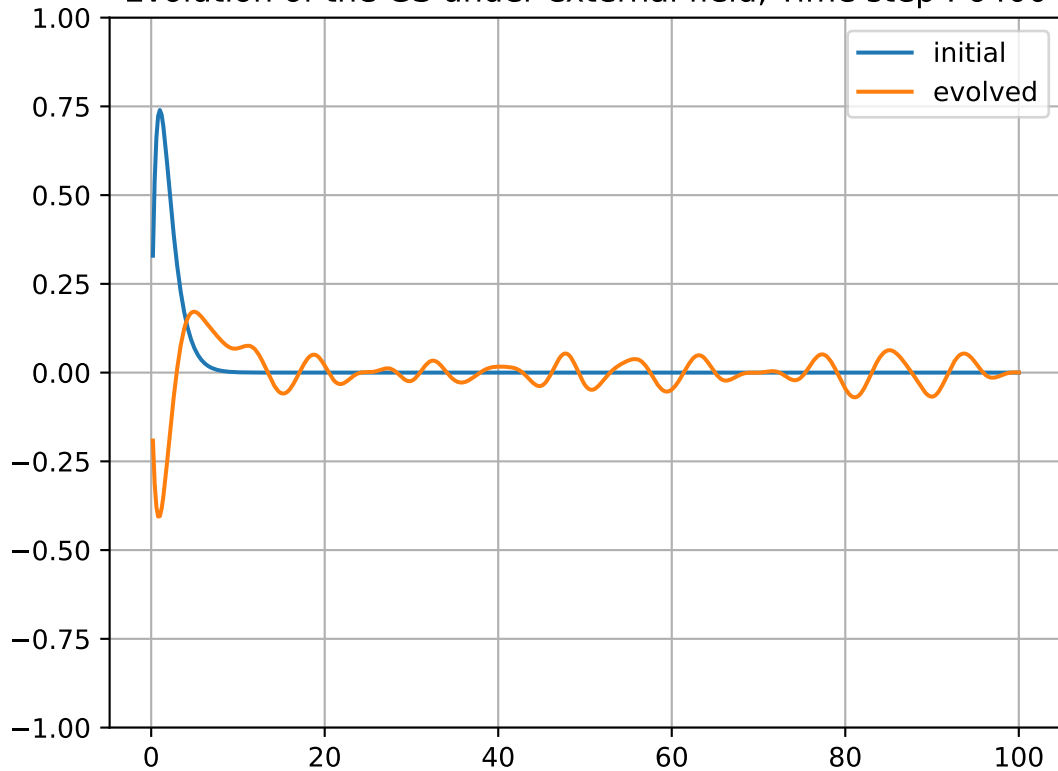
Evolution of the GS under external field, Time step : 6400
