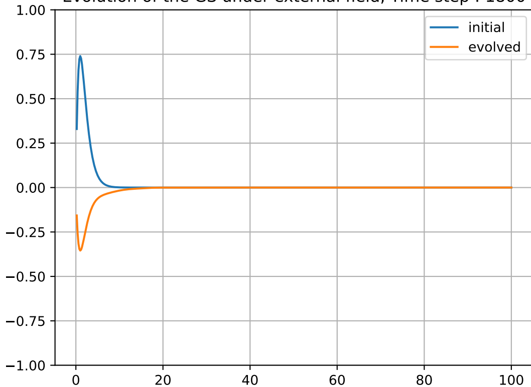
Evolution of the GS under external field, Time step : 1800
