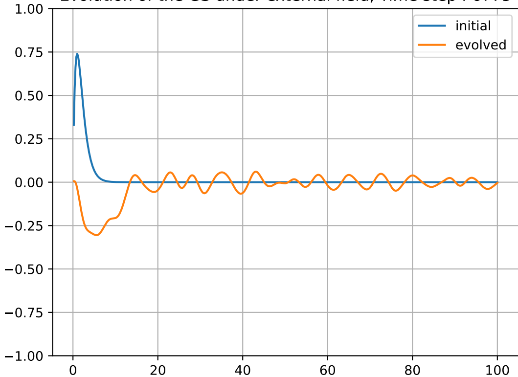
Evolution of the GS under external field, Time step : 6775
