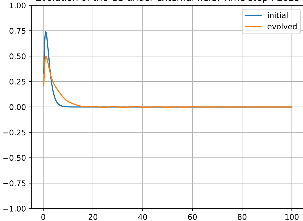
Evolution of the GS under external field, Time step : 2625
