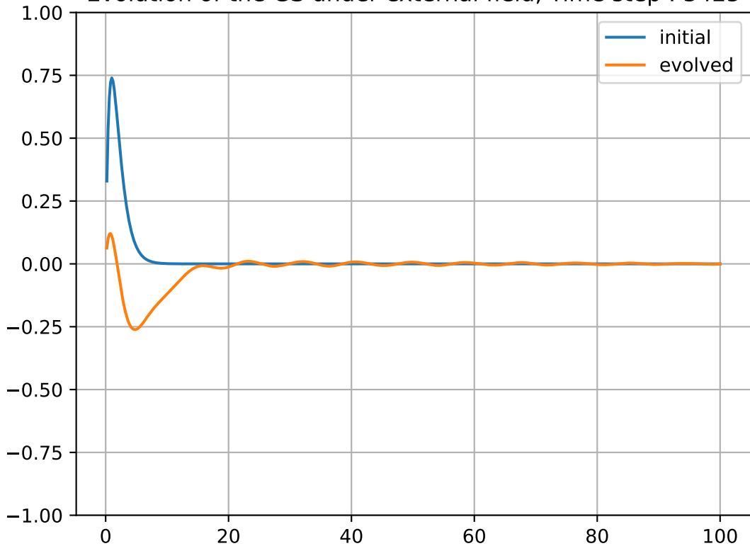
Evolution of the GS under external field, Time step : 3425
