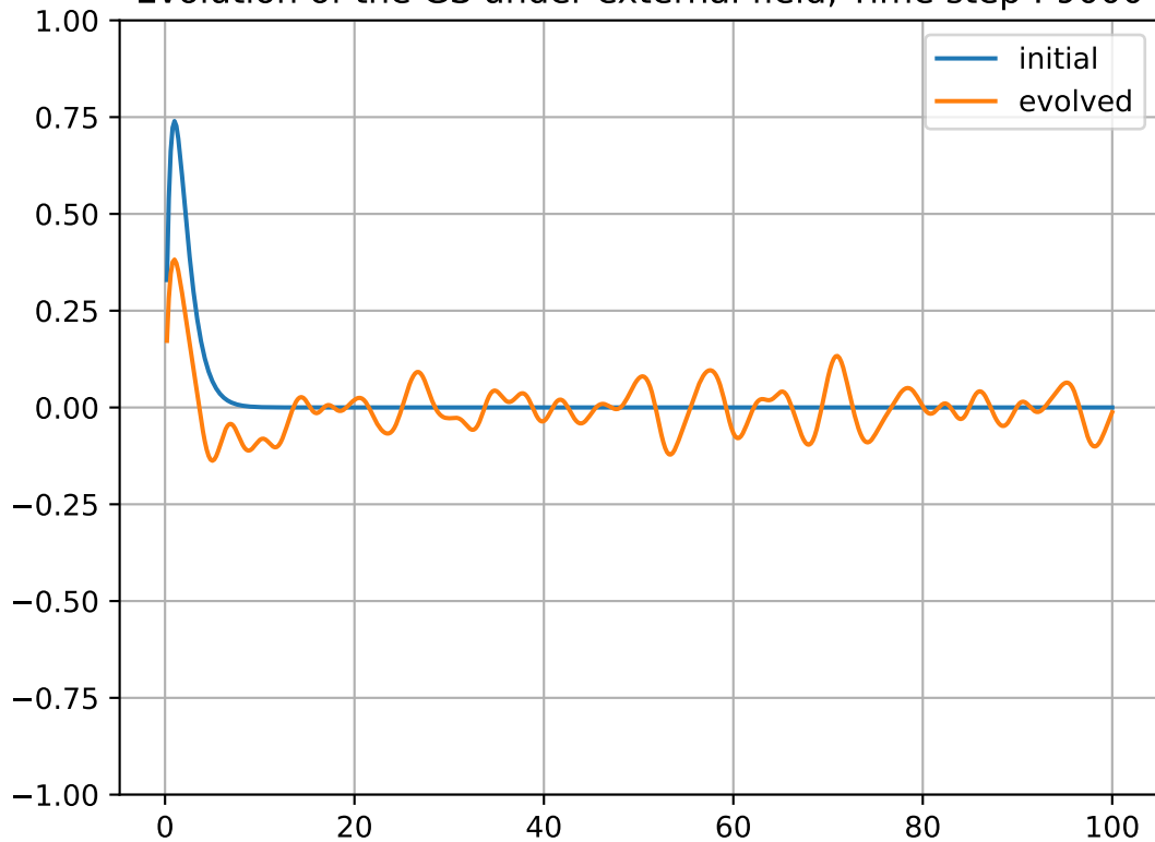
Evolution of the GS under external field, Time step : 9000
