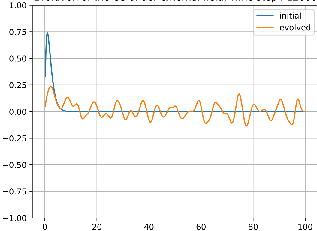
Evolution of the GS under external field, Time step : 12600
