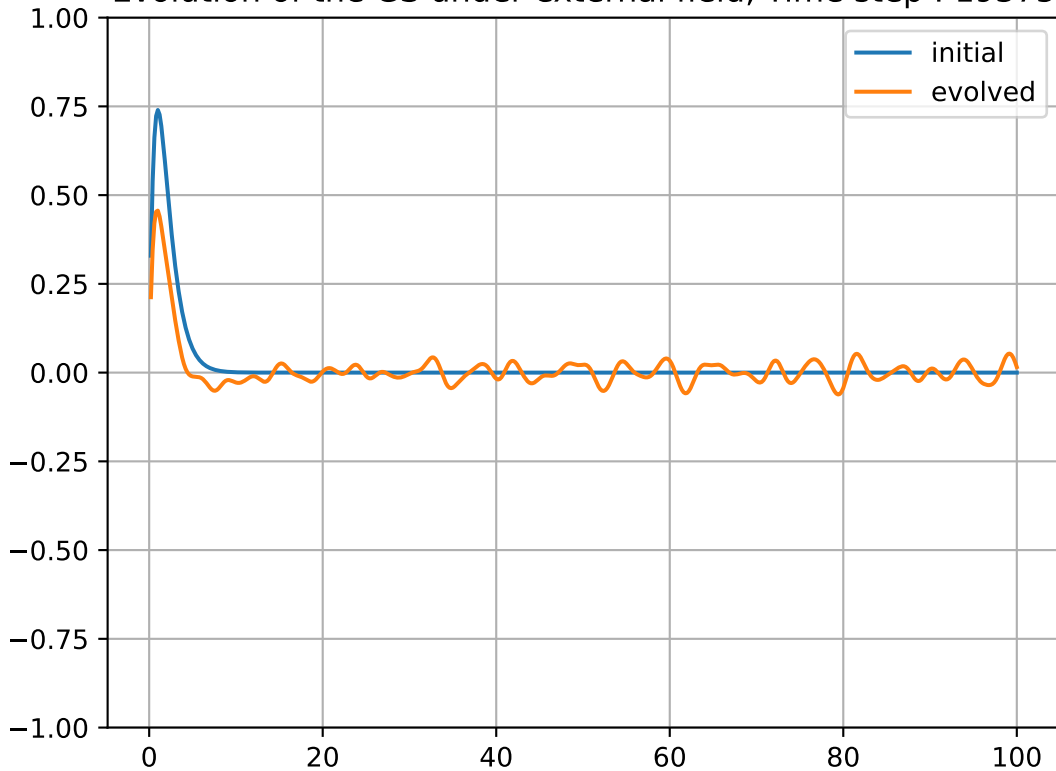
Evolution of the GS under external field, Time step : 19375
