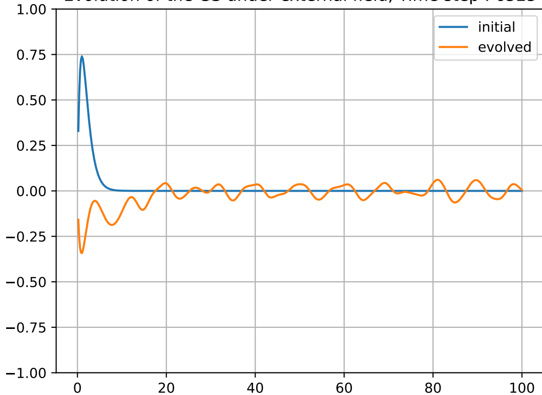
Evolution of the GS under external field, Time step : 6525
