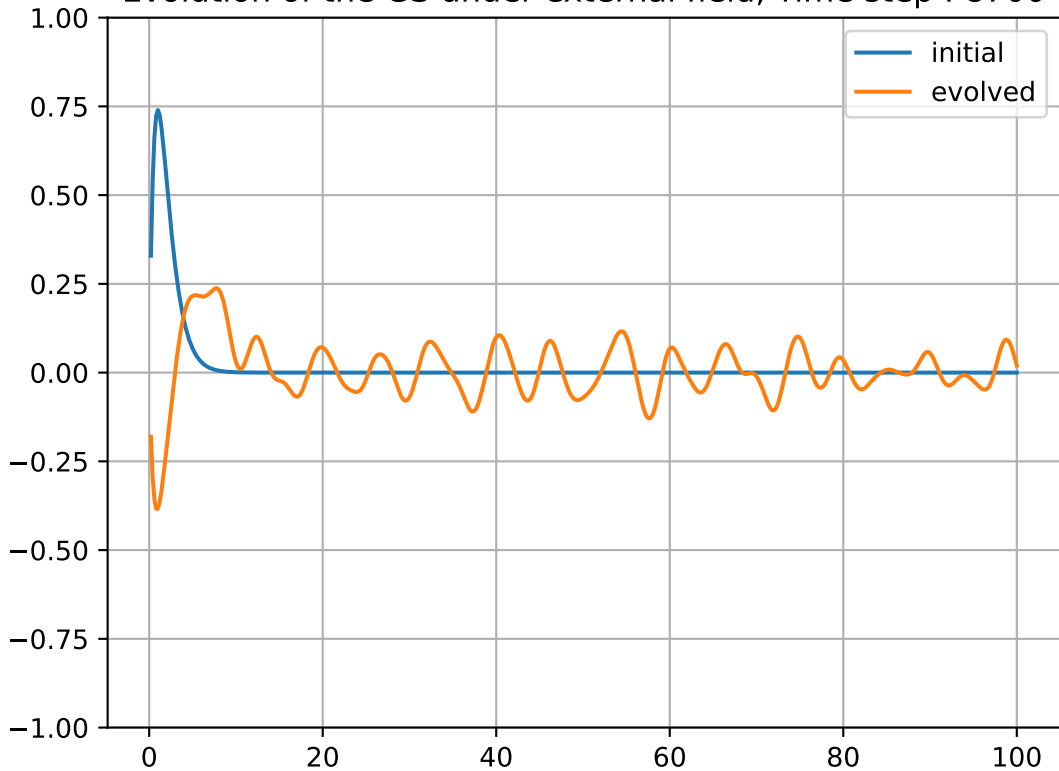
Evolution of the GS under external field, Time step : 8700
