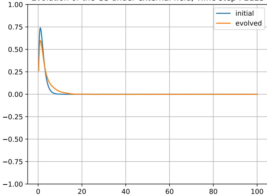
Evolution of the GS under external field, Time step : 2125
