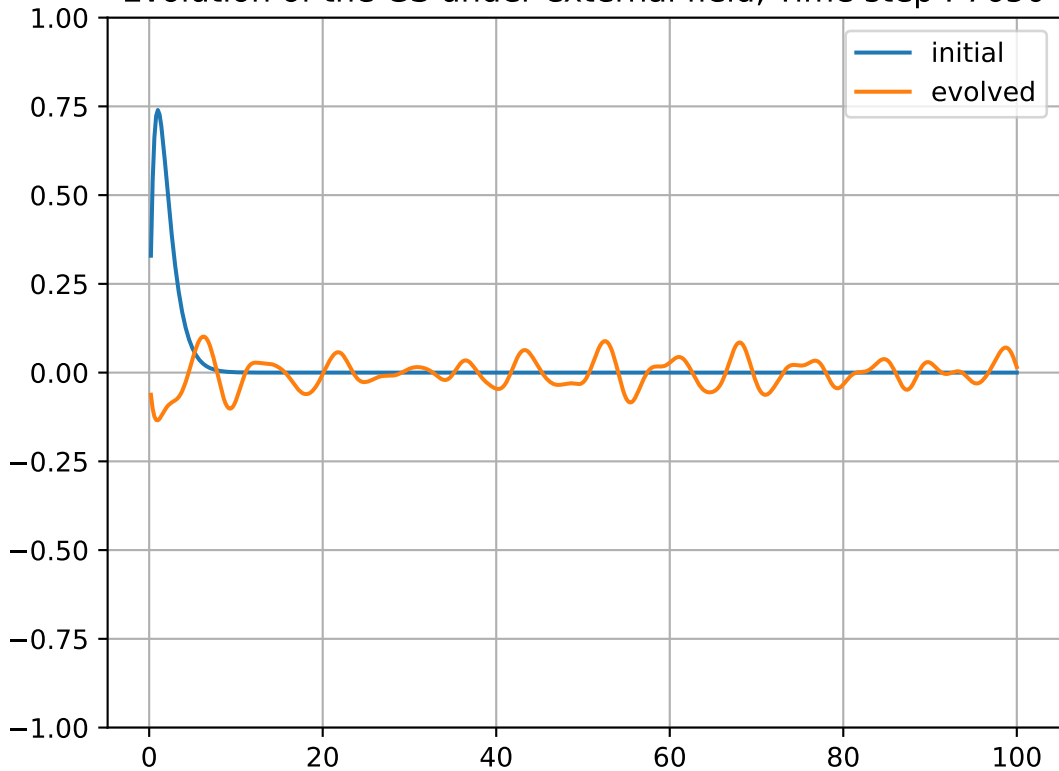
Evolution of the GS under external field, Time step : 7650
