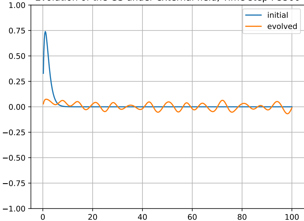
Evolution of the GS under external field, Time step : 5500
