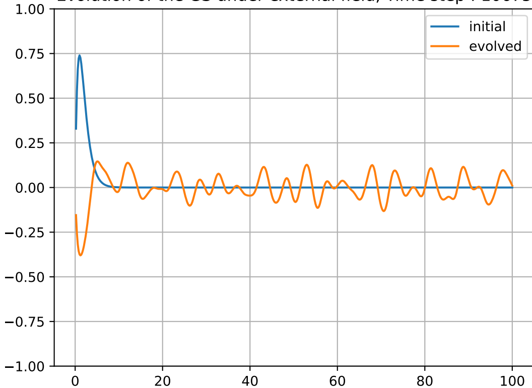
Evolution of the GS under external field, Time step : 10675
