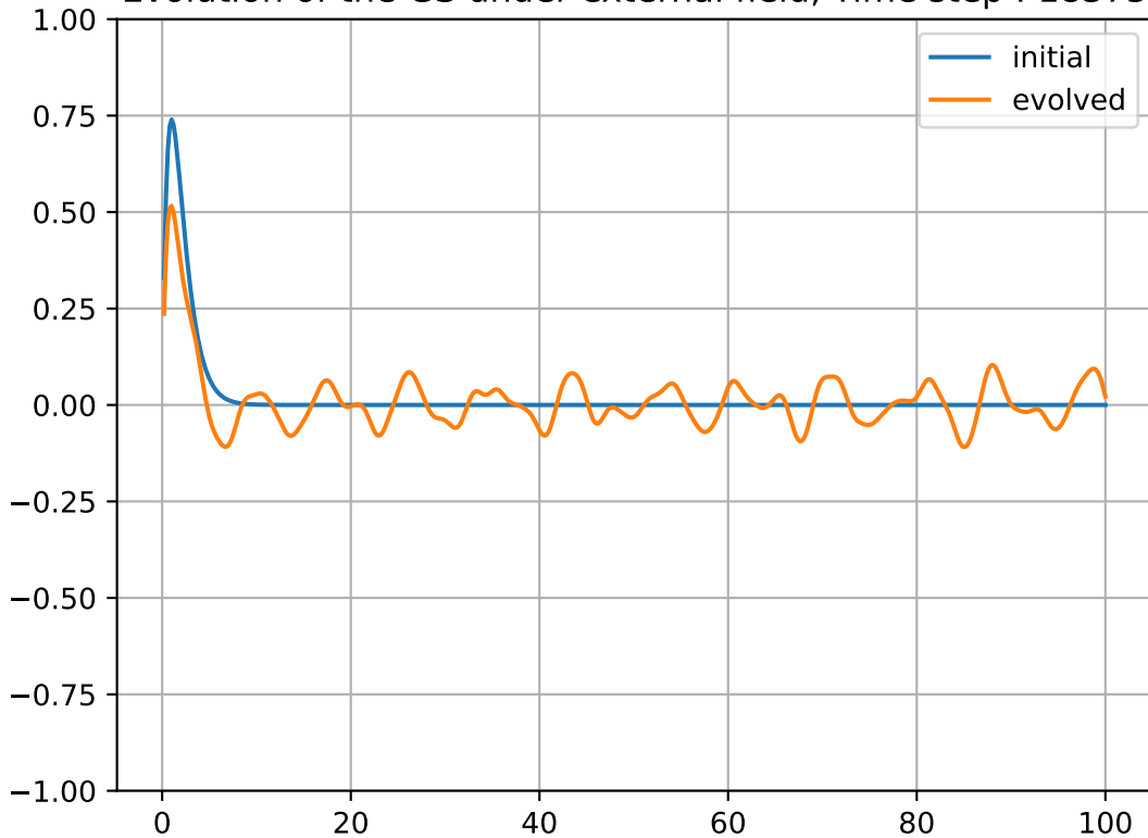
Evolution of the GS under external field, Time step : 18375
