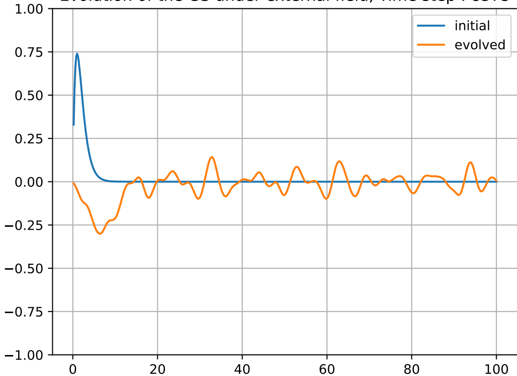
Evolution of the GS under external field, Time step : 8575
