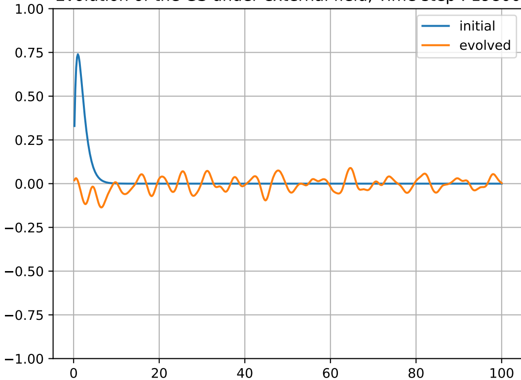
Evolution of the GS under external field, Time step : 19800
