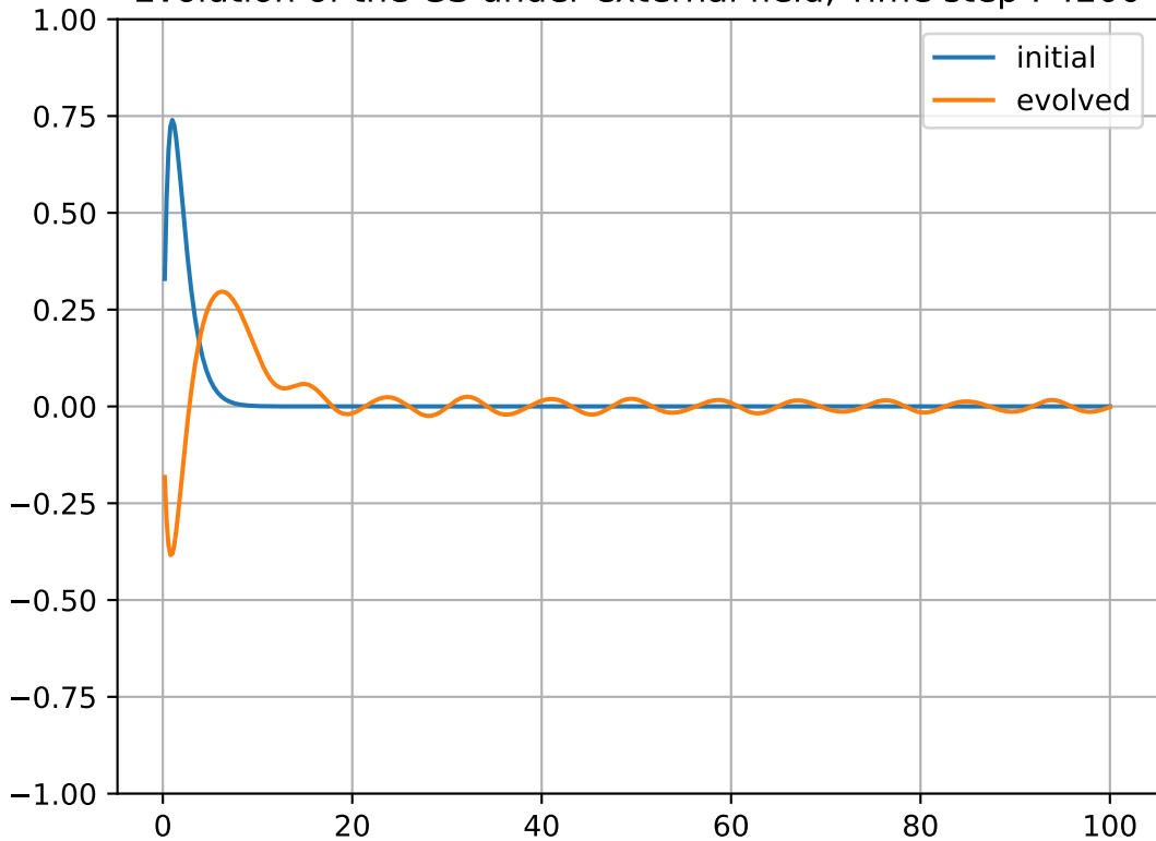
Evolution of the GS under external field, Time step : 4200
