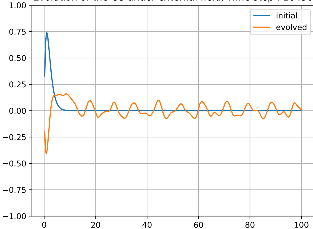
Evolution of the GS under external field, Time step : 16450
