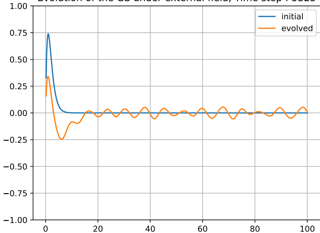
Evolution of the GS under external field, Time step : 5325
