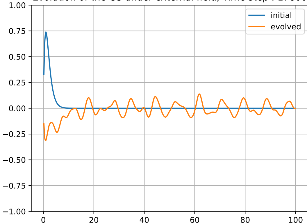
Evolution of the GS under external field, Time step : 17800
