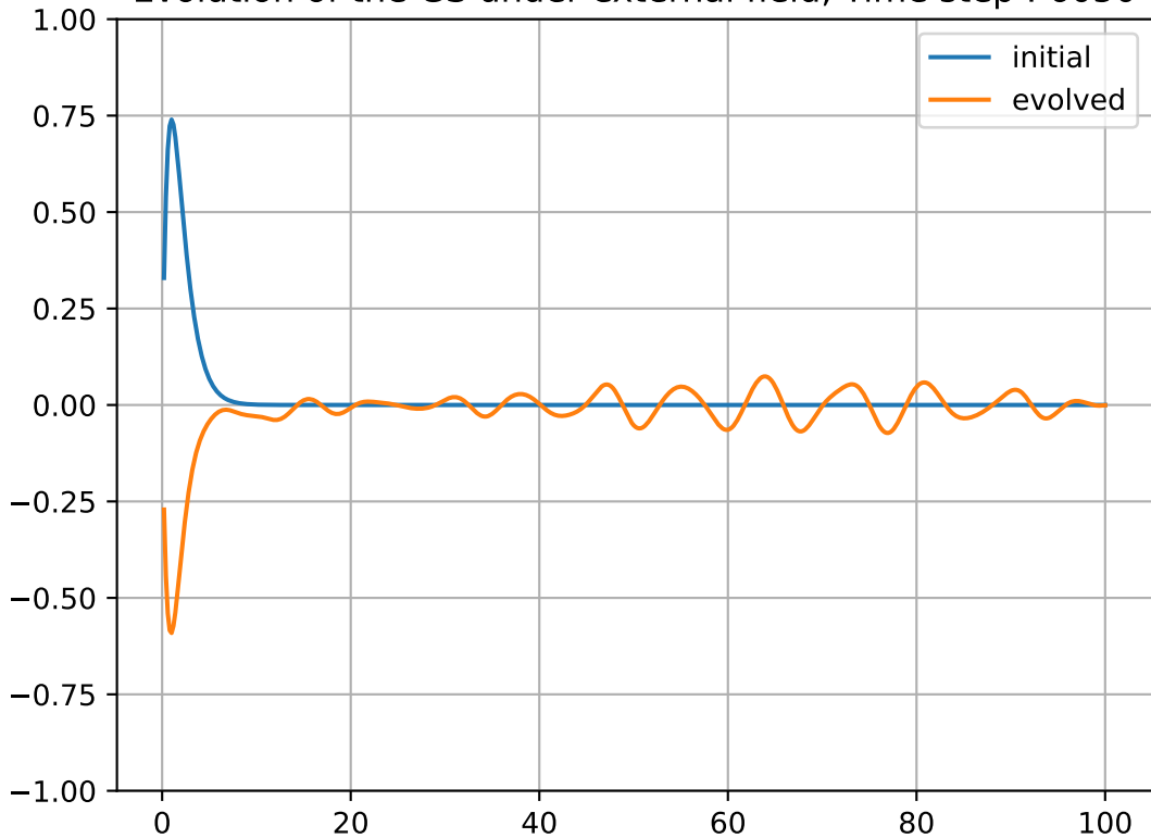
Evolution of the GS under external field, Time step : 6050
