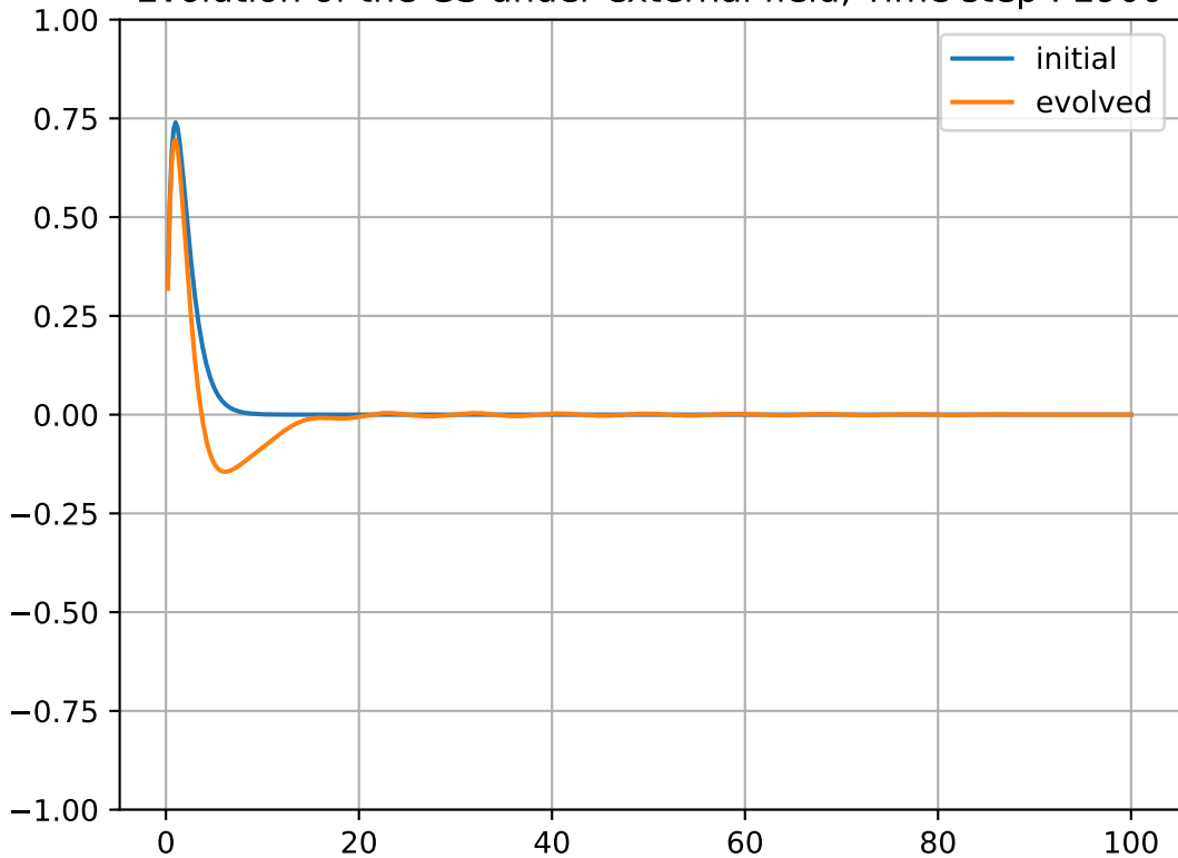
Evolution of the GS under external field, Time step : 2900
