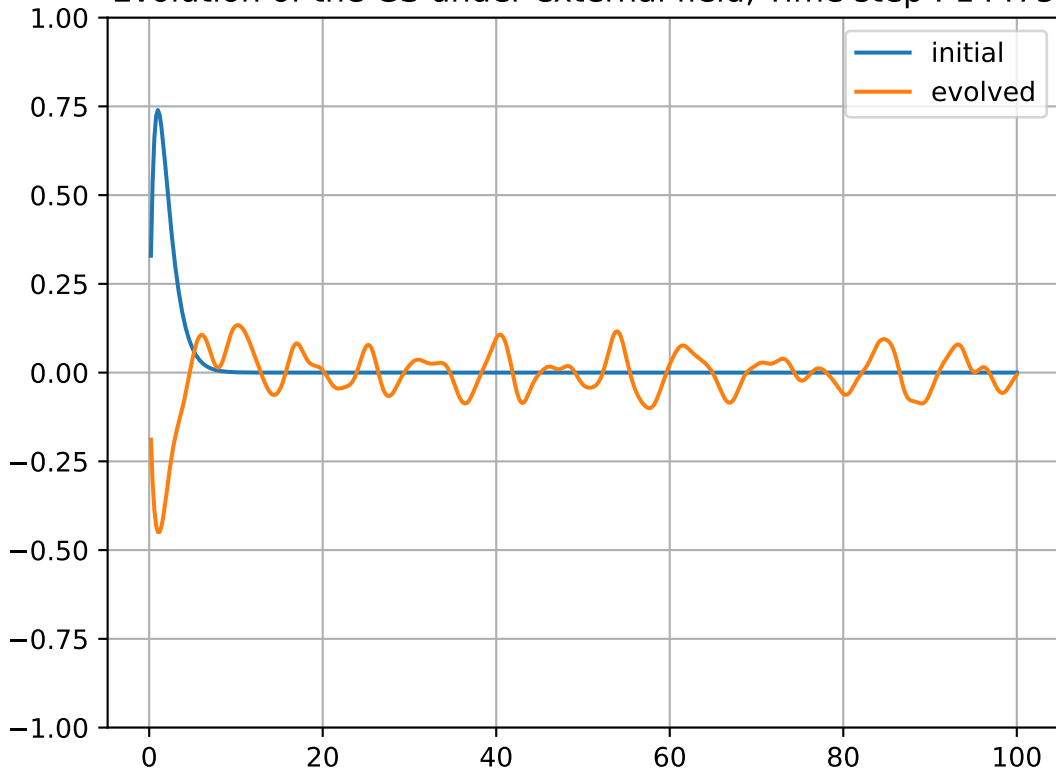
Evolution of the GS under external field, Time step : 14475
