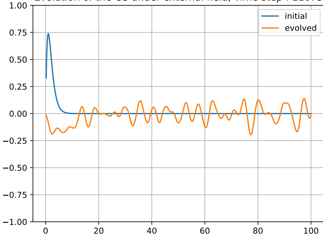
Evolution of the GS under external field, Time step : 11075
