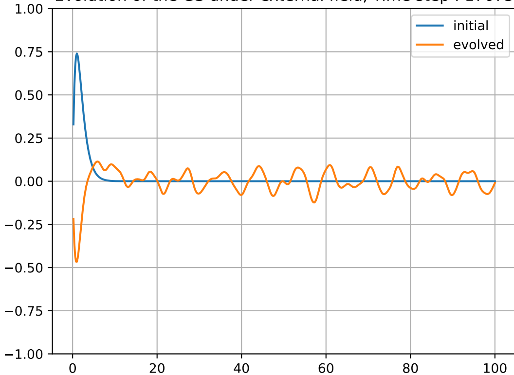
Evolution of the GS under external field, Time step : 17075
