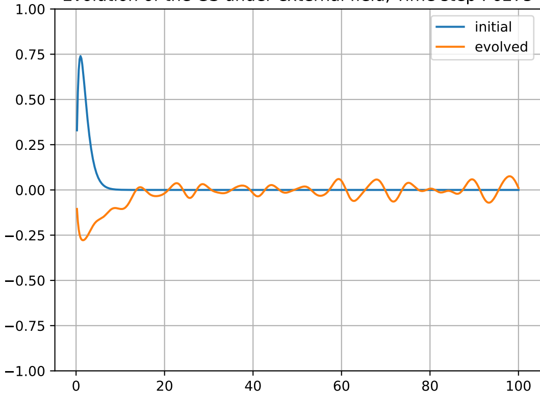
Evolution of the GS under external field, Time step : 6275
