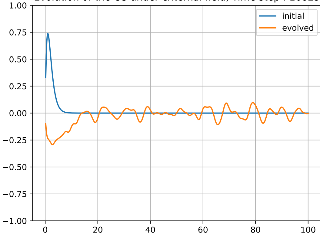
Evolution of the GS under external field, Time step : 16825
