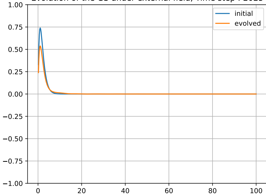
Evolution of the GS under external field, Time step : 2025
