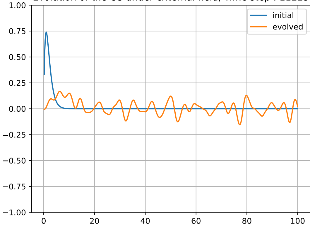
Evolution of the GS under external field, Time step : 11225
