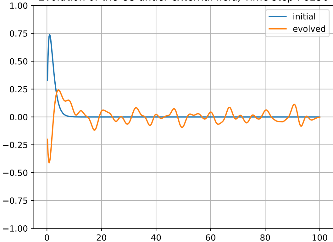
Evolution of the GS under external field, Time step : 8250
