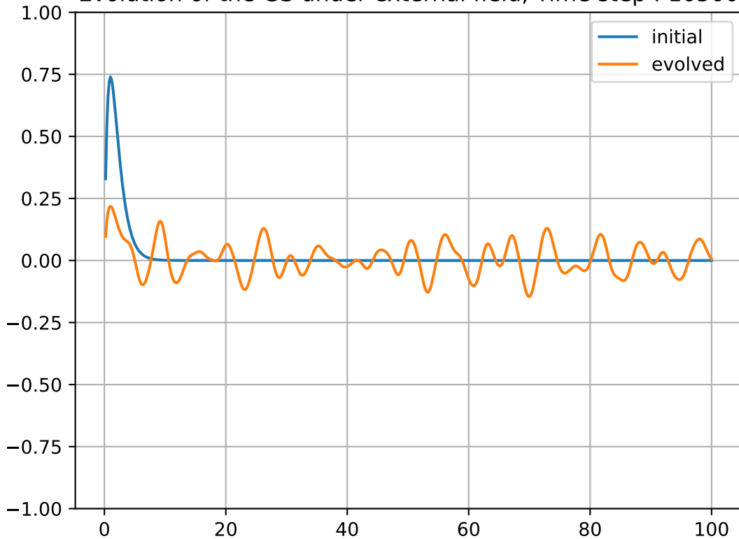
Evolution of the GS under external field, Time step : 10500
