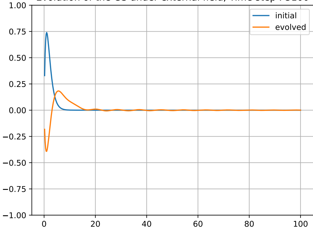
Evolution of the GS under external field, Time step : 3100
