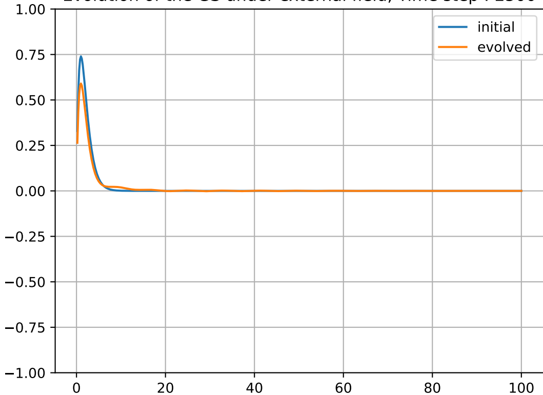
Evolution of the GS under external field, Time step : 2500
