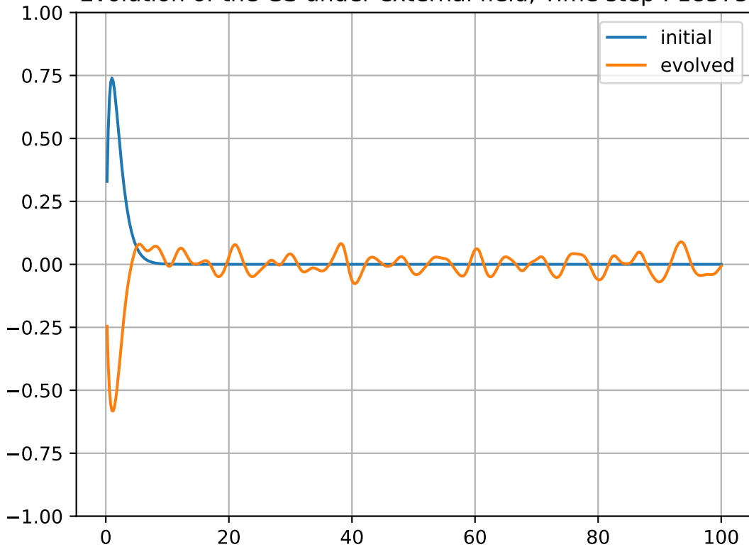
Evolution of the GS under external field, Time step : 18575
