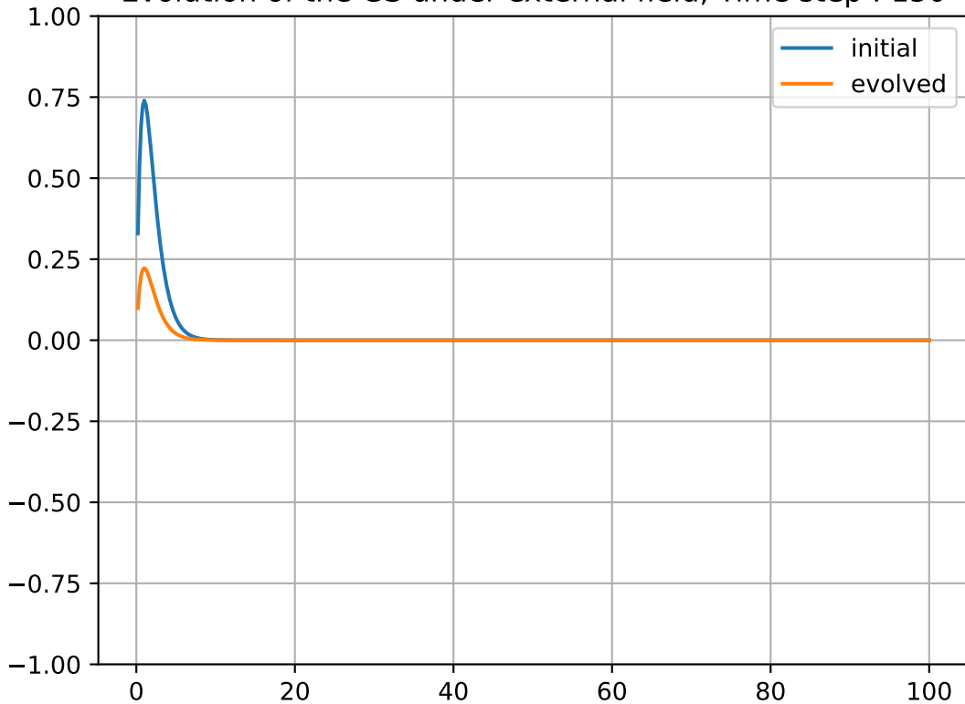
Evolution of the GS under external field, Time step : 150
