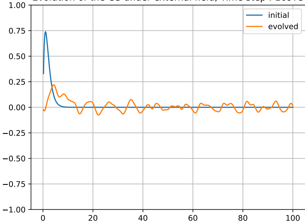
Evolution of the GS under external field, Time step : 16975
