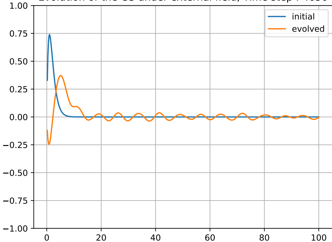
Evolution of the GS under external field, Time step : 4650
