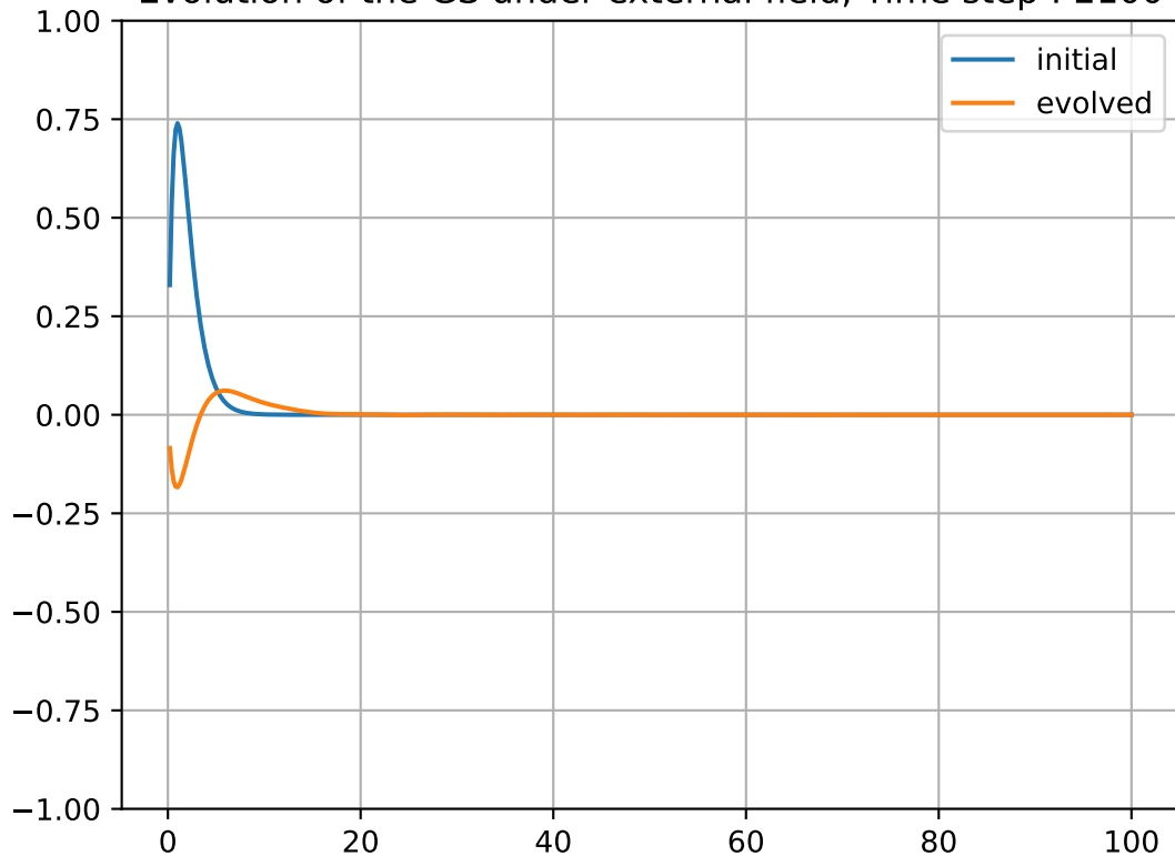
Evolution of the GS under external field, Time step : 2100
