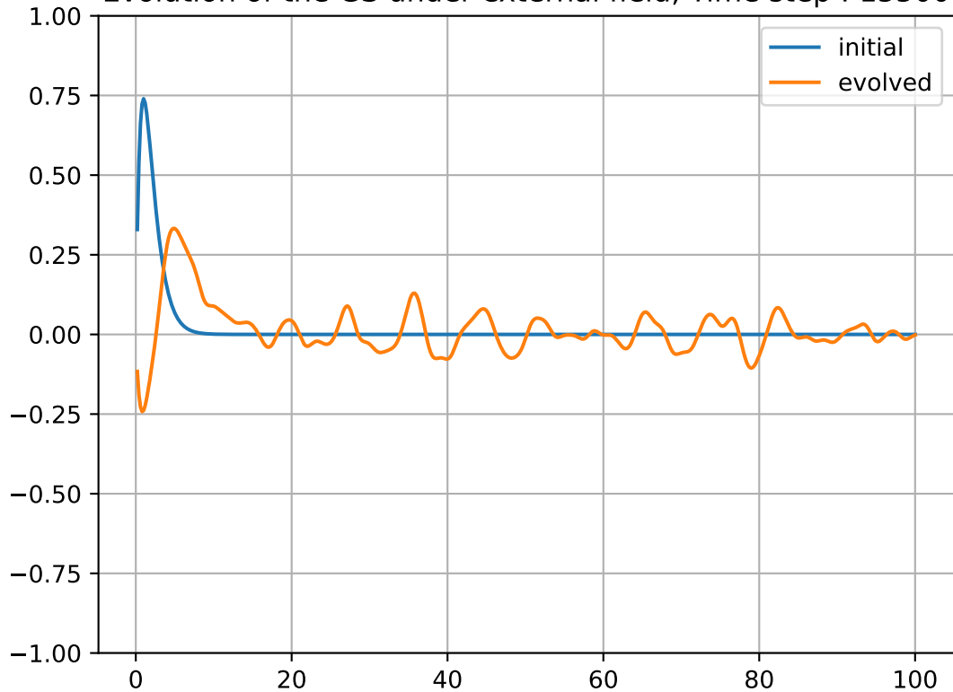
Evolution of the GS under external field, Time step : 15500
