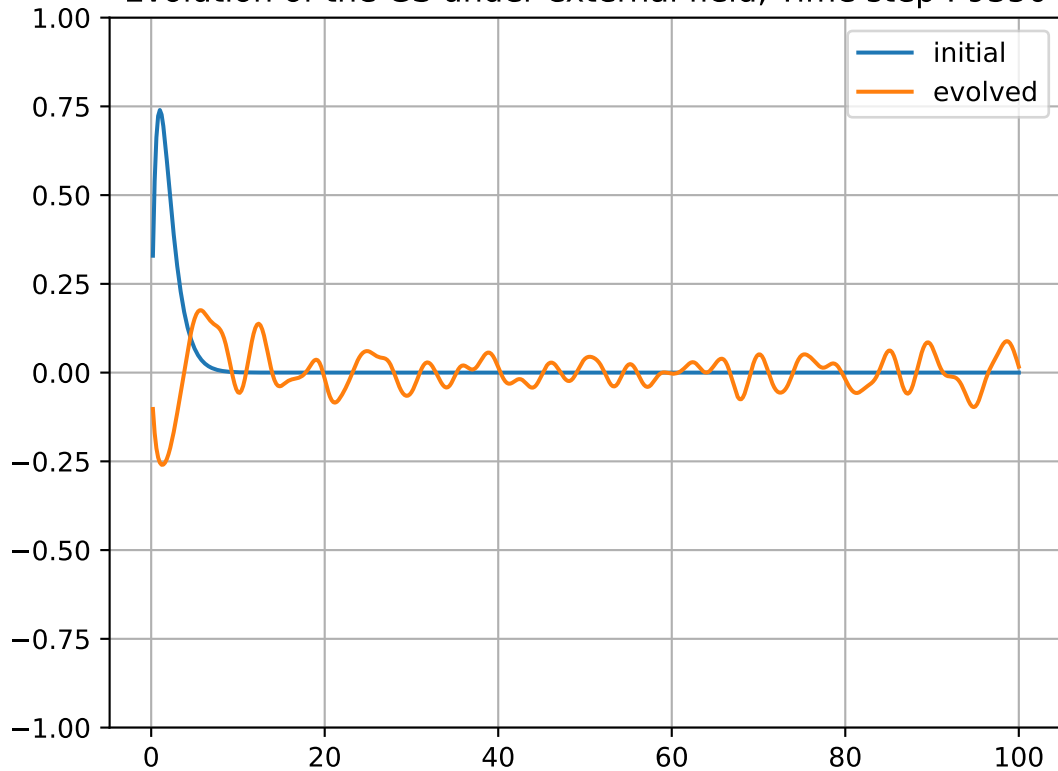
Evolution of the GS under external field, Time step : 9350
