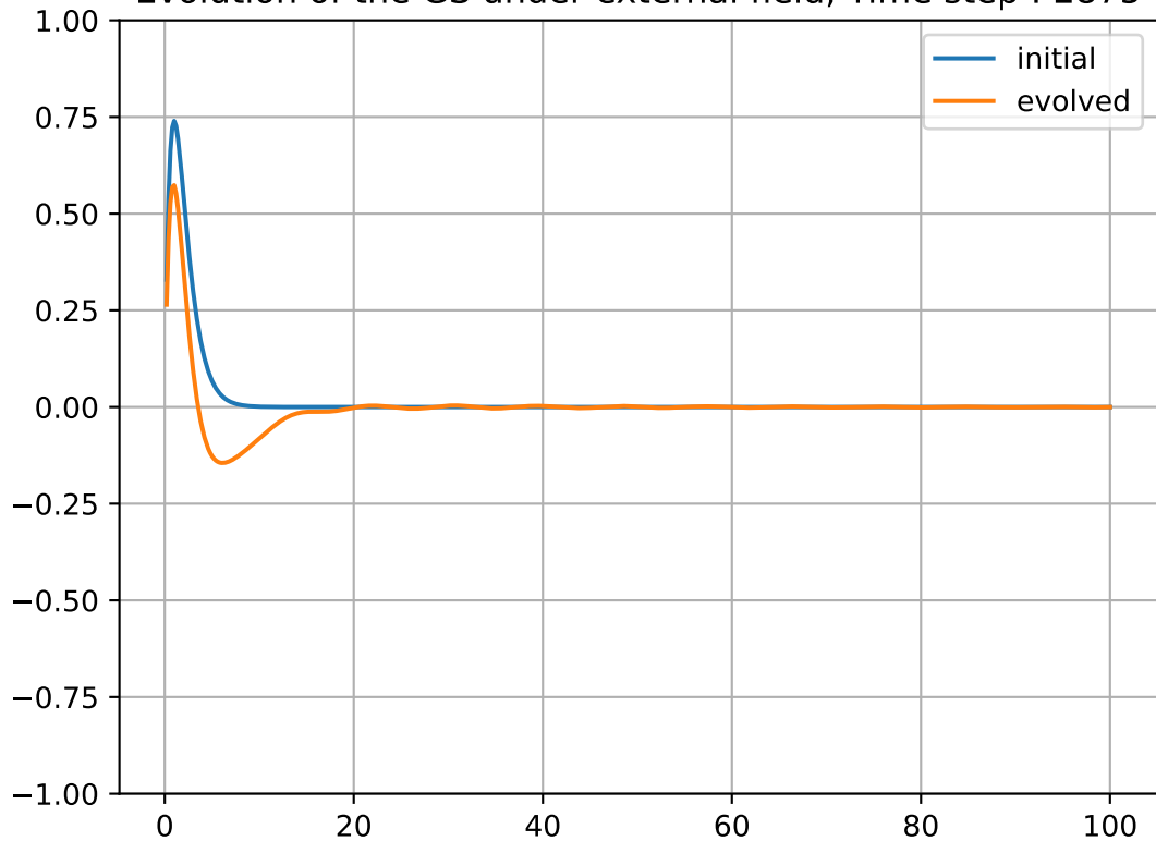
Evolution of the GS under external field, Time step : 2875
