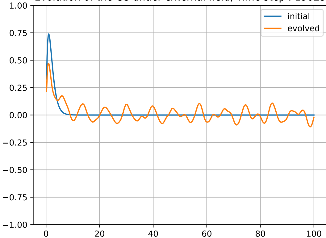
Evolution of the GS under external field, Time step : 19025
