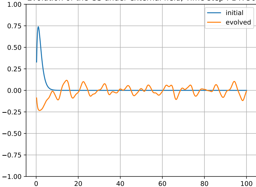
Evolution of the GS under external field, Time step : 14750
