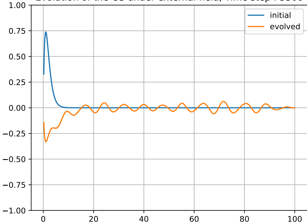
Evolution of the GS under external field, Time step : 5300
