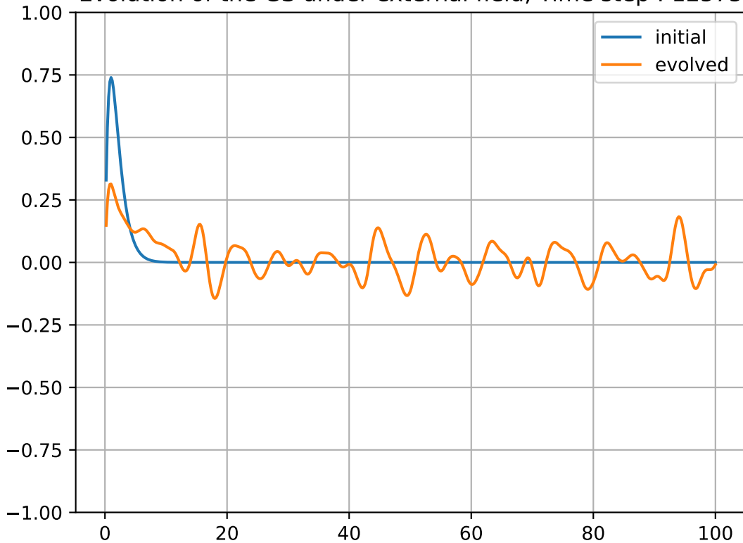
Evolution of the GS under external field, Time step : 12575
