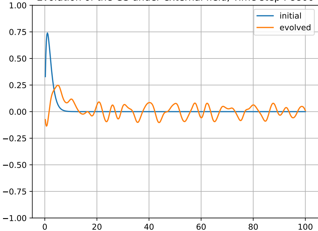
Evolution of the GS under external field, Time step : 8800
