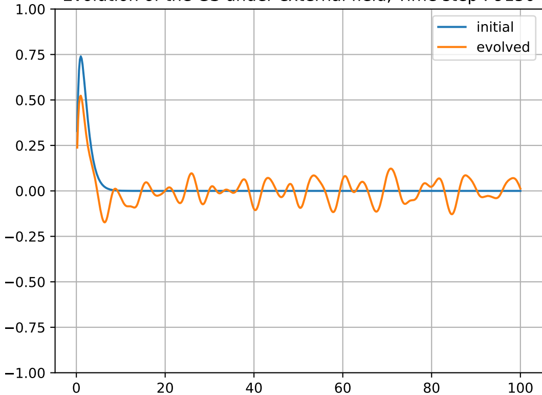
Evolution of the GS under external field, Time step : 9150
