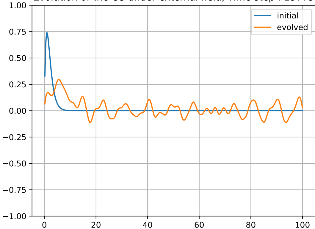
Evolution of the GS under external field, Time step : 13775
