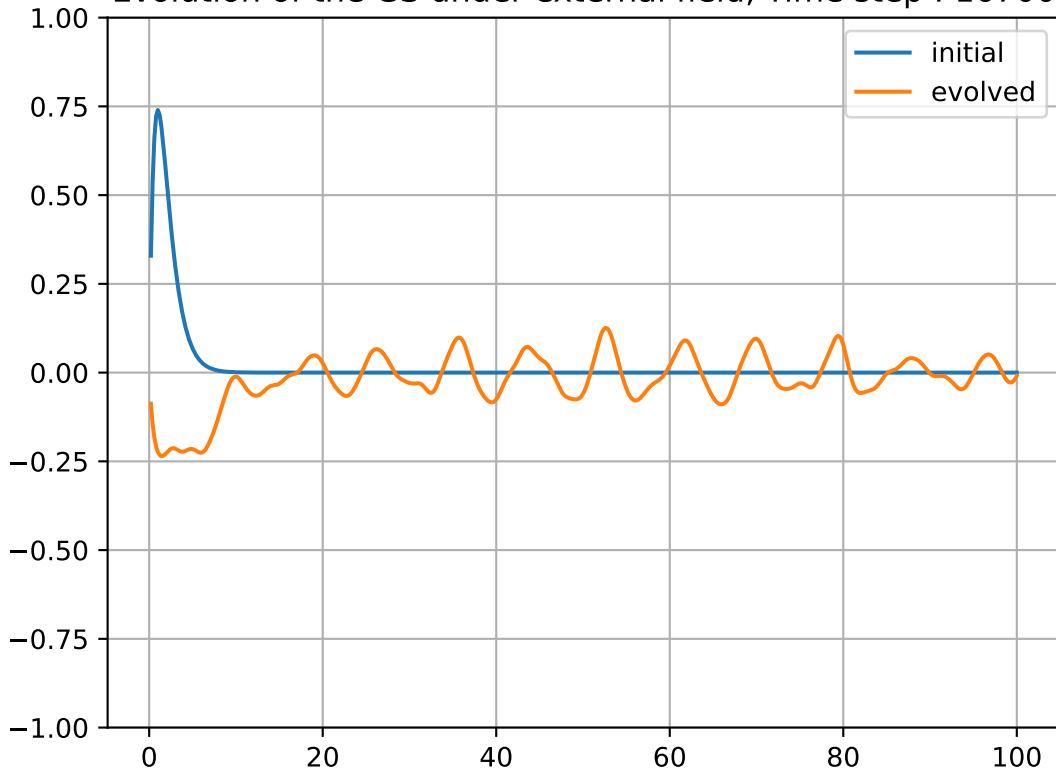
Evolution of the GS under external field, Time step : 16700
