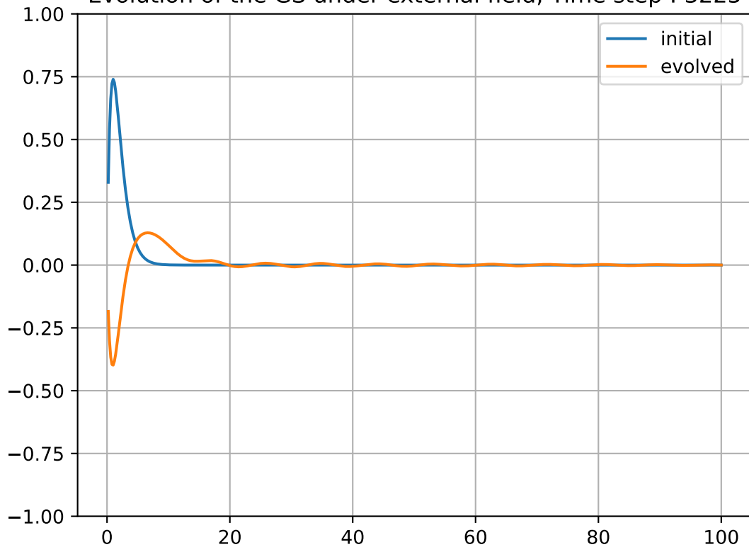
Evolution of the GS under external field, Time step : 3225
