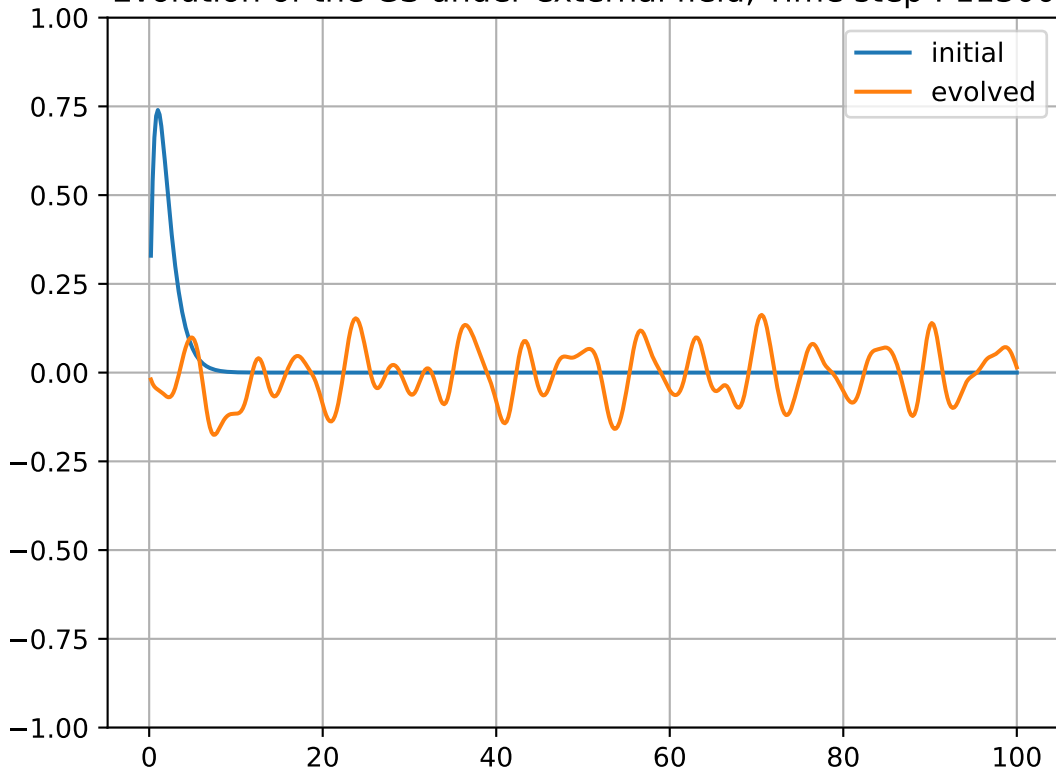
Evolution of the GS under external field, Time step : 11300
