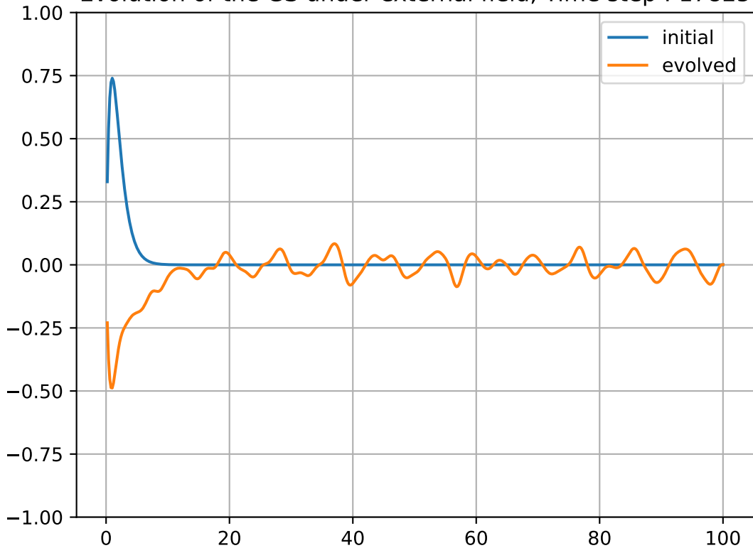
Evolution of the GS under external field, Time step : 17825
