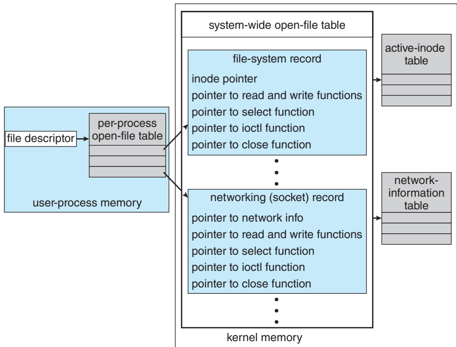
Figure 12.13 UNIX I/O kernel structure.
