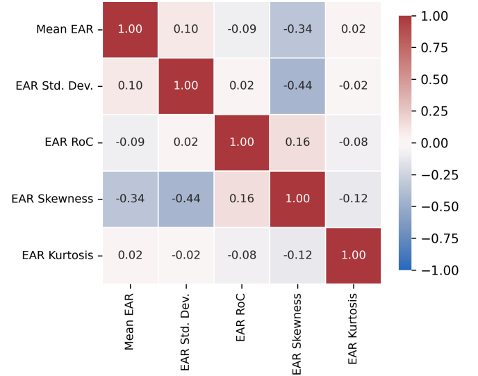
Fig. 3. Feature orthogonality (computed from the full 451,515-window dataset, SEED = 42). The largest off-diagonal correlation is r = -0.44 between Std. Dev. and Skewness; all remaining pairs stay below |r| = 0.35 . No two features carry the same physiological information.
