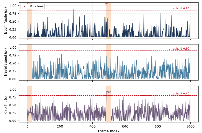
Fig. 9. One 1,000-frame session of the simulated CAN-bus telemetry (SEED=42). Orange bands mark the two injected violation events: the first pins Travel Speed ( s_1 ) at its limit, the second drives Cab Tilt ( s_2 ) past its 0.80 threshold. Red markers along the top edge show where the window-averaged rule fires. Despite ADC noise on every channel, no firing occurs outside the injected events — the zero false-positive rate of Table X, drawn instead of tabulated.
