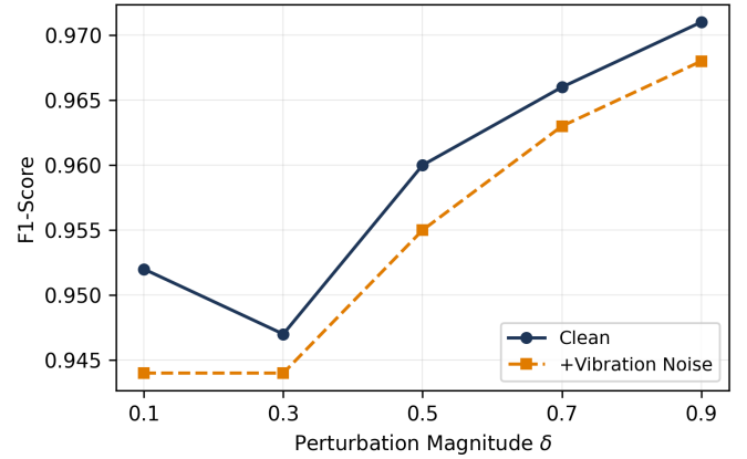
Fig. 8. F1-Score versus perturbation magnitude \delta , clean and under simulated camera vibration. The noise penalty stays bounded below 0.008 across the entire fatigue spectrum, and shrinks as fatigue deepens.
