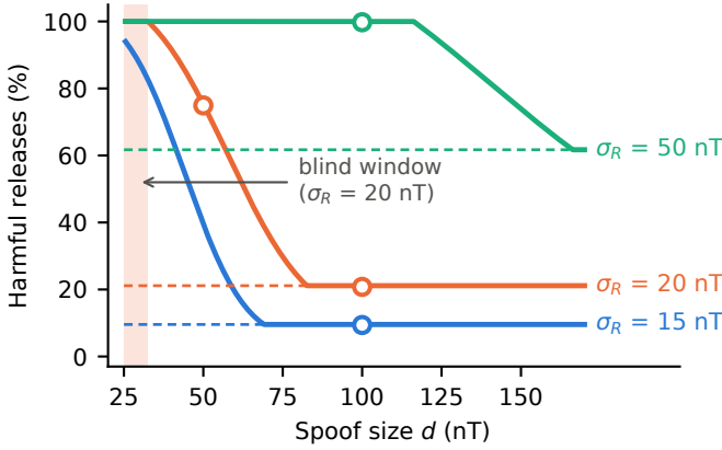
Fig. 2. Fallback harm from Eq. (3) (lines, post hoc), reference floors (dashed), and frozen-run observations with 95% intervals (circles). Shading: blind window at \sigma_R = 20 nT, spoofs of 25–32.6 nT that are harmful but raise no alarm.
