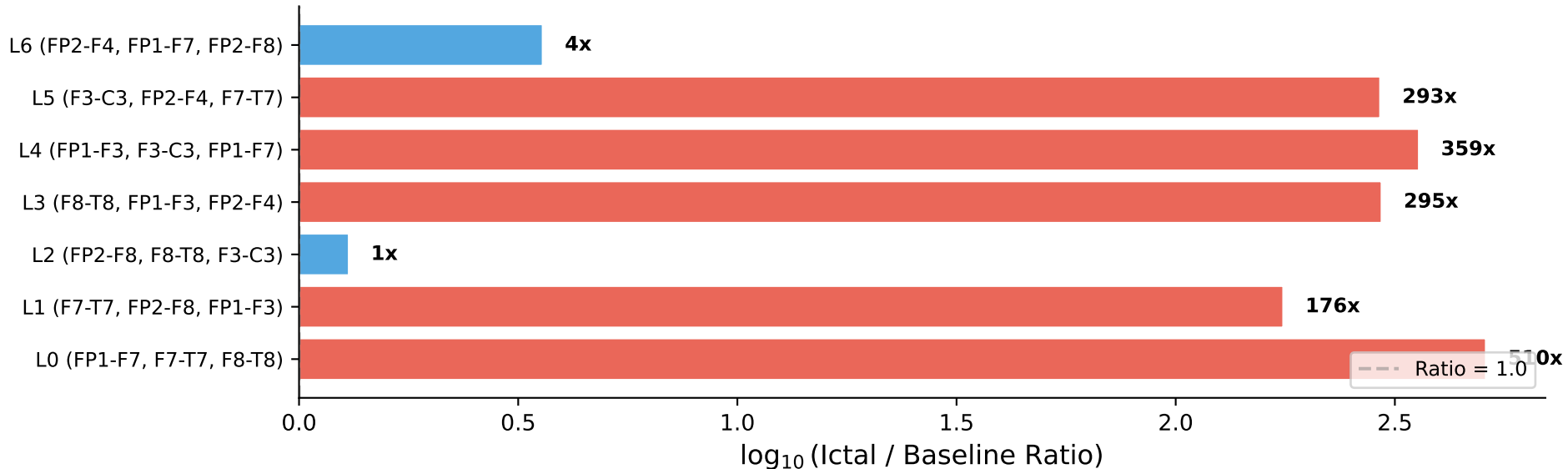
Fano-Line Decomposition: Patient 3 (chb03, trained A)
