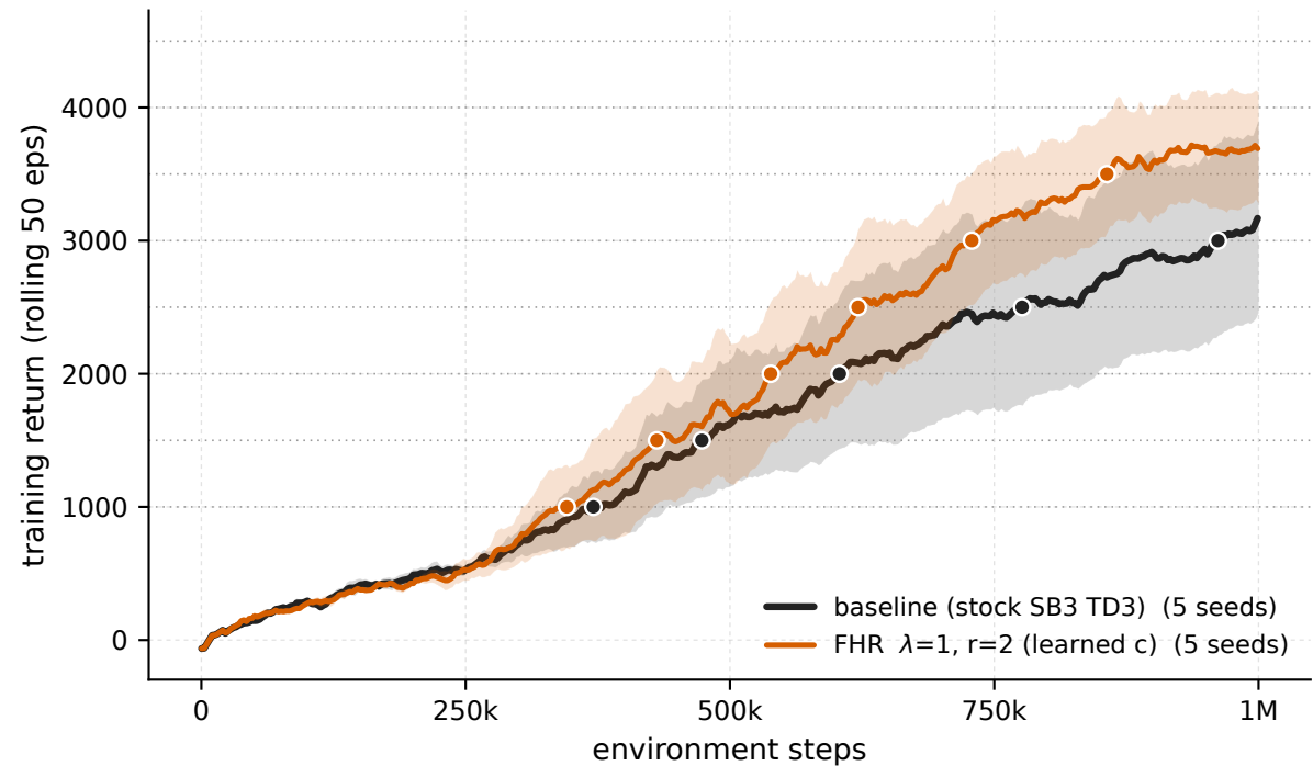
Ant-v5 - \lambda 1 \cdot r2 vs baseline (training stream)
