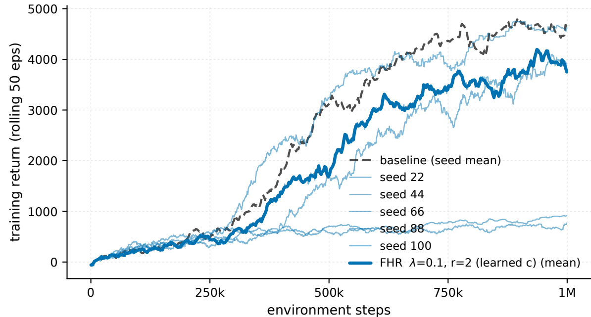
Ant-v5 - \lambda 0.1 \cdot r_2 , every seed (train)
