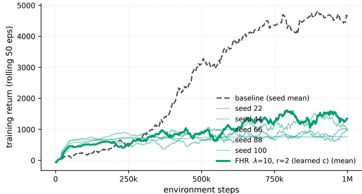
Ant-v5 - \lambda 10 \cdot r_2 , every seed (train)
