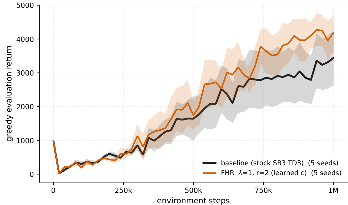
Ant-v5 - \lambda 1 \cdot r_2 vs baseline (greedy eval)
