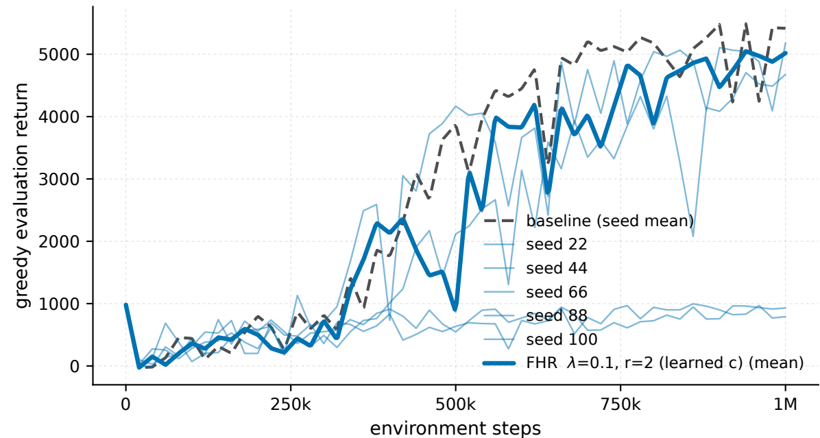
Ant-v5 - \lambda 0.1 \cdot r2 , every seed (eval)
