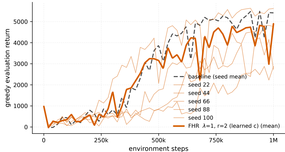
Ant-v5 - \lambda 1 \cdot r_2 , every seed (eval)
