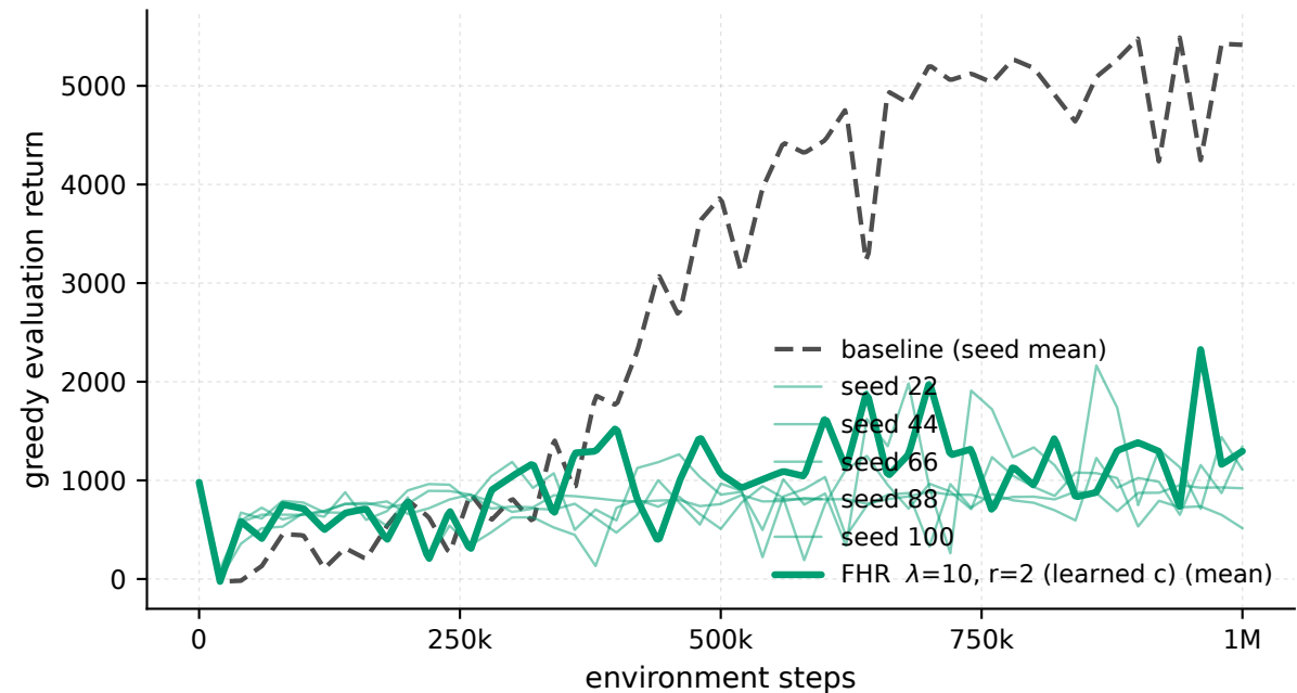
Ant-v5 - \lambda 10 \cdot r_2 , every seed (eval)
