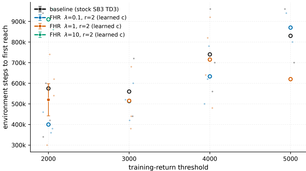
Ant-v5 - sample efficiency, greedy-eval stream (mean \pm 1 s.e.) open marker: not all seeds reached it
