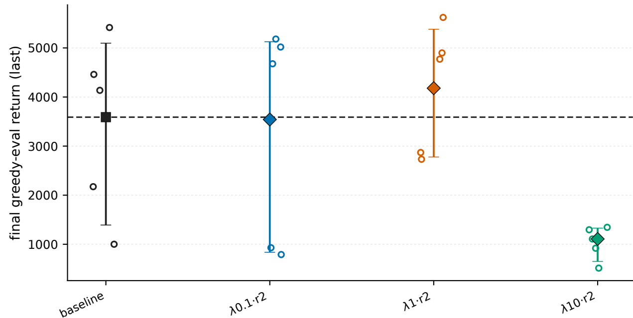
Ant-v5 - final return per arm: seeds (o), IQM with 95% bootstrap CI; dashed = baseline IQM
