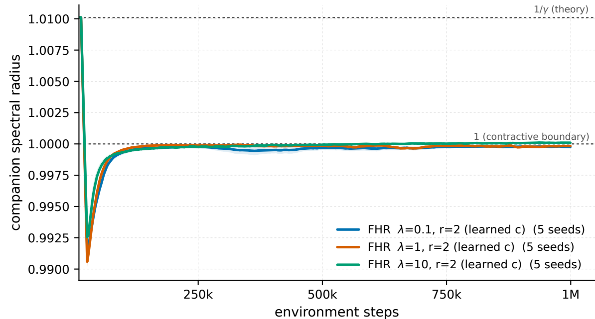
Ant-v5 - companion spectral radius
