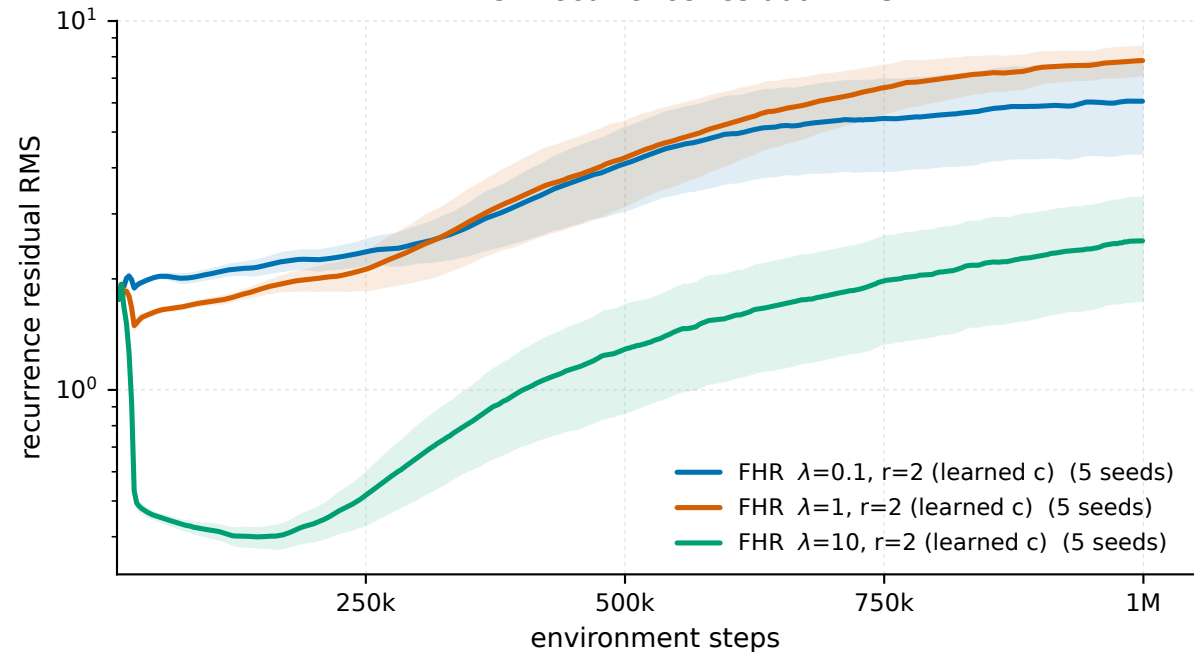
Ant-v5 - recurrence residual RMS
