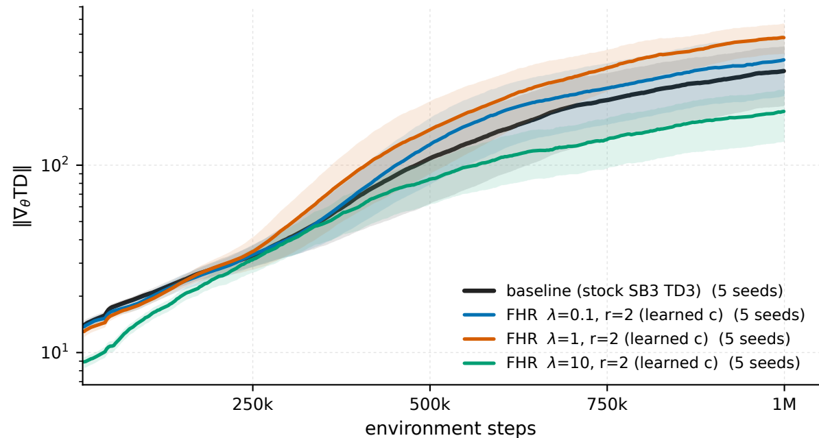
Ant-v5 - \|\nabla_{\theta}TD\|
