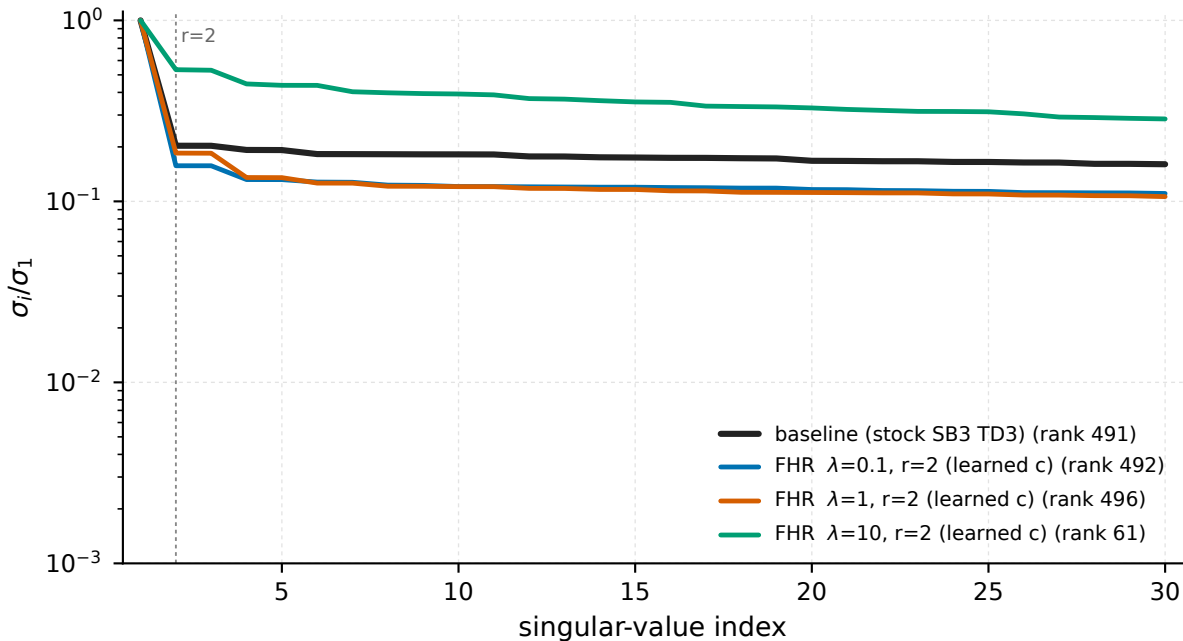
Ant-v5 - \text{Hankel}(\pi(s_t)_1) of the final policy (action dim 1)
