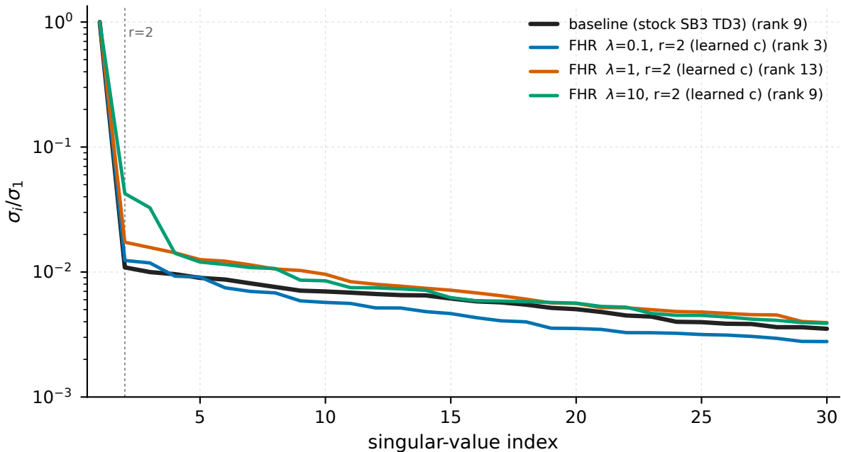
Ant-v5 - Hankel( Q(s_t, \pi(s_t)) ) of the final policy (critic trace)
