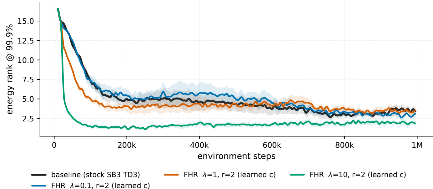
Ant-v5 - penalised windows, all arms energy rank @ 99.9%
