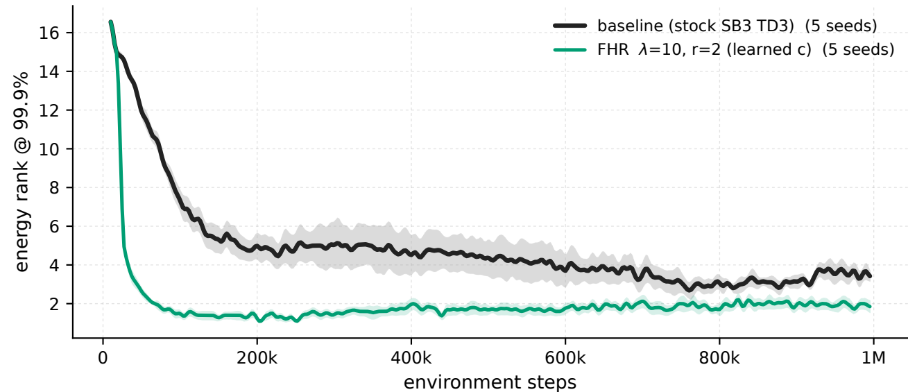
Ant-v5 - \lambda 10 \cdot r_2 vs baseline, penalised windows energy rank @ 99.9%
