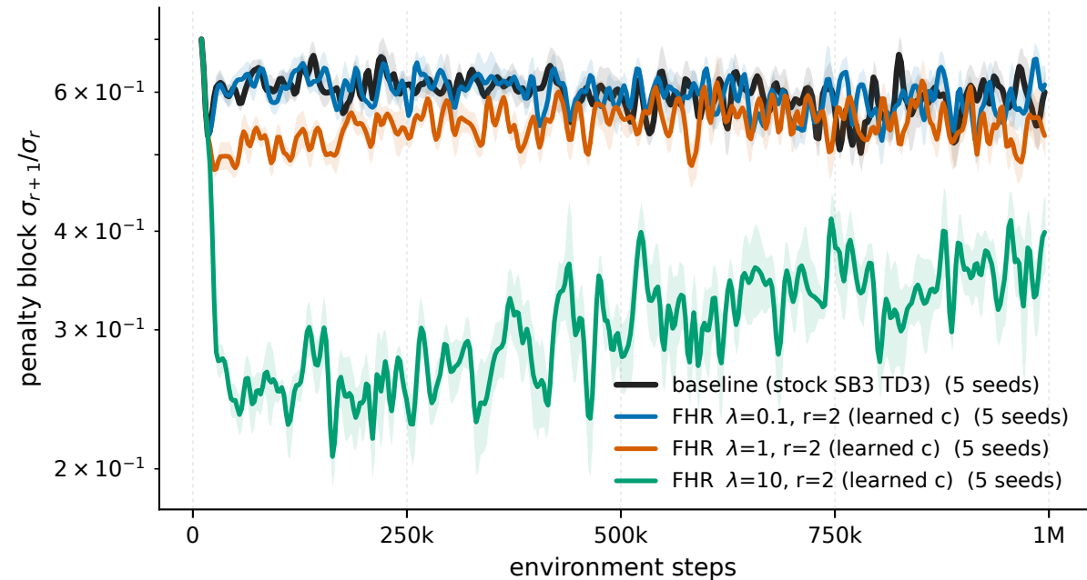
Ant-v5 - penalised windows: \sigma_{r+1}/\sigma_r of the penalty block
