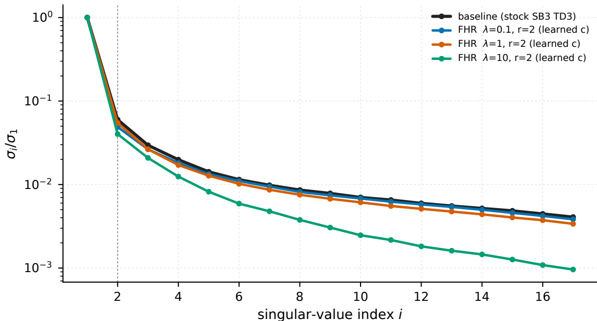
Ant-v5 - replay window spectrum, final 25% of training (median over seeds and critics)
