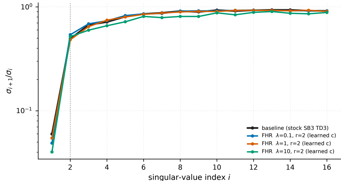
Ant-v5 - replay window spectrum, final 25% of training (median over seeds and critics)
