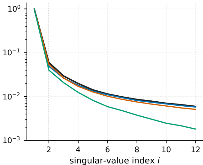
penalised replay windows, final quarter
