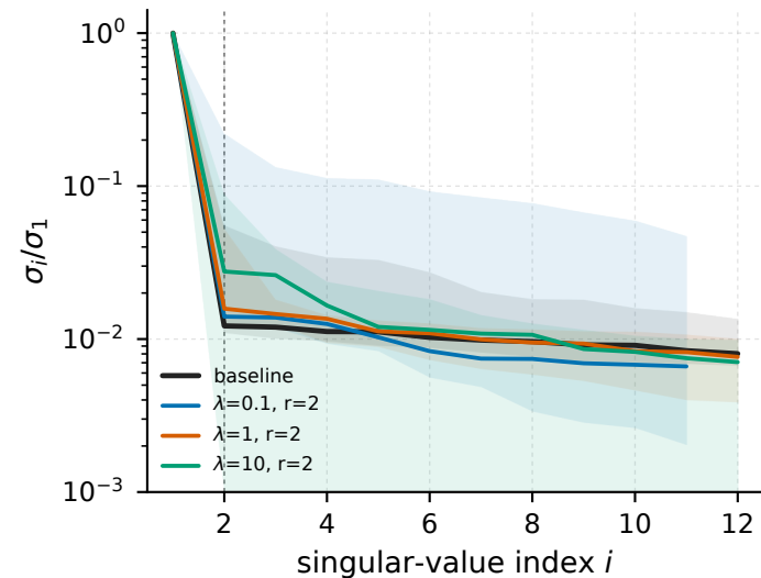
rollout Hankel( Q(s_t, \pi(s_t)) ), final policy
