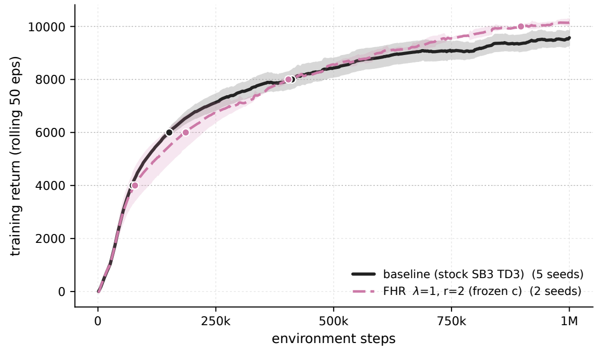
HalfCheetah-v5 - \lambda 1 \cdot r 2 frozen-c vs baseline (training stream)
