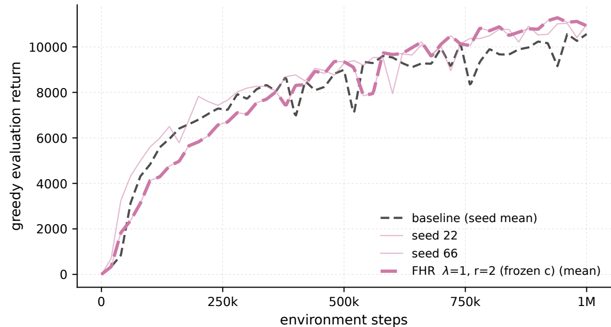
HalfCheetah-v5 - \lambda 1 \cdot r_2 frozen-c, every seed (eval)
