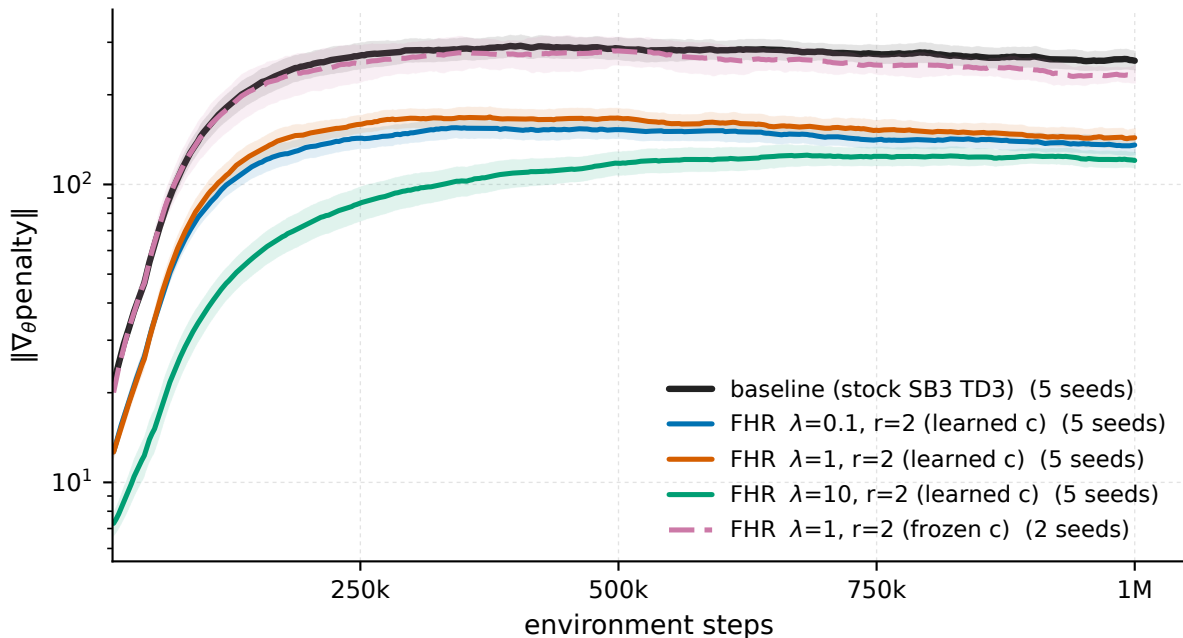
HalfCheetah-v5 - \|\nabla_{\theta}\text{penalty}\|
