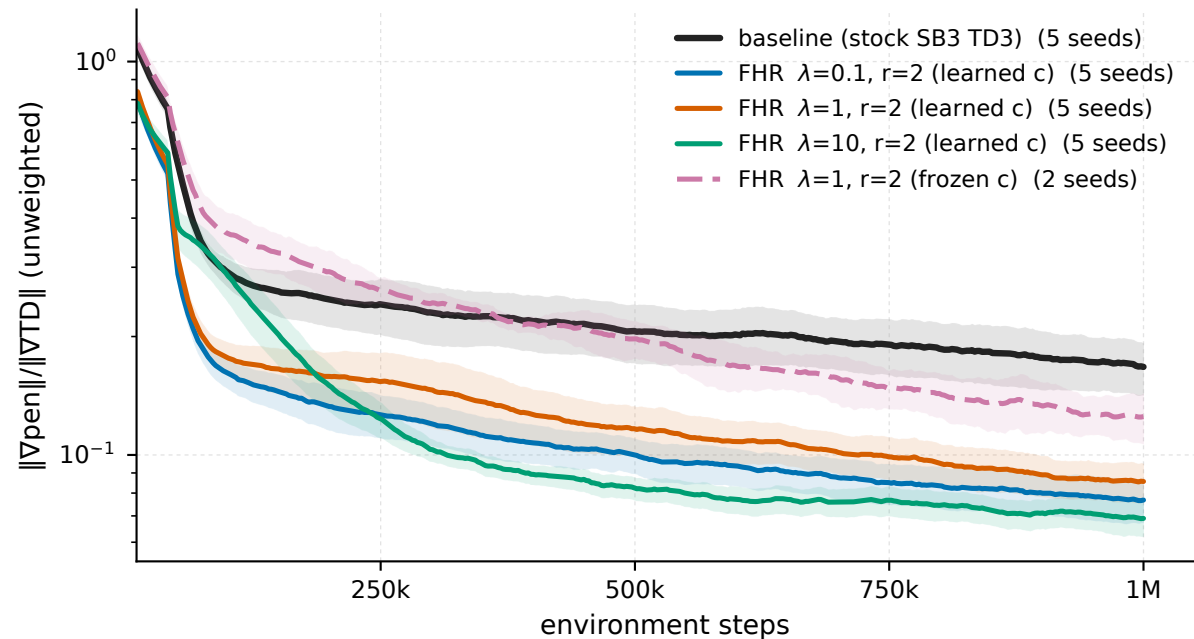
HalfCheetah-v5 - \|\nabla_{\text{pen}}\|/\|\nabla_{\text{TD}}\| (unweighted)
