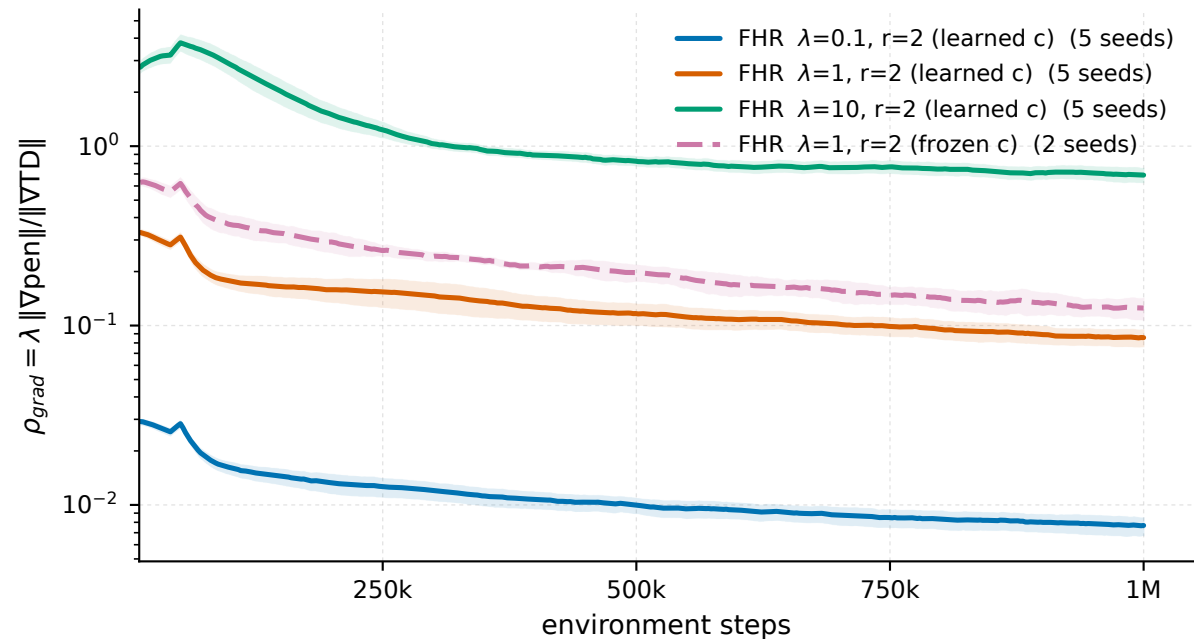
HalfCheetah-v5 - \rho_{grad} = \lambda \|\nabla pen\|/\|\nabla TD\|
