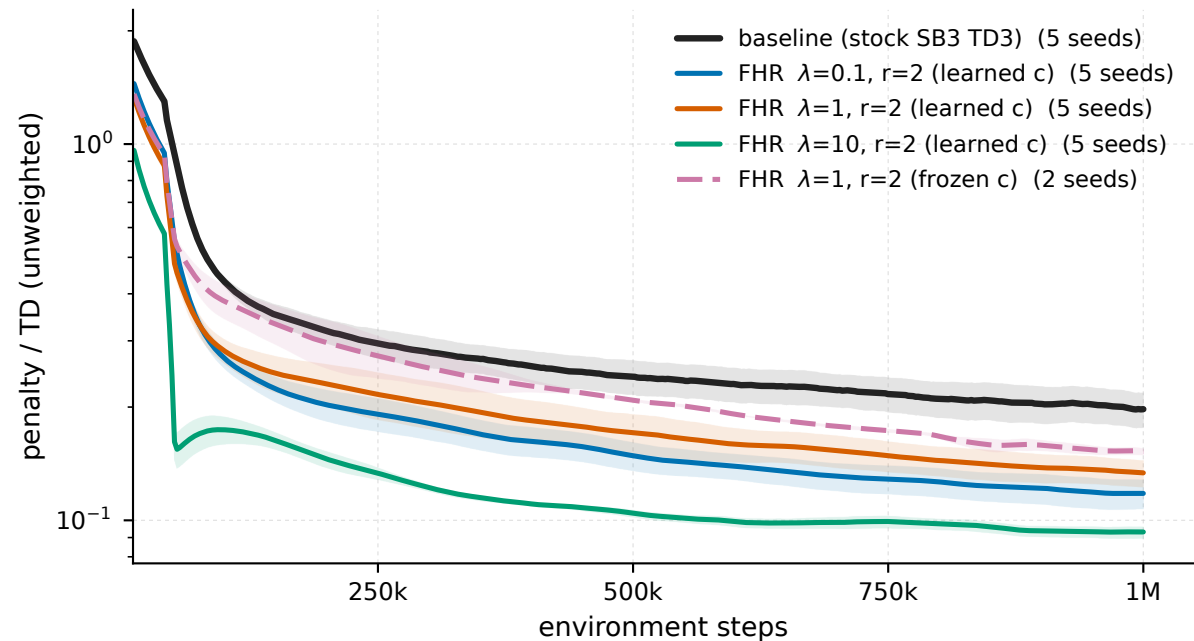
HalfCheetah-v5 - penalty / TD (unweighted)
