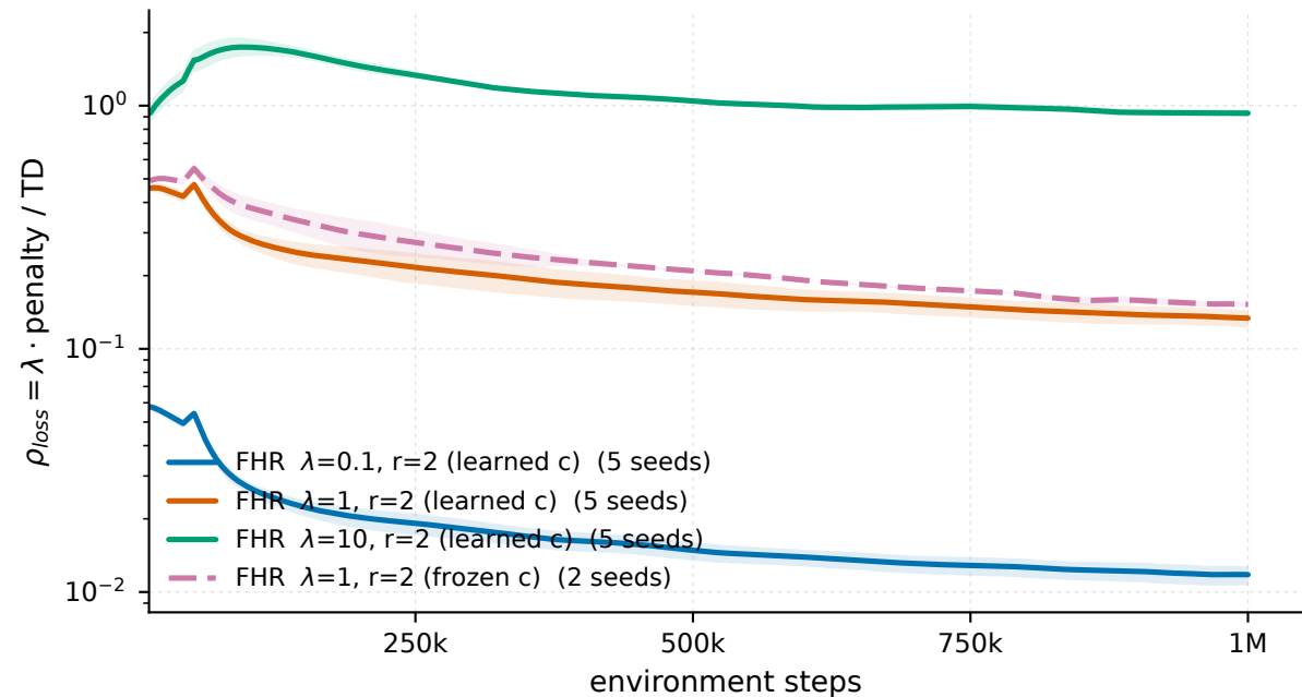
HalfCheetah-v5 - \rho_{loss} = \lambda \cdot \text{penalty} / \text{TD}
