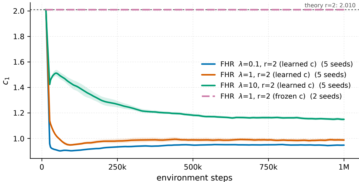
HalfCheetah-v5 - recurrence coefficient c_1 vs the Bellman theory value
