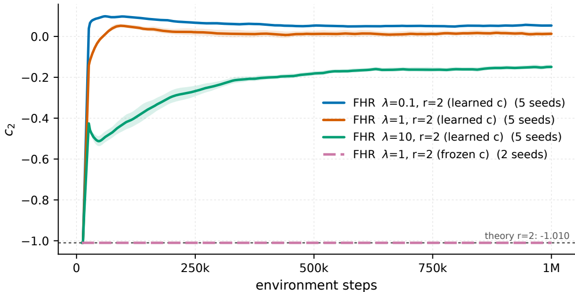
HalfCheetah-v5 - recurrence coefficient c_2 vs the Bellman theory value
