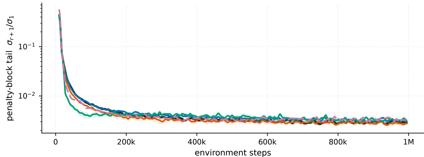
HalfCheetah-v5 - penalised windows, all arms penalty-block tail \sigma_{r+1}/\sigma_1
