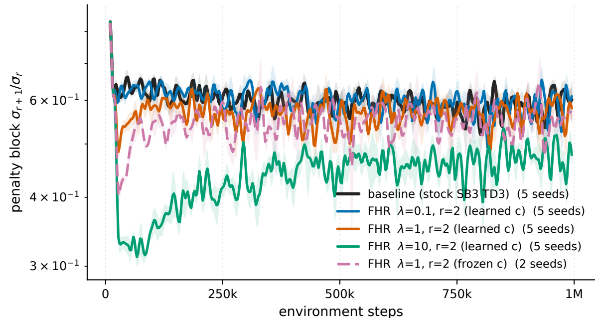
HalfCheetah-v5 - penalised windows: \sigma_{r+1}/\sigma_r of the penalty block
