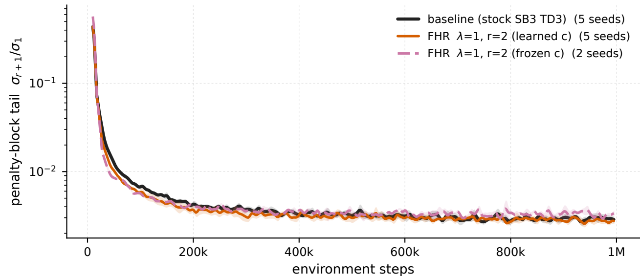
HalfCheetah-v5 - \lambda 1 \cdot r_2 , \lambda 1 \cdot r_2 frozen-c vs baseline, penalised windows penalty-block tail \sigma_{r+1}/\sigma_1
