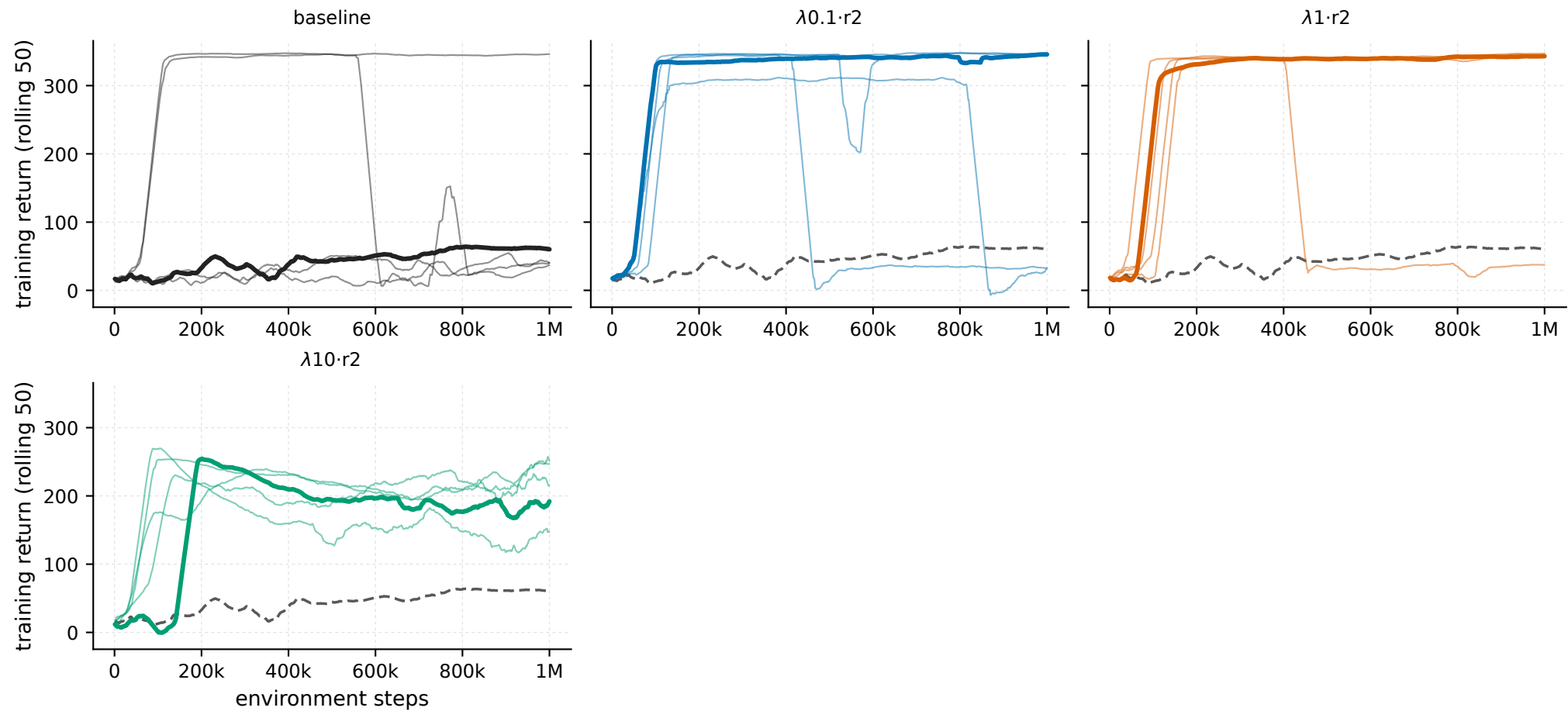
Swimmer-v5 - every seed per arm (train); grey dashed = baseline seed mean
