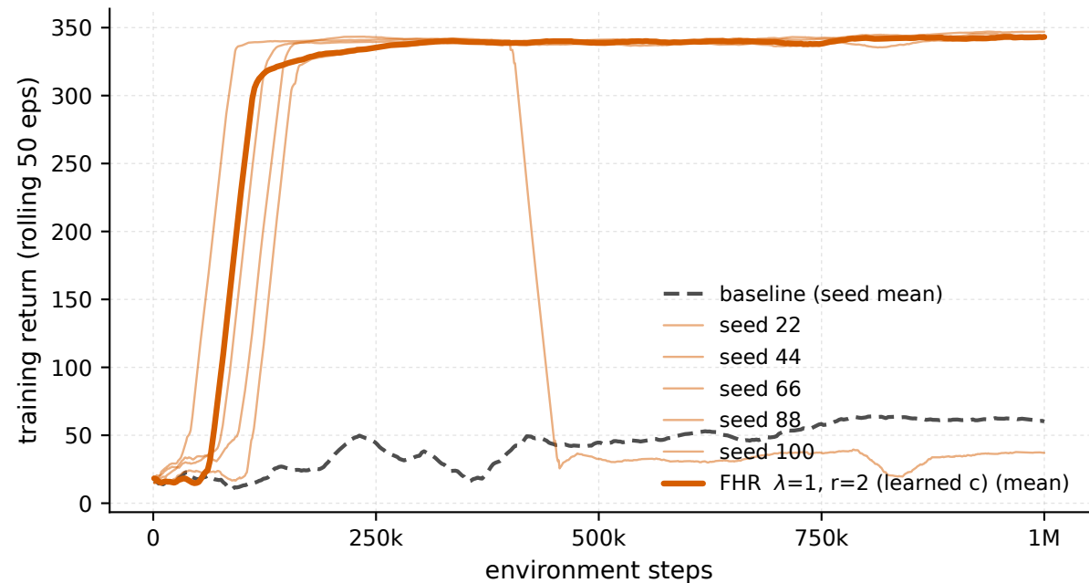
Swimmer-v5 - \lambda 1 \cdot r_2 , every seed (train)
