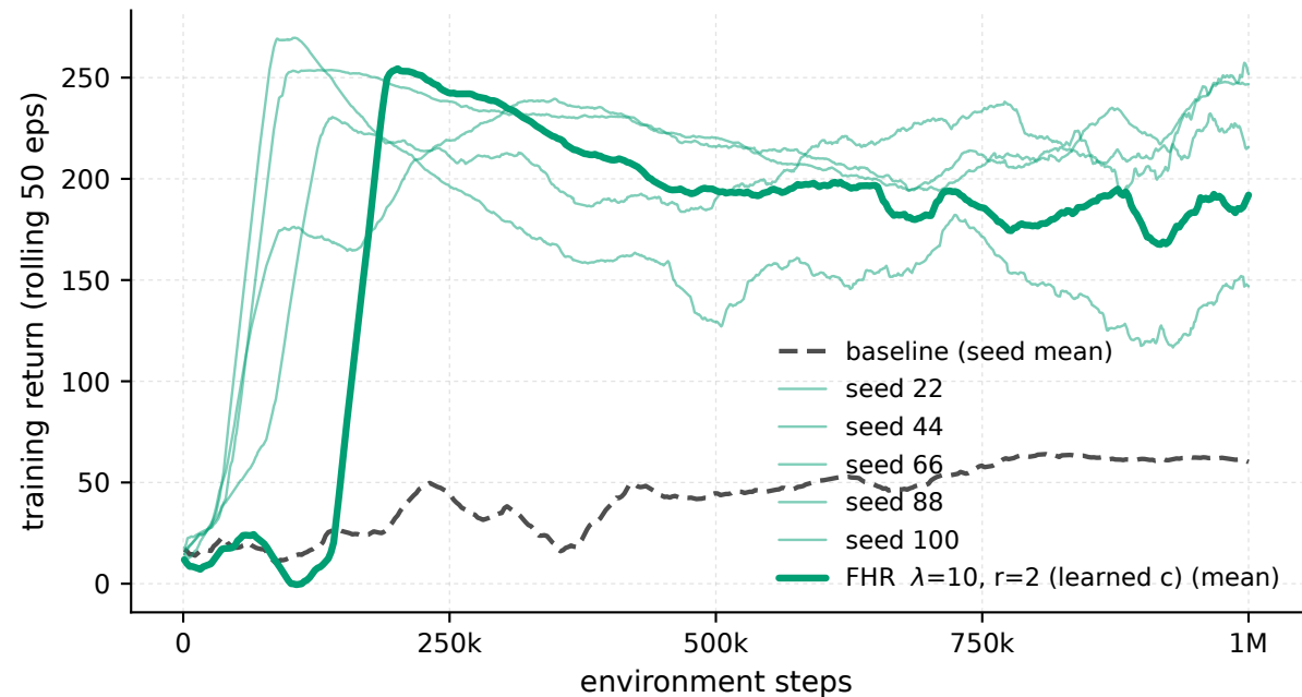
Swimmer-v5 - \lambda 10 \cdot r2 , every seed (train)
